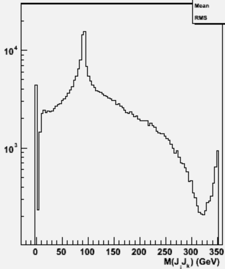
2jets mass(All comb)w100589 uubb_o
