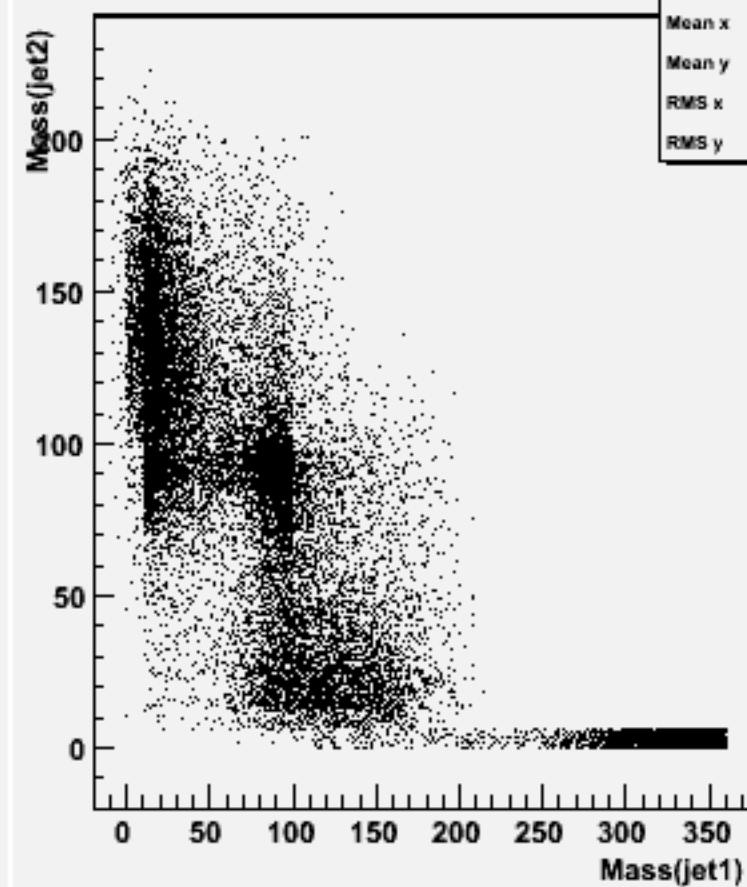
Jet mass for forced 2-jets : w100589 uubb_o
