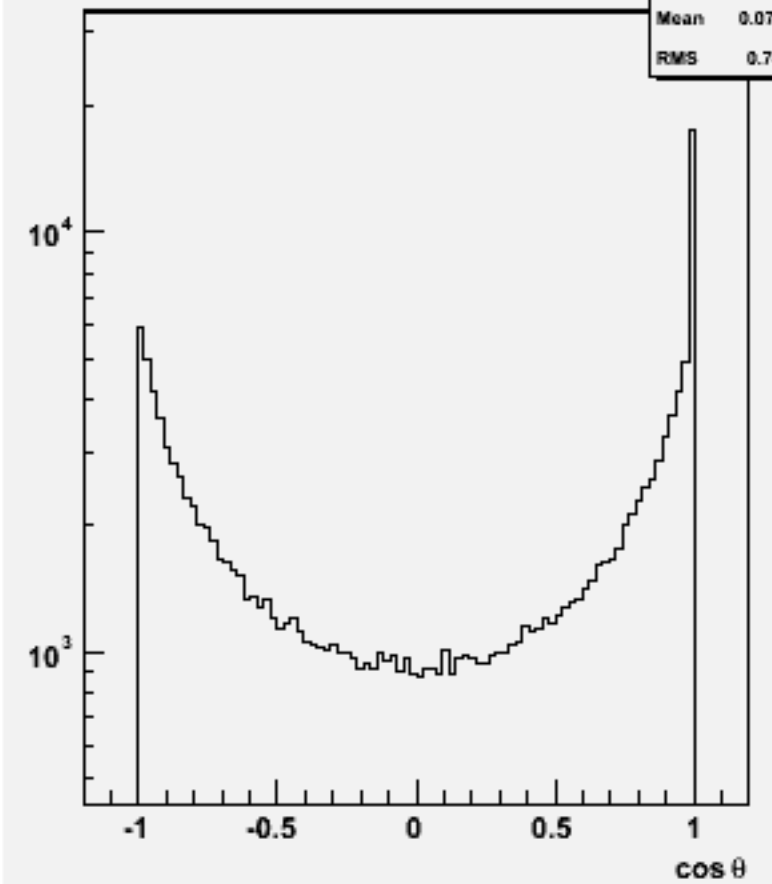
Jet cosθ (All jets)w100589 uubb_o
