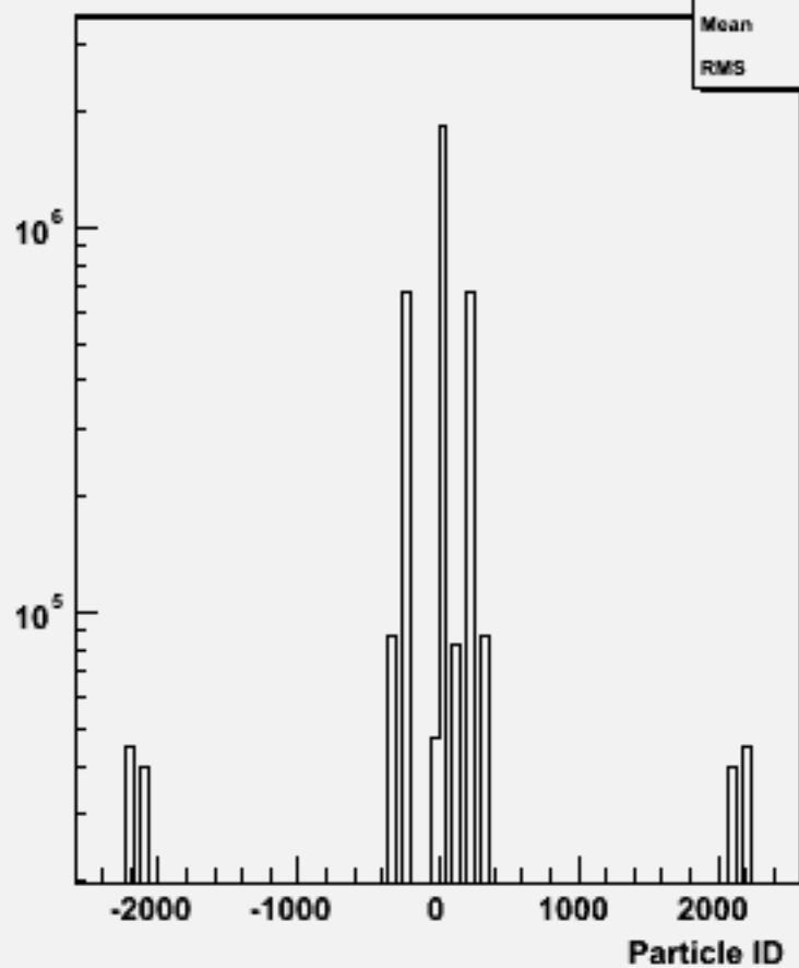
Particle ID : w100589 uubb_o
