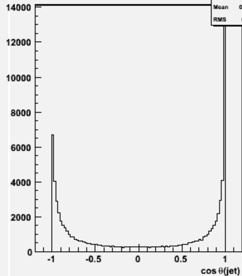
cos \theta for 2-jets :w100589 uubb_o
