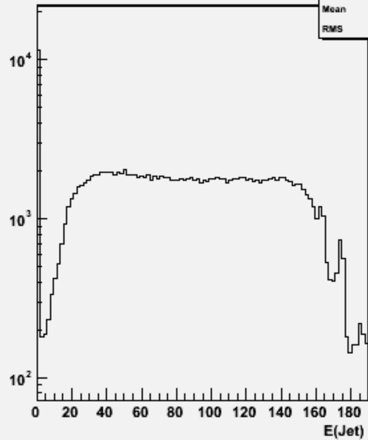
Jet energies(All jets)w100589 uubb_o
