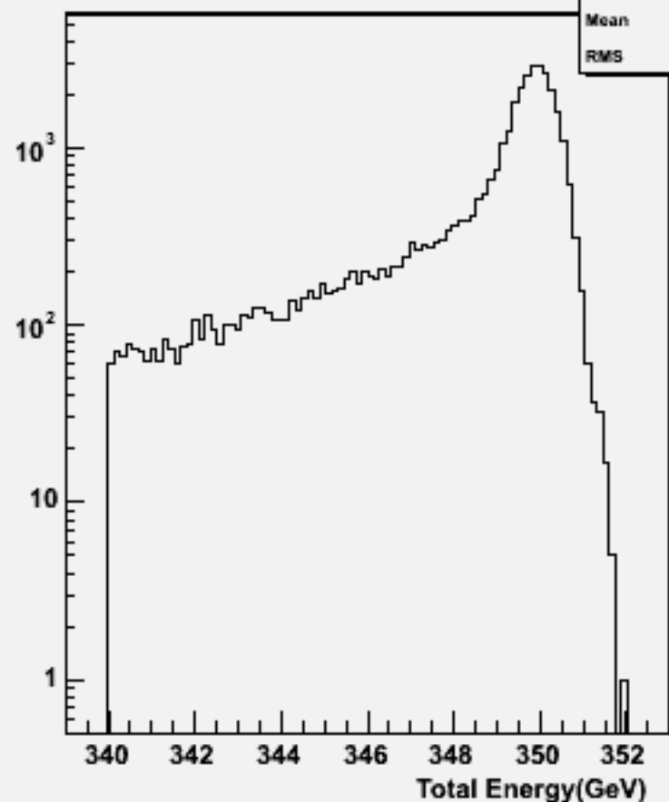
Total Energy (inc. \nu ): w100589 uubb_o
