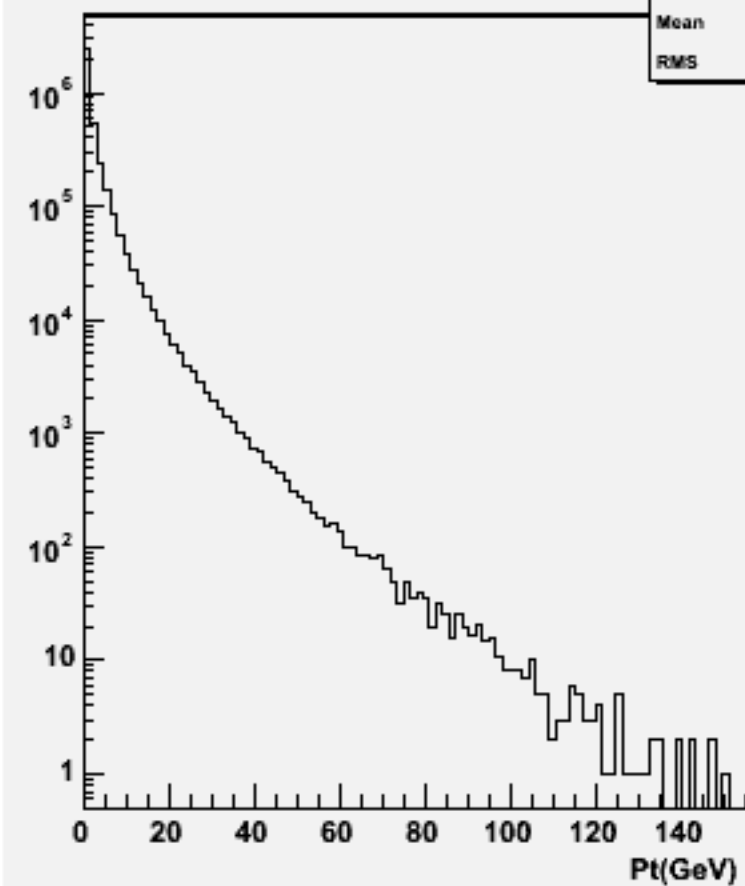
Particle Pt : w100589 uubb_o
