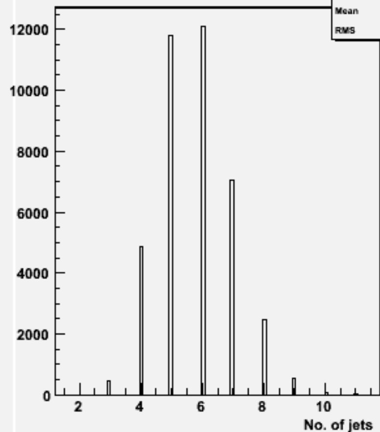
No. jets (ycut=0.001) : w100589 uubb_o
