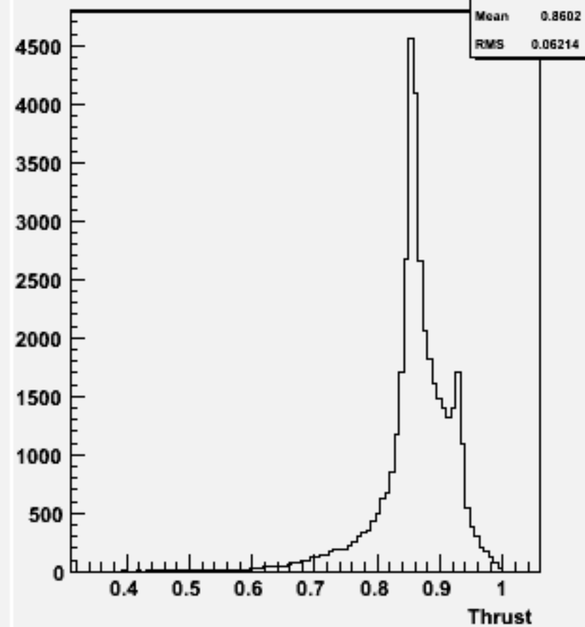
Thrust w100589 uubb_o
