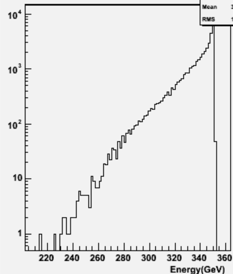
Total Energy (w/o \nu ): w100589 uubb_o
