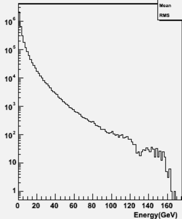
Particle Energy : w100589 uubb_o
