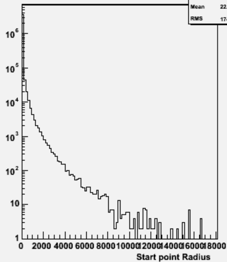
Start point R : w100589 uubb_o
