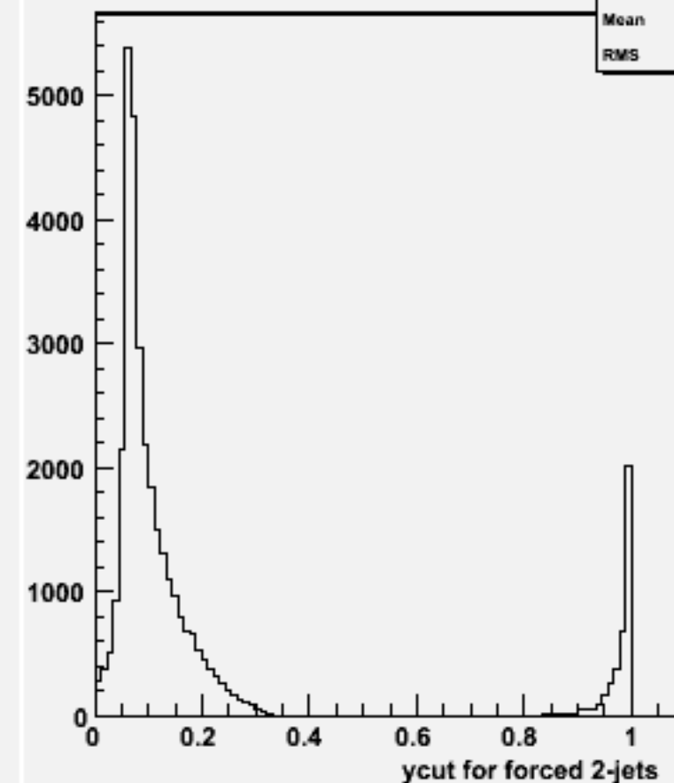
Ycut for 2-jets :w100589 uubb_o
