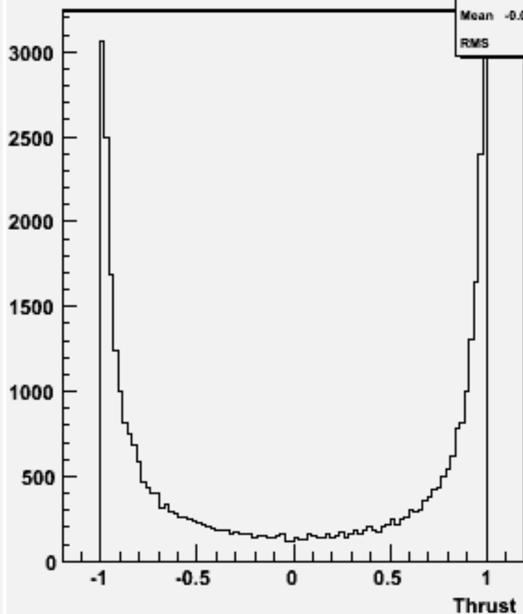
cos \Theta (thrust) w100589 uubb_o
