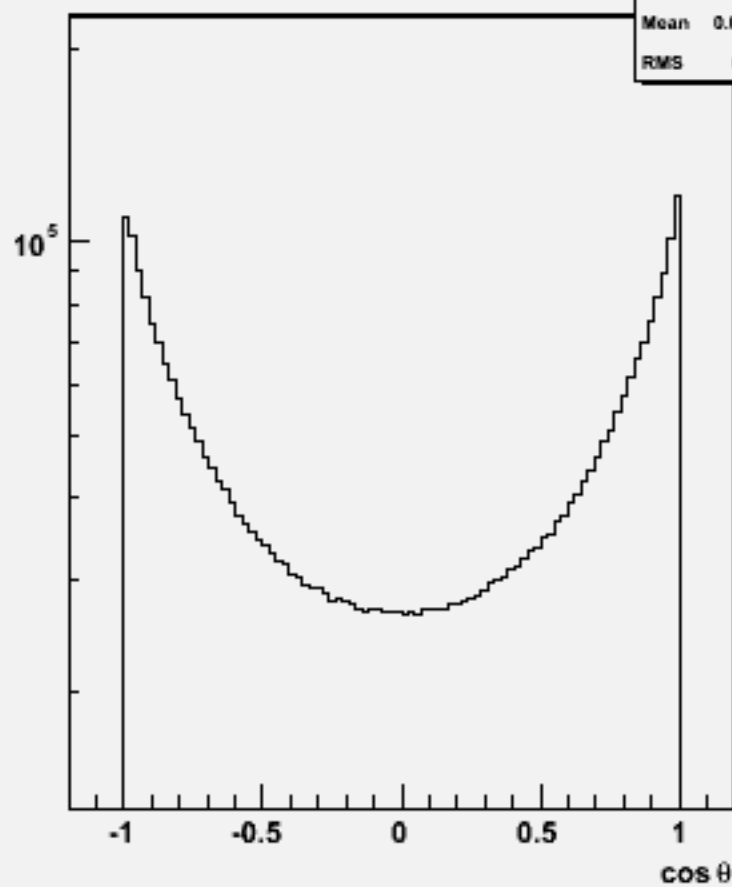
Particle cosθ : w100589 uubb_o
