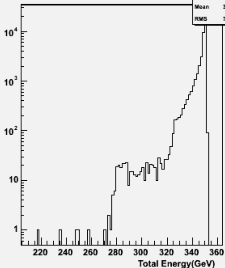
Total Energy (inc. \nu ): w100589 uubb_o
