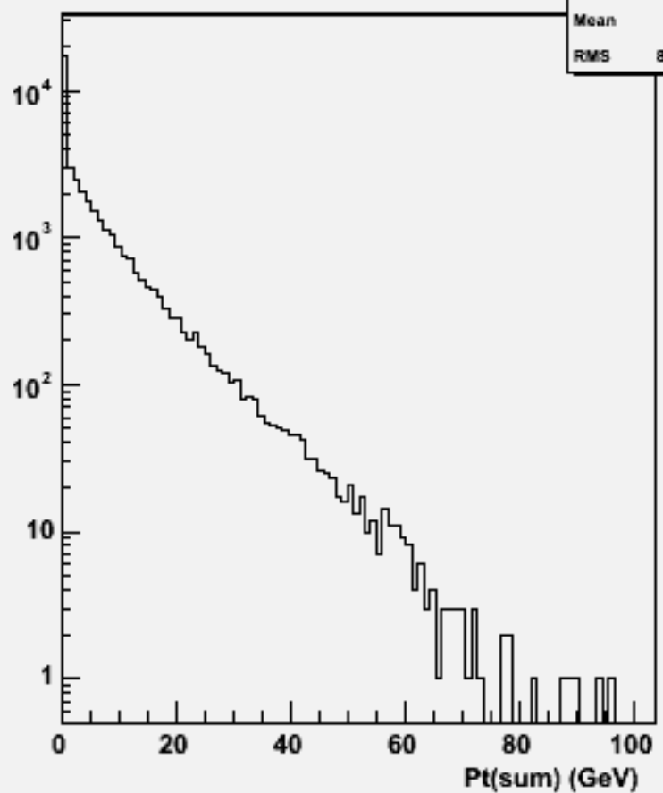
Pt Sum: w100589 uubb_o
