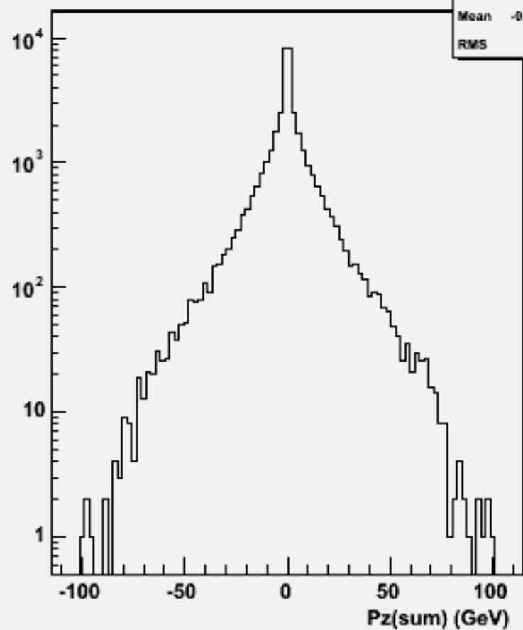
Pz Sum: w100589 uubb_o
