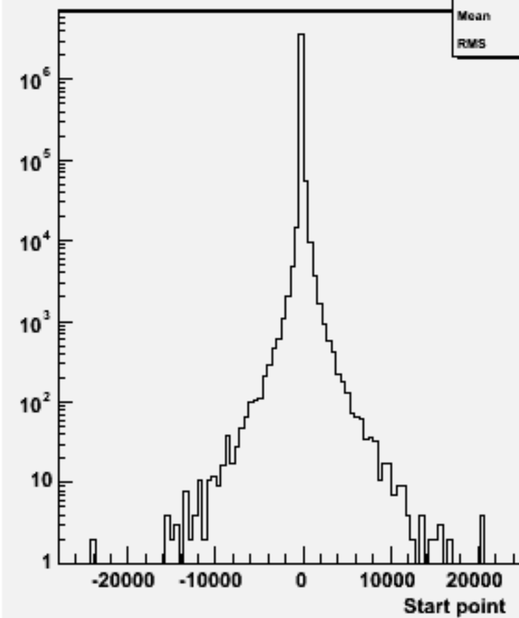
Start point Z : w100589 uubb_o
