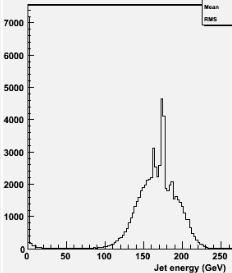
energy for 2-jets :w100589 uubb_o
