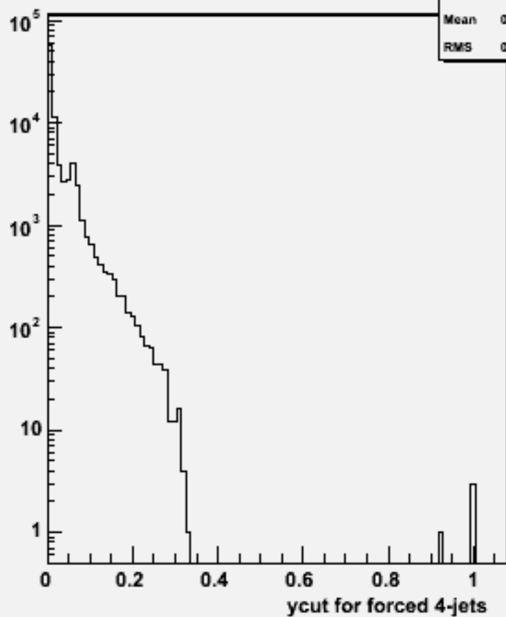
Ycut for 4-jets :w100588 uubb_o
