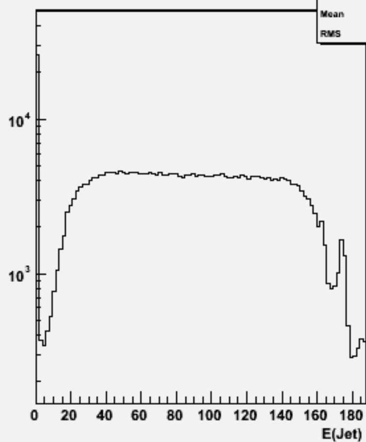
Jet energies(All jets)w100588 uubb_o
