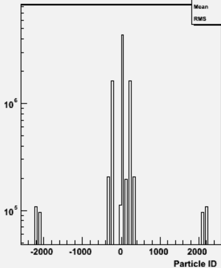
Particle ID : w100588 uubb_o
