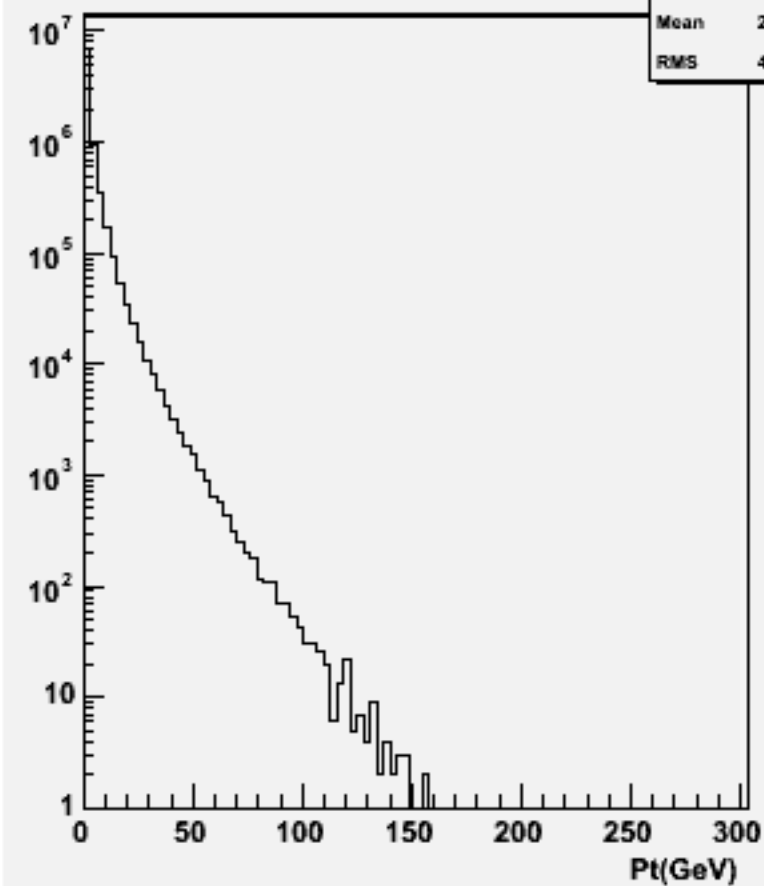
Particle Pt : w100588 uubb_o
