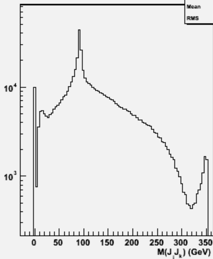
2jets mass(All comb)w100588 uubb_o
