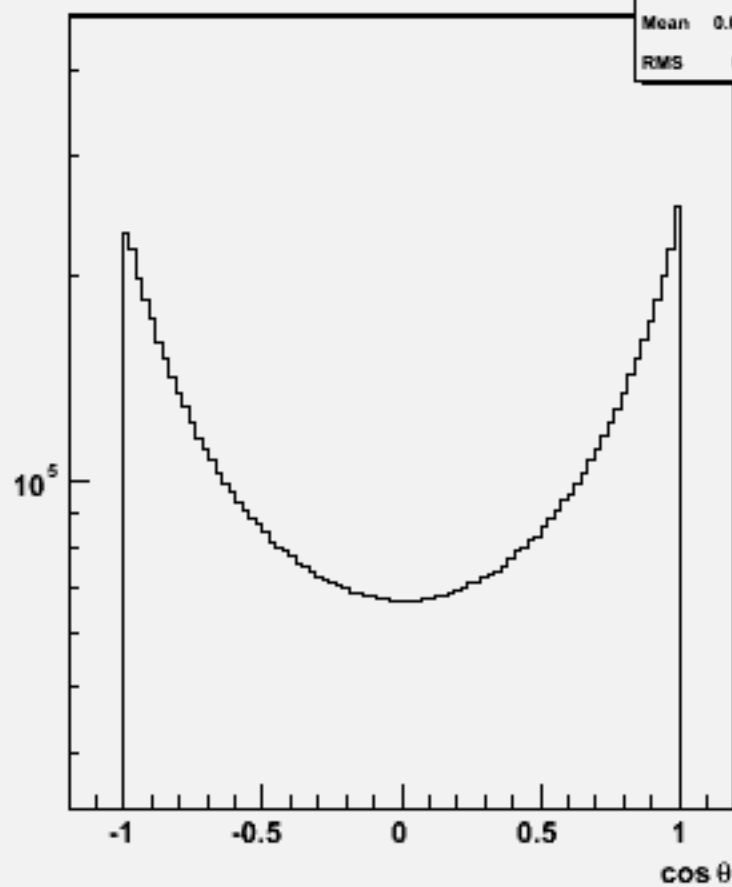
Particle cos \theta : w100588 uubb_o
