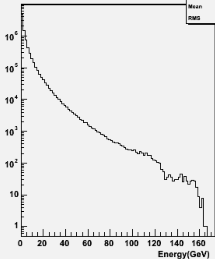
Particle Energy : w100588 uubb_o
