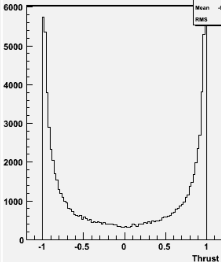
cos \Theta (thrust) w100584 uuss_o
