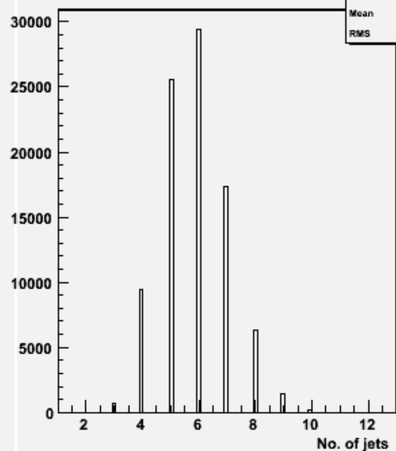
No. jets (ycut=0.001) : w100584 uuss_o
