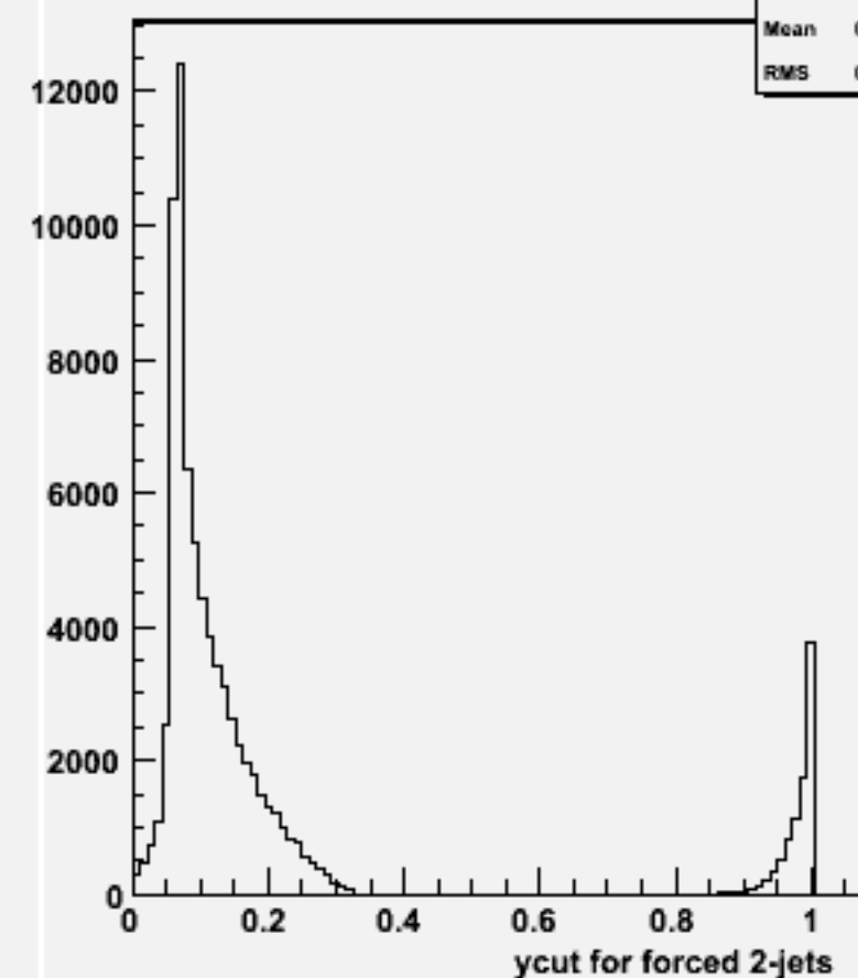
Ycut for 2-jets :w100584 uuss_o
