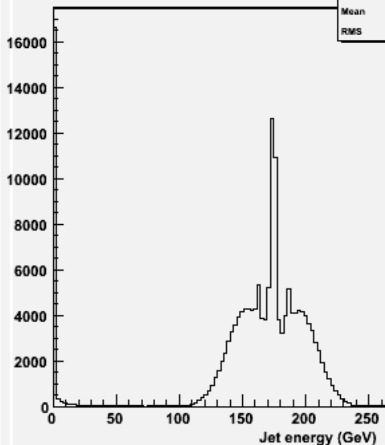
energy for 2-jets :w100584 uuss_o
