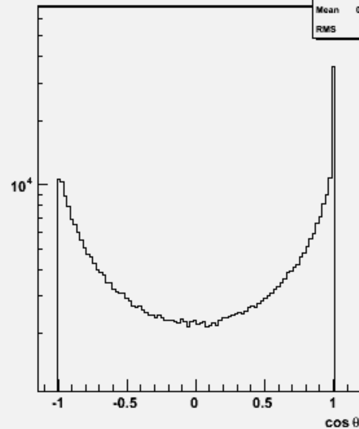
Jet cos \theta (All jets)w100584 uuss_o
