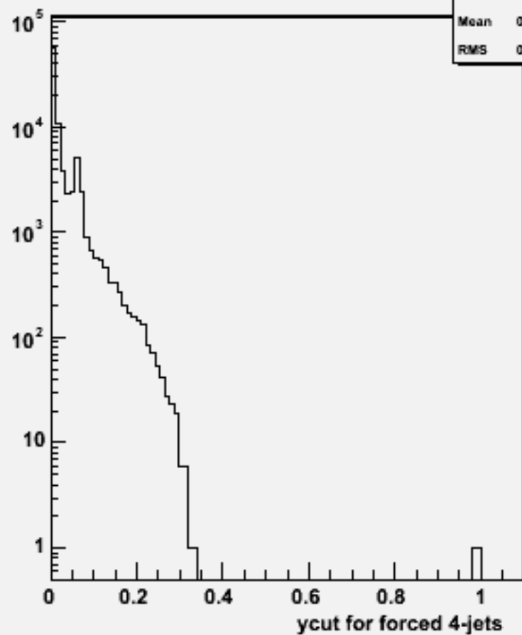
Ycut for 4-jets :w100584 uuss_o
