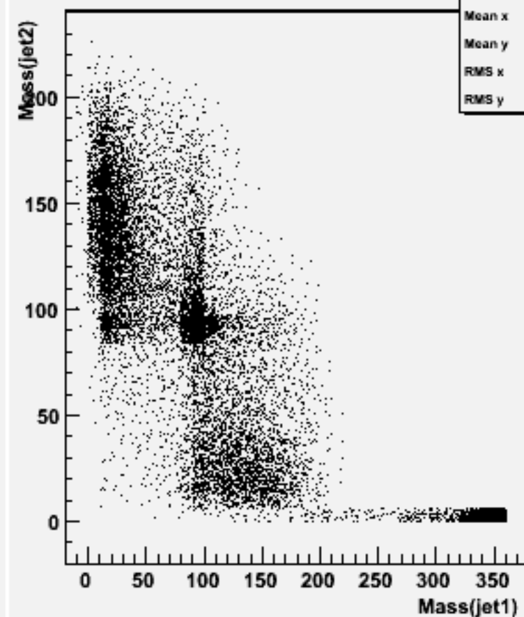
Jet mass for forced 2-jets : w100584 uuss_o
