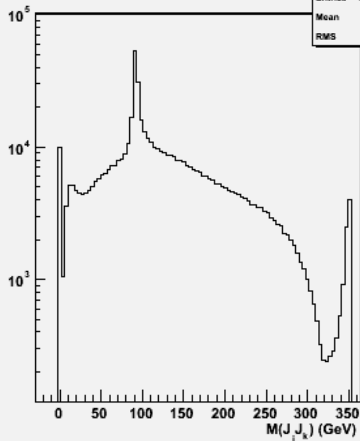
2jets mass(All comb)w100584 uuss_o
