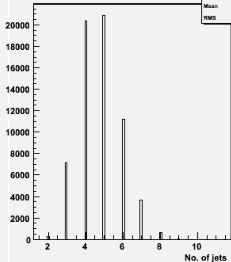
No. jets (ycut=0.001) : w100576 uue2e2_o
