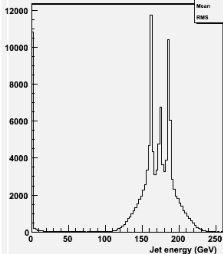
energy for 2-jets :w100576 uue2e2_o
