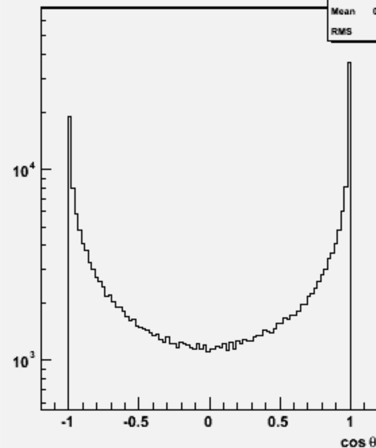
Jet cos \theta (All jets)w100576 uue2e2_o
