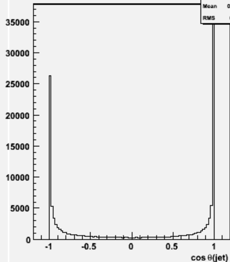
cos \theta for 2-jets :w100576 uue2e2_o
