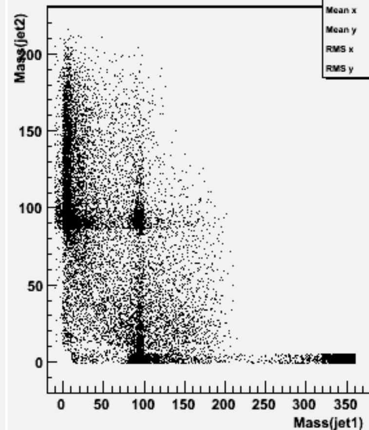
Jet mass for forced 2-jets : w100576 uue2e2_o
