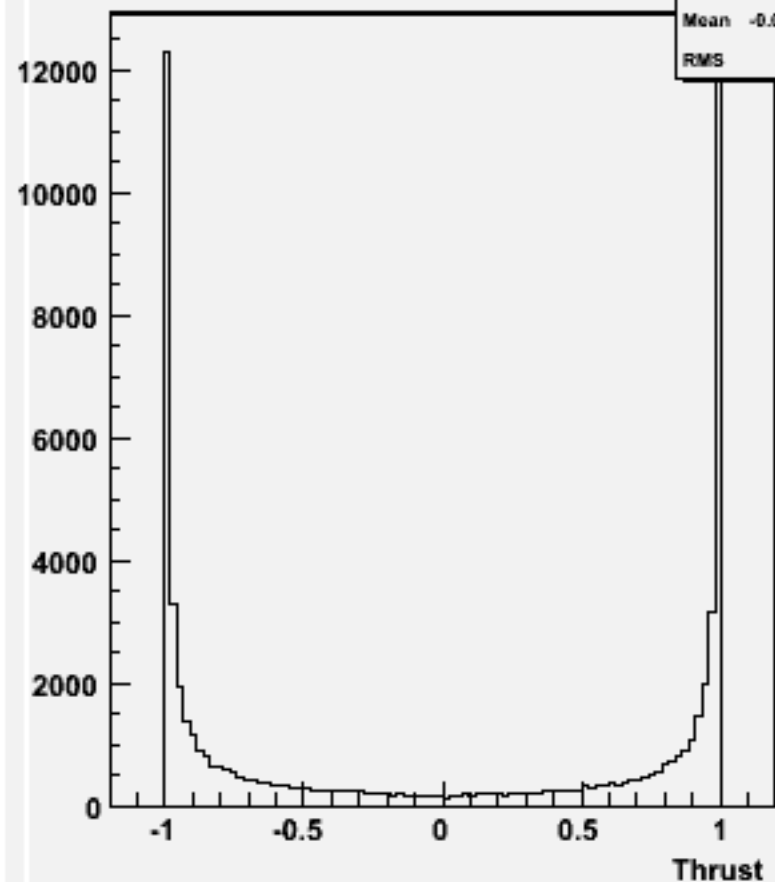
cos \Theta (thrust) w100576 uue2e2_o
