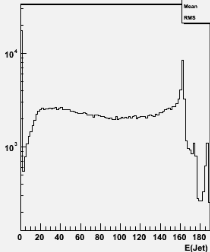
Jet energies(All jets)w100576 uue2e2_o
