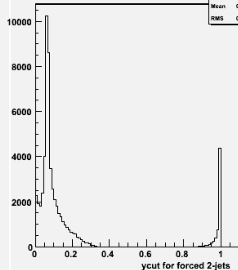
Ycut for 2-jets :w100576 uue2e2_o
