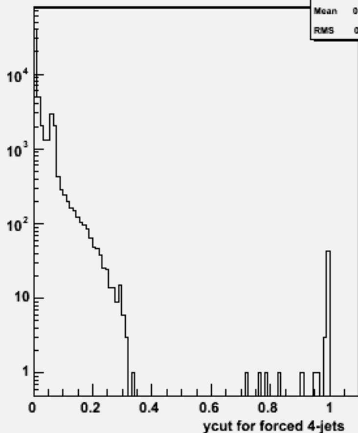
Ycut for 4-jets :w100576 uue2e2_o
