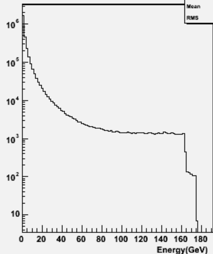
Particle Energy : w100576 uue2e2_o
