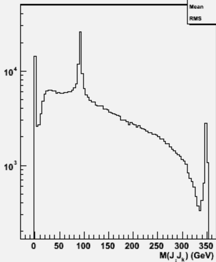
2jets mass(All comb)w100576 uue2e2_o
