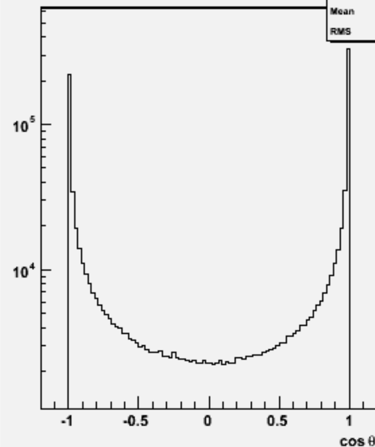
Jet cos \theta (All jets)w100574 uue1e1_o
