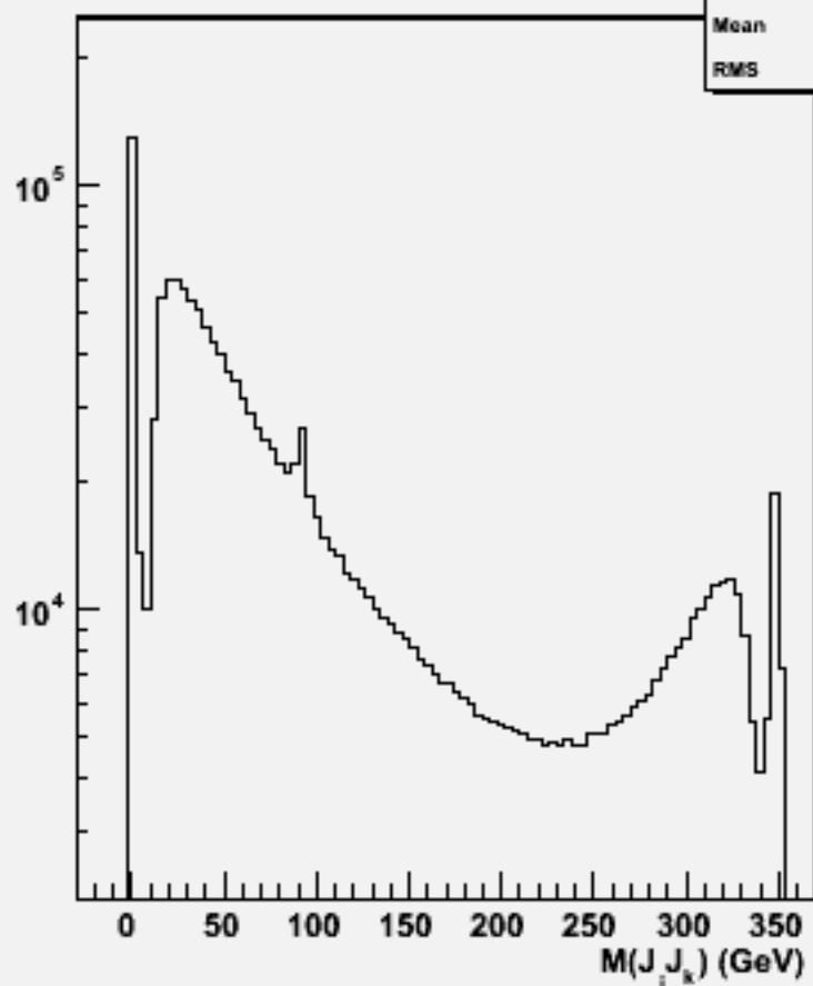
2jets mass(All comb)w100574 uue1e1_o
