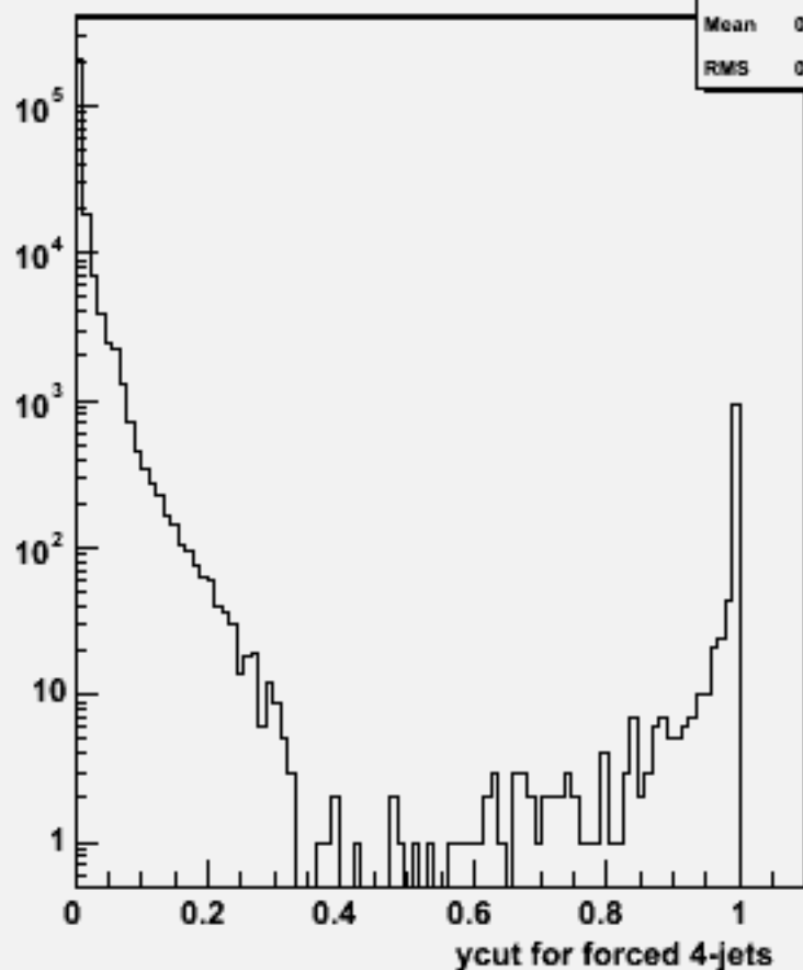
Ycut for 4-jets :w100574 uue1e1_o
