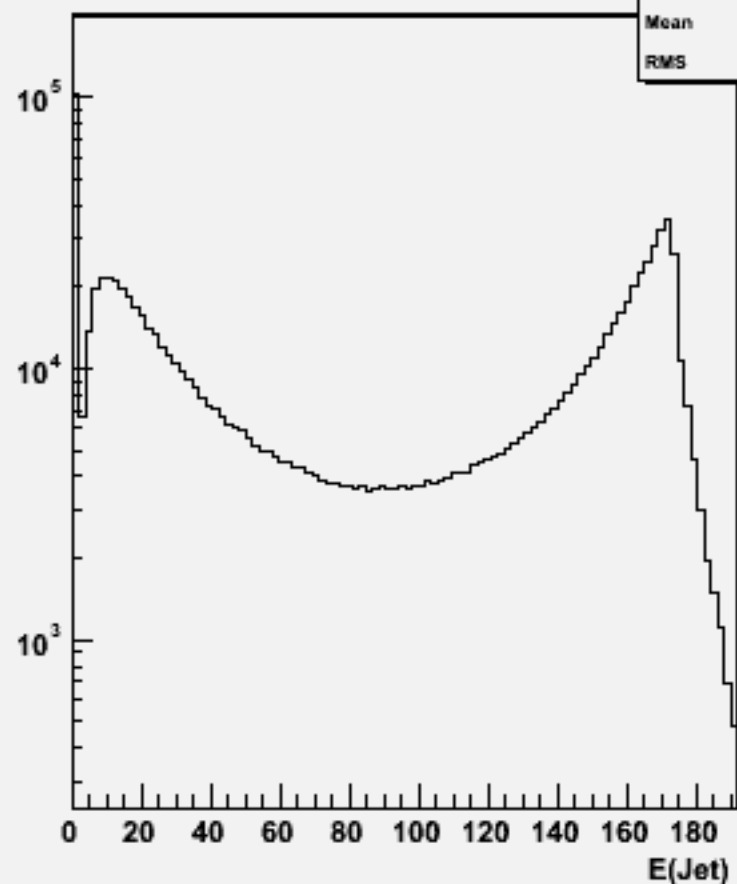
Jet energies(All jets)w100574 uue1e1_o
