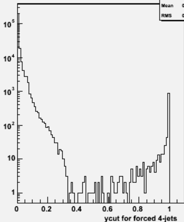
Ycut for 4-jets :w100572 uue1e1_o
