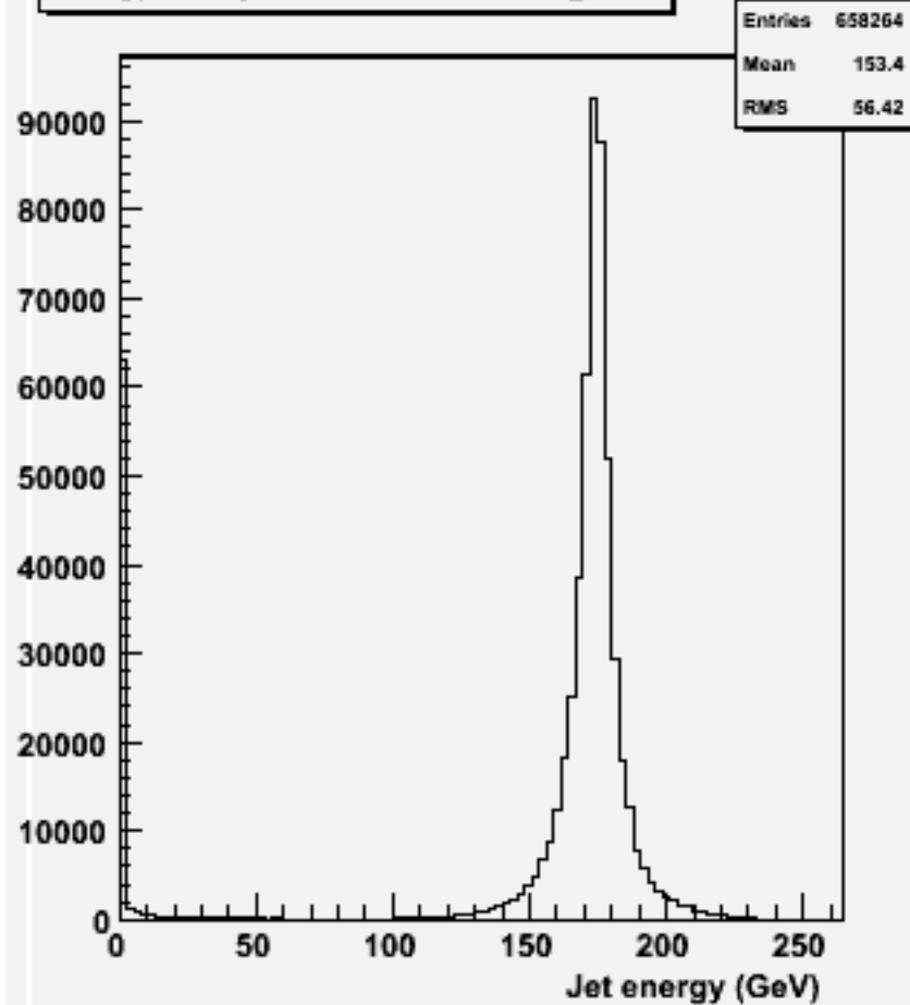
energy for 2-jets :w100572 uue1e1_o
