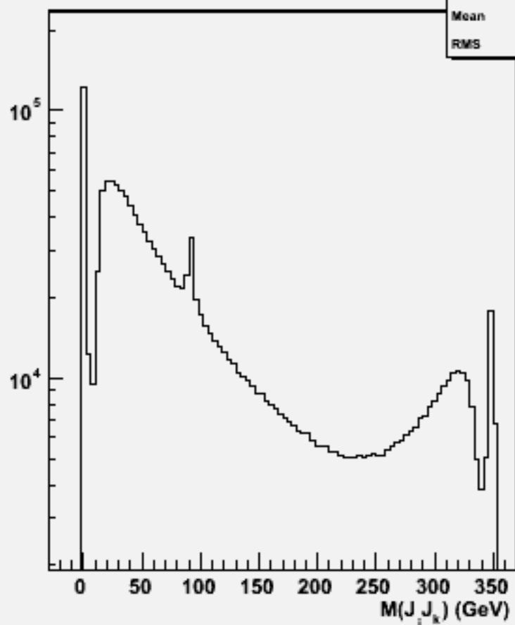
2jets mass(All comb)w100572 uue1e1_o
