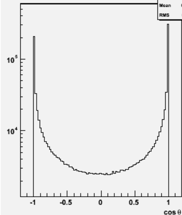
Jet cos \theta (All jets)w100572 uue1e1_o
