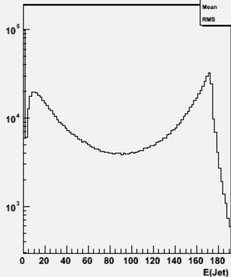
Jet energies(All jets)w100572 uue1e1_o
