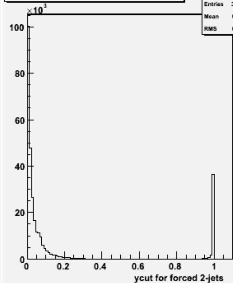
Ycut for 2-jets :w100572 uue1e1_o
