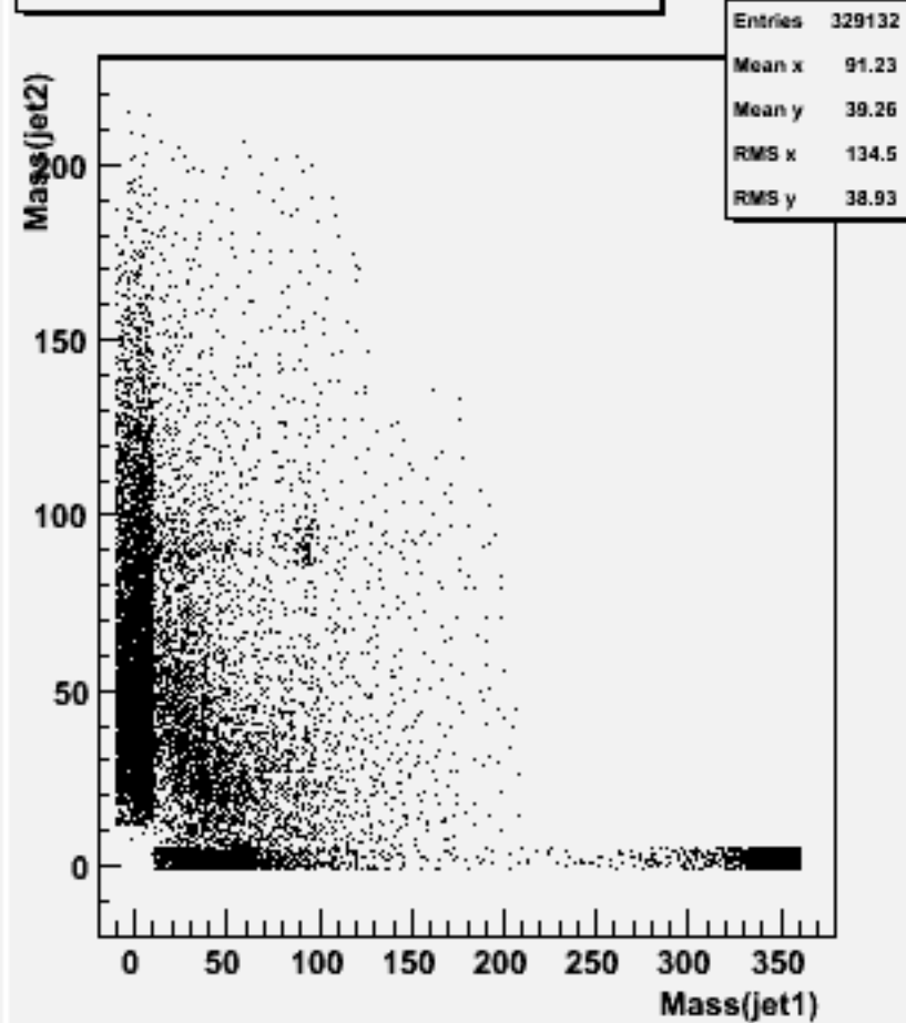
Jet mass for forced 2-jets : w100572 uue1e1_o
