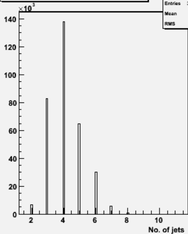
No. jets (ycut=0.001) : w100572 uue1e1_o
