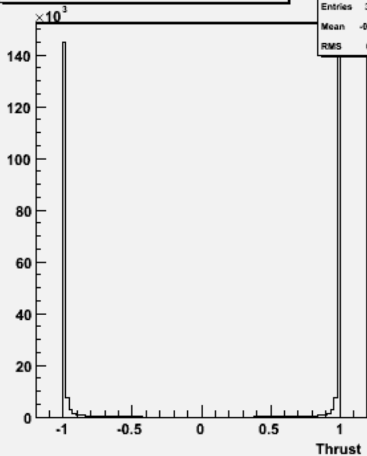
cos \Theta (thrust) w100572 uue1e1_o
