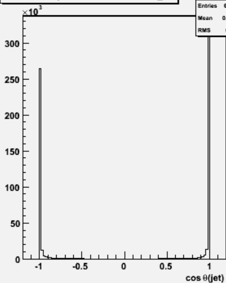
cos \theta for 2-jets :w100572 uue1e1_o
