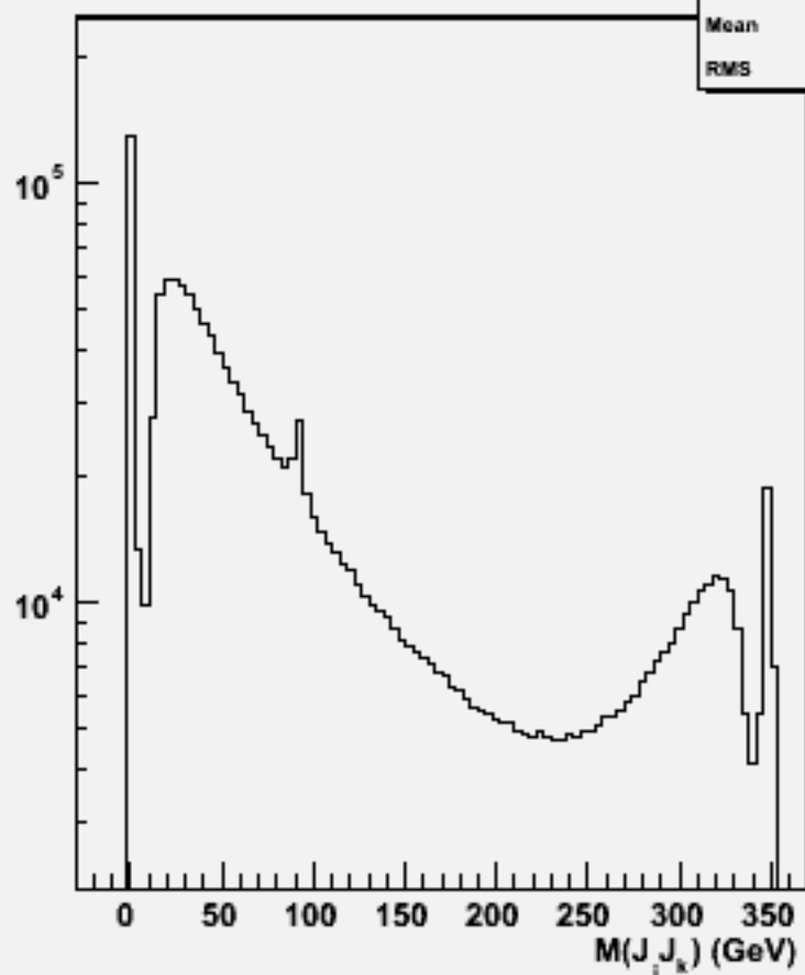
2jets mass(All comb)w100571 uue1e1_o
