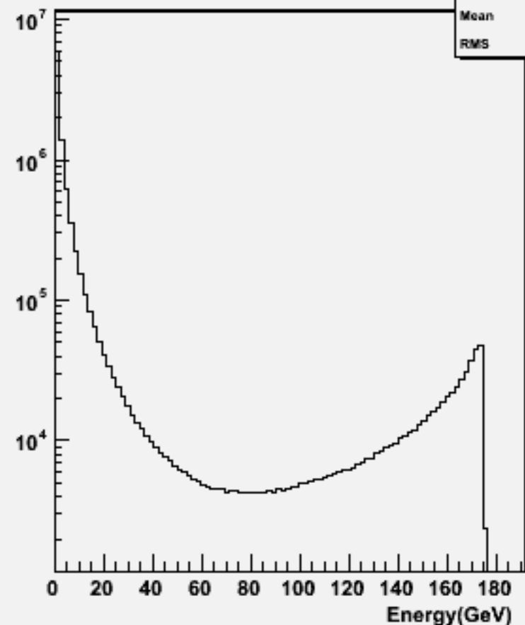
Particle Energy : w100571 uue1e1_o
