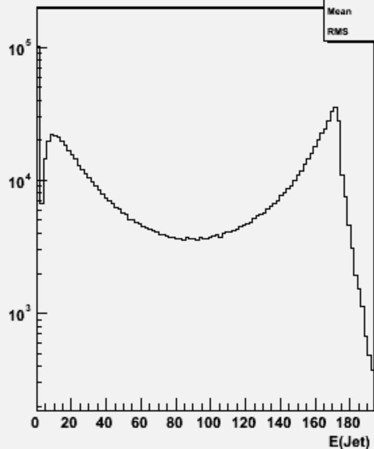
Jet energies(All jets)w100571 uue1e1_o
