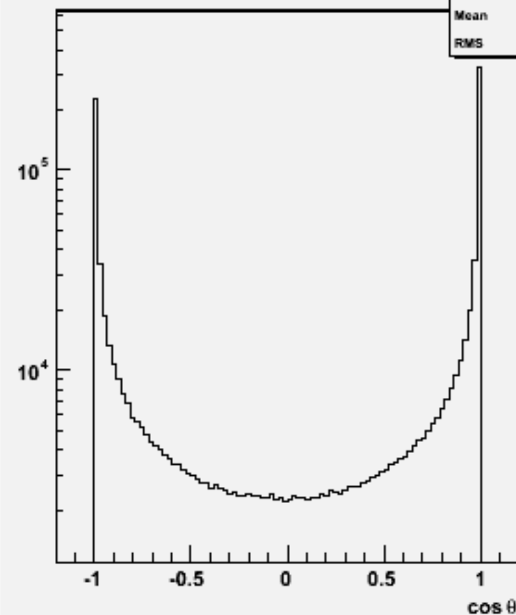
Jet cos \theta (All jets)w100571 uue1e1_o
