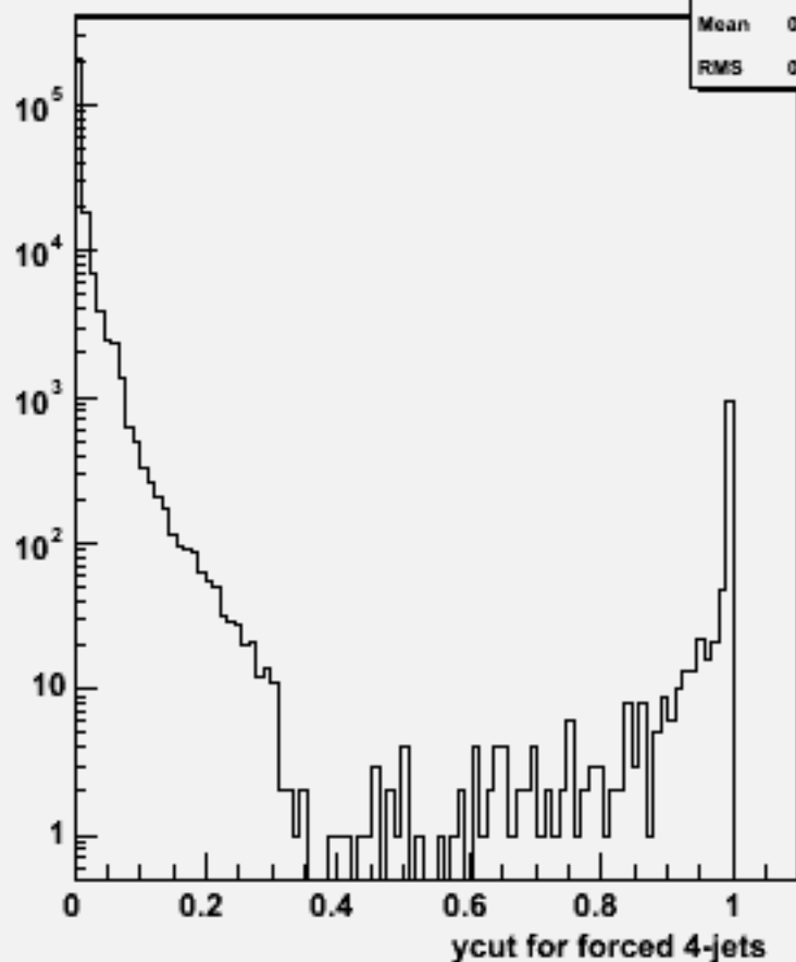
Ycut for 4-jets :w100571 uue1e1_o
