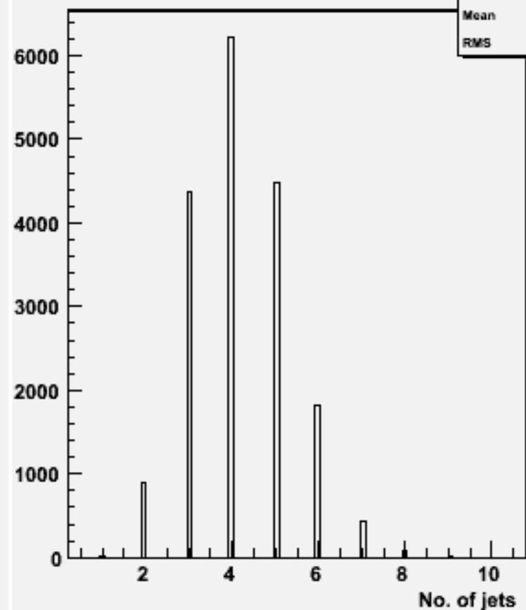
No. jets (ycut=0.001) : w100565 n3n3ss_o
