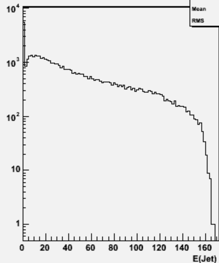
Jet energies(All jets)w100565 n3n3ss_o
