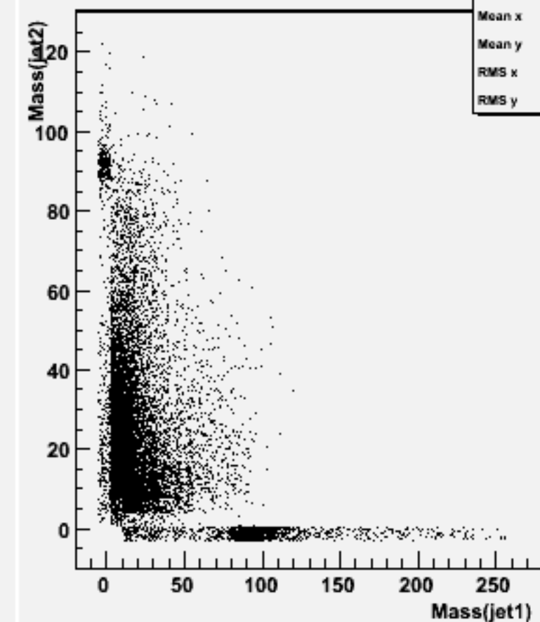
Jet mass for forced 2-jets : w100565 n3n3ss_o
