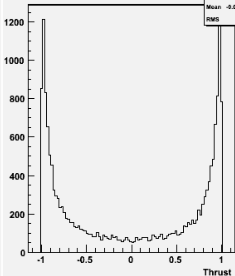
cos \Theta (thrust) w100565 n3n3ss_o
