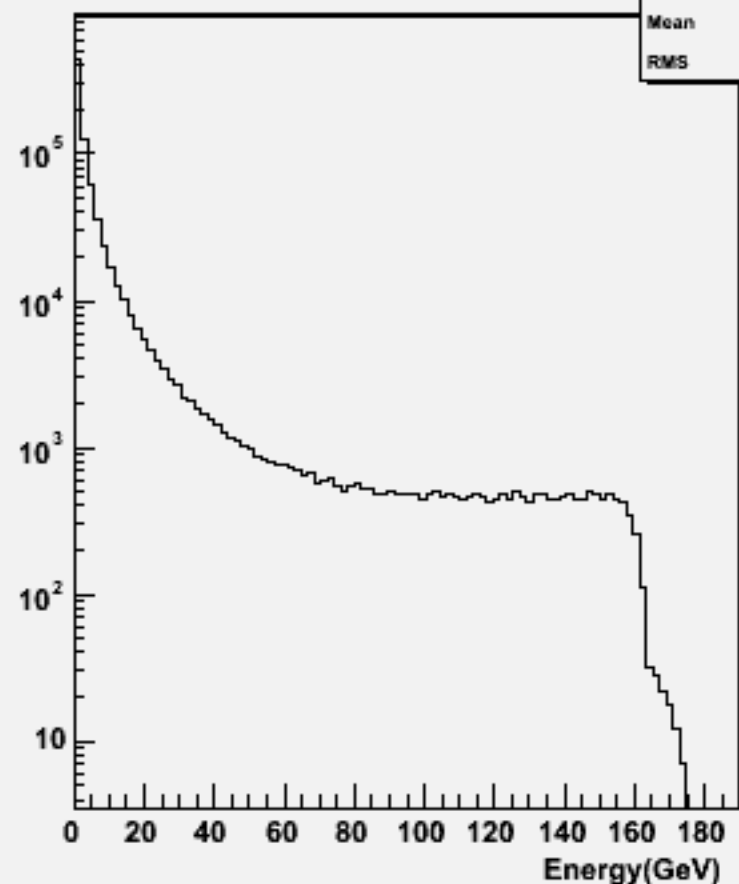
Particle Energy : w100565 n3n3ss_o
