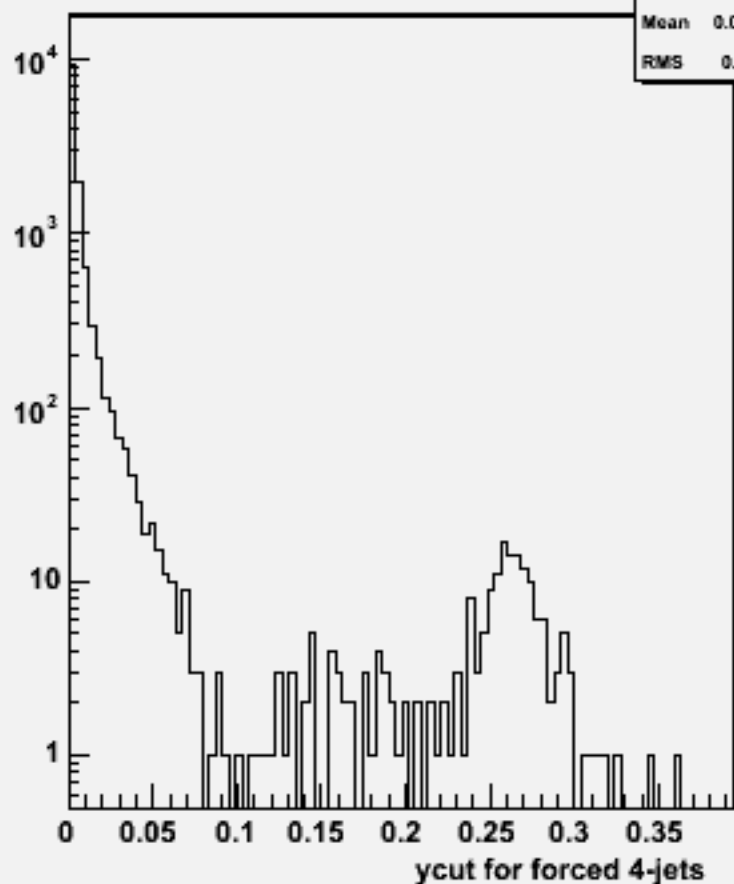
Ycut for 4-jets :w100565 n3n3ss_o
