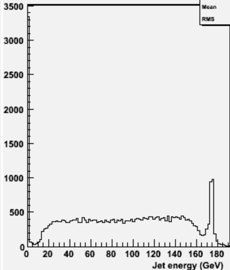
energy for 2-jets :w100565 n3n3ss_o
