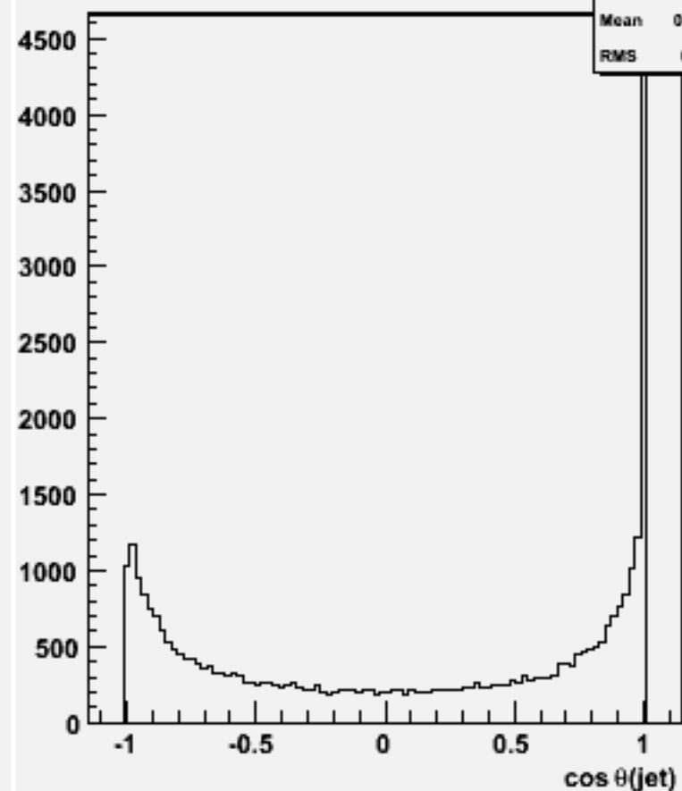
cos \theta for 2-jets :w100565 n3n3ss_o
