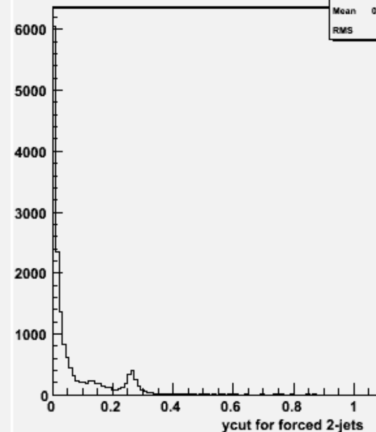
Ycut for 2-jets :w100565 n3n3ss_o
