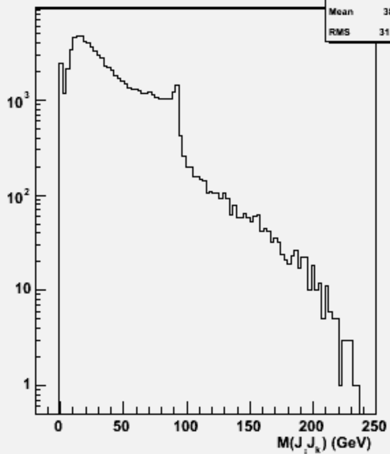
2jets mass(All comb)w100565 n3n3ss_o
