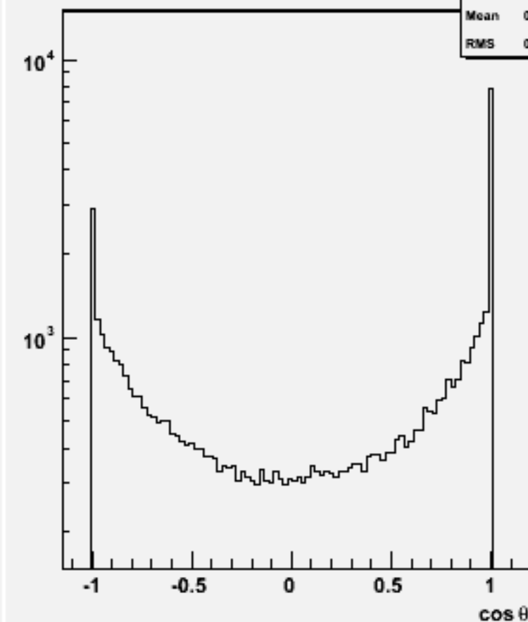
Jet cos \theta (All jets)w100565 n3n3ss_o
