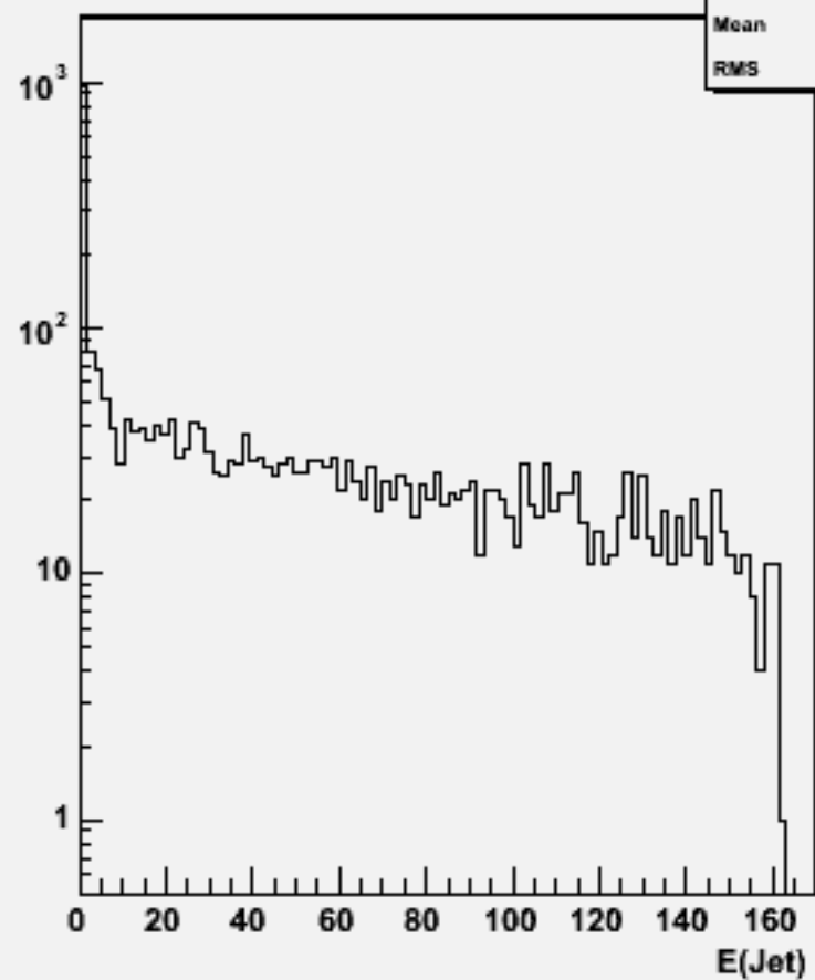
Jet energies(All jets)w100557 n3n3e2e2_o
