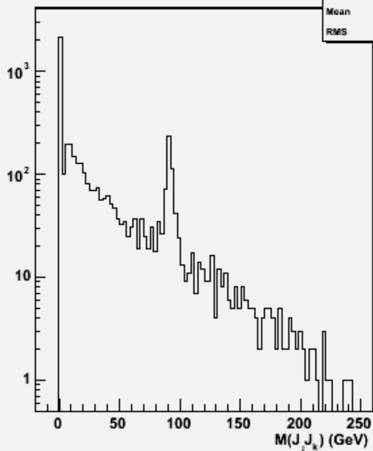
2jets mass(All comb)w100557 n3n3e2e2_o
