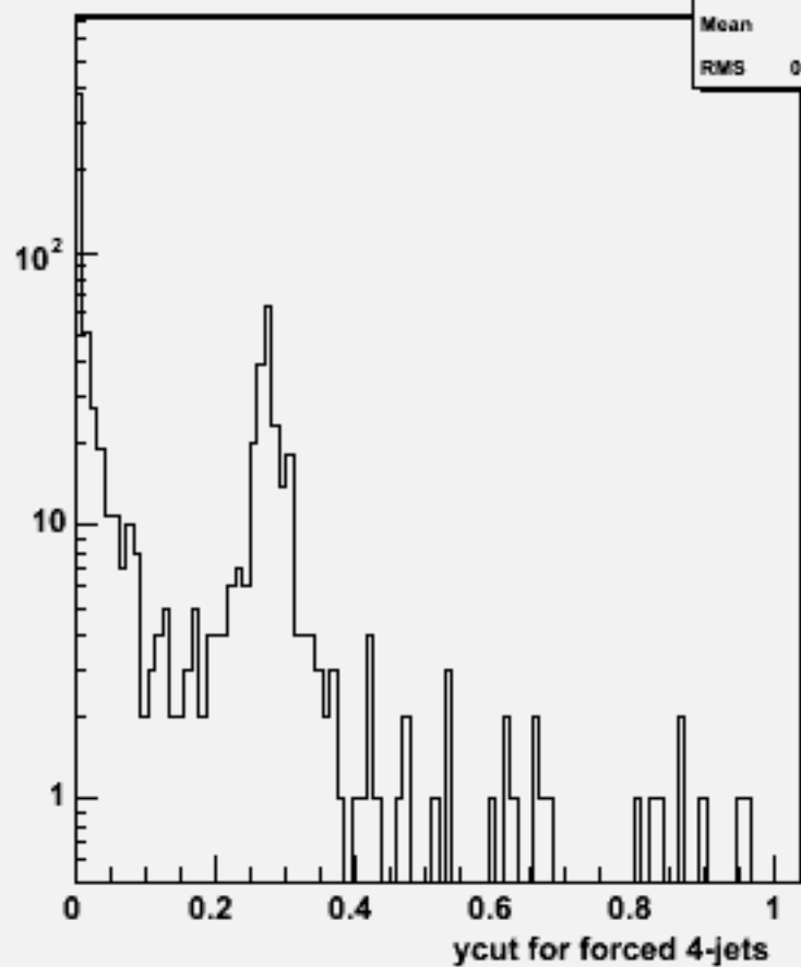
Ycut for 4-jets :w100557 n3n3e2e2_o
