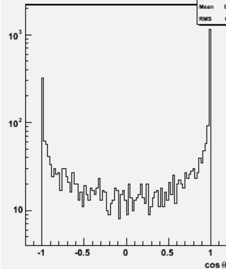
Jet cosθ (All jets)w100557 n3n3e2e2_o
