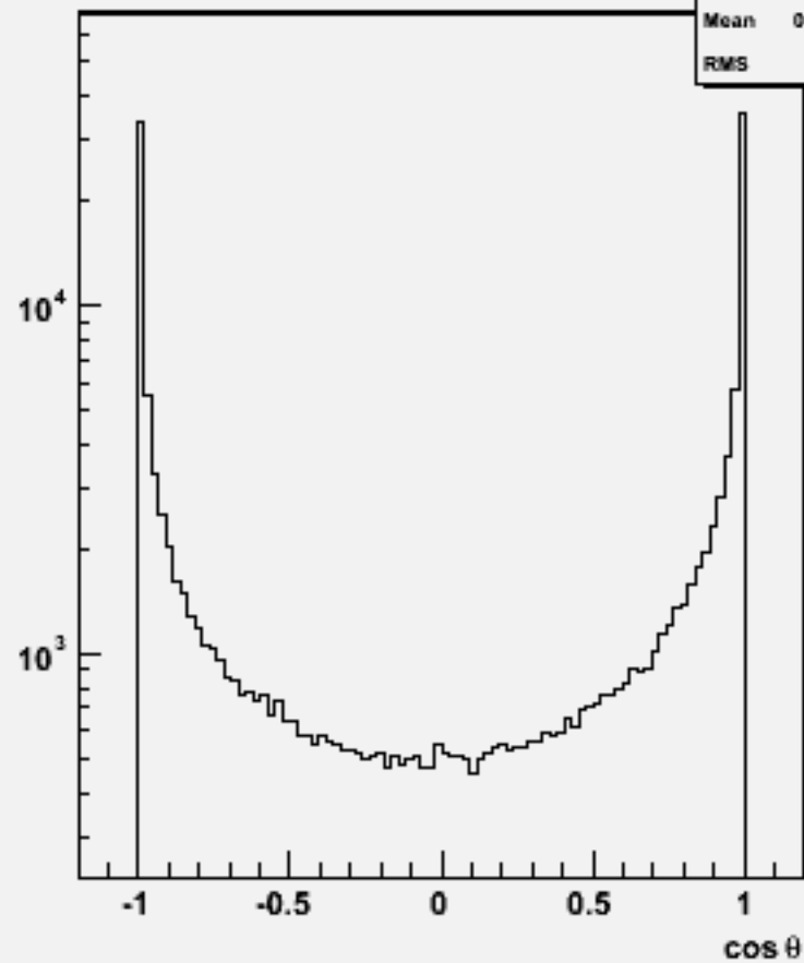
Particle cos \theta : w100551 n3n3e1e1_o
