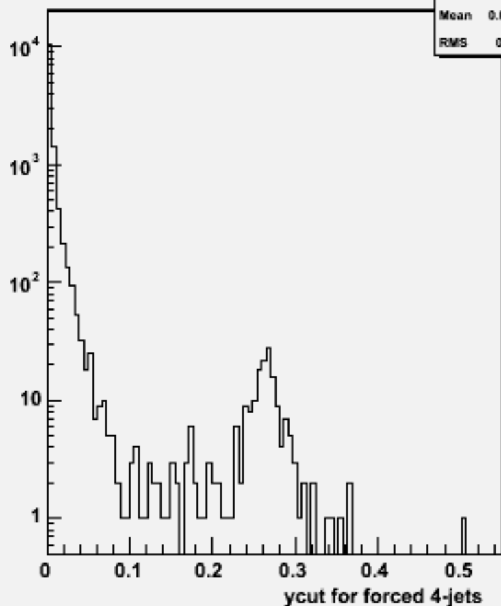
Ycut for 4-jets :w100545 n2n2ss_o
