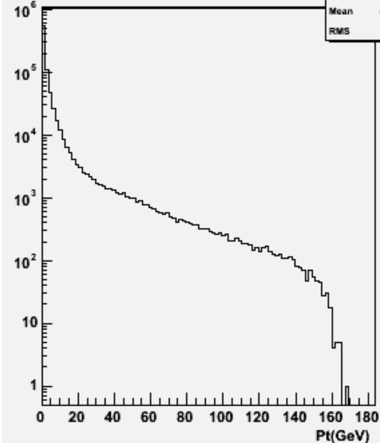
Particle Pt : w100545 n2n2ss_o
