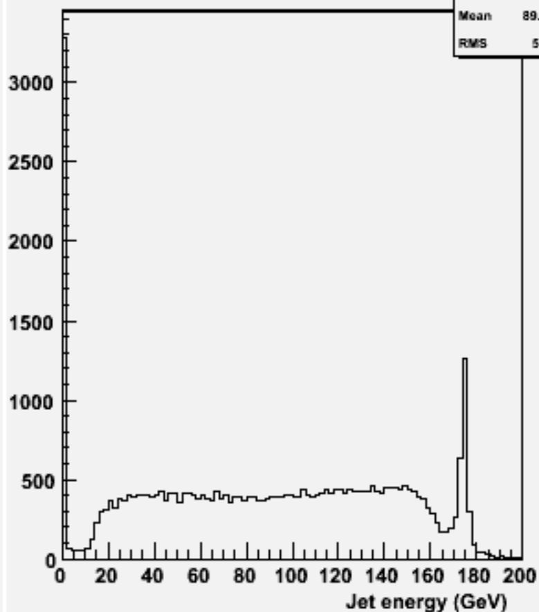
energy for 2-jets :w100545 n2n2ss_o
