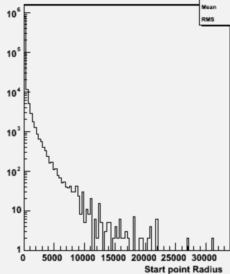
Start point R : w100545 n2n2ss_o
