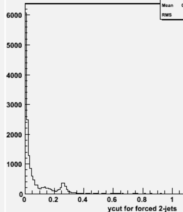
Ycut for 2-jets :w100545 n2n2ss_o
