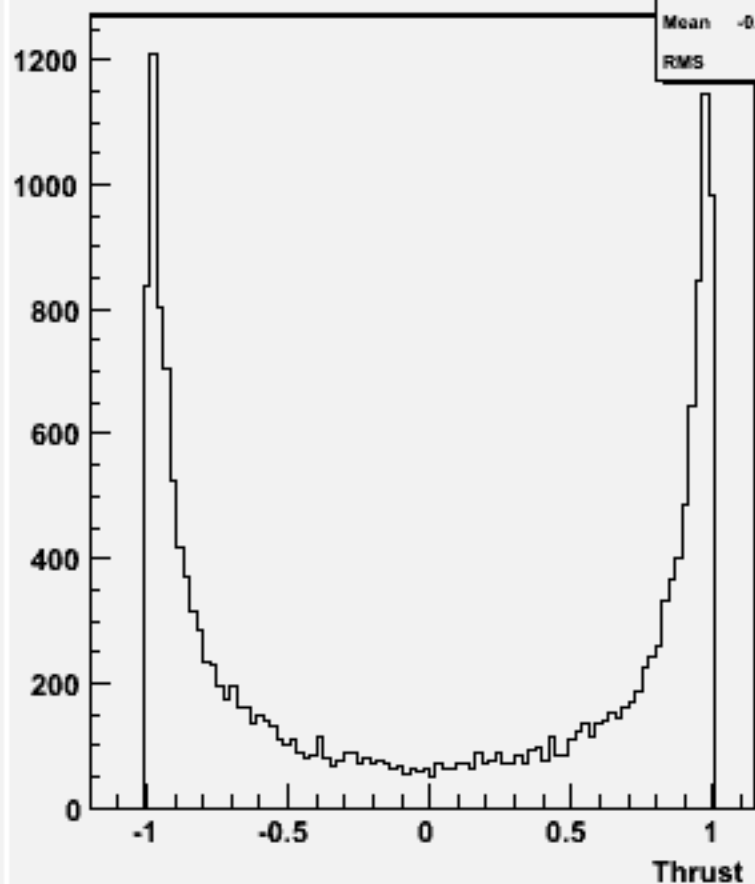
cos \Theta (thrust) w100545 n2n2ss_o
