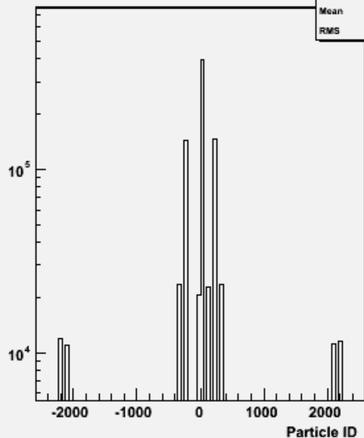
Particle ID : w100545 n2n2ss_o
