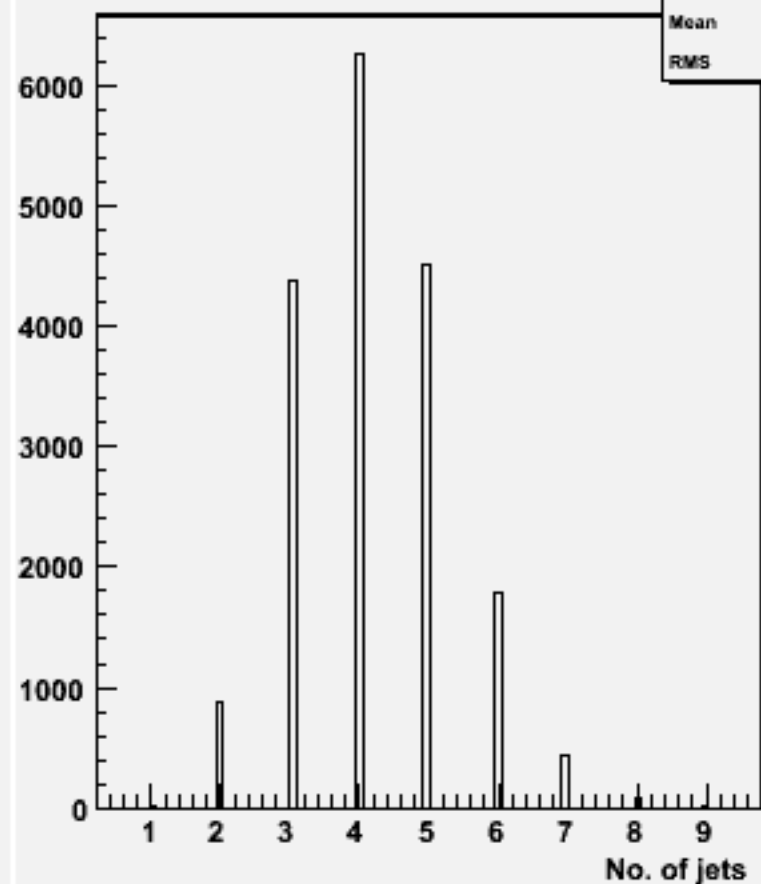
No. jets (ycut=0.001) : w100545 n2n2ss_o
