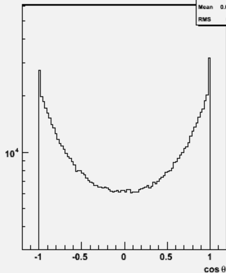
Particle cosθ : w100545 n2n2ss_o
