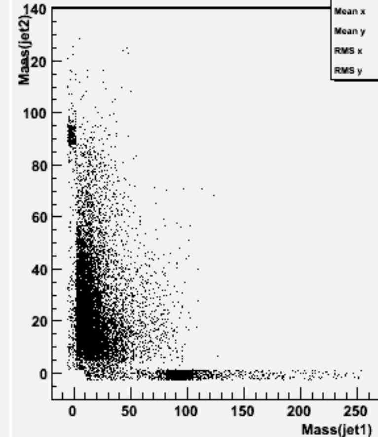
Jet mass for forced 2-jets : w100545 n2n2ss_o
