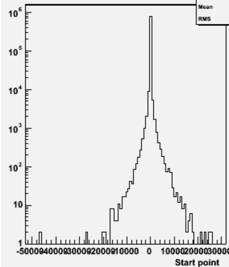
Start point Z : w100545 n2n2ss_o
