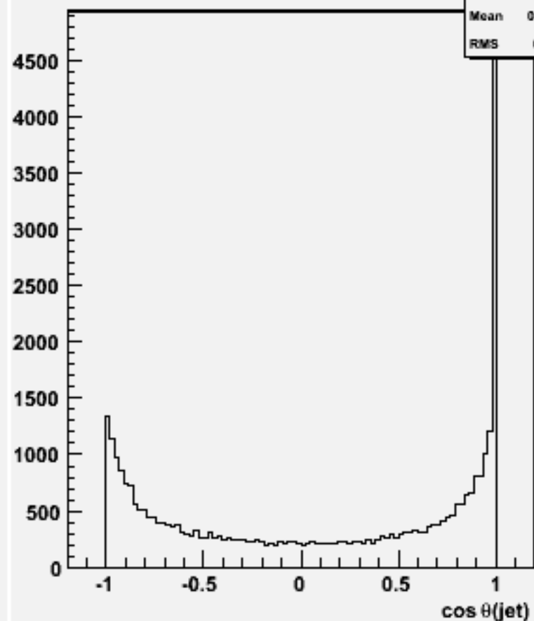
cos \theta for 2-jets :w100545 n2n2ss_o
