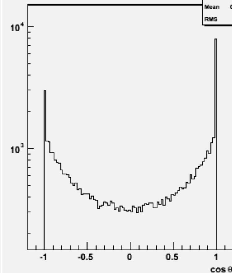
Jet cos \theta (All jets)w100545 n2n2ss_o
