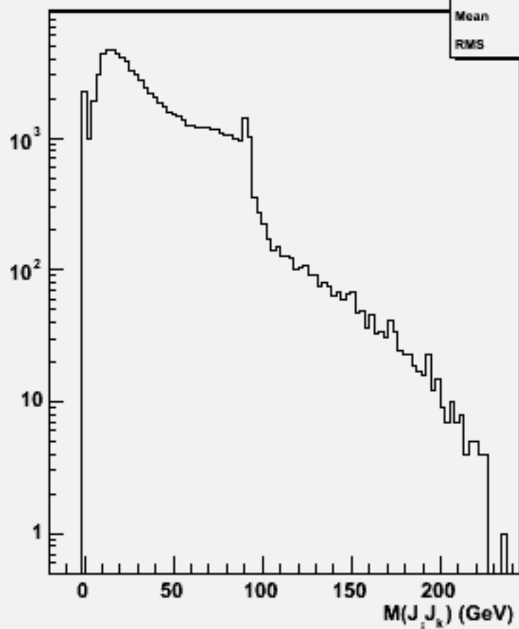
2jets mass(All comb)w100545 n2n2ss_o
