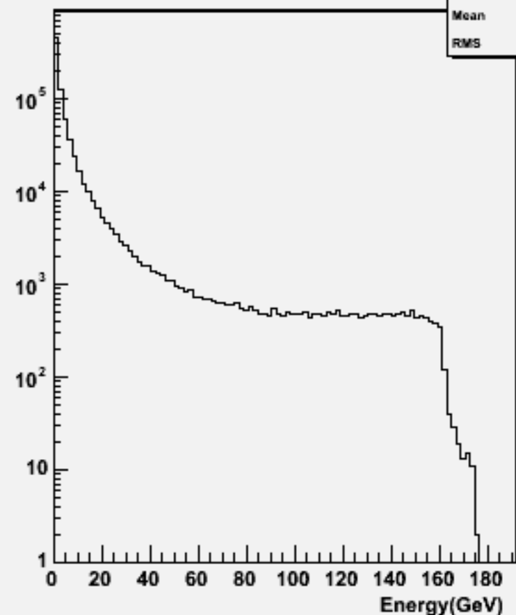
Particle Energy : w100545 n2n2ss_o
