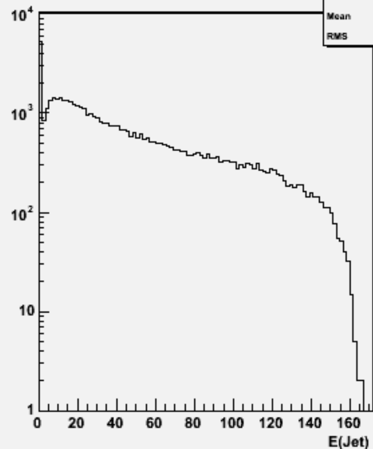
Jet energies(All jets)w100545 n2n2ss_o
