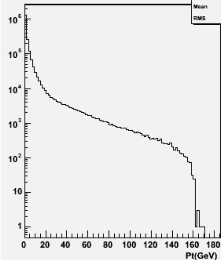
Particle Pt : w100544 n2n2ss_o
