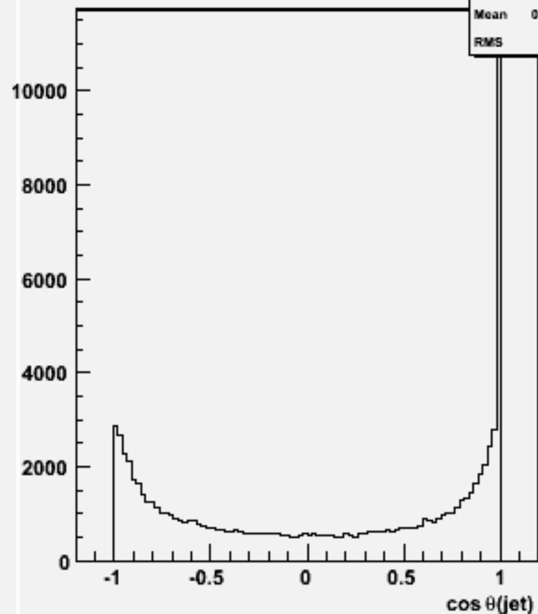
cos \theta for 2-jets :w100544 n2n2ss_o
