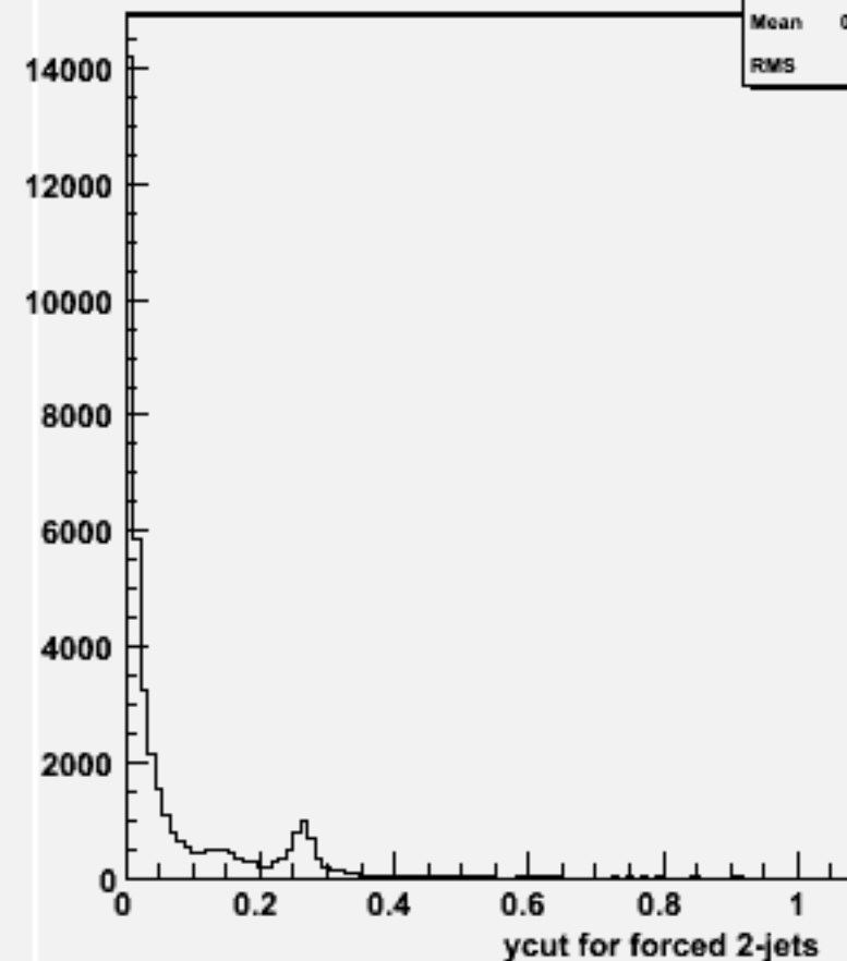
Ycut for 2-jets :w100544 n2n2ss_o
