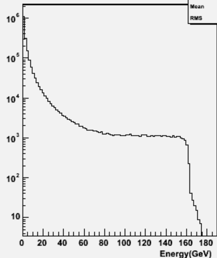
Particle Energy : w100544 n2n2ss_o
