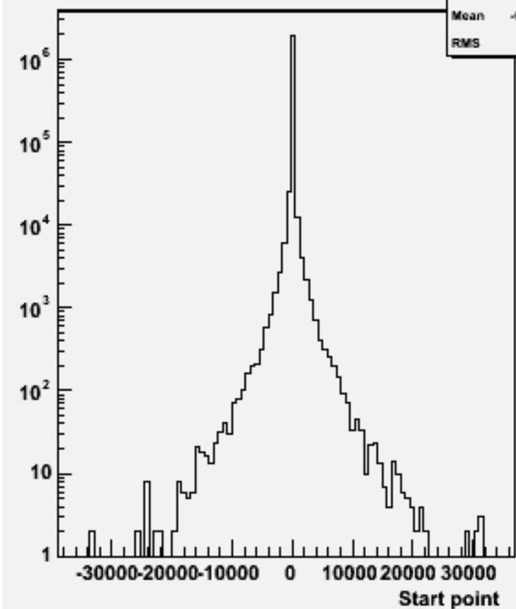
Start point Z : w100544 n2n2ss_o
