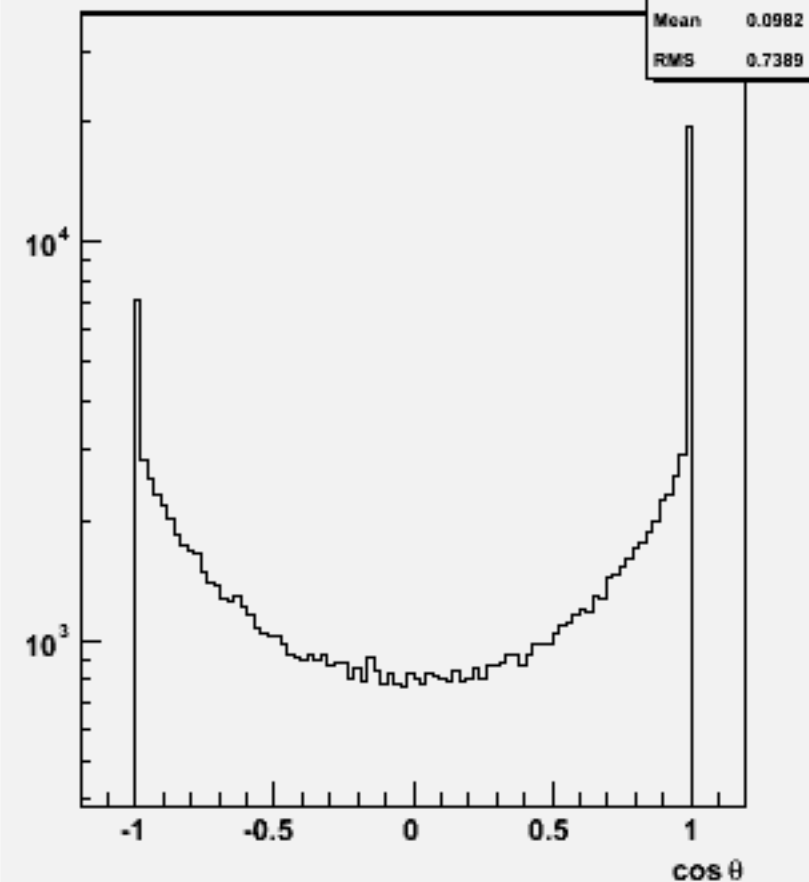
Jet cos \theta (All jets)w100544 n2n2ss_o
