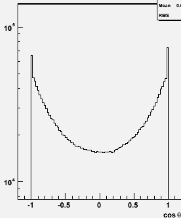
Particle cosθ : w100544 n2n2ss_o
