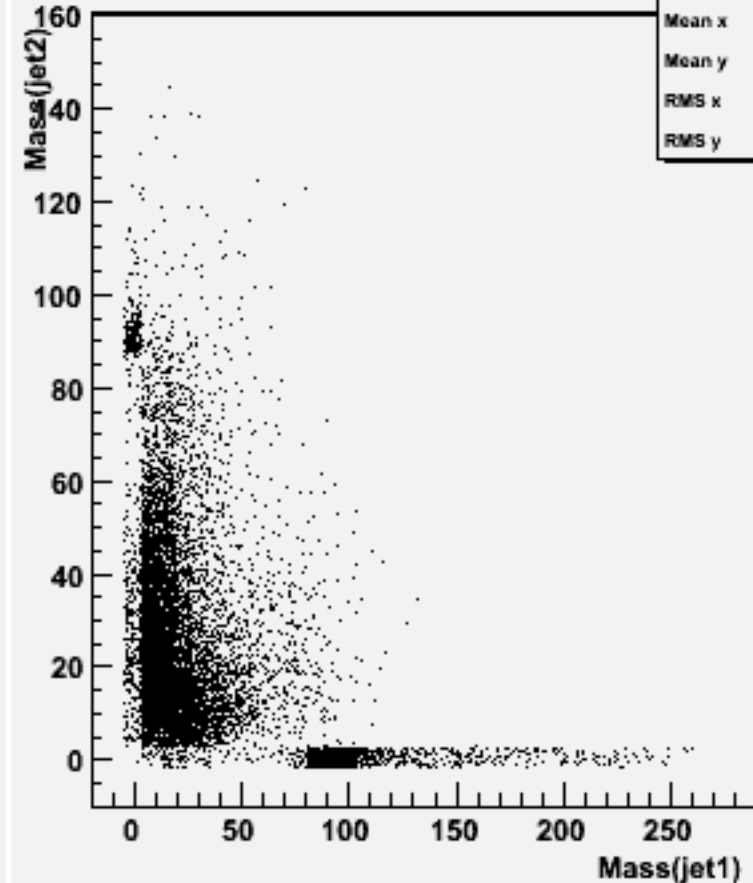
Jet mass for forced 2-jets : w100544 n2n2ss_o
