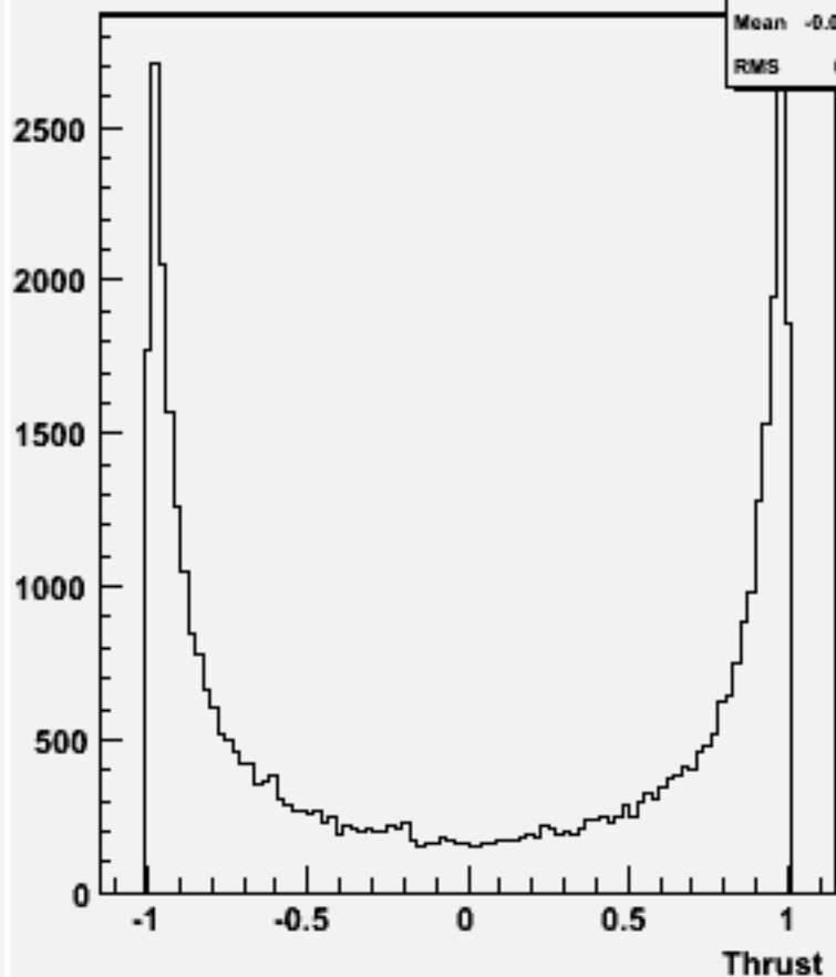
cos \Theta (thrust) w100544 n2n2ss_o
