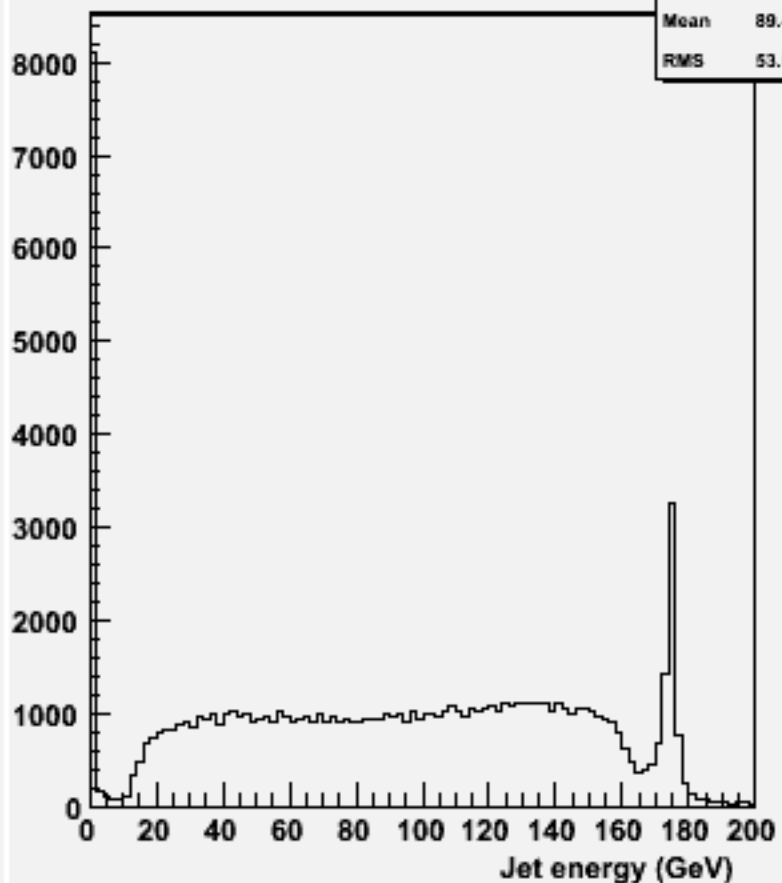
energy for 2-jets :w100544 n2n2ss_o
