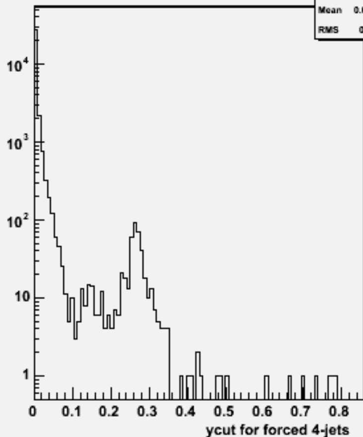
Ycut for 4-jets :w100544 n2n2ss_o
