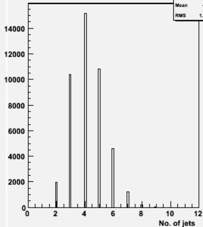
No. jets (ycut=0.001) : w100544 n2n2ss_o
