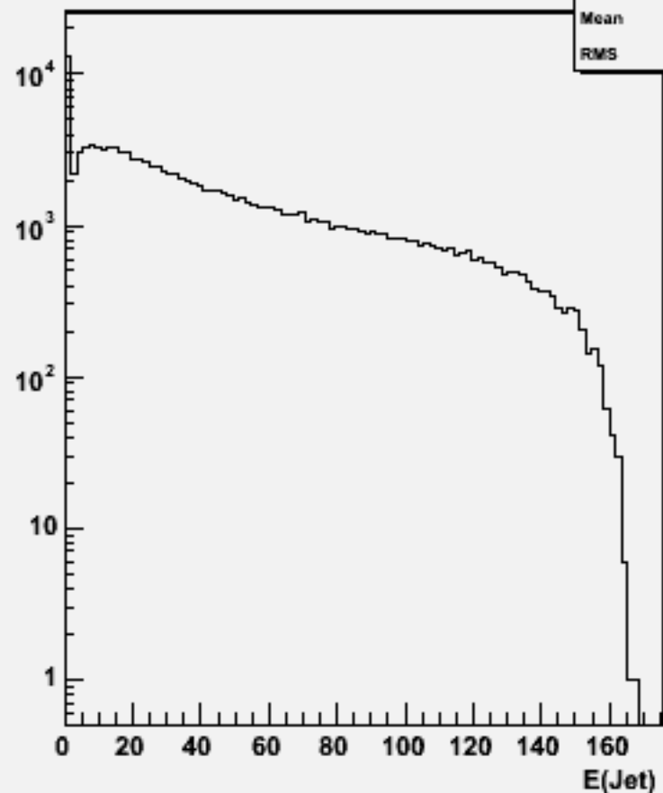
Jet energies(All jets)w100544 n2n2ss_o
