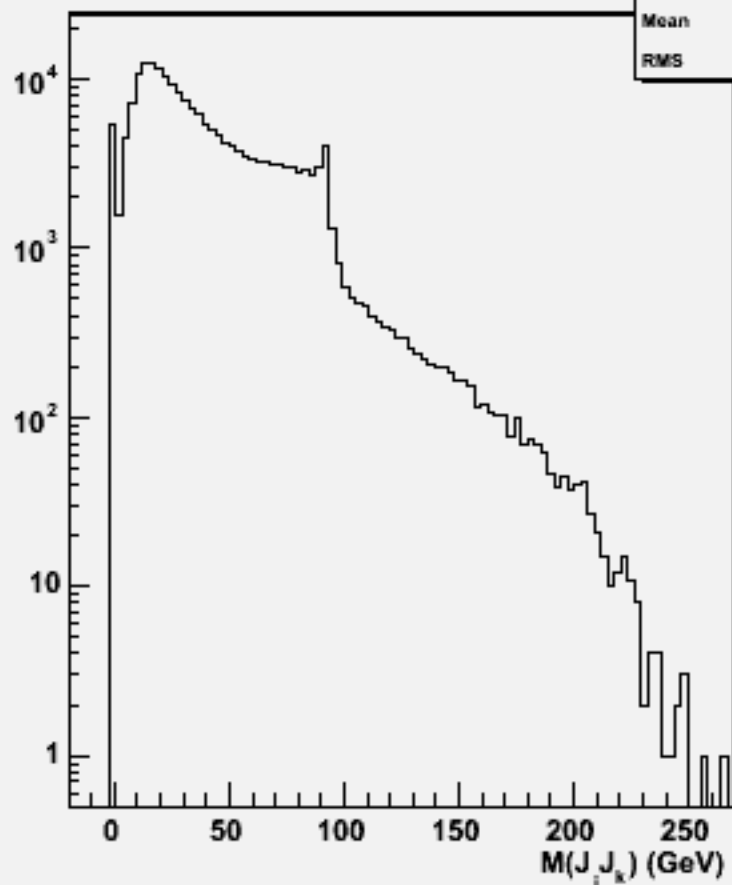
2jets mass(All comb)w100544 n2n2ss_o
