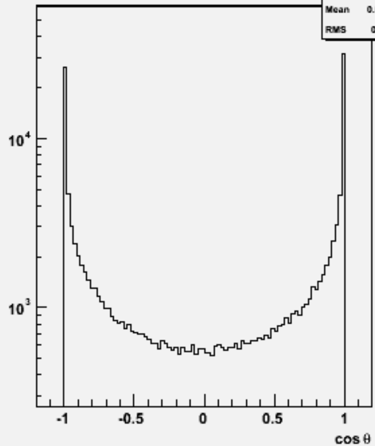
Particle cos \theta : w100533 n2n2e1e1_o
