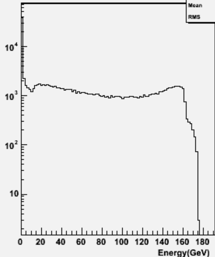
Start point R : w100533 n2n2e1e1_o
