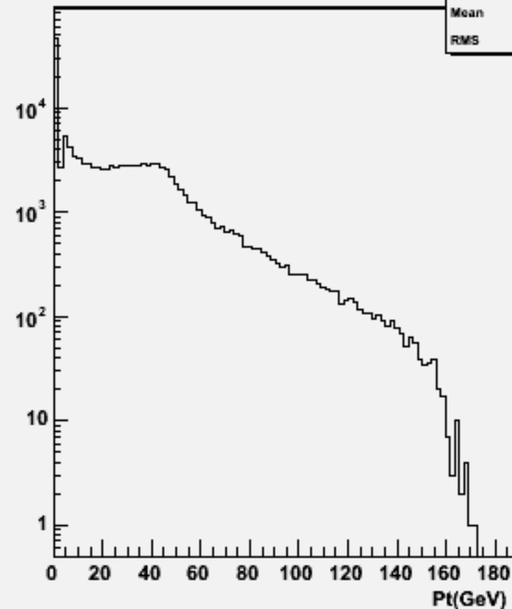
Start point Z : w100533 n2n2e1e1_o
