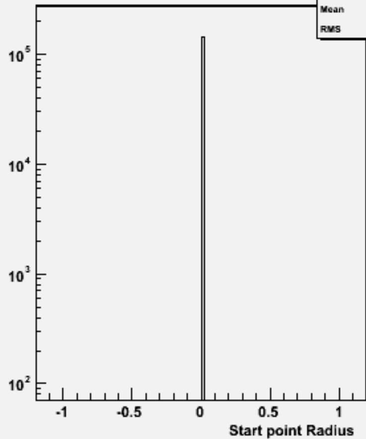
Start point R : w100533 n2n2e1e1_o
