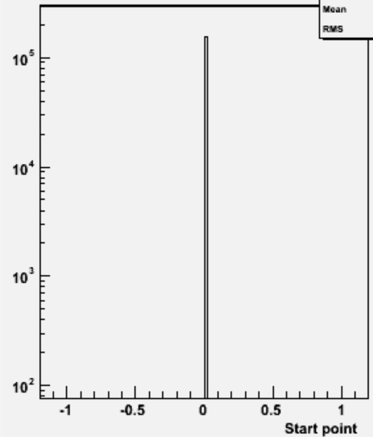
Start point Z : w100531 n2n2e1e1_o
