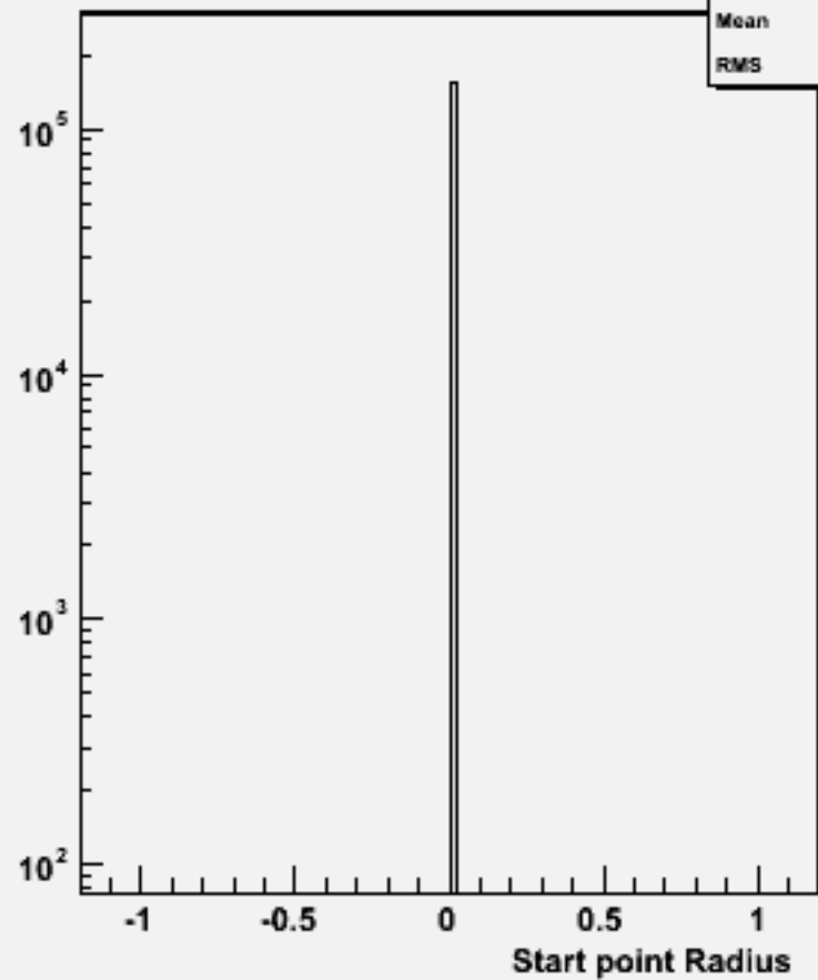
Start point R : w100531 n2n2e1e1_o
