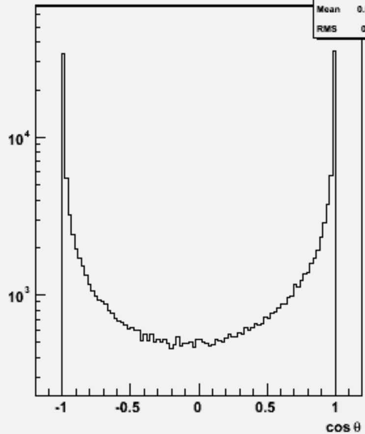
Particle cos \theta : w100531 n2n2e1e1_o
