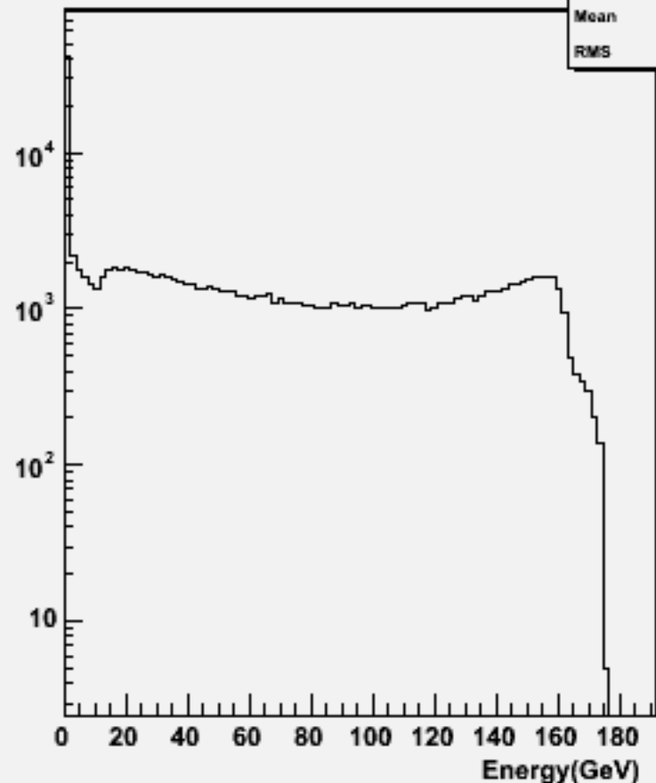
Start point R : w100531 n2n2e1e1_o
