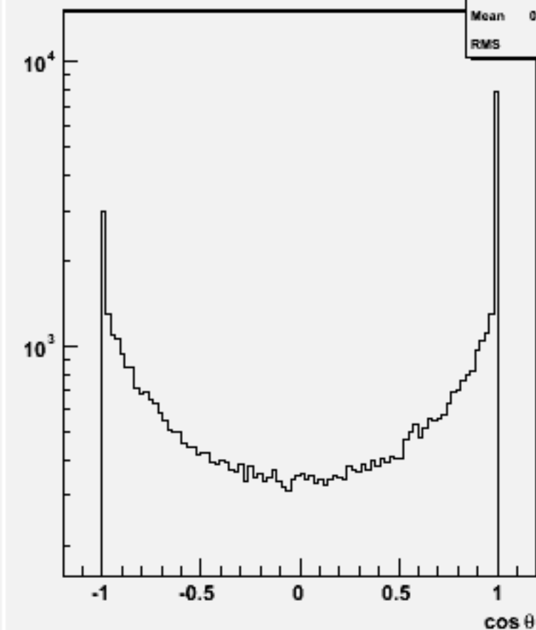
Jet cos \theta (All jets)w100529 n1n1bb_o
