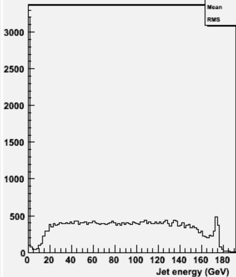
energy for 2-jets :w100529 n1n1bb_o
