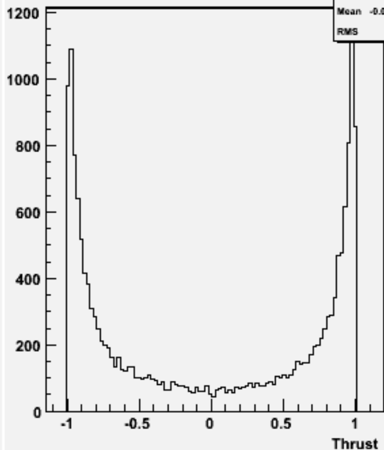
cos \Theta (thrust) w100529 n1n1bb_o
