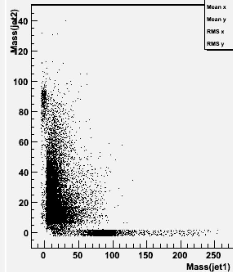
Jet mass for forced 2-jets : w100529 n1n1bb_o
