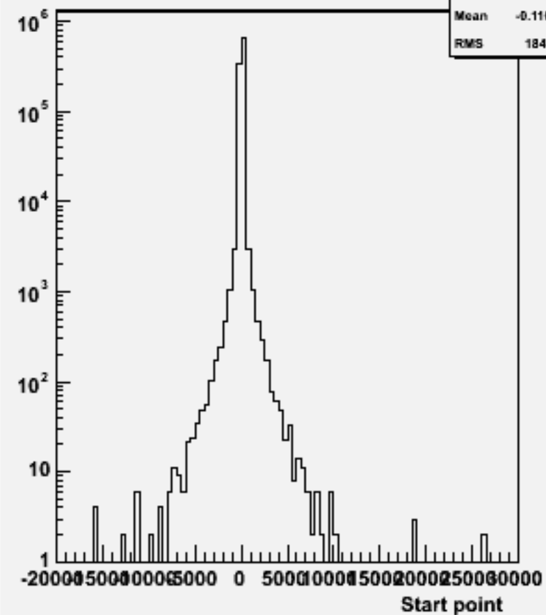
Start point Z : w100529 n1n1bb_o
