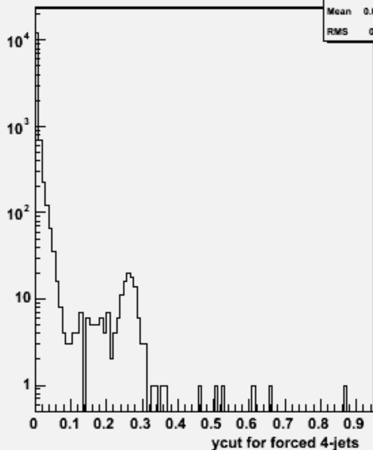
Ycut for 4-jets :w100529 n1n1bb_o
