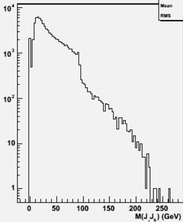
2jets mass(All comb)w100529 n1n1bb_o
