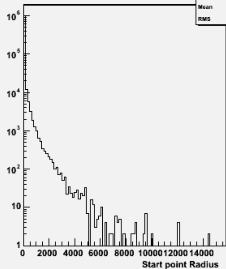
Start point R : w100529 n1n1bb_o
