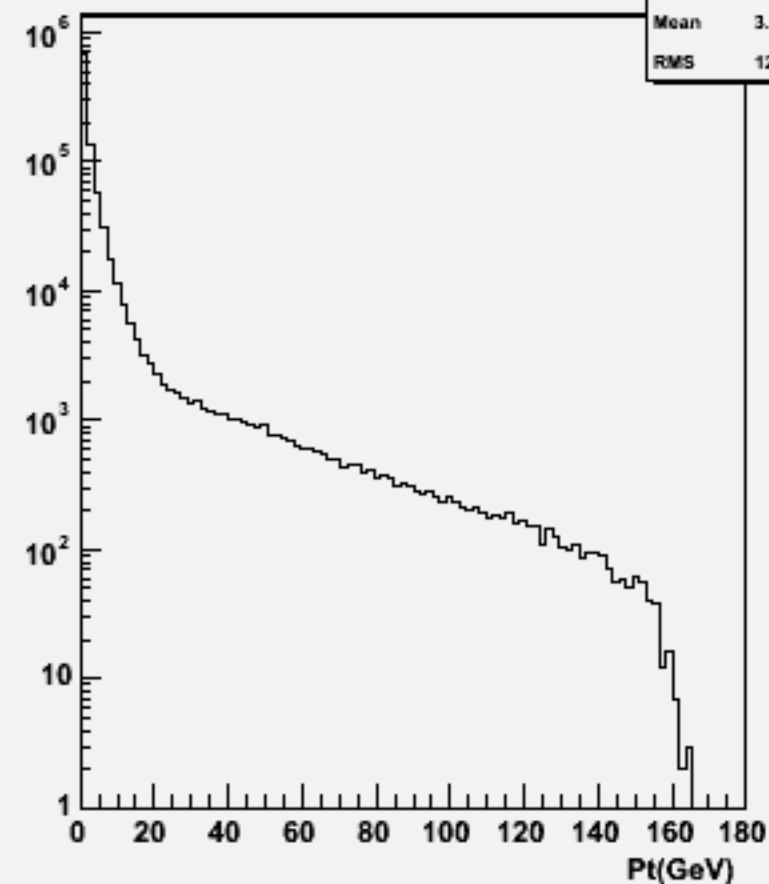
Particle Pt : w100529 n1n1bb_o
