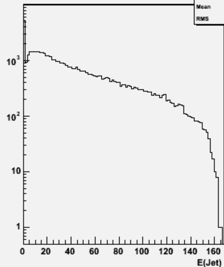
Jet energies(All jets)w100529 n1n1bb_o
