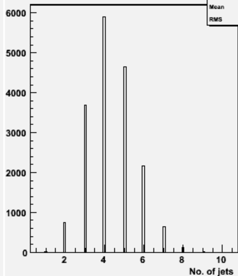
No. jets (ycut=0.001) : w100529 n1n1bb_o
