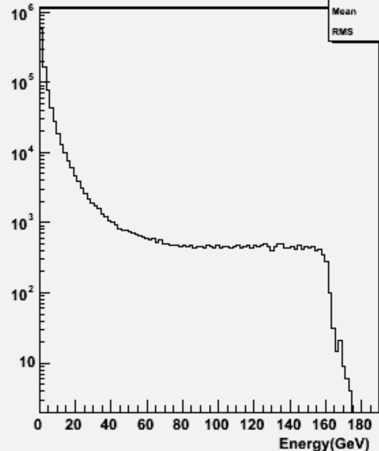
Particle Energy : w100529 n1n1bb_o
