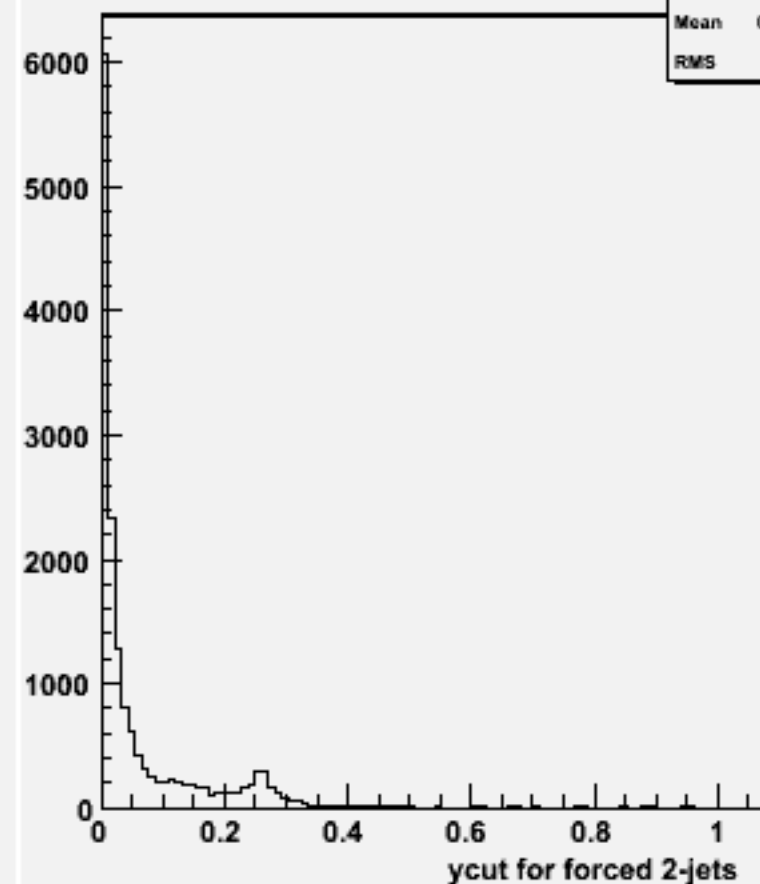
Ycut for 2-jets :w100529 n1n1bb_o
