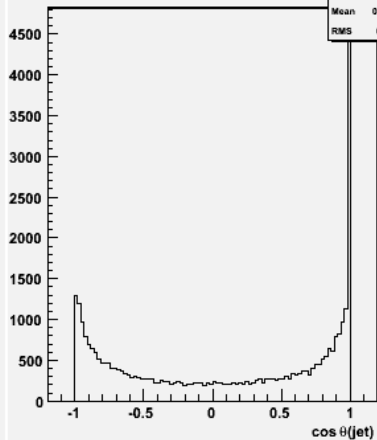
cos \theta for 2-jets :w100529 n1n1bb_o
