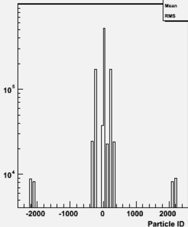
Particle ID : w100529 n1n1bb_o
