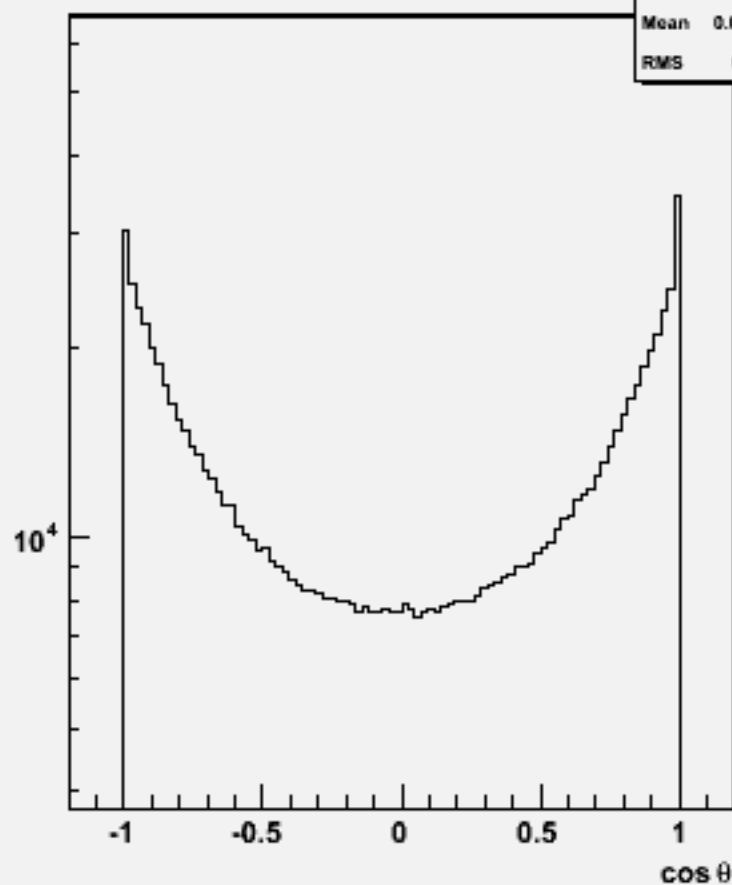
Particle cos \theta : w100529 n1n1bb_o
