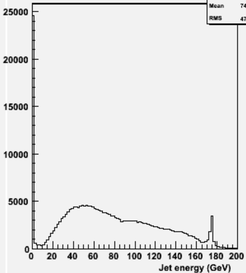
energy for 2-jets :w100524 n1n1ss_o
