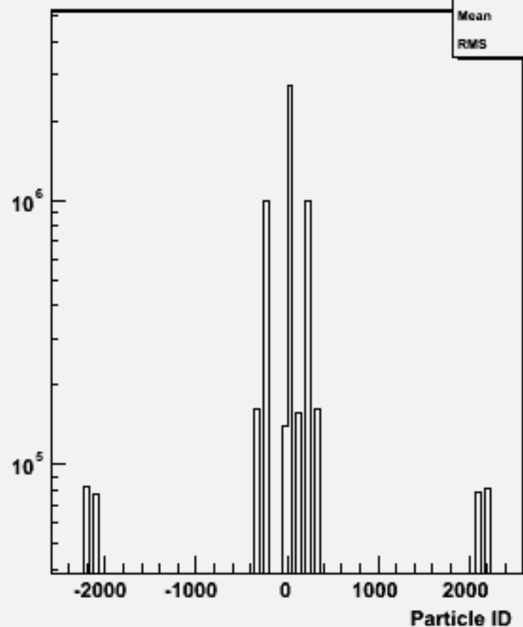
Particle ID : w100524 n1n1ss_o
