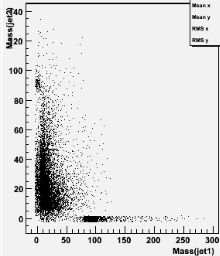
Jet mass for forced 2-jets : w100524 n1n1ss_o
