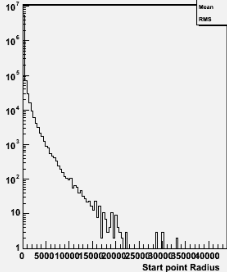
Start point R : w100524 n1n1ss_o
