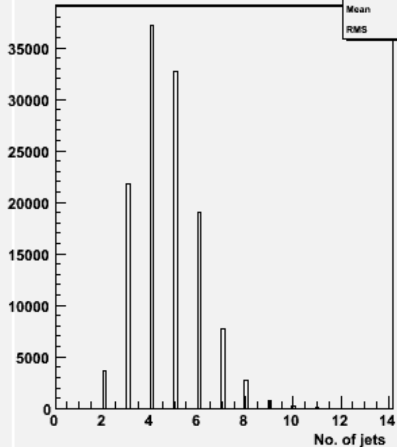
No. jets (ycut=0.001) : w100524 n1n1ss_o
