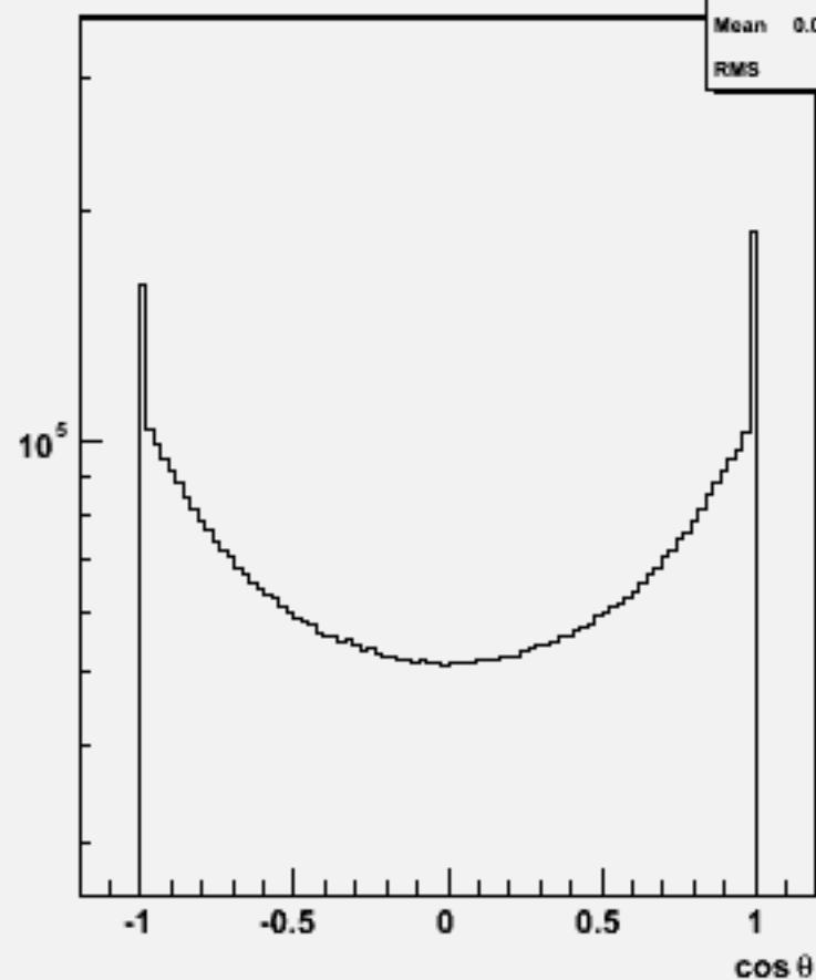
Particle \cos\theta : w100524 n1n1ss_o
