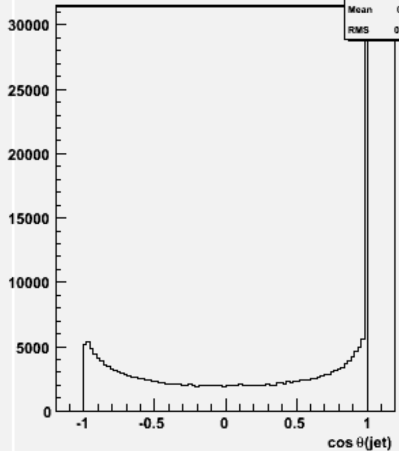
cos \theta for 2-jets :w100524 n1n1ss_o
