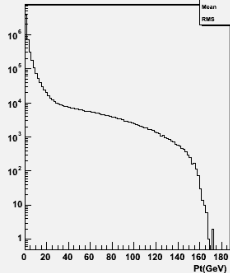
Particle Pt : w100524 n1n1ss_o
