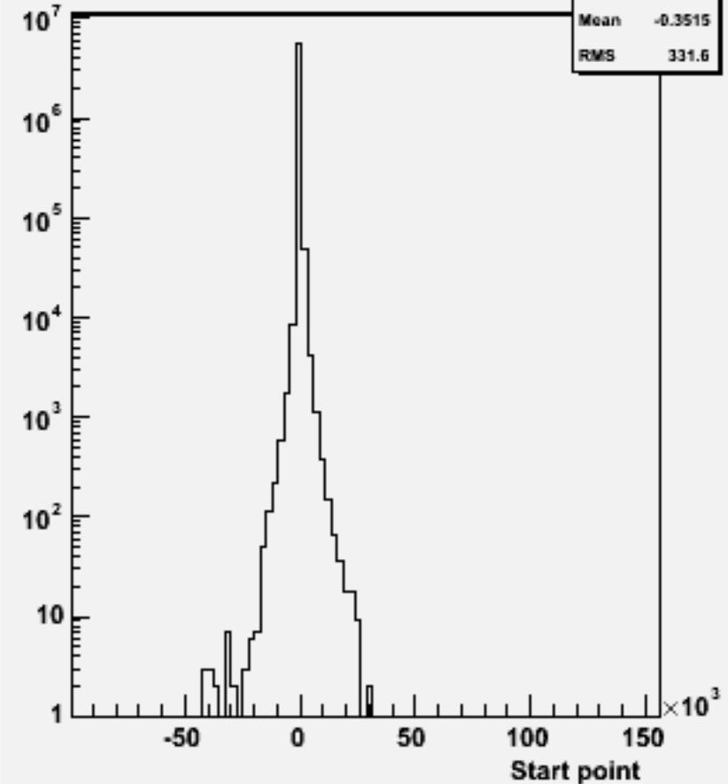
Start point Z : w100524 n1n1ss_o
