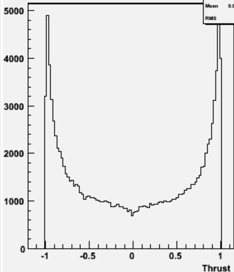
cos \theta (thrust) w100524 n1n1ss_o
