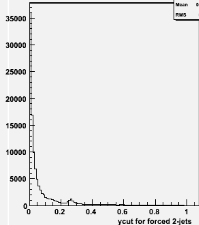
Ycut for 2-jets :w100524 n1n1ss_o
