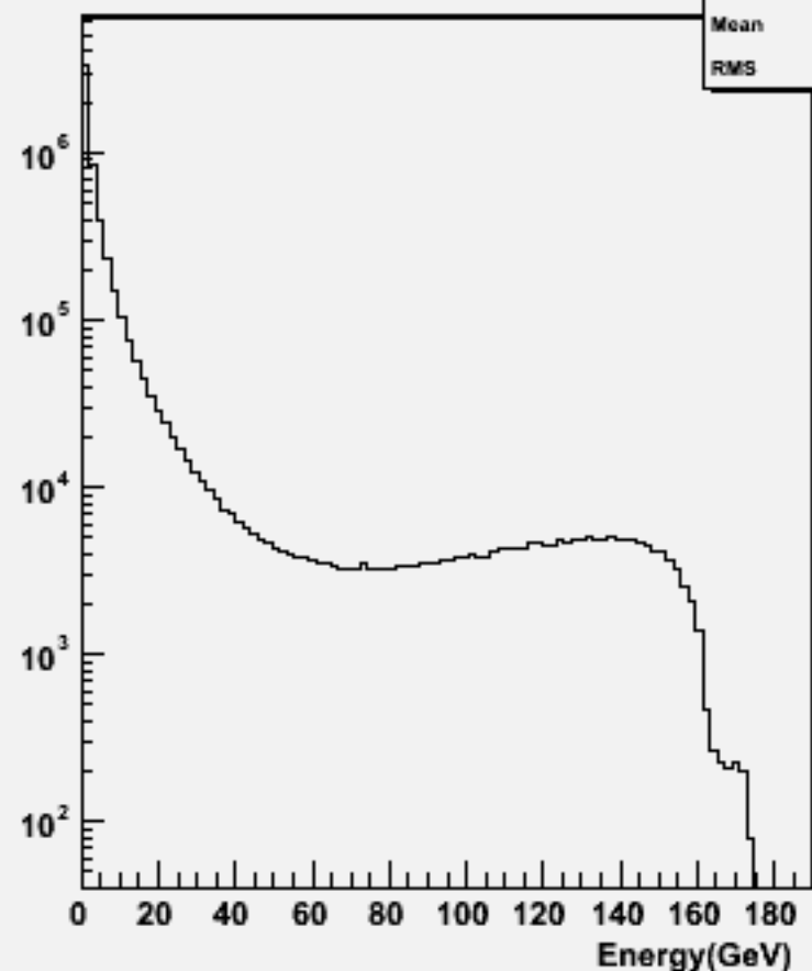
Particle Energy : w100524 n1n1ss_o
