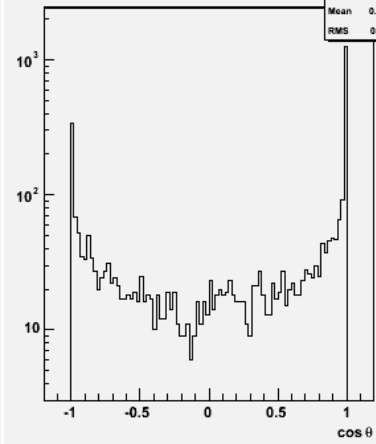
Jet cosθ (All jets)w100513 n1n1e2e2_o
