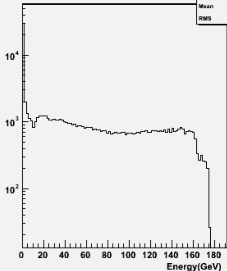
Particle Energy : w100513 n1n1e2e2_o
