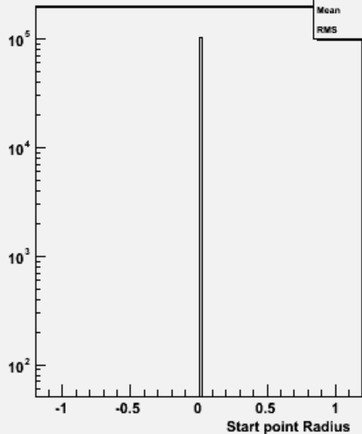
Start point R : w100513 n1n1e2e2_o
