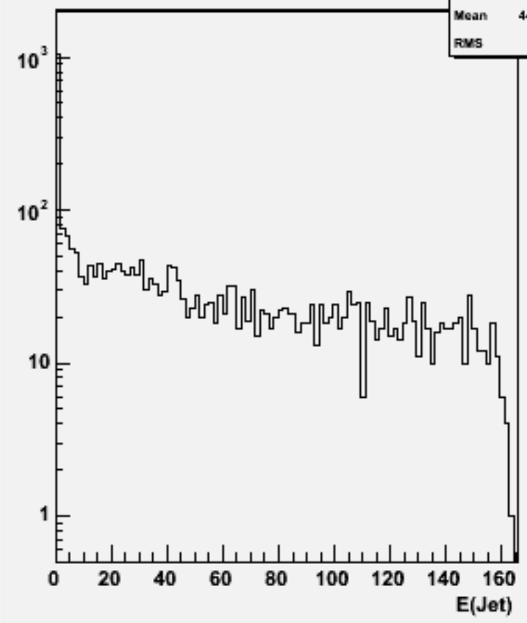
Jet energies(All jets)w100513 n1n1e2e2_o
