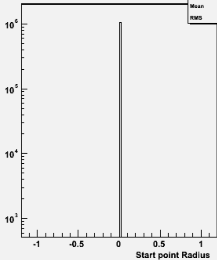
Start point R : w100512 n1n1e2e2_o
