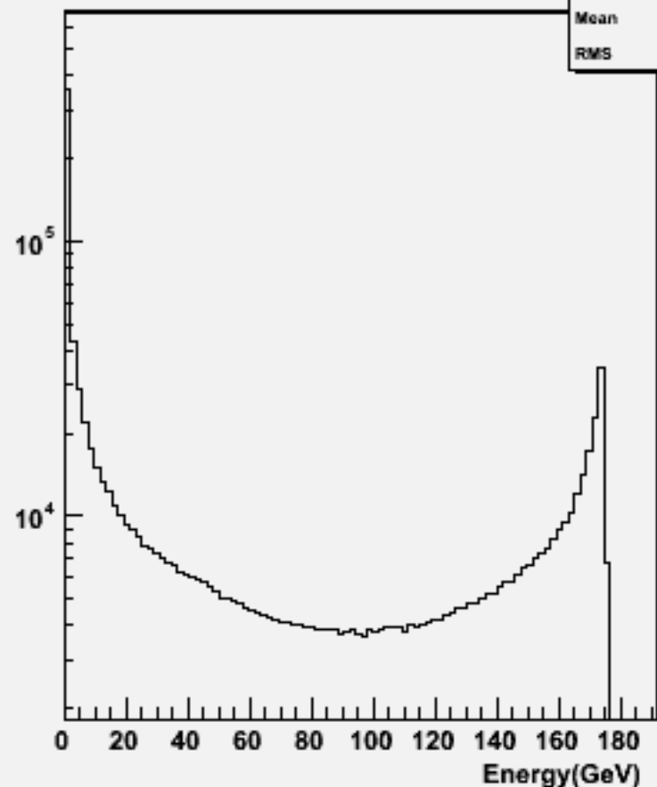
Start point R : w100512 n1n1e2e2_o
