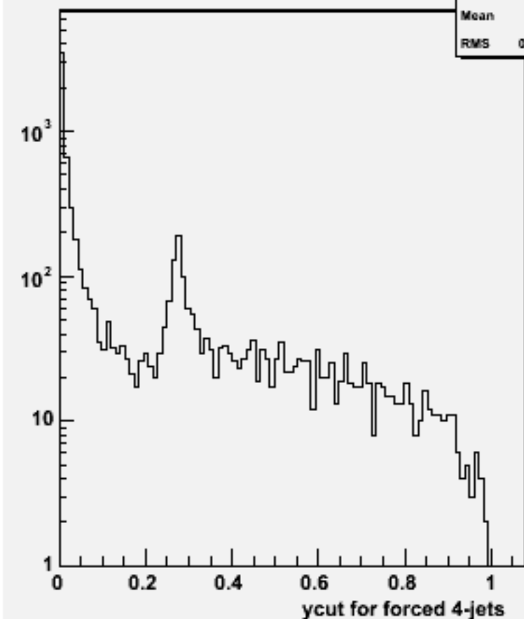
Ycut for 4-jets :w100512 n1n1e2e2_o
