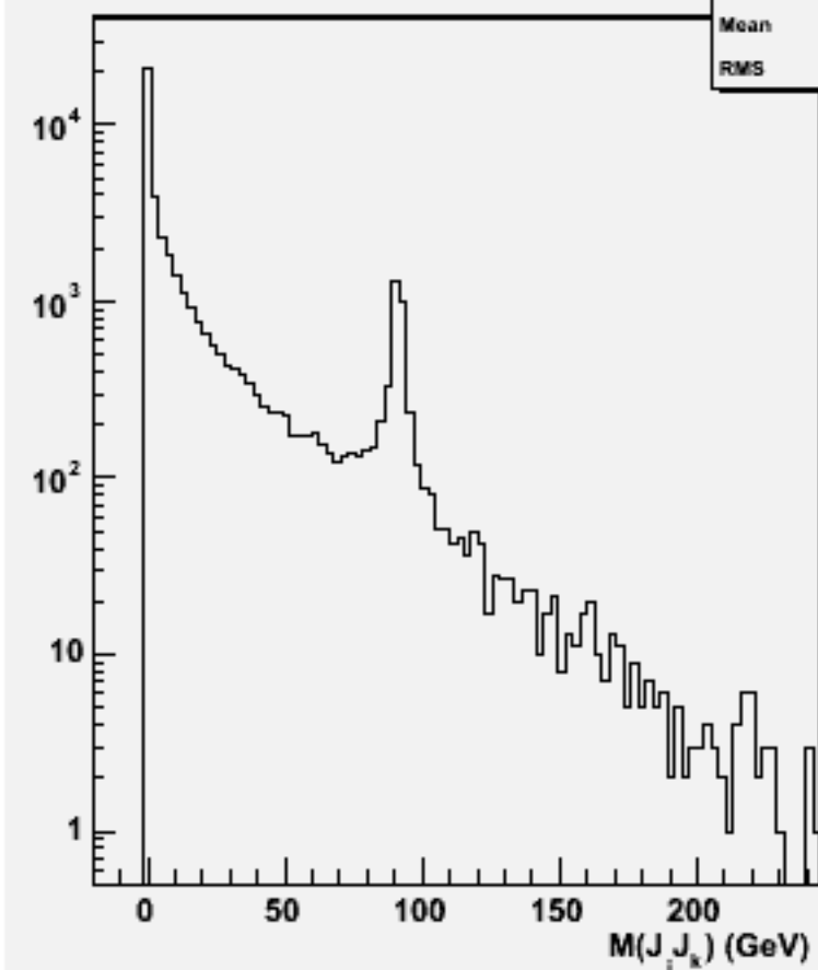
2jets mass(All comb)w100512 n1n1e2e2_o
