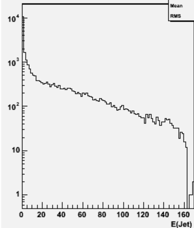
Jet energies(All jets)w100512 n1n1e2e2_o
