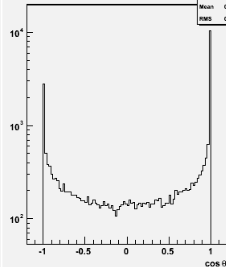
Jet cos \theta (All jets)w100512 n1n1e2e2_o
