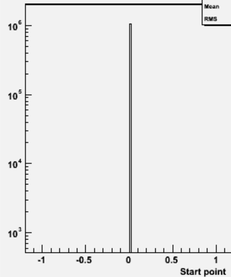
Start point Z : w100512 n1n1e2e2_o
