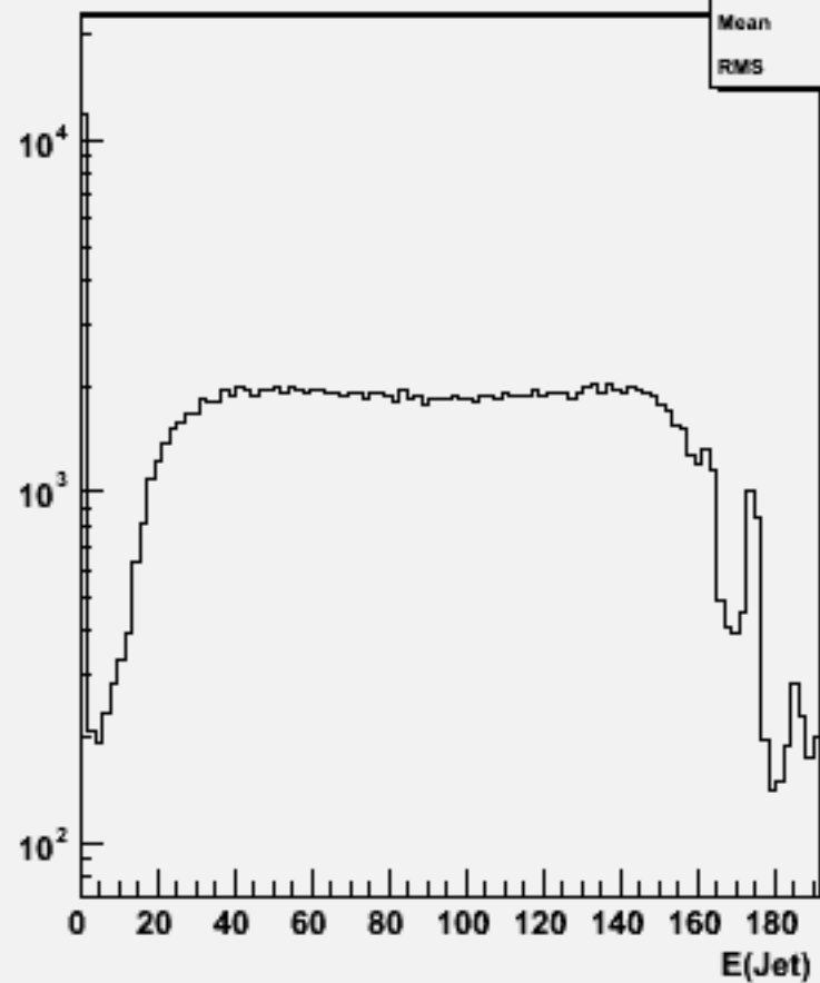
Jet energies(All jets)w100500 uuuu_o
