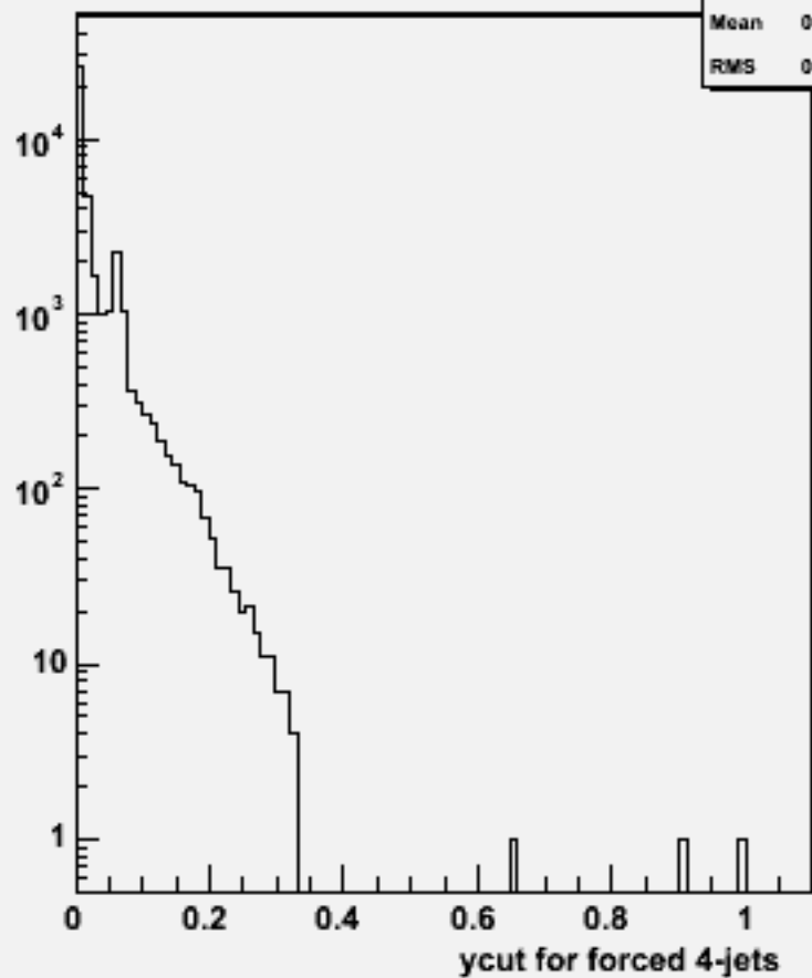
Ycut for 4-jets :w100500 uuuu_o
