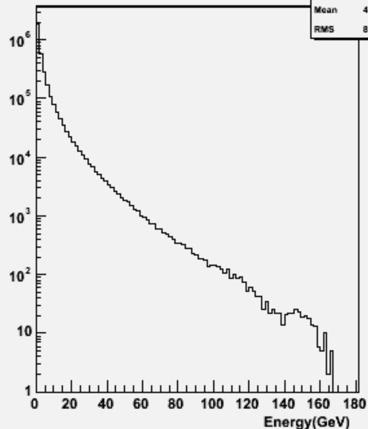
Particle Energy : w100500 uuuu_o
