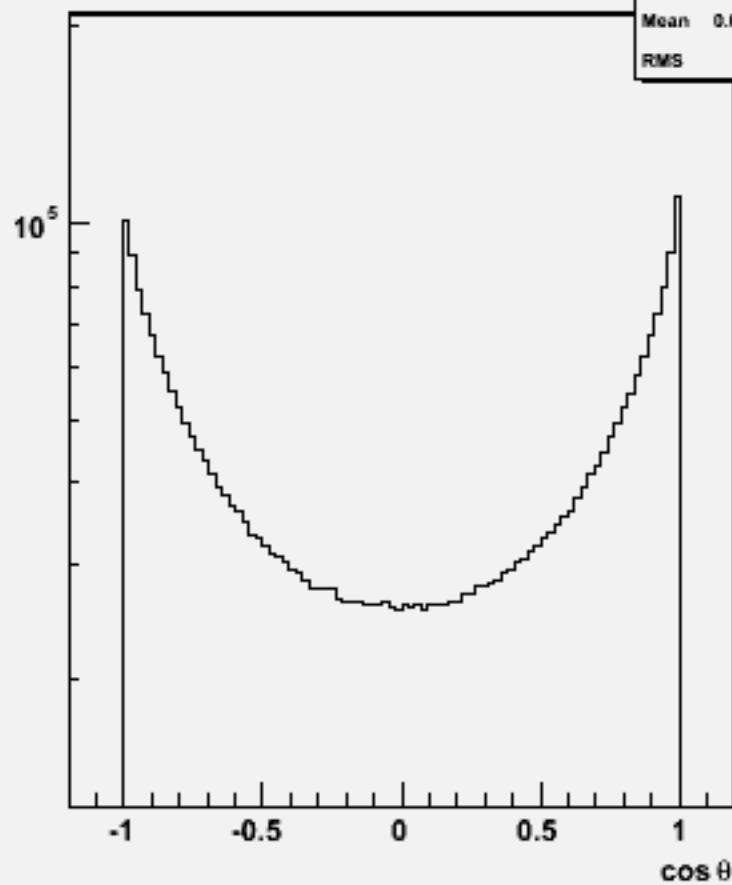
Particle cosθ : w100500 uuuu_o
