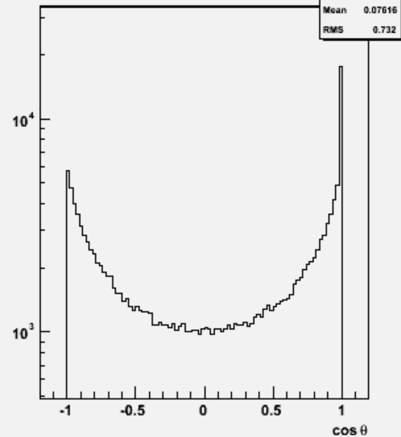
Jet cosθ (All jets)w100500 uuuu_o
