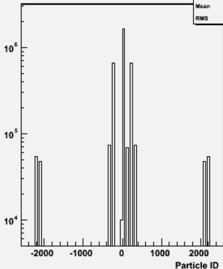
Particle ID : w100500 uuuu_o
