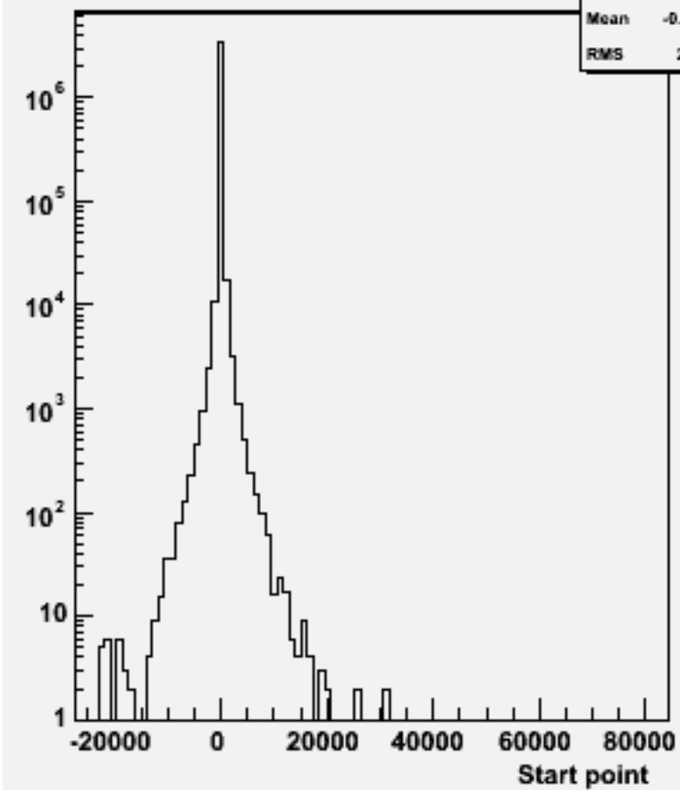
Start point Z : w100500 uuuu_o
