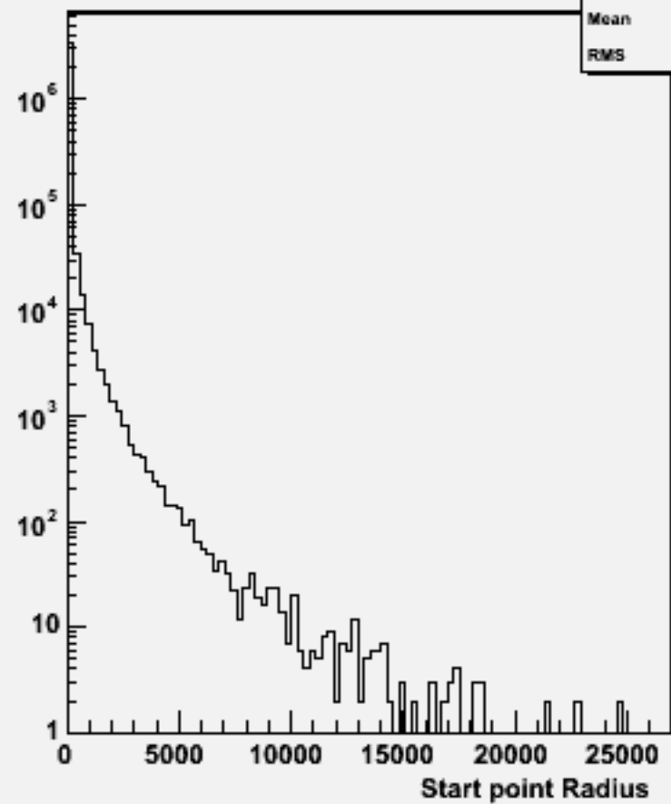
Start point R : w100500 uuuu_o
