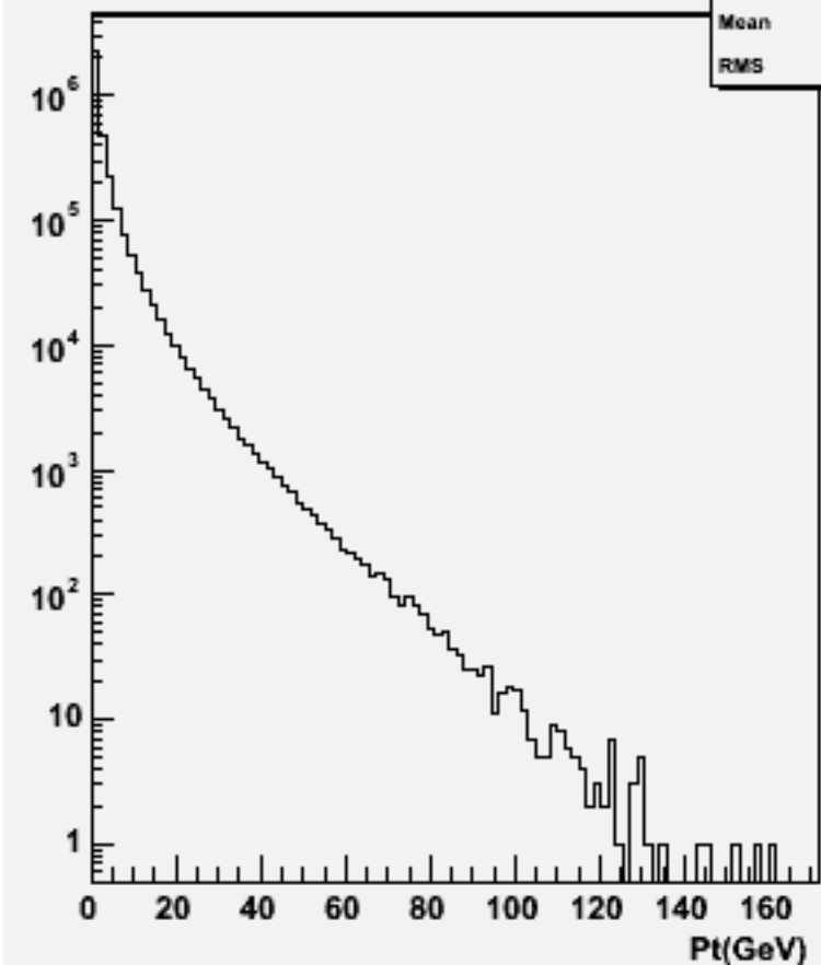
Particle Pt : w100500 uuuu_o
