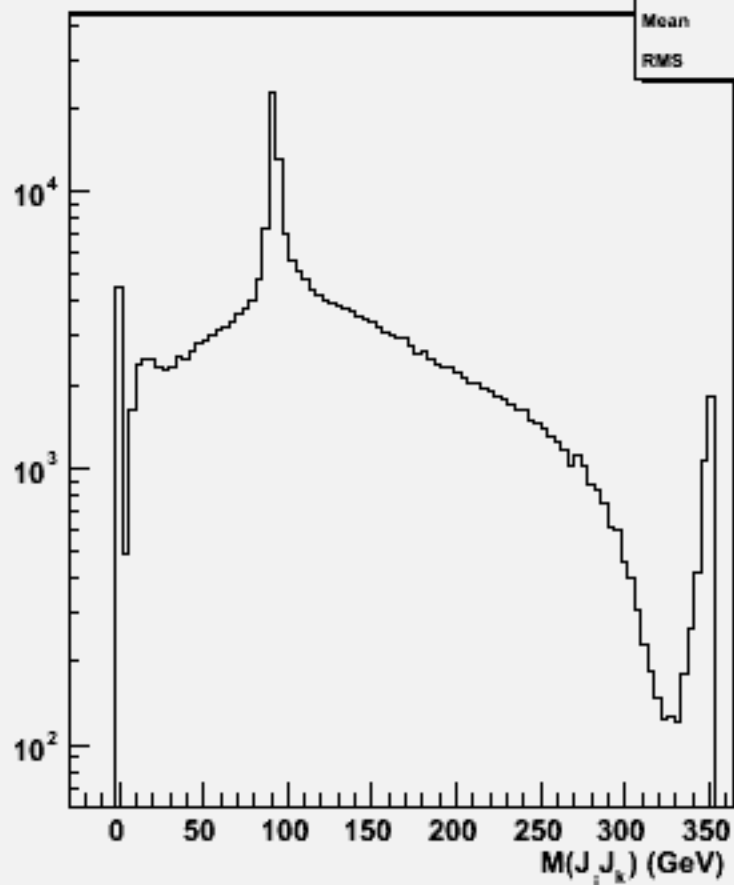
2jets mass(All comb)w100500 uuuu_o
