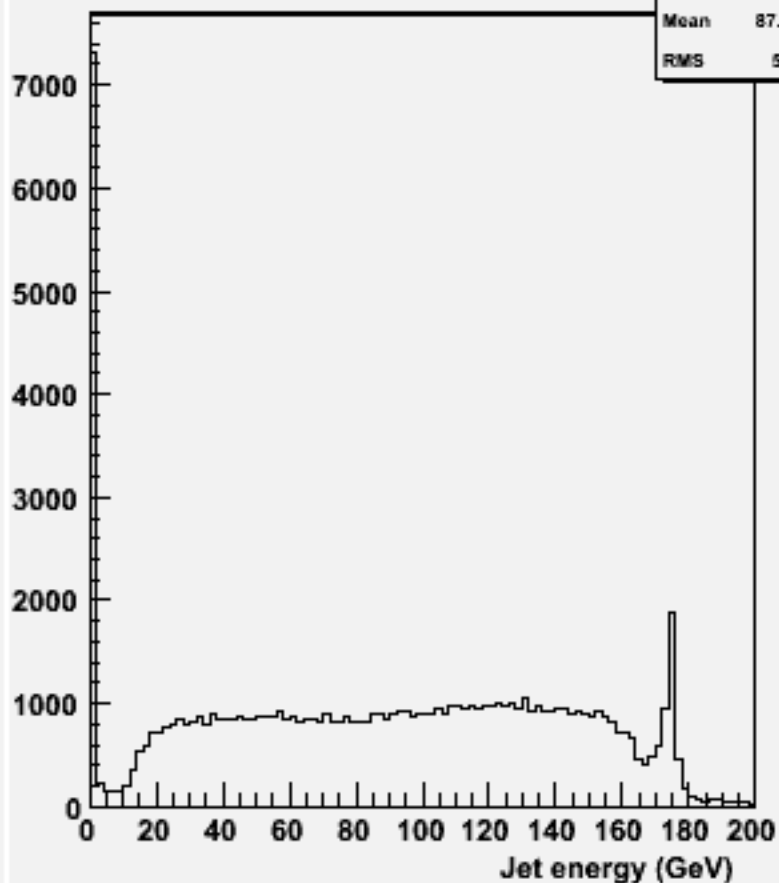
energy for 2-jets :w100496 n3n3cc_o
