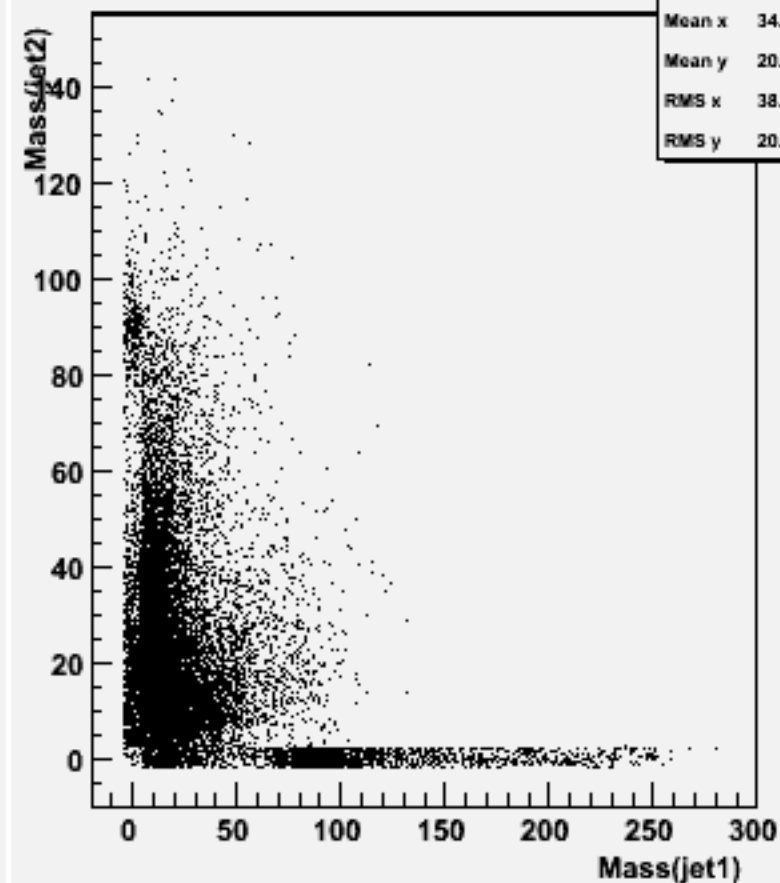
Jet mass for forced 2-jets : w100496 n3n3cc_o
