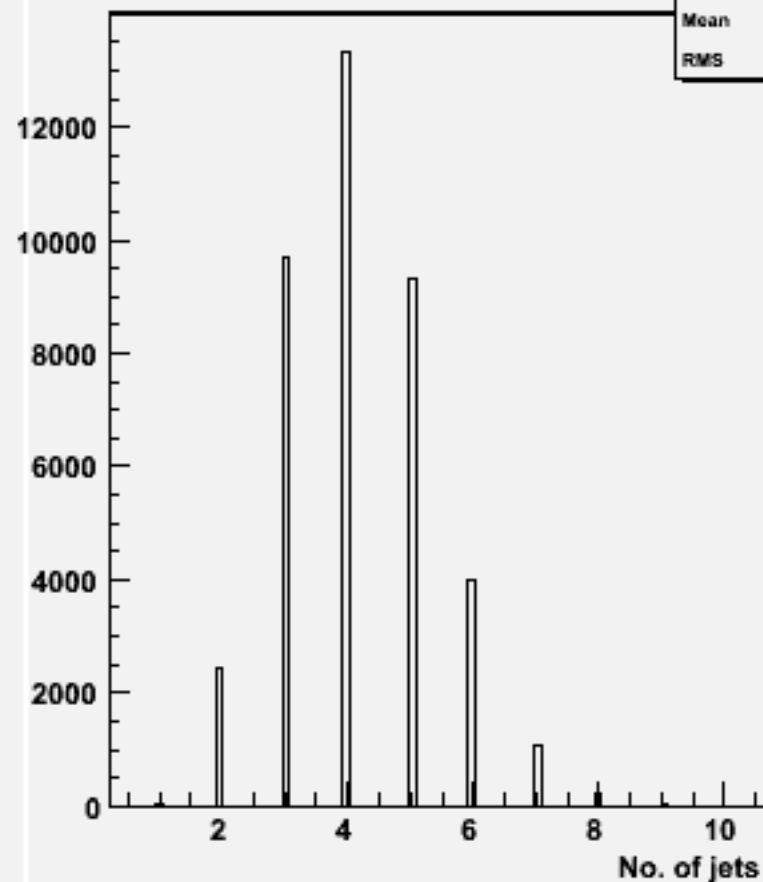
No. jets (ycut=0.001) : w100496 n3n3cc_o
