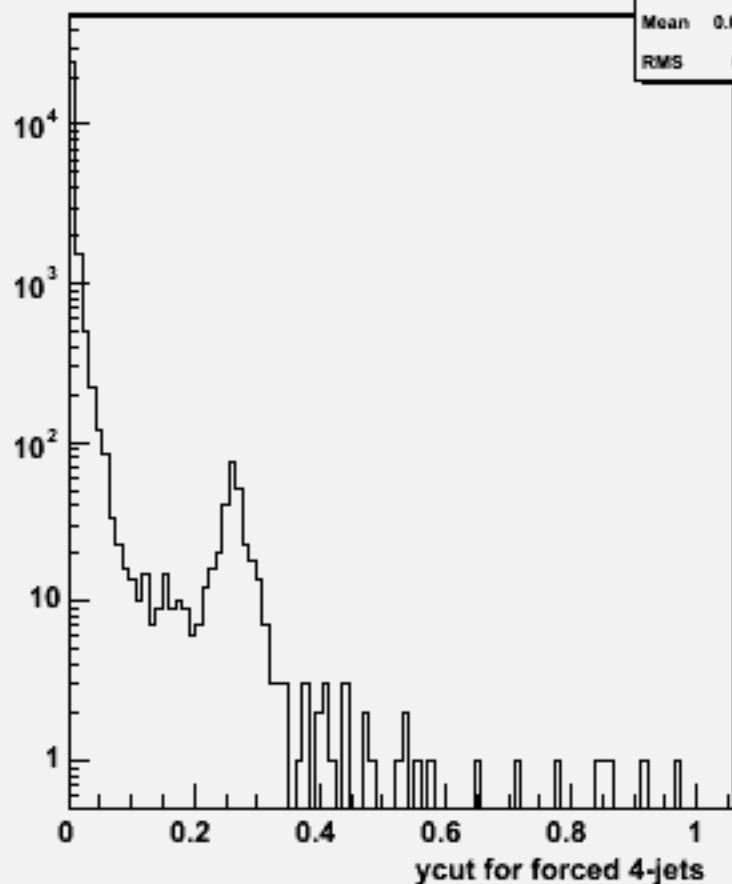
Ycut for 4-jets :w100496 n3n3cc_o
