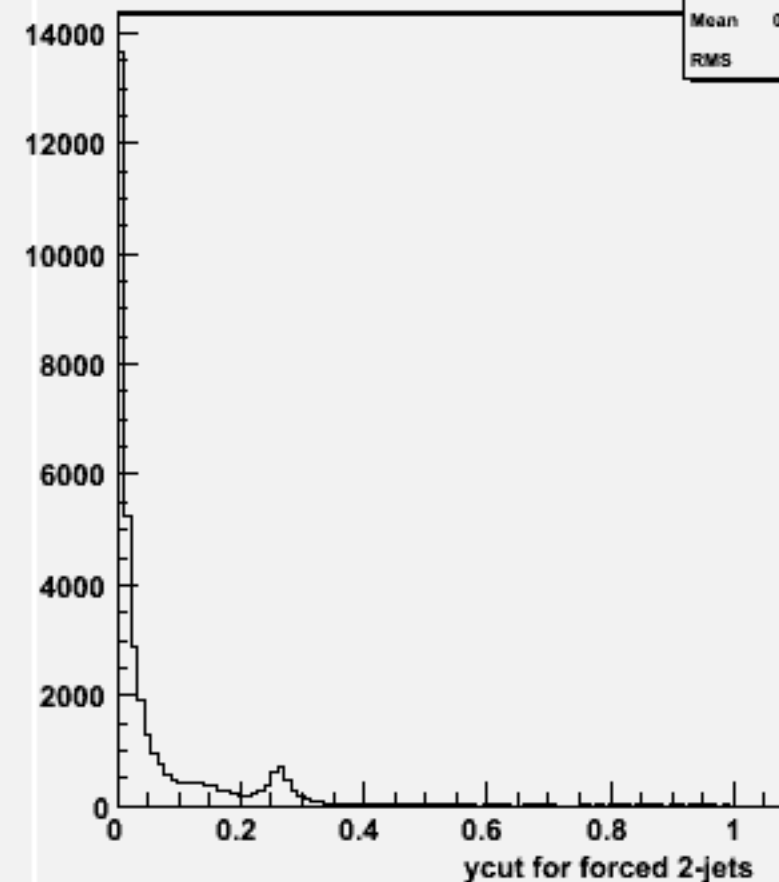
Ycut for 2-jets :w100496 n3n3cc_o
