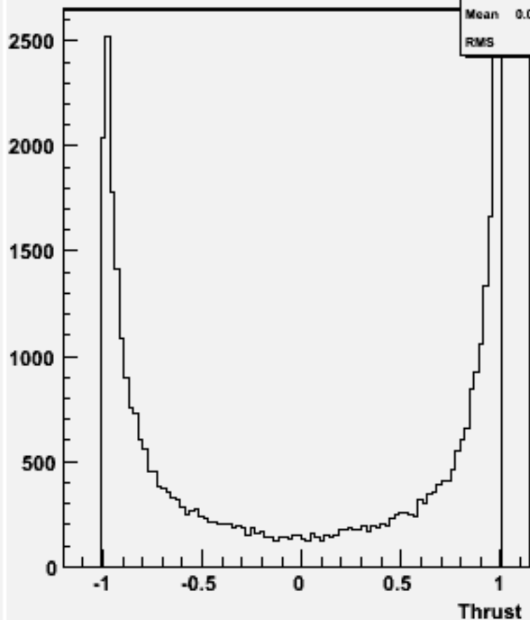
cos \Theta (thrust) w100496 n3n3cc_o
