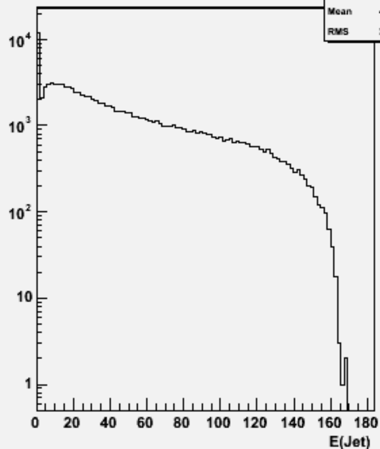
Jet energies(All jets)w100488 n2n2cc_o
