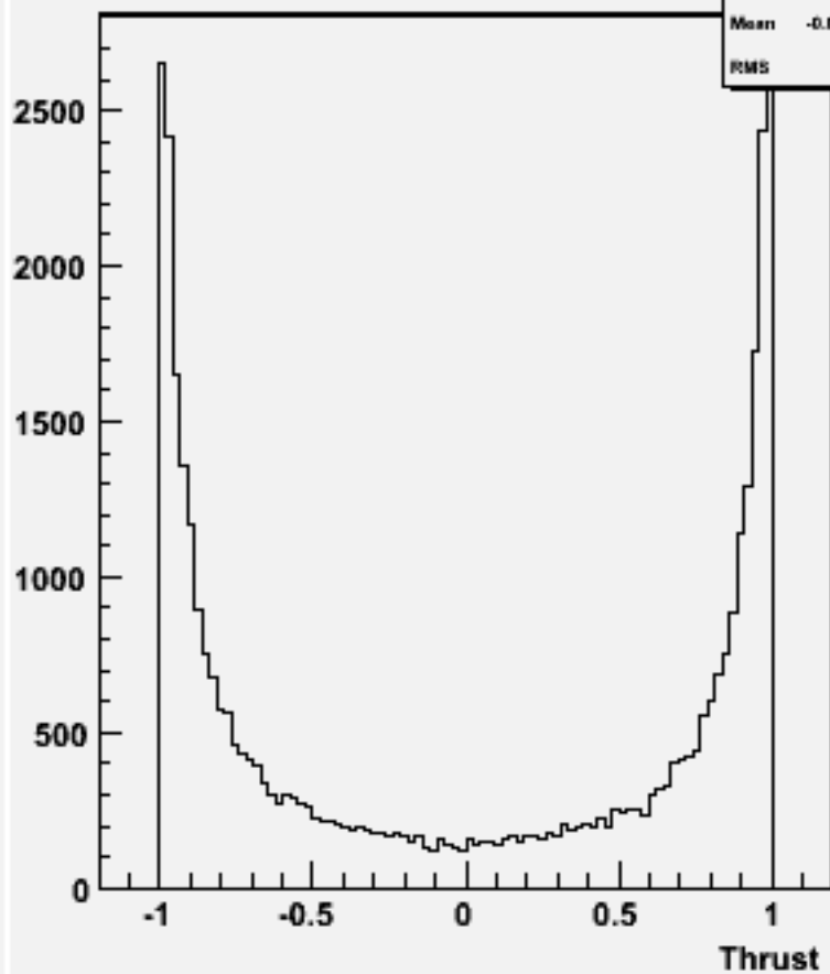
cos \Theta (thrust) w100488 n2n2cc_o
