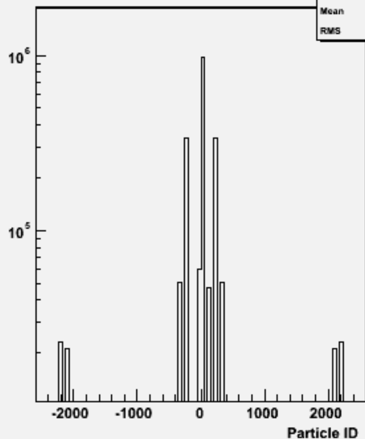
Particle ID : w100488 n2n2cc_o
