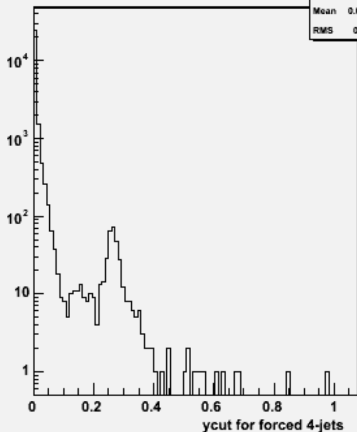
Ycut for 4-jets :w100488 n2n2cc_o
