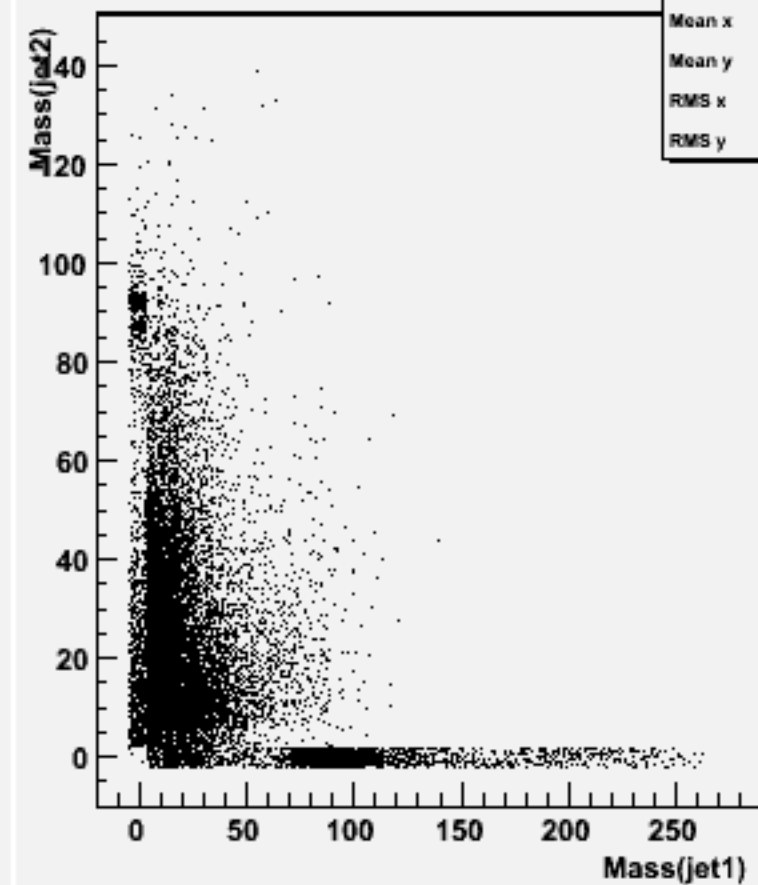
Jet mass for forced 2-jets : w100488 n2n2cc_o
