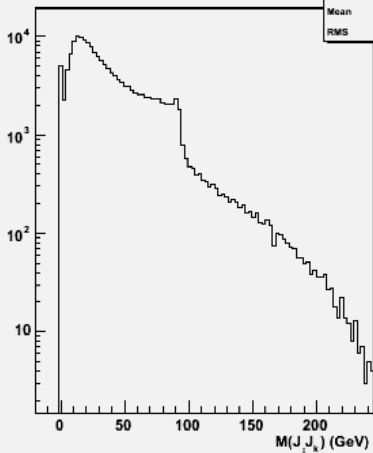
2jets mass(All comb)w100488 n2n2cc_o
