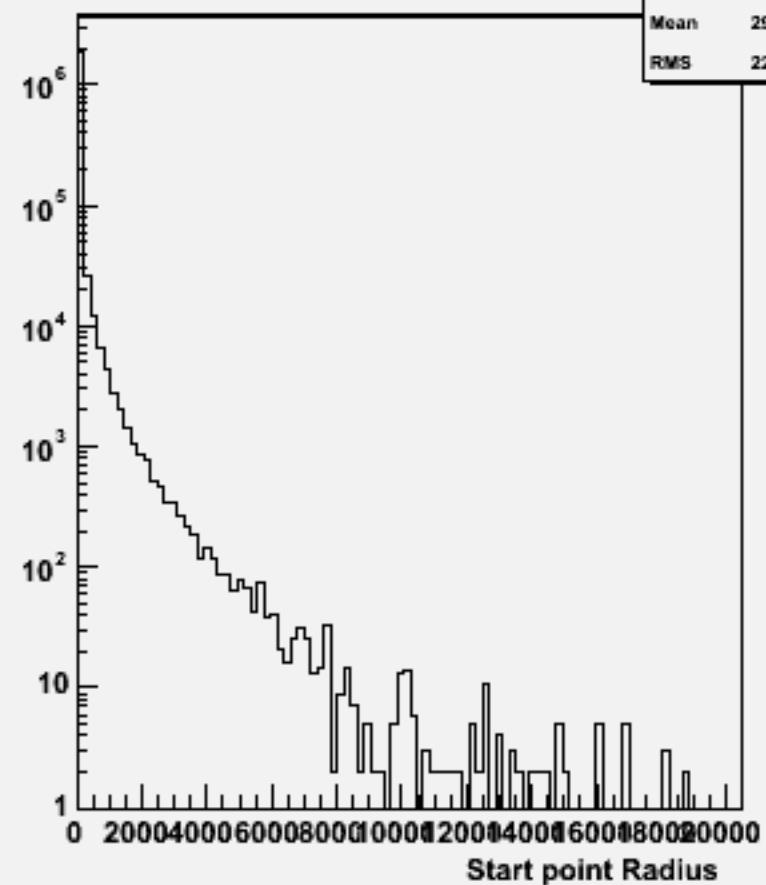
Start point R : w100488 n2n2cc_o
