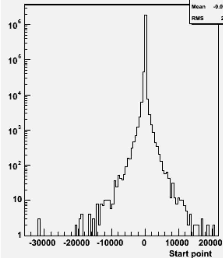
Start point Z : w100488 n2n2cc_o
