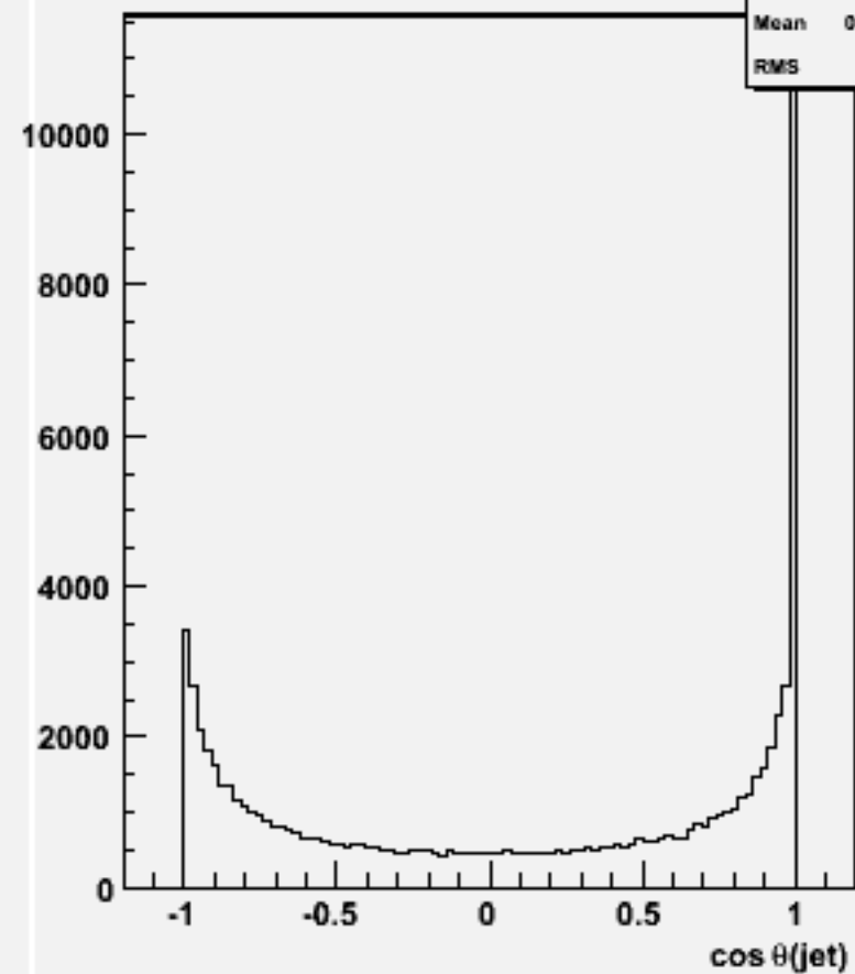
cos \theta for 2-jets :w100488 n2n2cc_o
