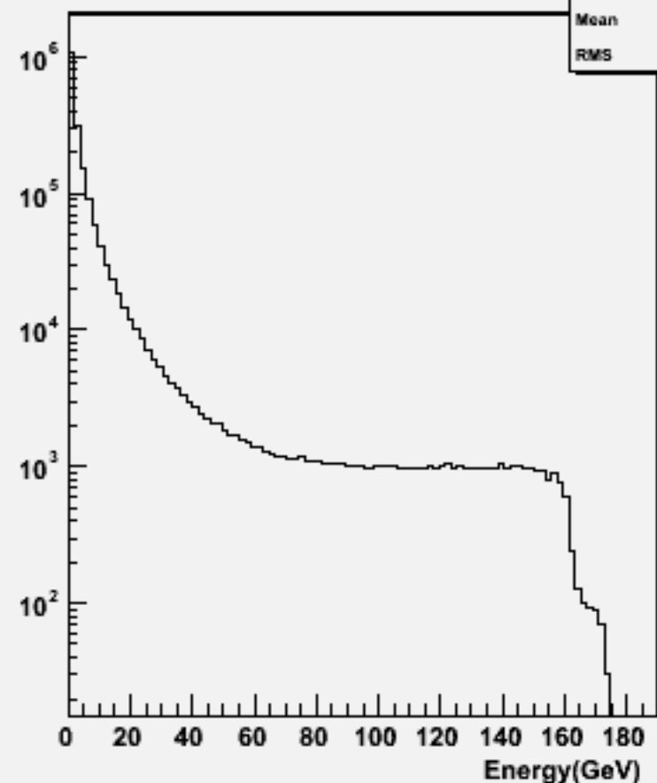
Particle Energy : w100488 n2n2cc_o
