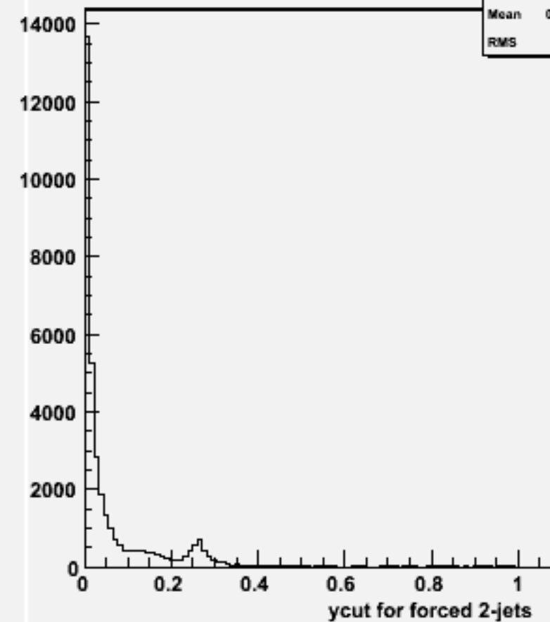
Ycut for 2-jets :w100488 n2n2cc_o
