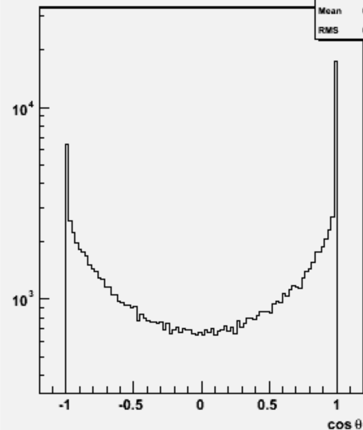
Jet cos \theta (All jets)w100488 n2n2cc_o
