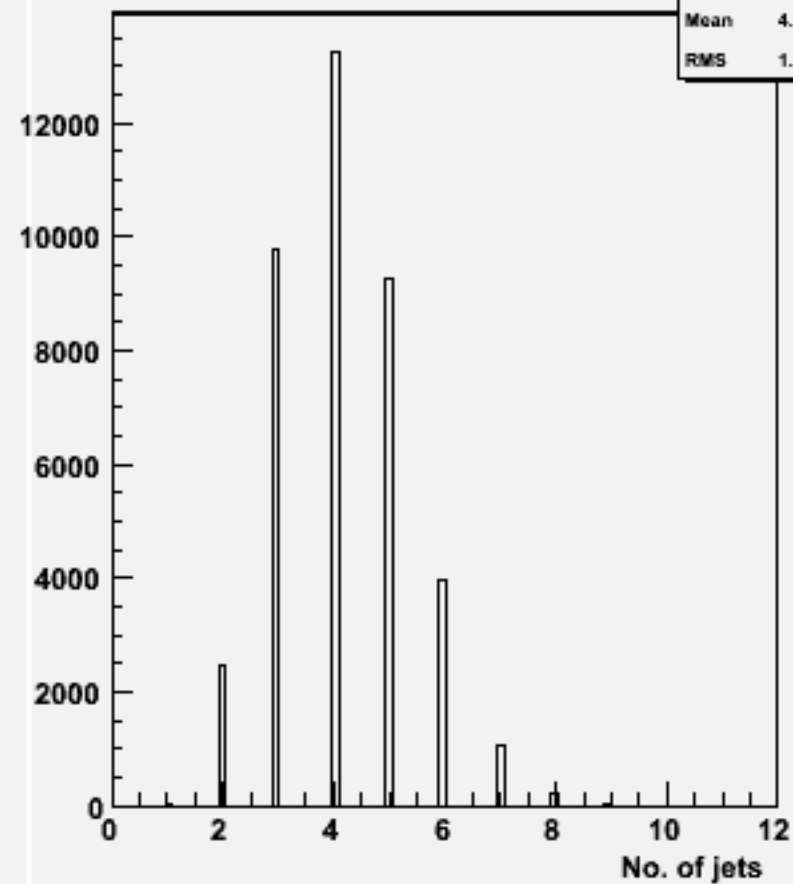
No. jets (ycut=0.001) : w100488 n2n2cc_o
