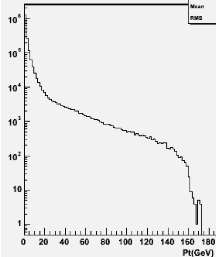
Particle Pt : w100488 n2n2cc_o
