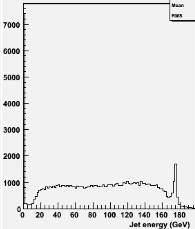
energy for 2-jets :w100488 n2n2cc_o
