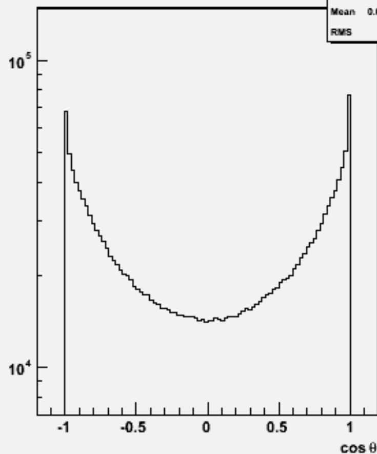
Particle cosθ : w100488 n2n2cc_o
