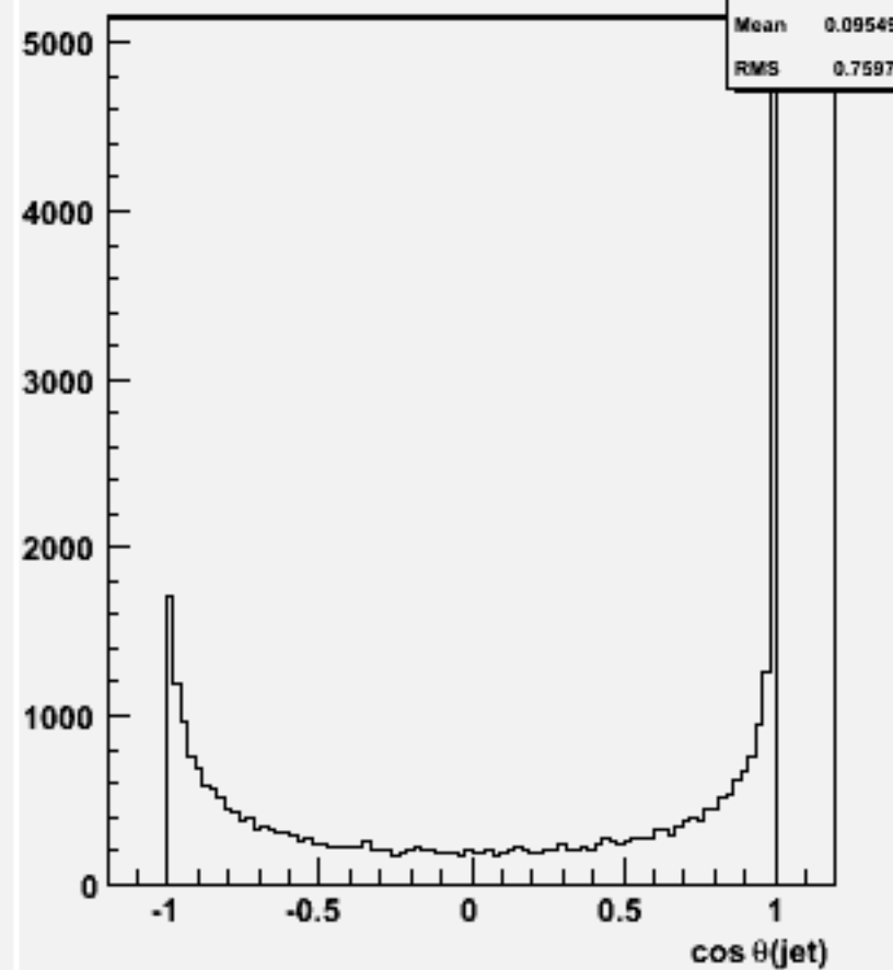
cos \theta for 2-jets :w100481 n1n1cc_o
