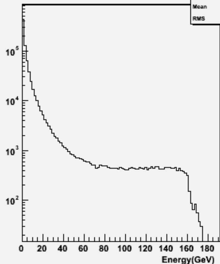
Particle Energy : w100481 n1n1cc_o
