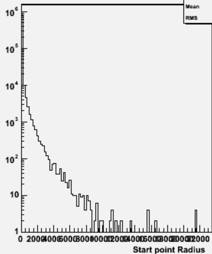
Start point R : w100481 n1n1cc_o
