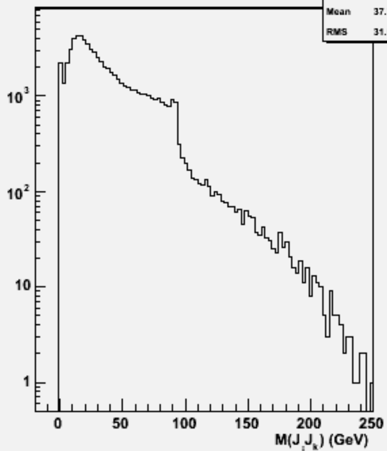
2jets mass(All comb)w100481 n1n1cc_o
