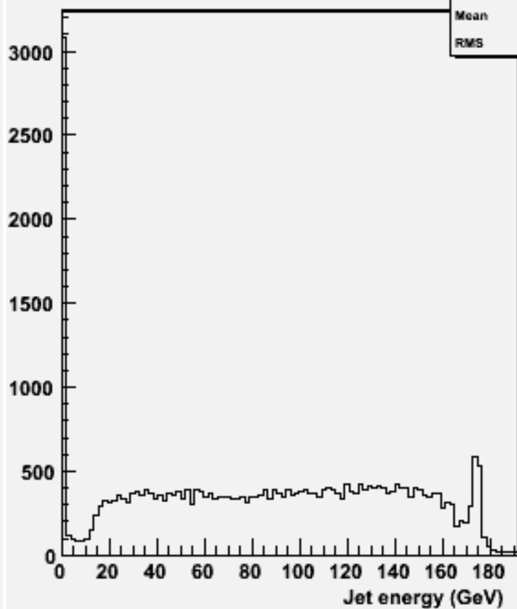
energy for 2-jets :w100481 n1n1cc_o
