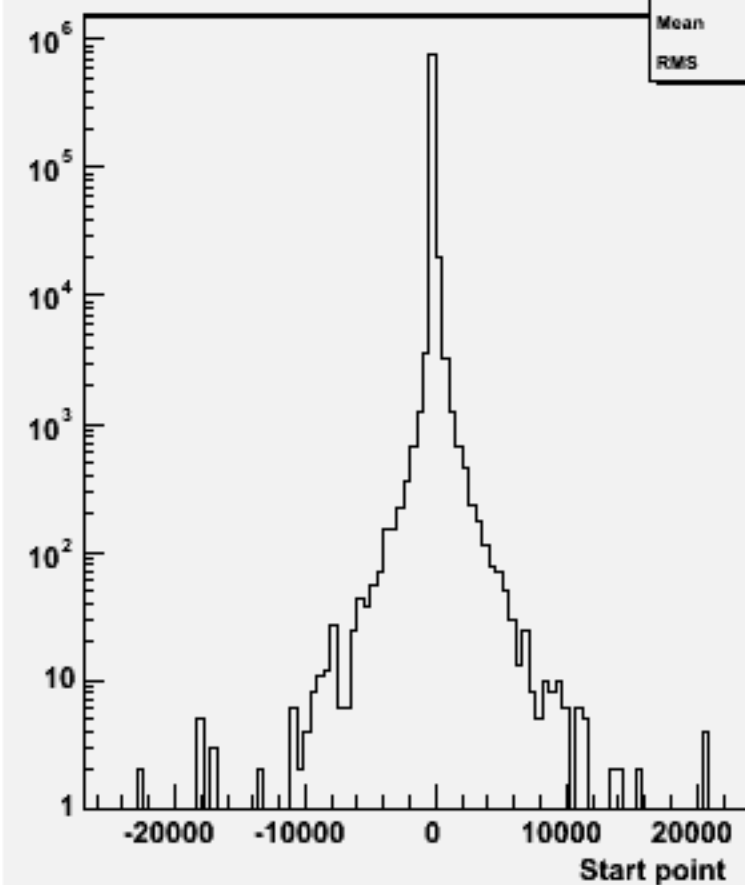
Start point Z : w100481 n1n1cc_o
