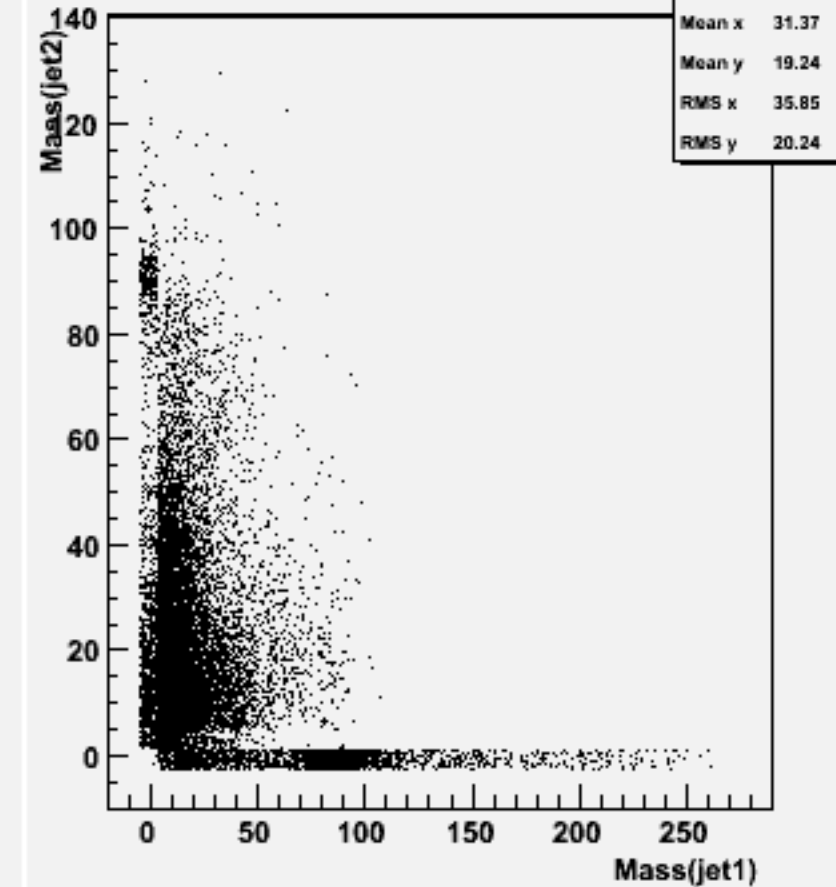
Jet mass for forced 2-jets : w100481 n1n1cc_o
