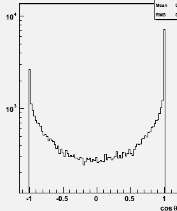
Jet cos \theta (All jets)w100481 n1n1cc_o
