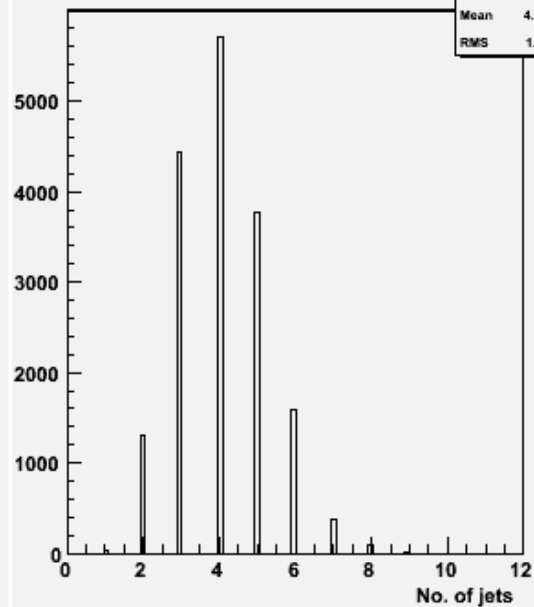
No. jets (ycut=0.001) : w100481 n1n1cc_o
