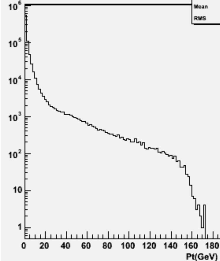
Particle Pt : w100481 n1n1cc_o
