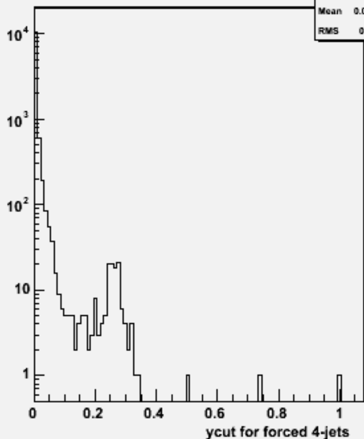
Ycut for 4-jets :w100481 n1n1cc_o
