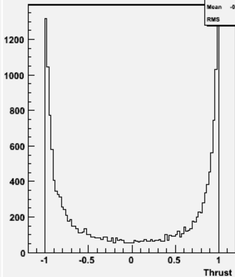
cos \Theta (thrust) w100481 n1n1cc_o
