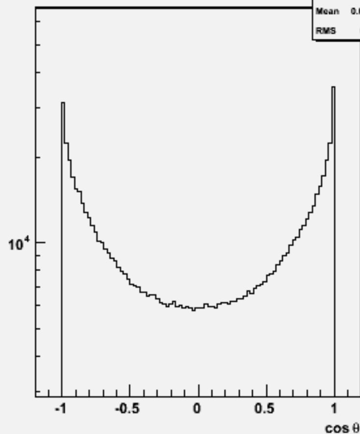
Particle cosθ : w100481 n1n1cc_o
