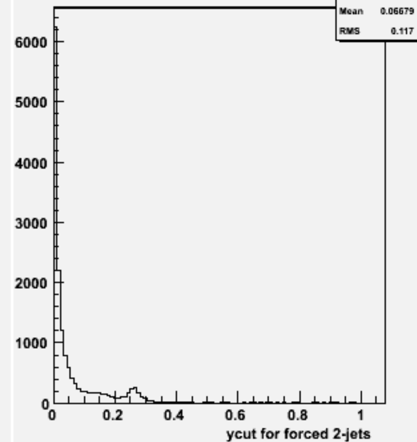
Ycut for 2-jets :w100481 n1n1cc_o
