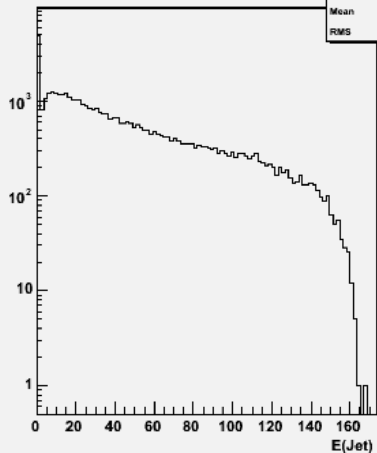
Jet energies(All jets)w100481 n1n1cc_o
