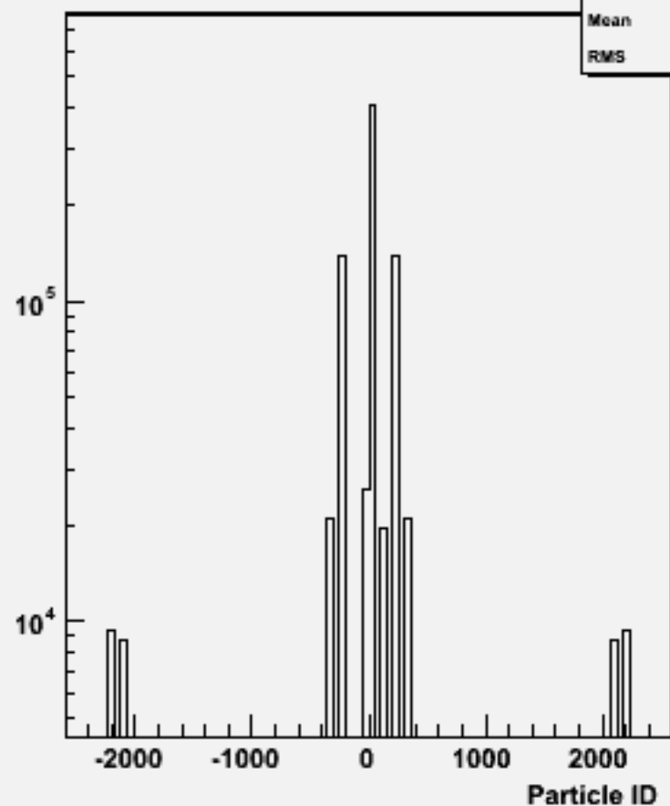
Particle ID : w100481 n1n1cc_o
