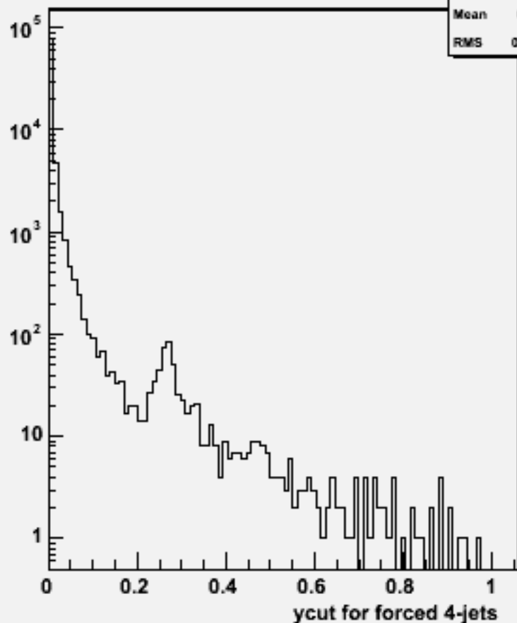
Ycut for 4-jets :w100476 n1n1uu_o
