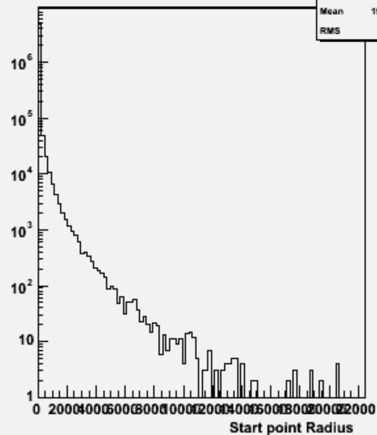
Start point R : w100476 n1n1uu_o
