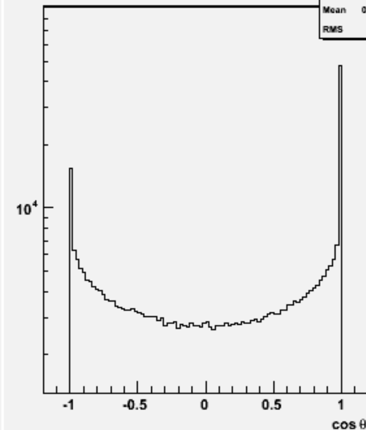
Jet cos \theta (All jets)w100476 n1n1uu_o
