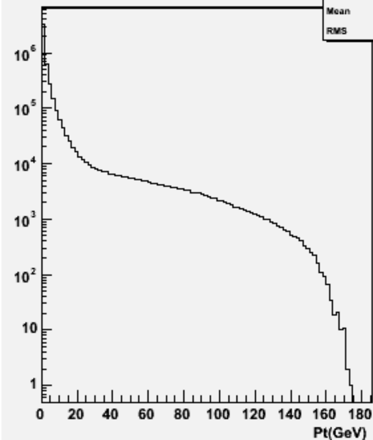
Particle Pt : w100476 n1n1uu_o
