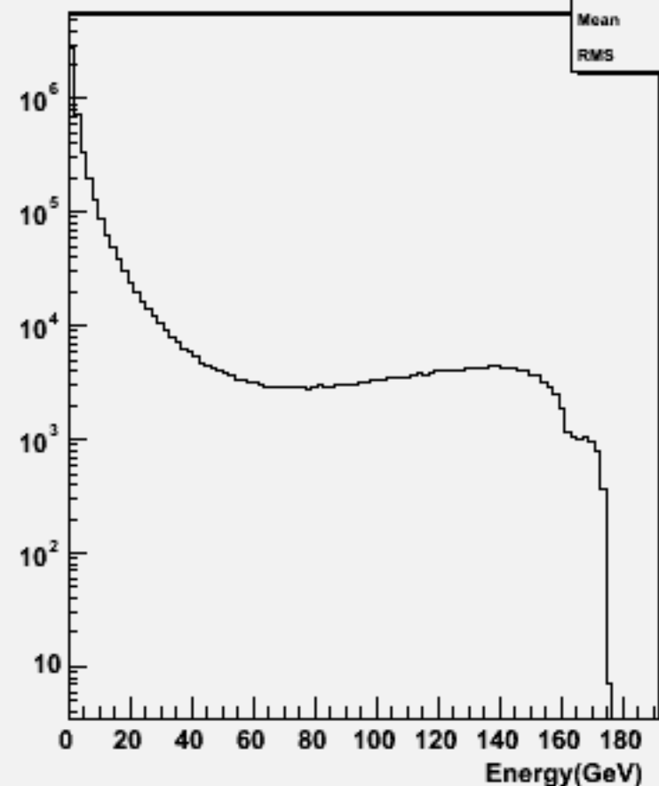
Particle Energy : w100476 n1n1uu_o
