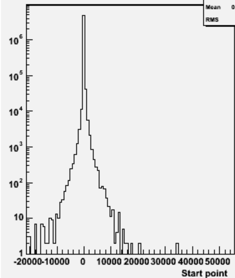
Start point Z : w100476 n1n1uu_o
