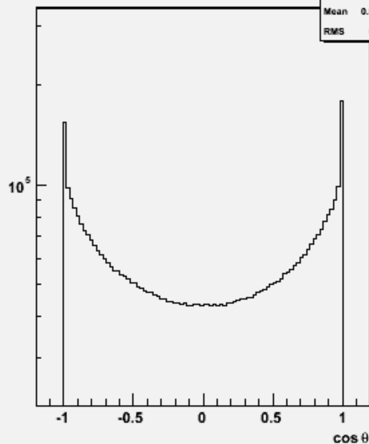
Particle cosθ : w100476 n1n1uu_o
