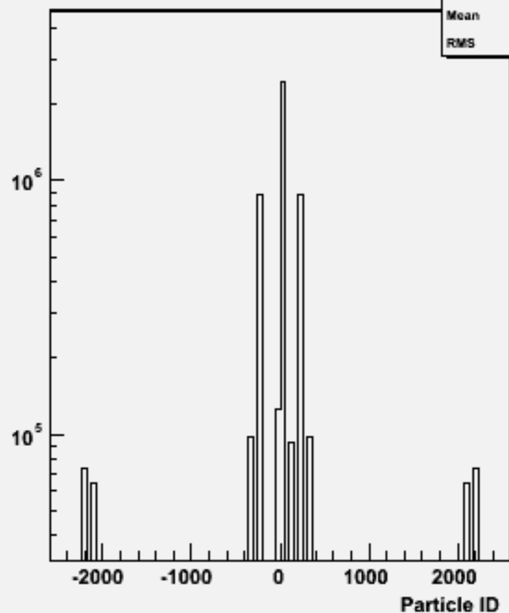
Particle ID : w100476 n1n1uu_o
