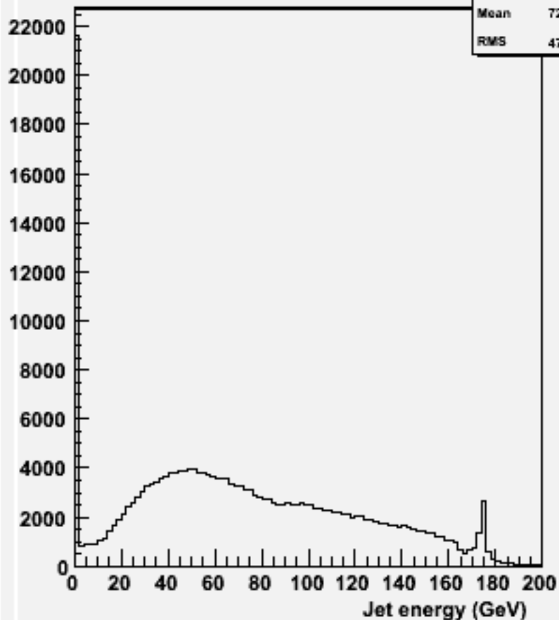
energy for 2-jets :w100476 n1n1uu_o
