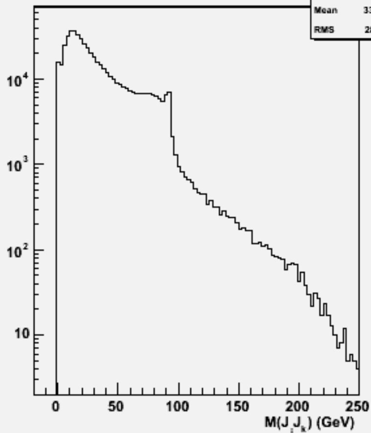
2jets mass(All comb)w100476 n1n1uu_o
