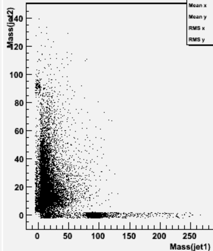
Jet mass for forced 2-jets : w100476 n1n1uu_o
