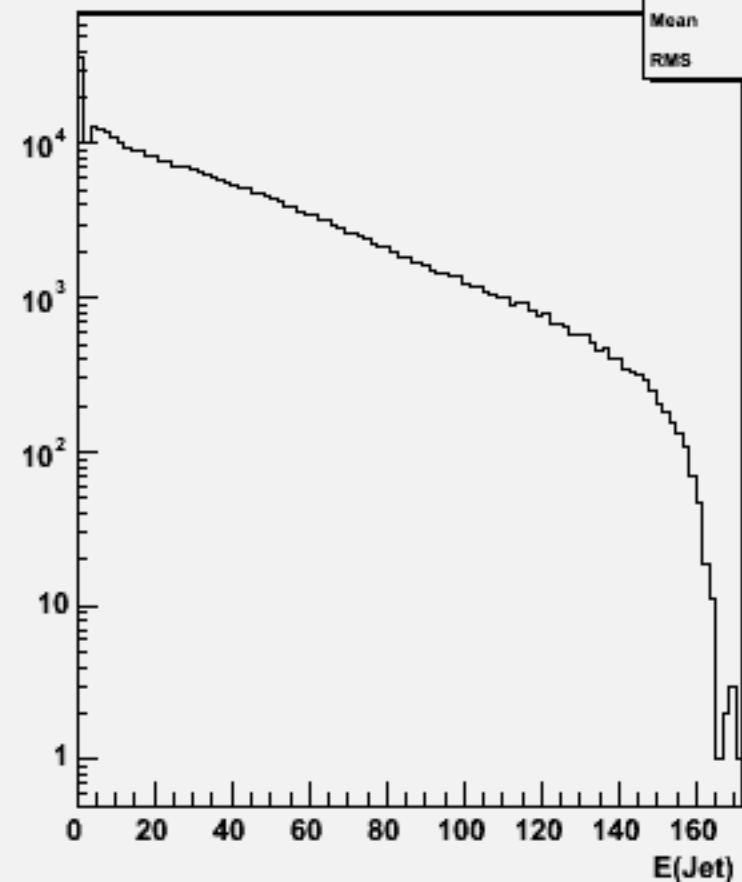
Jet energies(All jets)w100476 n1n1uu_o
