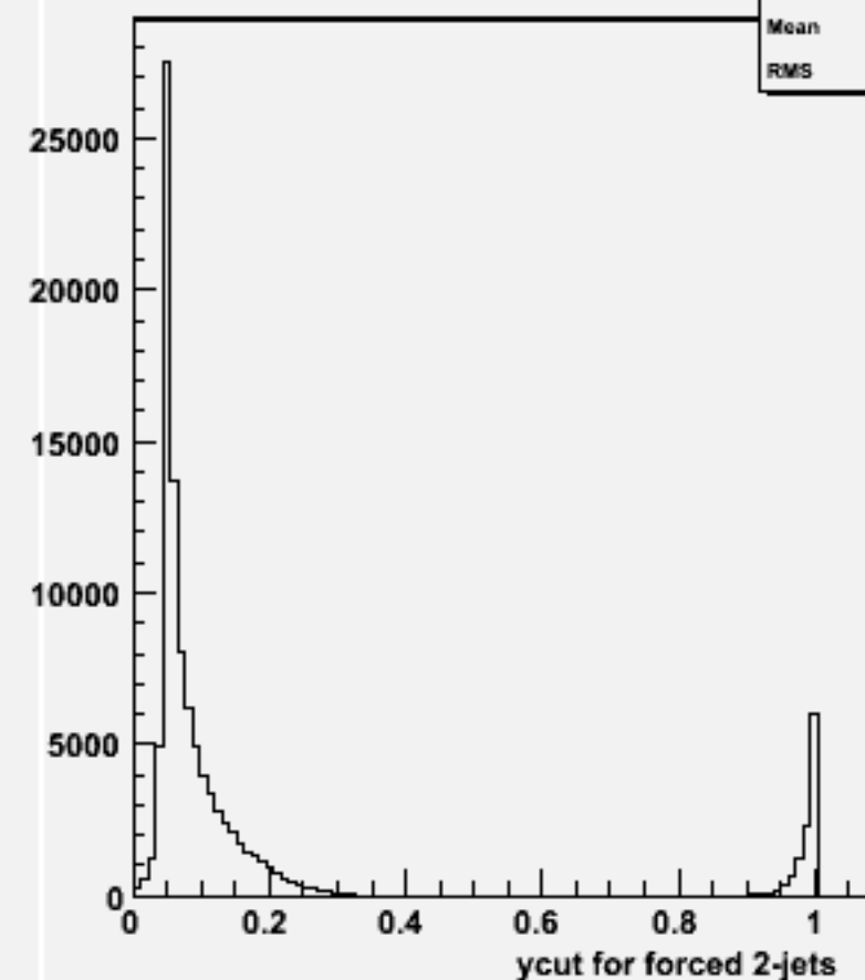
Ycut for 2-jets :w100468 csdu_o
