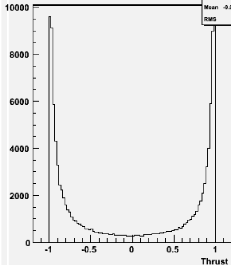
cos \Theta (thrust) w100468 csdu_o
