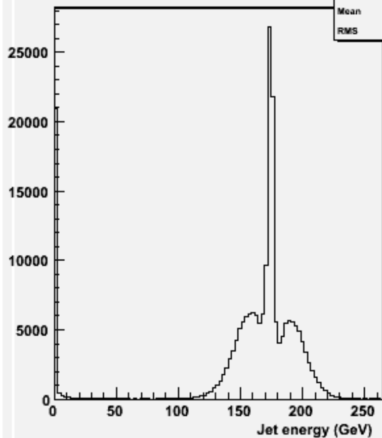
energy for 2-jets :w100468 csdu_o
