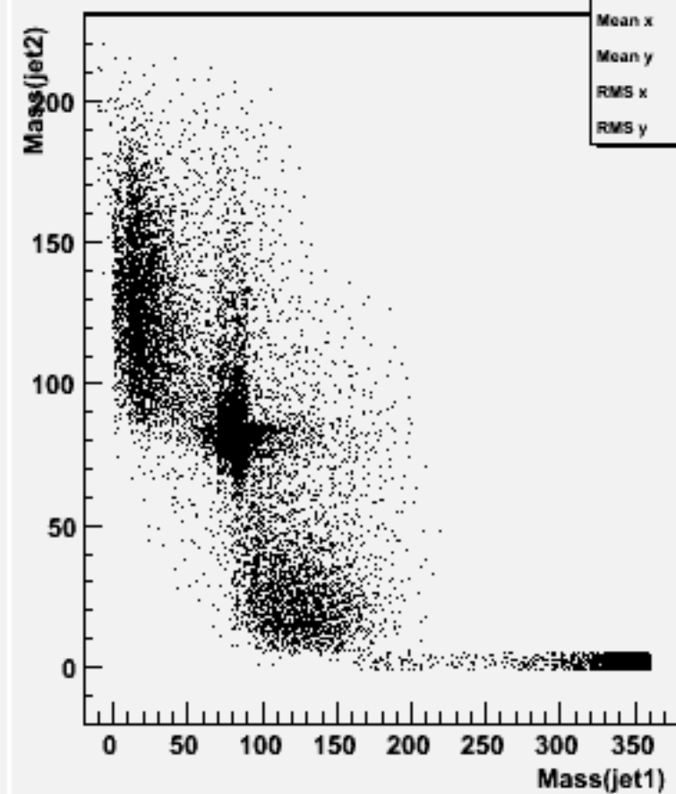
Jet mass for forced 2-jets : w100468 csdu_o
