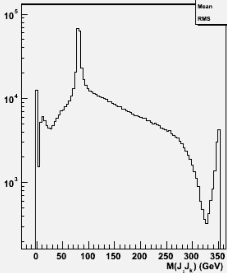
2jets mass(All comb)w100468 csdu_o
