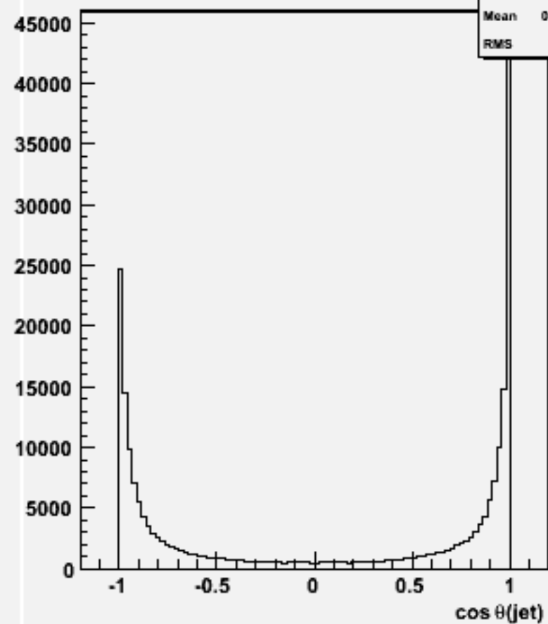
cos \theta for 2-jets :w100468 csdu_o
