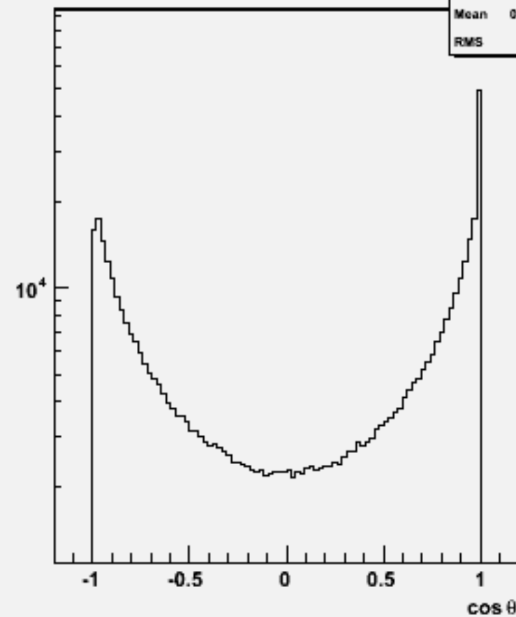
Jet cos \theta (All jets)w100468 csdu_o
