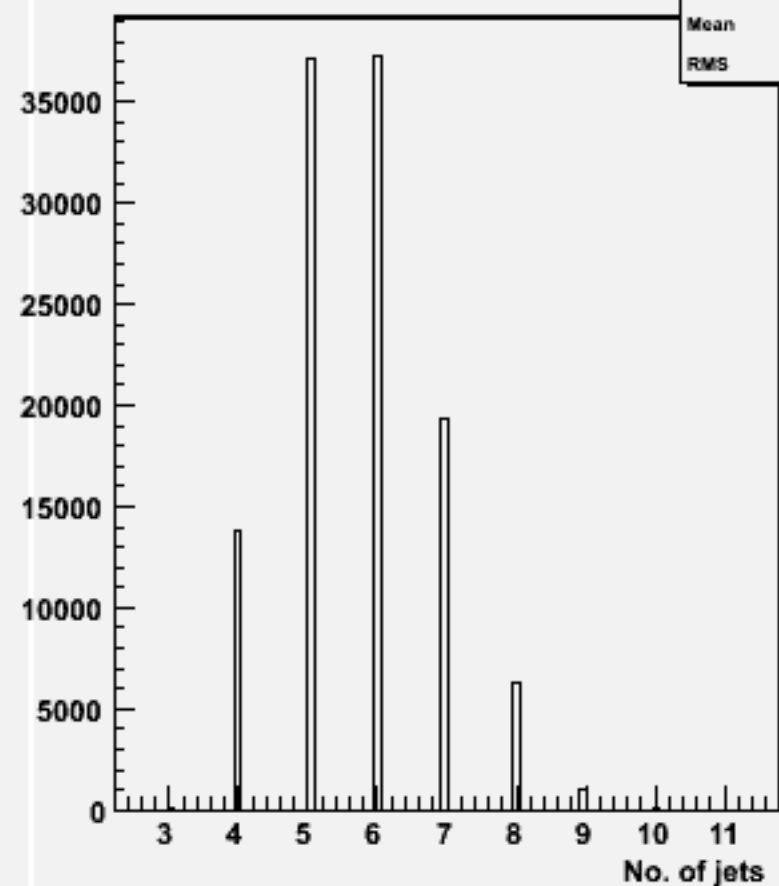
No. jets (ycut=0.001) : w100468 csdu_o
