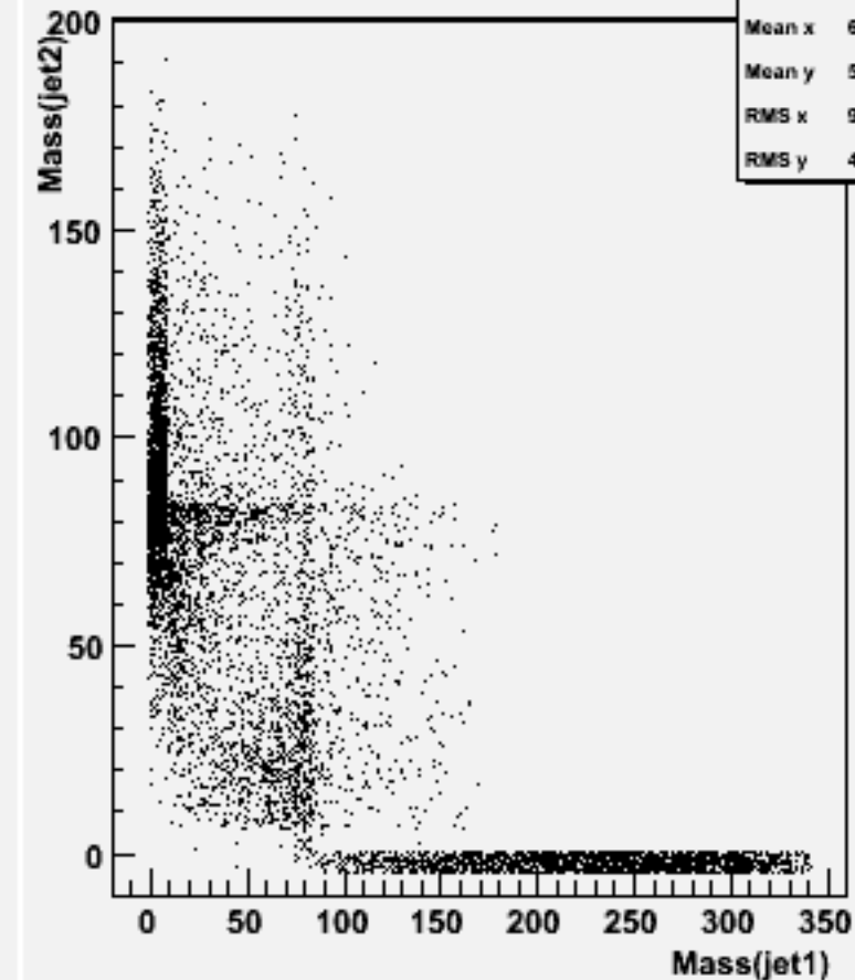
Jet mass for forced 2-jets : w100457 cse1n1_o
