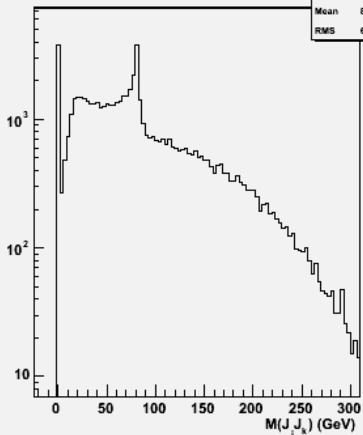
2jets mass(All comb)w100457 cse1n1_o
