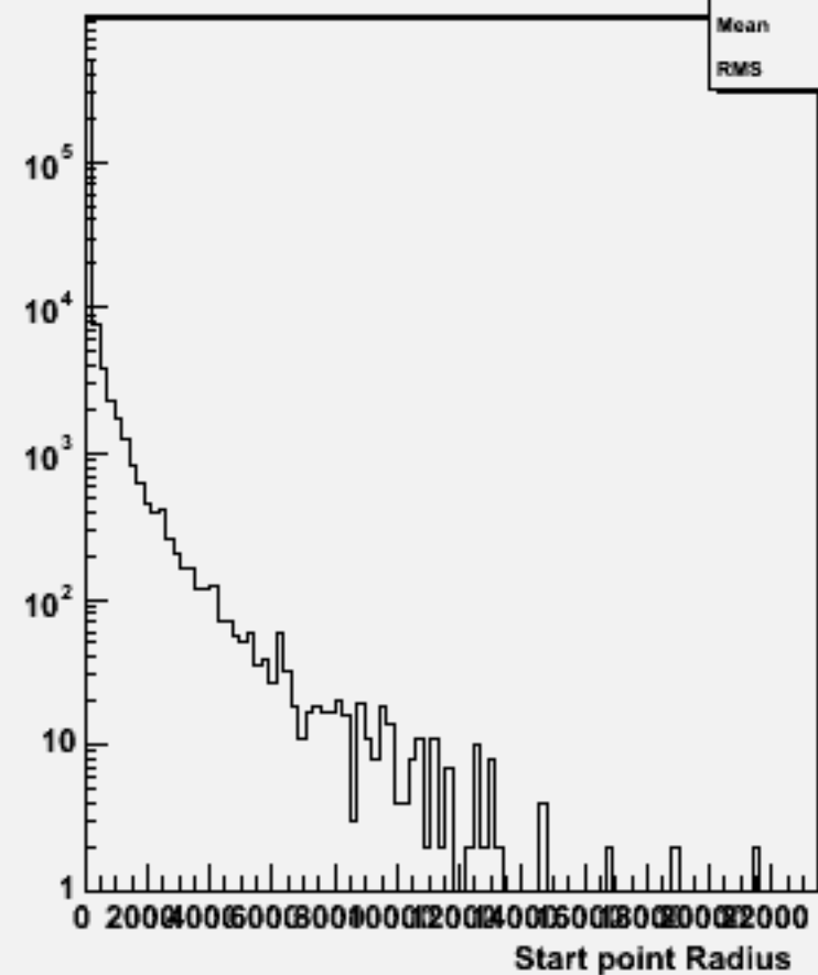
Start point R : w100457 cse1n1_o
