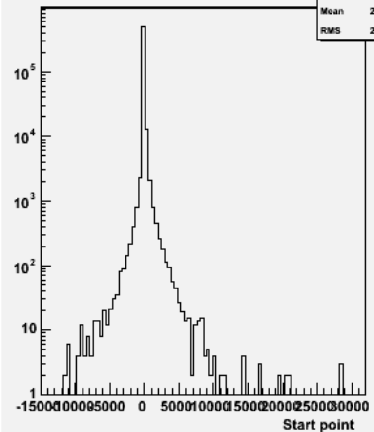
Start point Z : w100457 cse1n1_o
