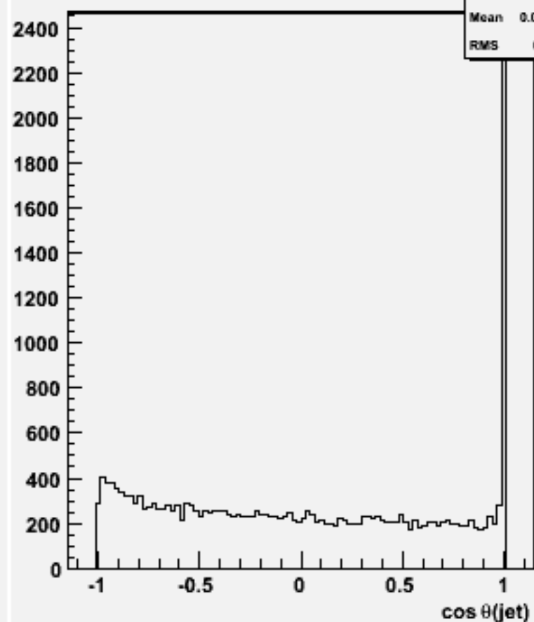
cos \theta for 2-jets :w100457 cse1n1_o
