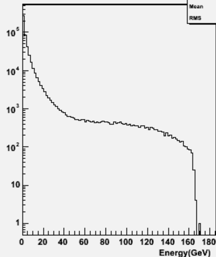
Particle Energy : w100457 cse1n1_o
