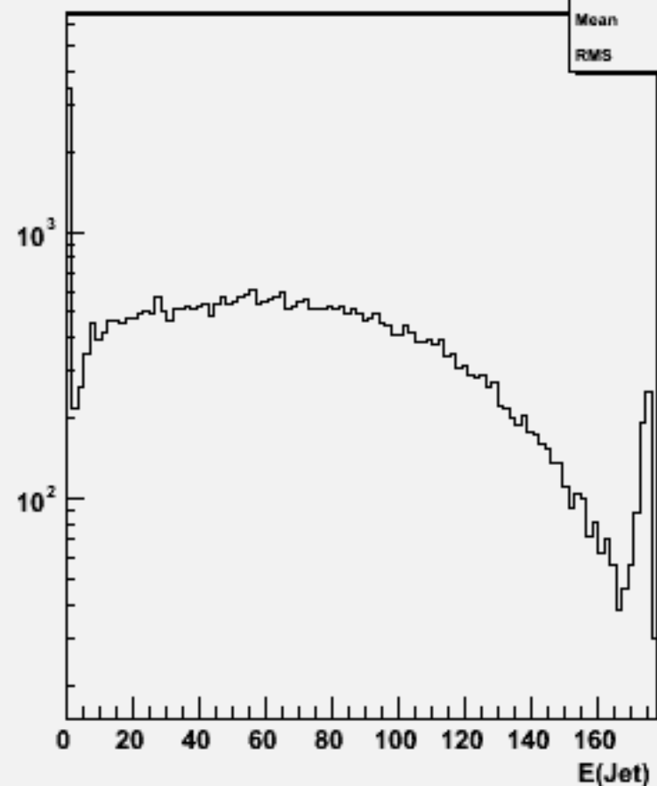
Jet energies(All jets)w100457 cse1n1_o
