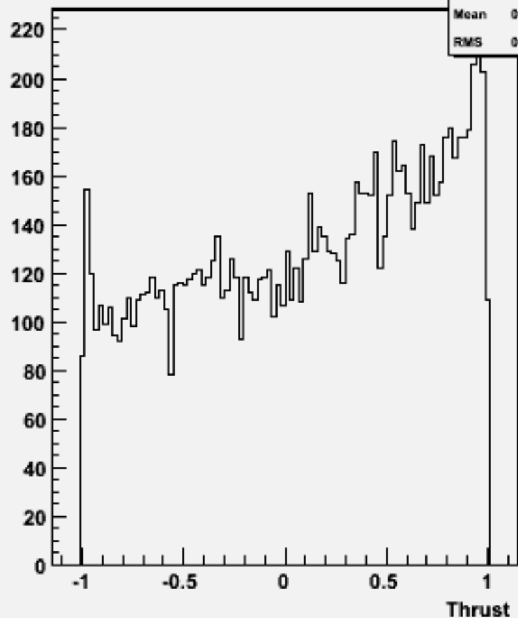
cos \Theta (thrust) w100457 cse1n1_o
