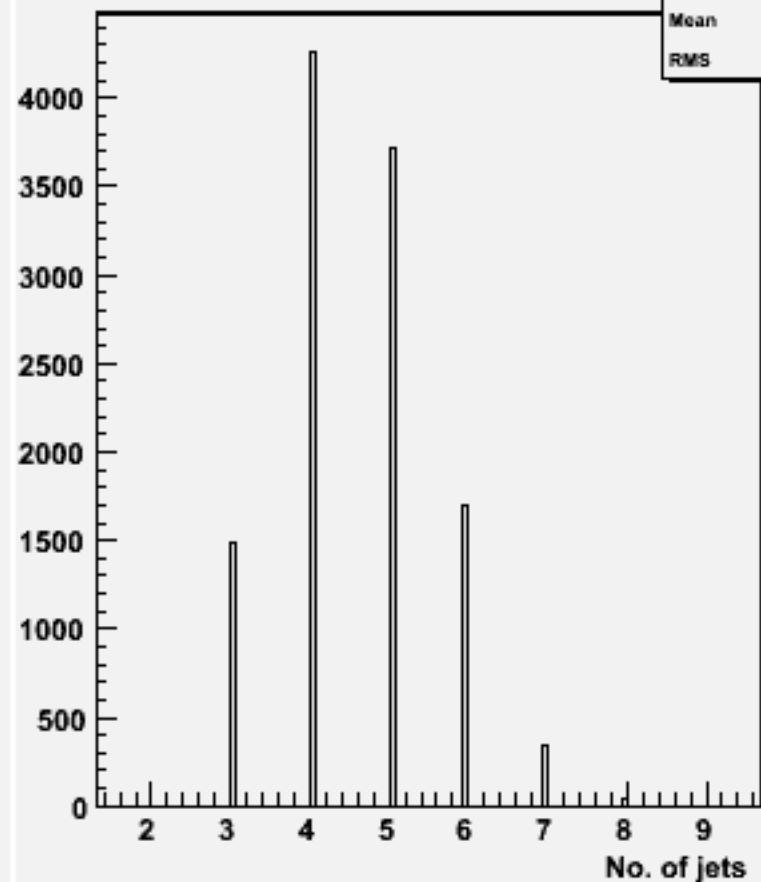
No. jets (ycut=0.001) : w100457 cse1n1_o
