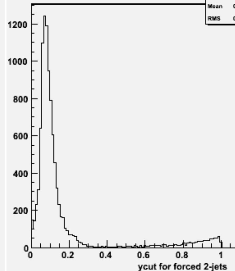
Ycut for 2-jets :w100457 cse1n1_o
