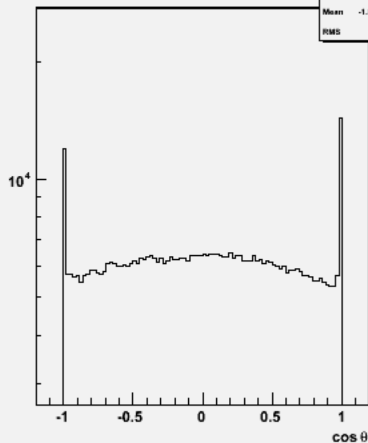
Particle cosθ : w100457 cse1n1_o
