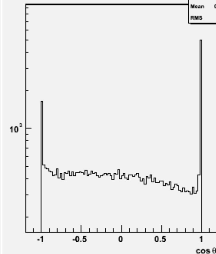
Jet cos \theta (All jets)w100457 cse1n1_o
