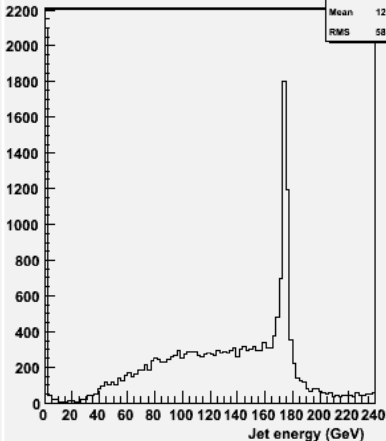
energy for 2-jets :w100457 cse1n1_o
