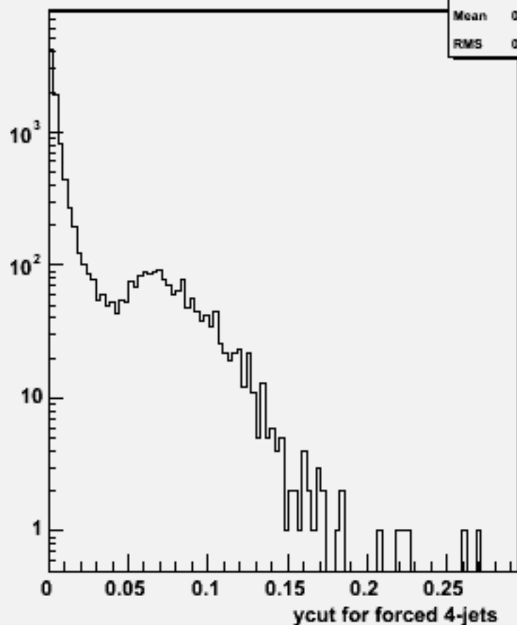
Ycut for 4-jets :w100457 cse1n1_o
