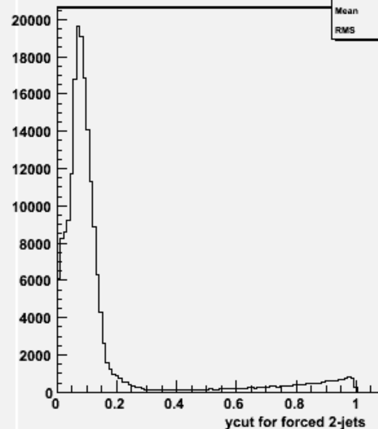
Ycut for 2-jets :w100444 ude3n3_o
