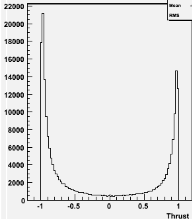
cos \Theta (thrust) w100444 ude3n3_o
