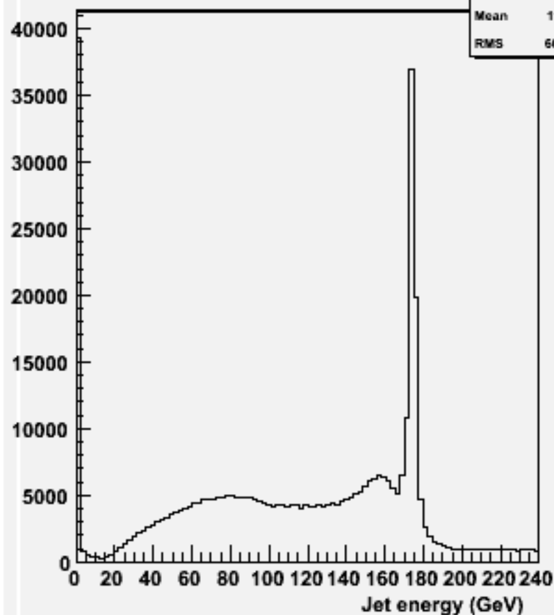
energy for 2-jets :w100444 ude3n3_o
