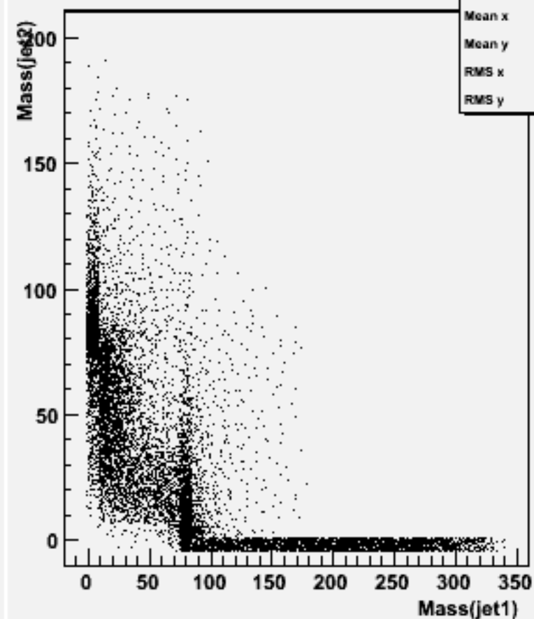
Jet mass for forced 2-jets : w100444 ude3n3_o
