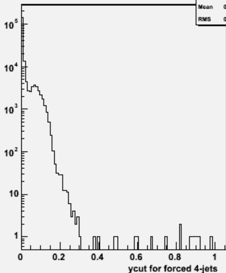
Ycut for 4-jets :w100444 ude3n3_o
