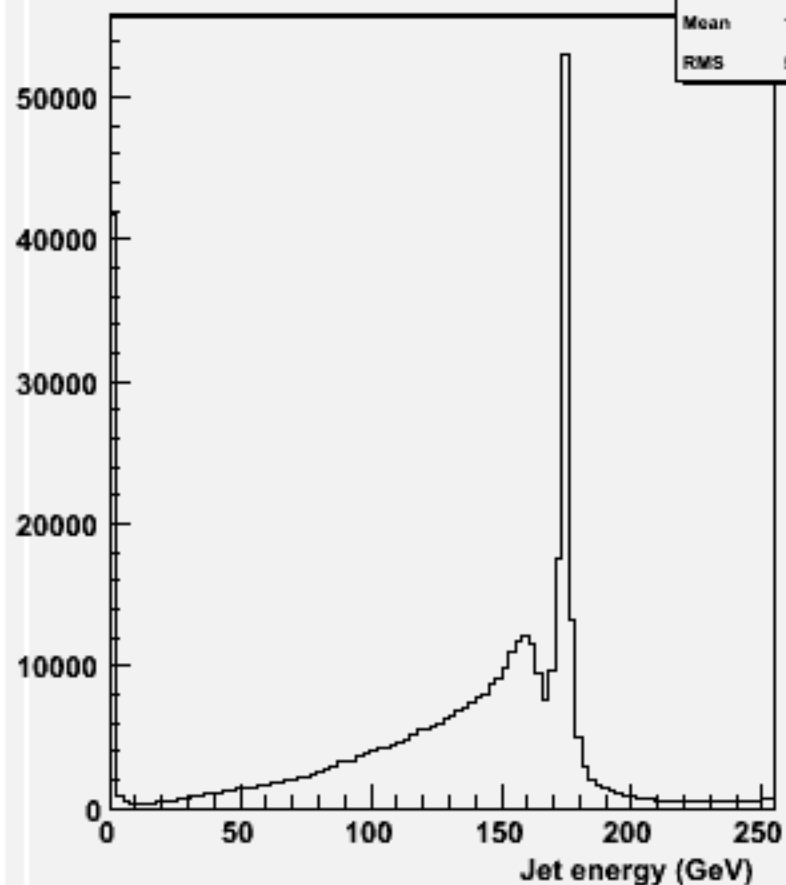
energy for 2-jets :w100436 ude1n1_o
