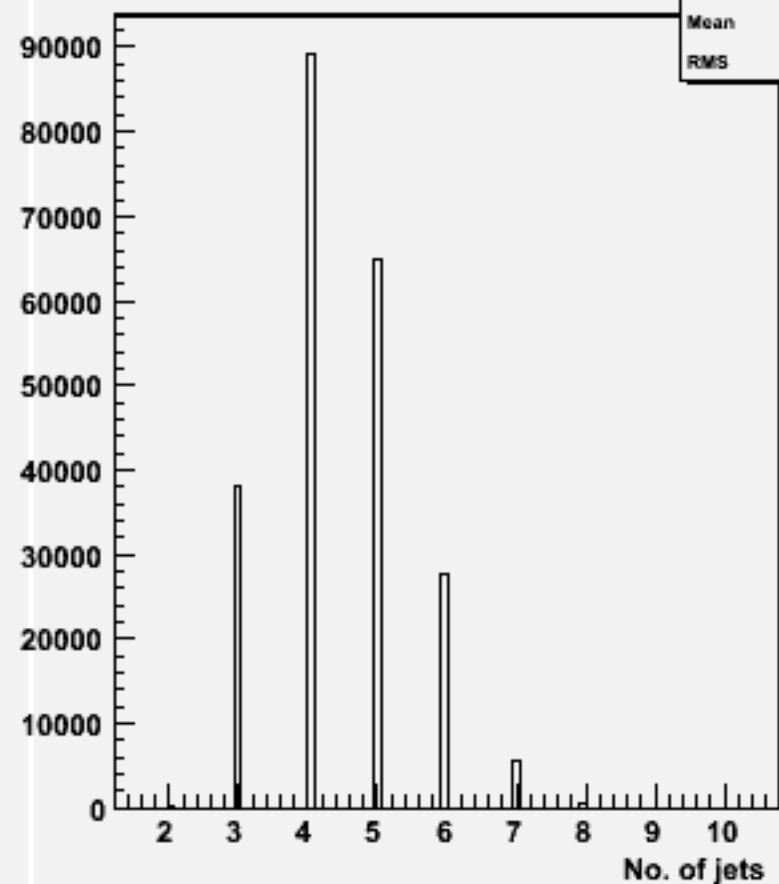
No. jets (ycut=0.001) : w100436 ude1n1_o
