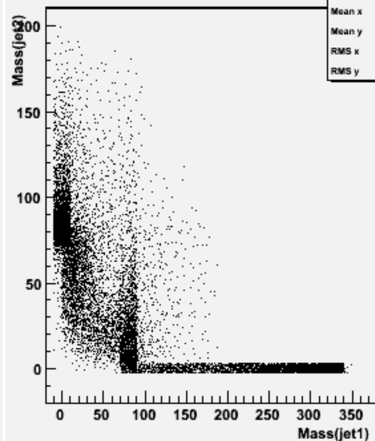
Jet mass for forced 2-jets : w100436 ude1n1_o
