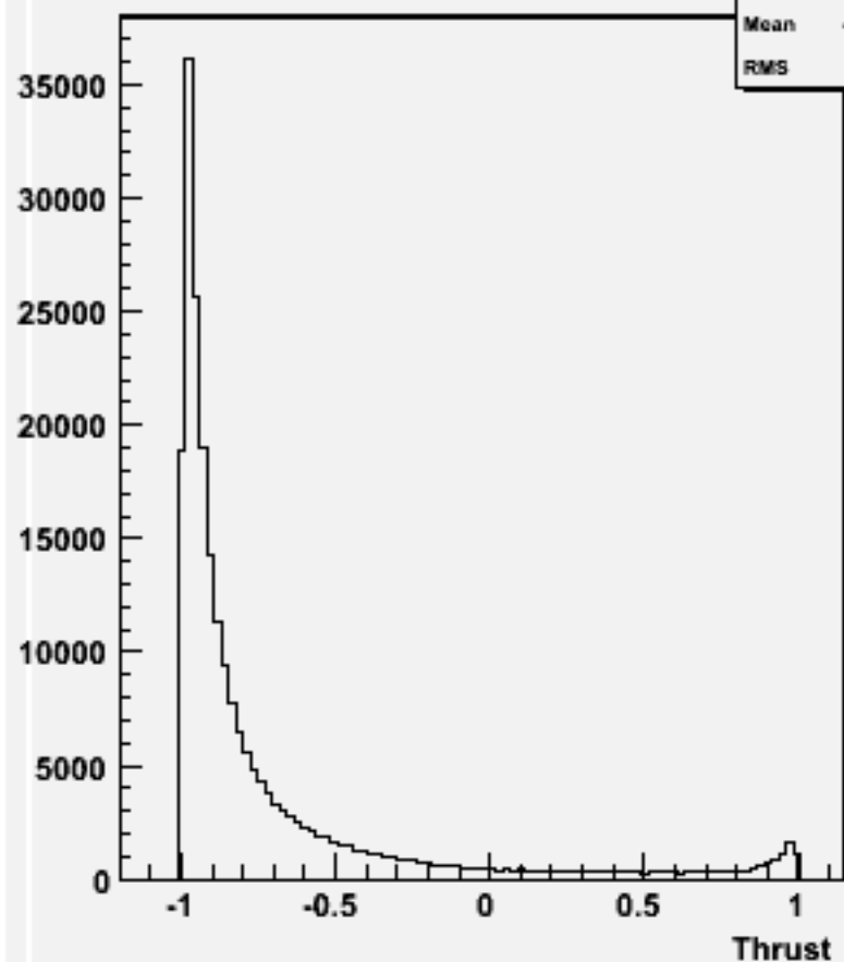
cos \Theta (thrust) w100436 ude1n1_o
