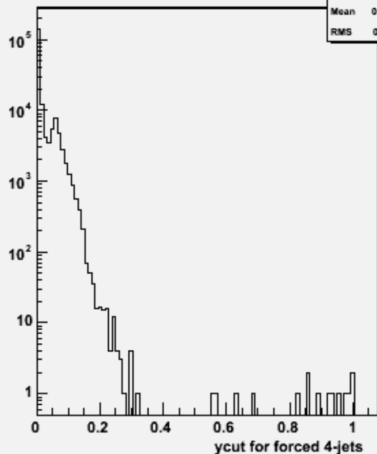
Ycut for 4-jets :w100436 ude1n1_o
