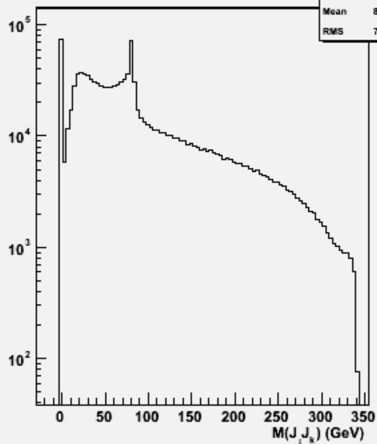
2jets mass(All comb)w100436 ude1n1_o
