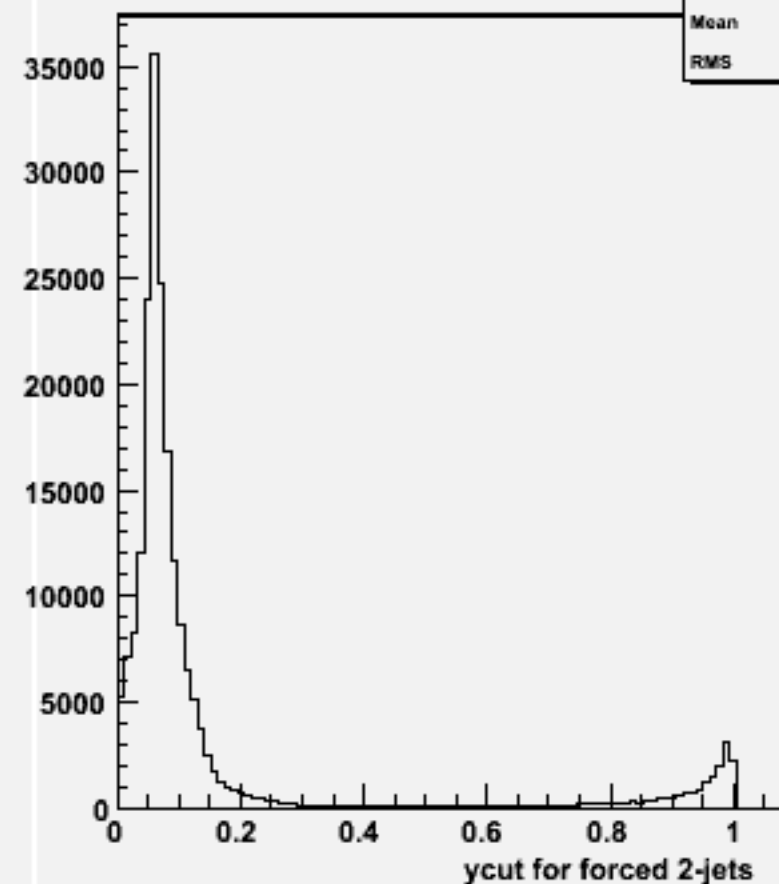
Ycut for 2-jets :w100436 ude1n1_o
