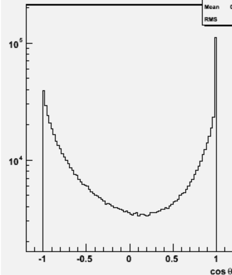
Jet cos \theta (All jets)w100436 ude1n1_o
