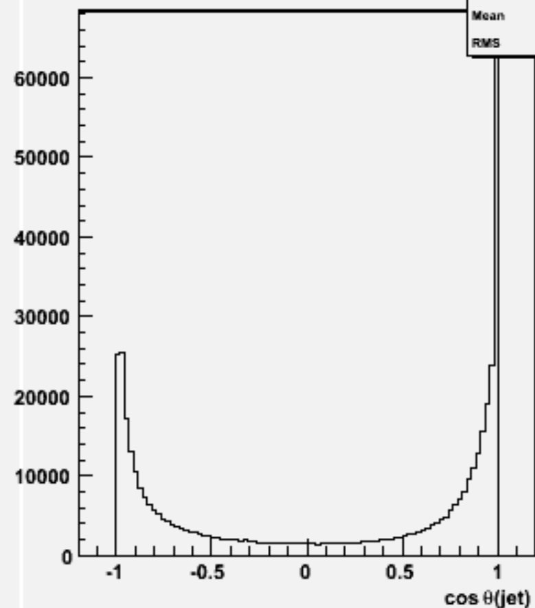
cos \theta for 2-jets :w100436 ude1n1_o
