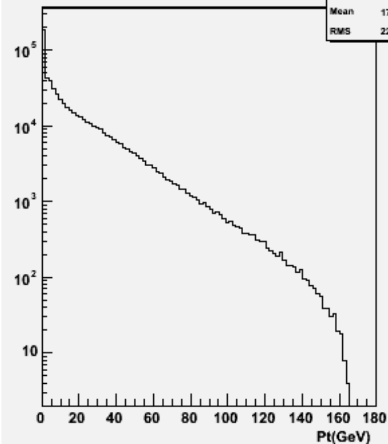
Particle Pt : w100418 n3e3e1n1_o
