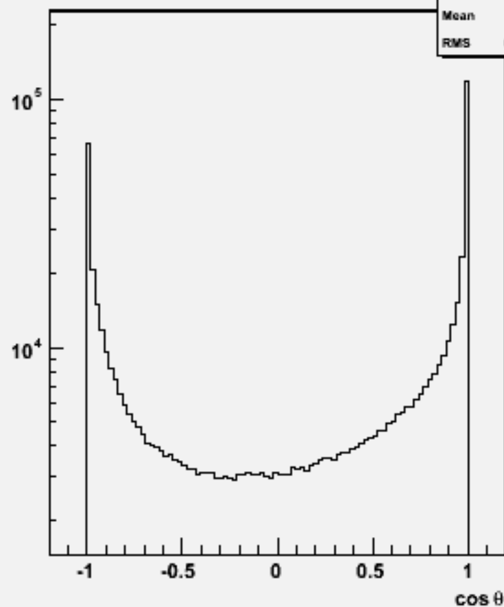
Particle cos \theta : w100418 n3e3e1n1_o
