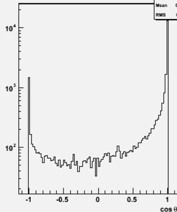
Jet cos \theta (All jets)w100418 n3e3e1n1_o
