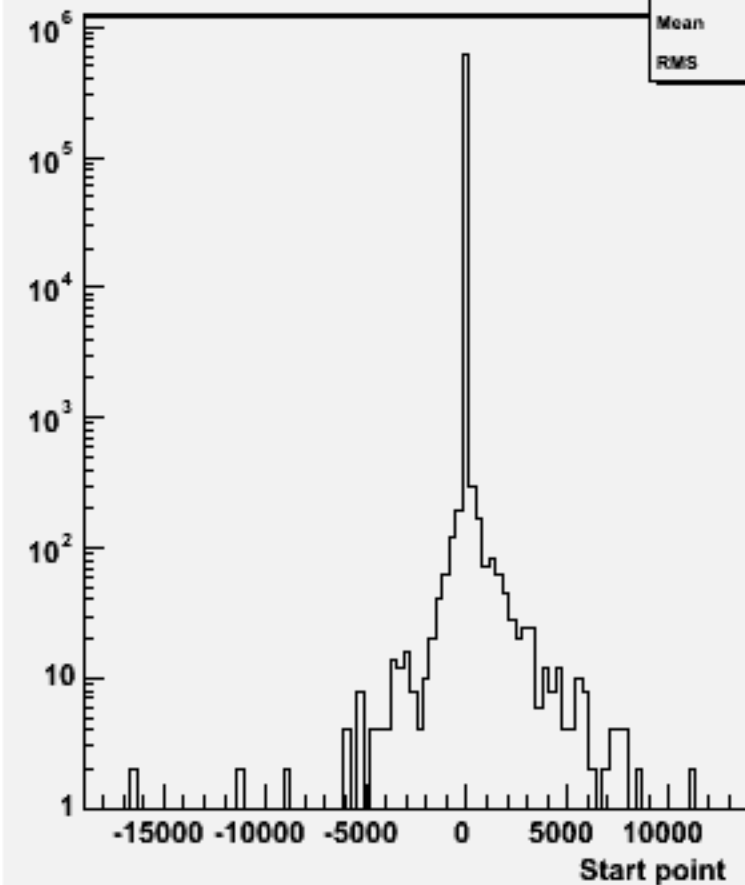
Start point Z : w100418 n3e3e1n1_o
