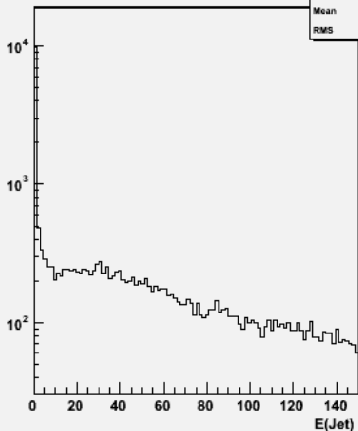
Jet energies(All jets)w100418 n3e3e1n1_o
