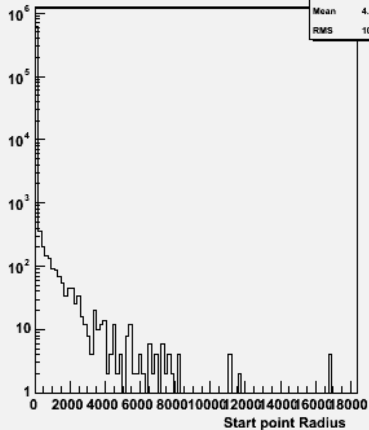
Start point R : w100418 n3e3e1n1_o
