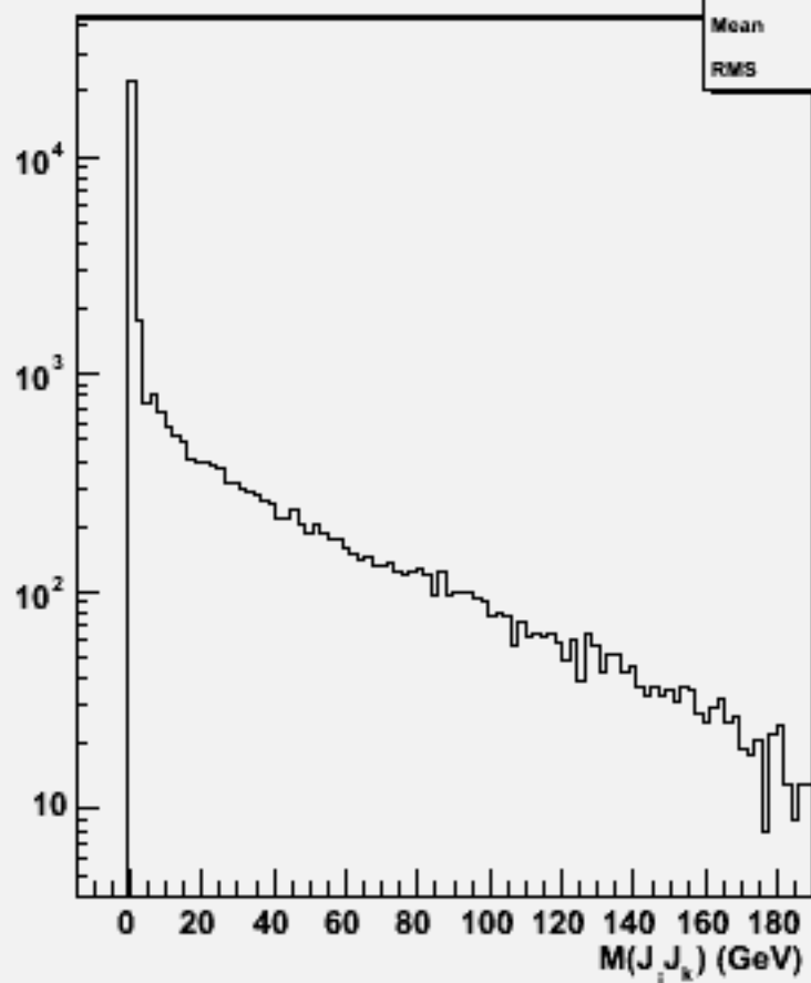
2jets mass(All comb)w100418 n3e3e1n1_o
