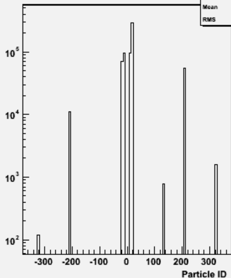
Particle ID : w100418 n3e3e1n1_o
