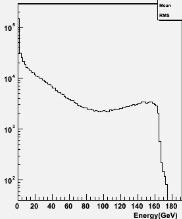
Particle Energy : w100418 n3e3e1n1_o
