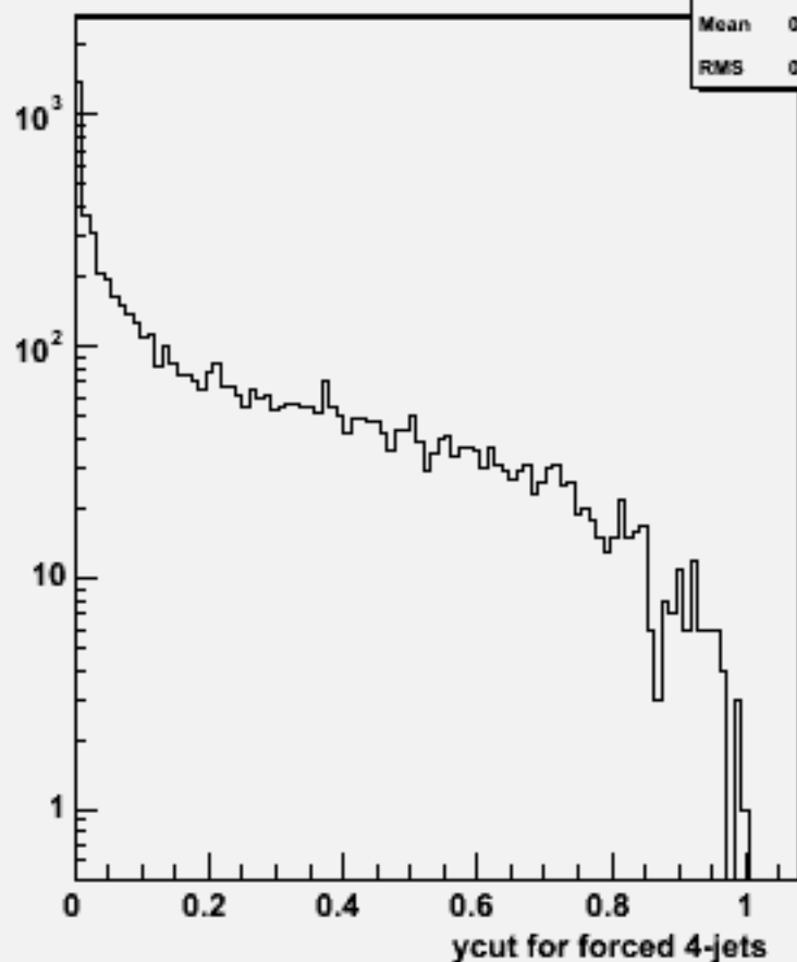
Ycut for 4-jets :w100418 n3e3e1n1_o
