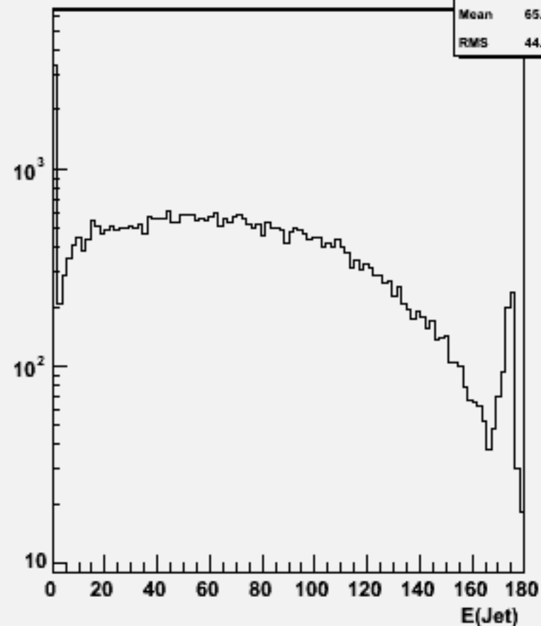
Jet energies(All jets)w100413 n2e2sc_o
