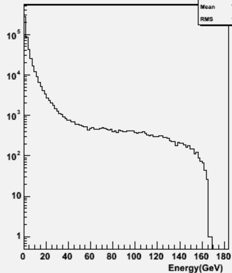
Start point R : w100413 n2e2sc_o
