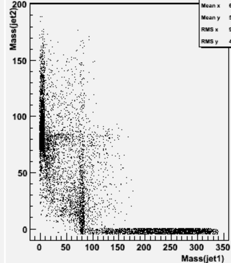
Jet mass for forced 2-jets : w100413 n2e2sc_o
