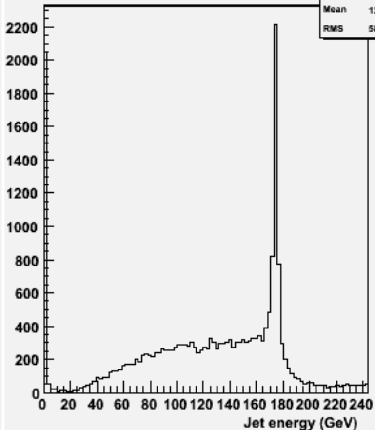
energy for 2-jets :w100413 n2e2sc_o
