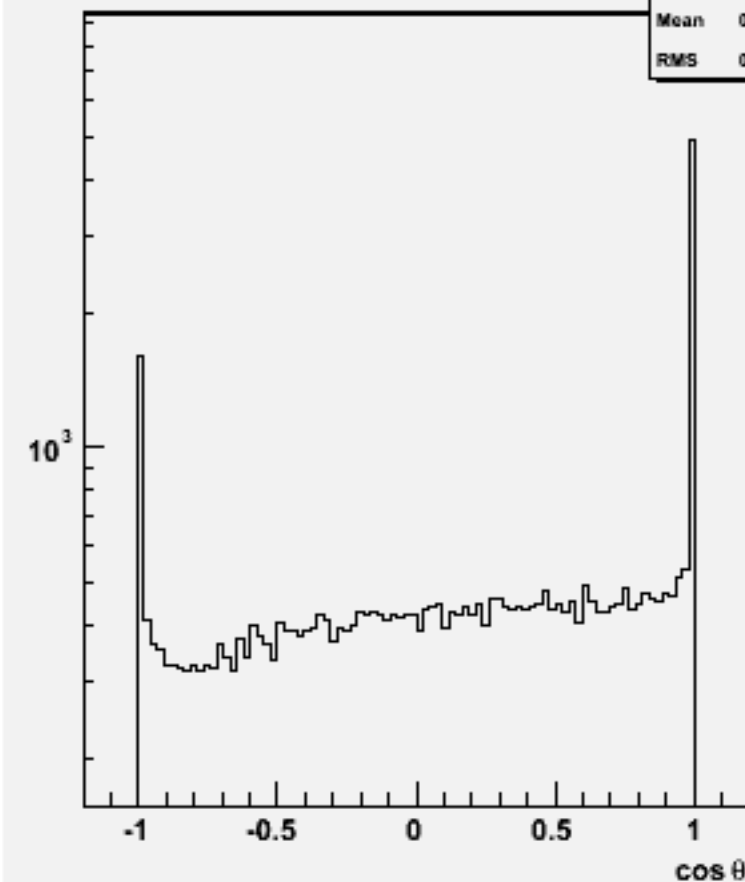
Jet cos \theta (All jets)w100413 n2e2sc_o
