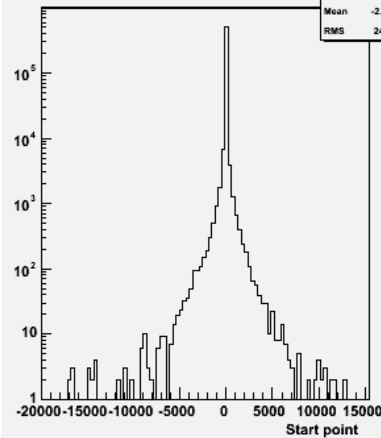
Start point Z : w100413 n2e2sc_o
