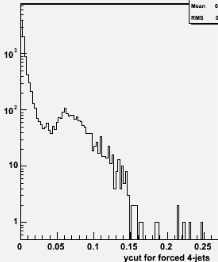
Ycut for 4-jets :w100413 n2e2sc_o
