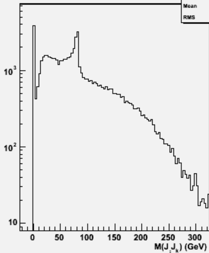
2jets mass(All comb)w100413 n2e2sc_o
