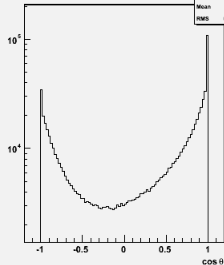
Jet cos \theta (All jets)w100408 n2e2du_o
