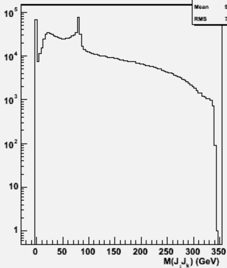
2jets mass(All comb)w100408 n2e2du_o
