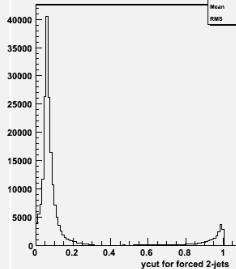
Ycut for 2-jets :w100408 n2e2du_o
