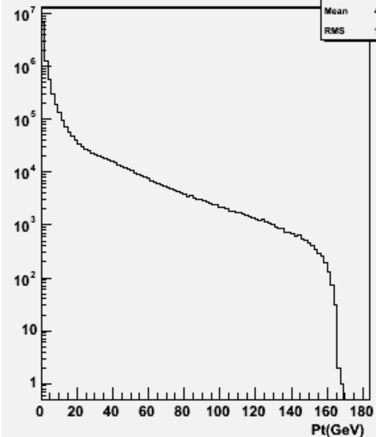
Particle Pt : w100408 n2e2du_o
