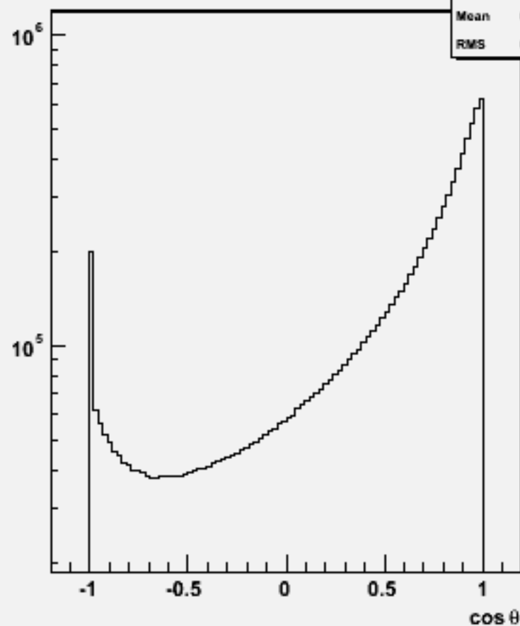
Particle cosθ : w100408 n2e2du_o
