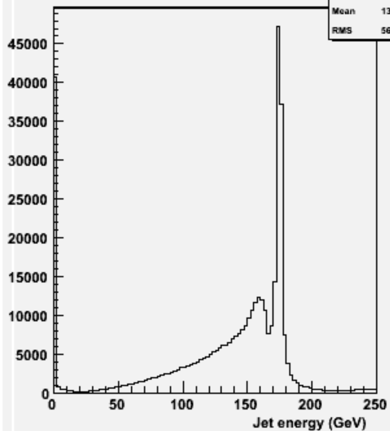
energy for 2-jets :w100408 n2e2du_o
