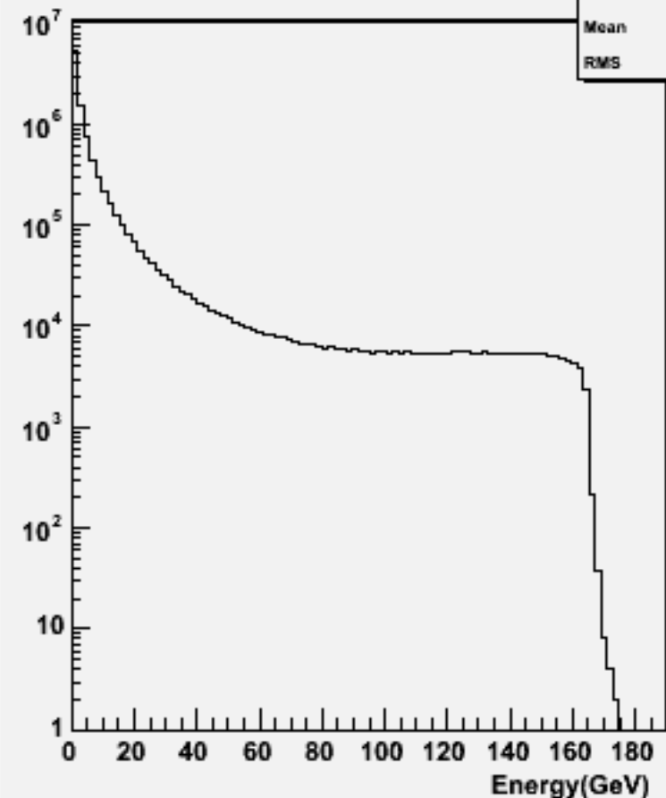
Particle Energy : w100408 n2e2du_o
