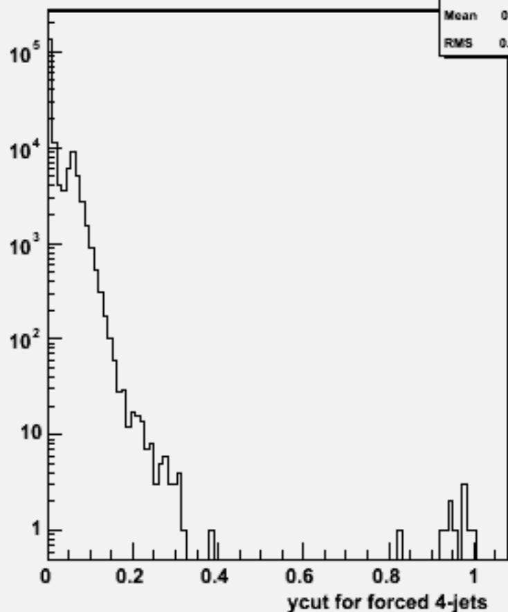
Ycut for 4-jets :w100408 n2e2du_o
