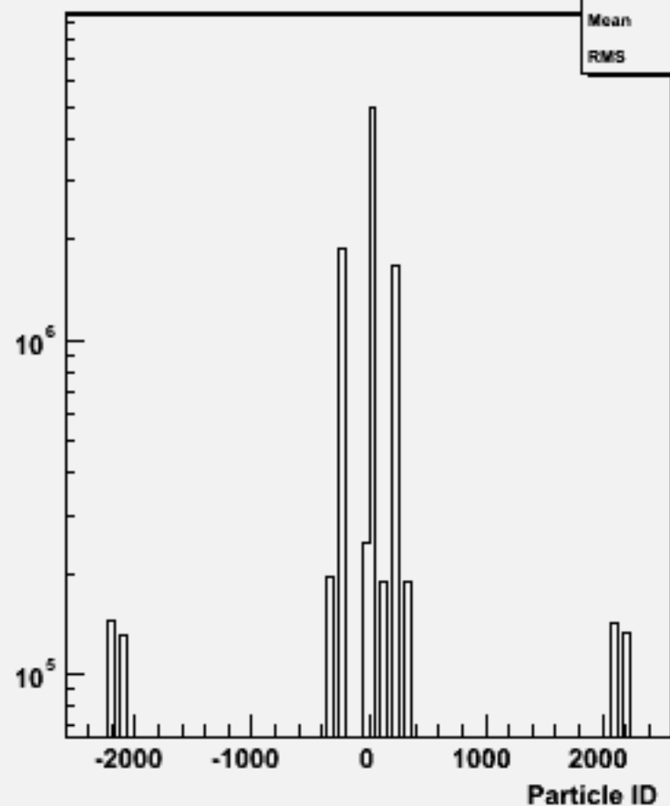
Particle ID : w100408 n2e2du_o
