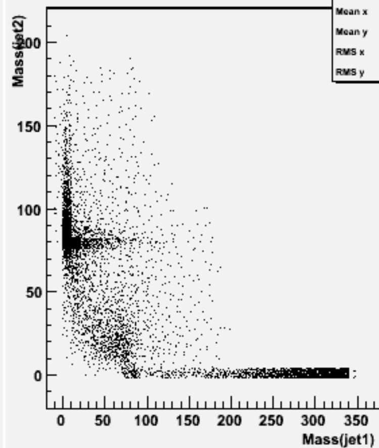
Jet mass for forced 2-jets : w100408 n2e2du_o
