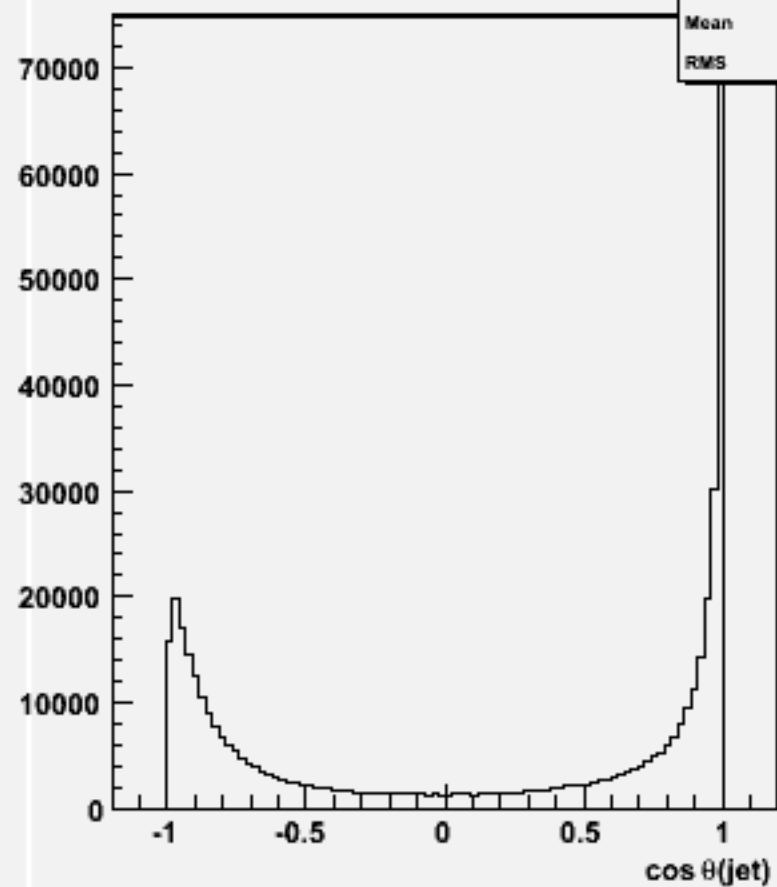
cos \theta for 2-jets :w100408 n2e2du_o
