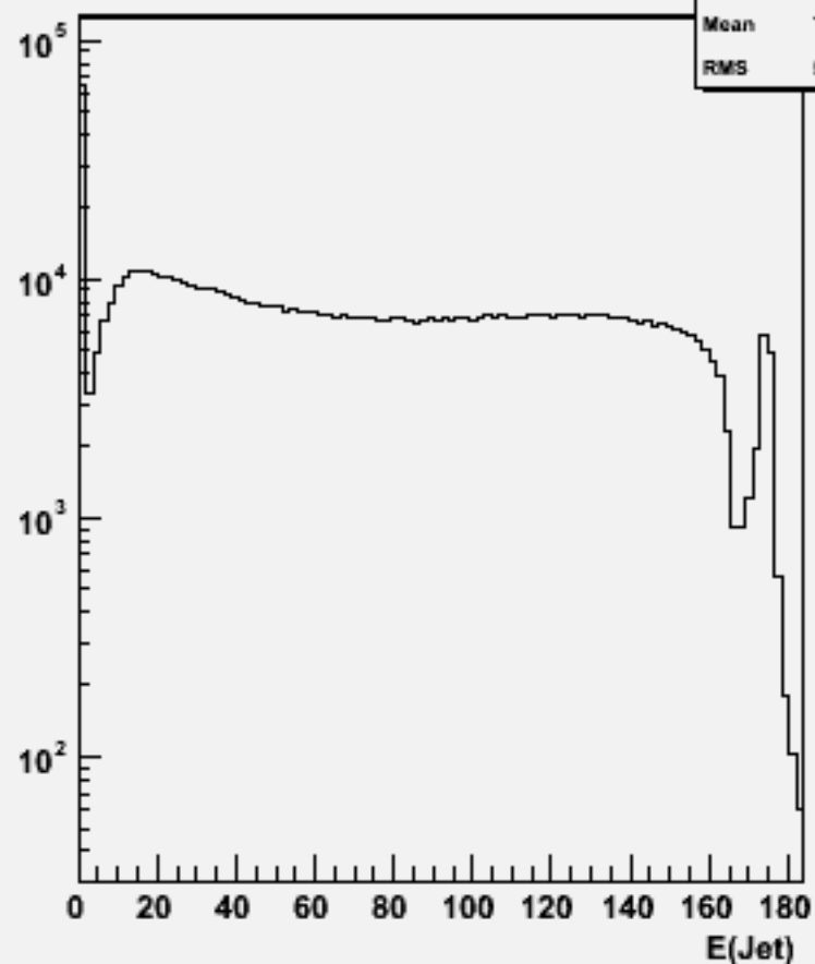
Jet energies(All jets)w100408 n2e2du_o
