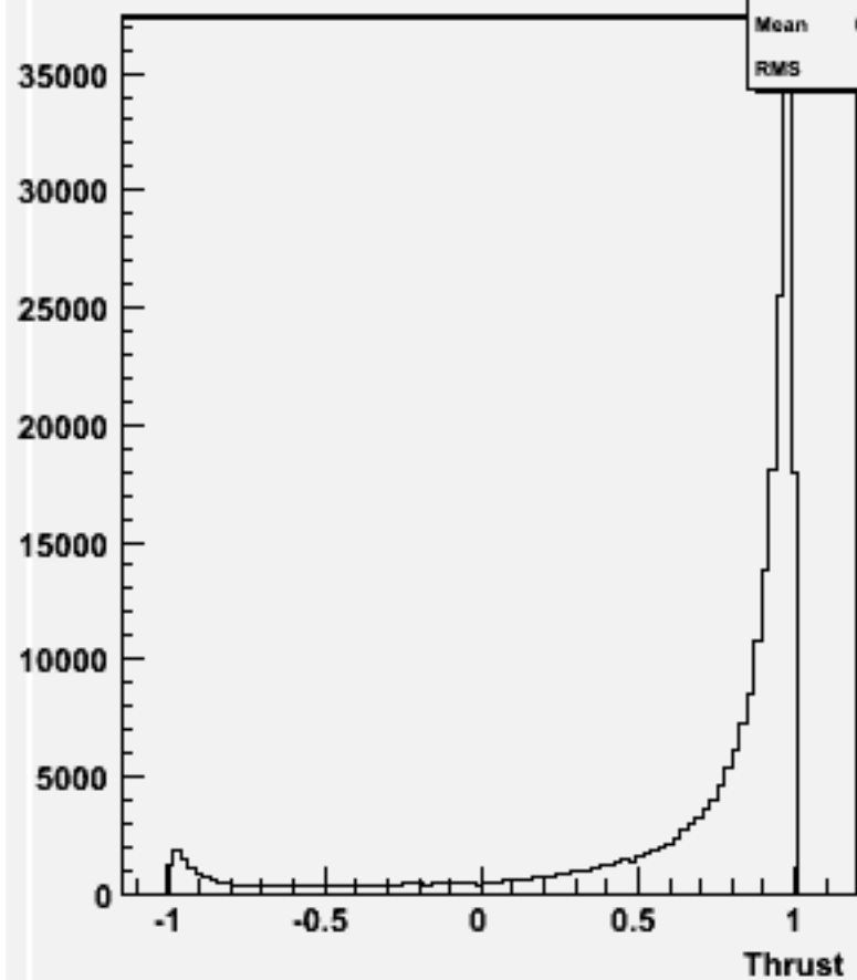
cos \Theta (thrust) w100408 n2e2du_o
