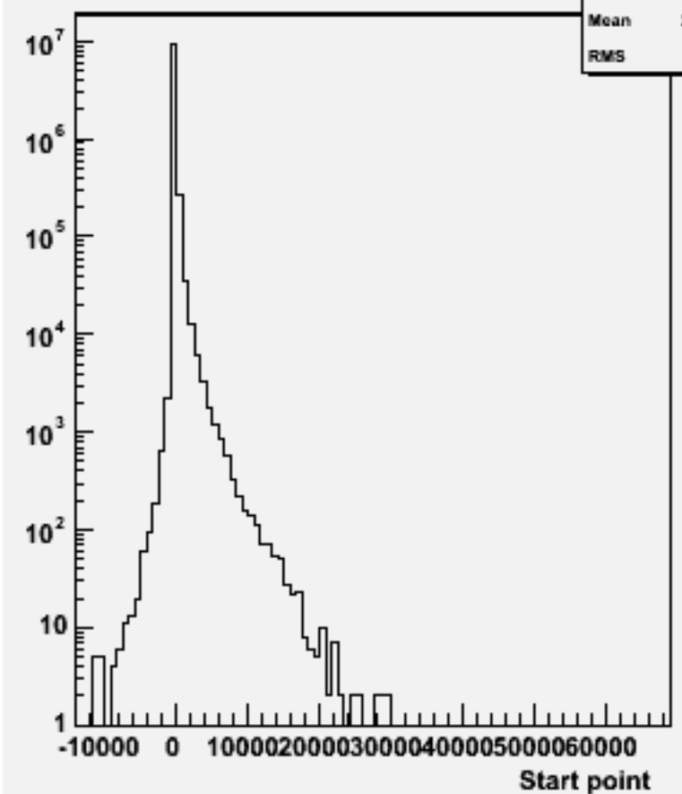
Start point Z : w100408 n2e2du_o
