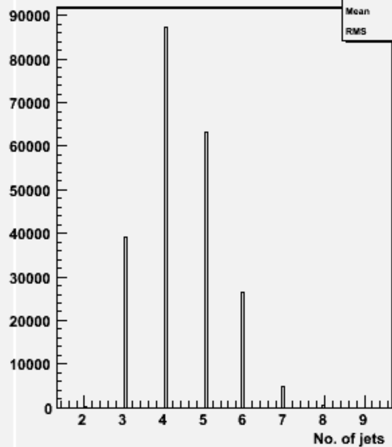
No. jets (ycut=0.001) : w100408 n2e2du_o
