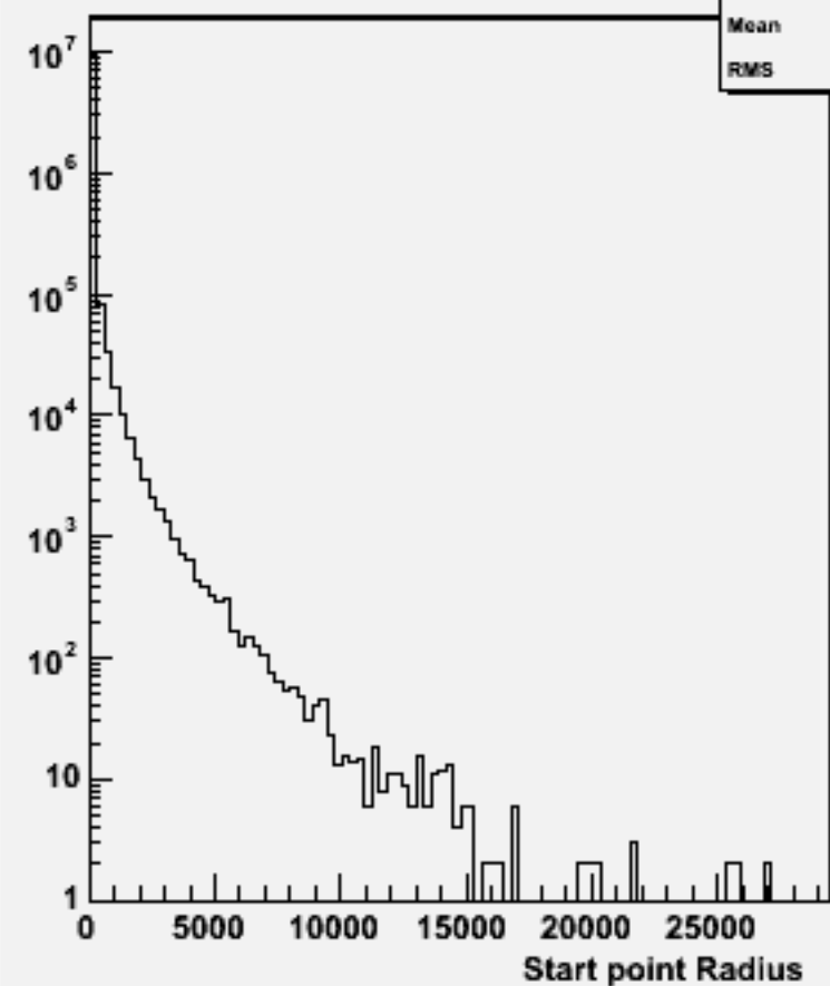
Start point R : w100408 n2e2du_o
