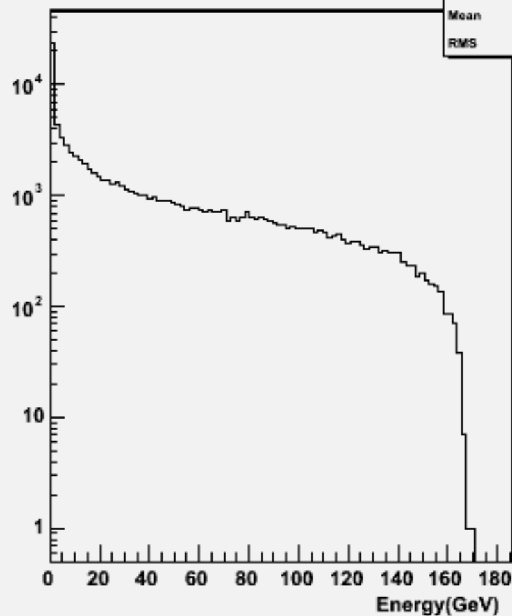
Particle Energy : w100405 n2e2e3n3_o
