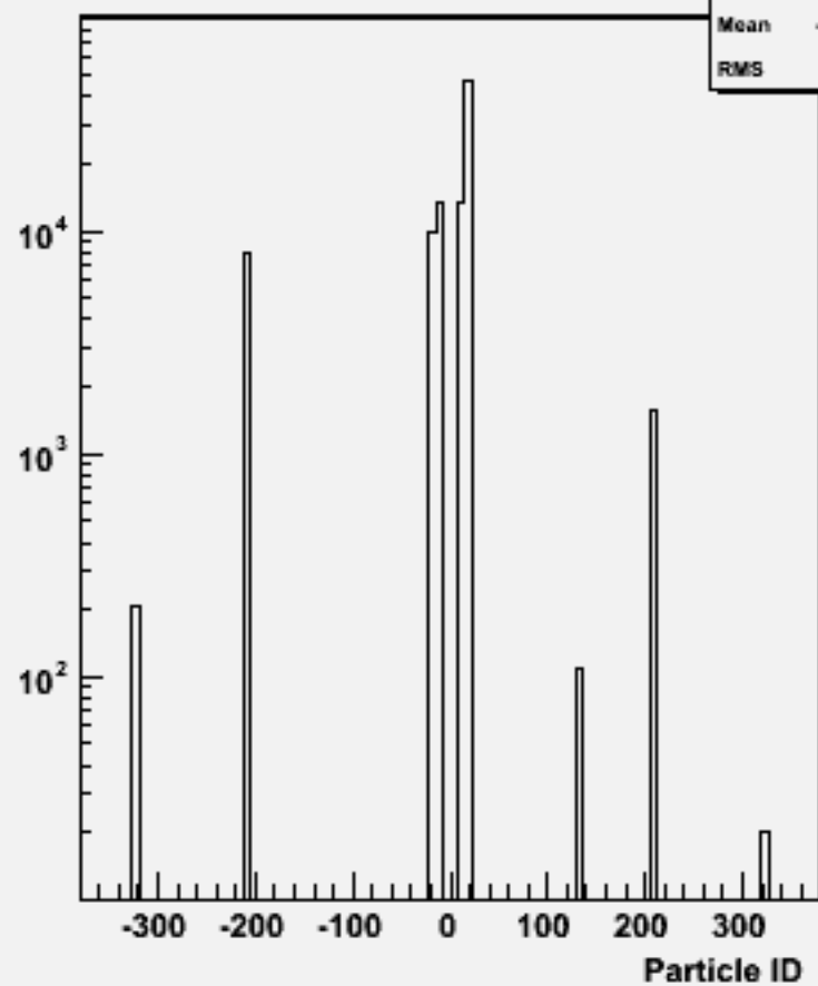
Particle ID : w100405 n2e2e3n3_o
