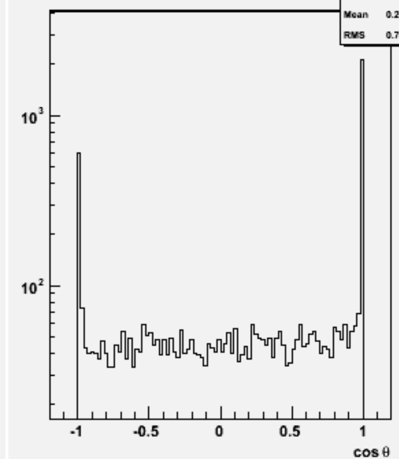
Jet cos \theta (All jets)w100405 n2e2e3n3_o
