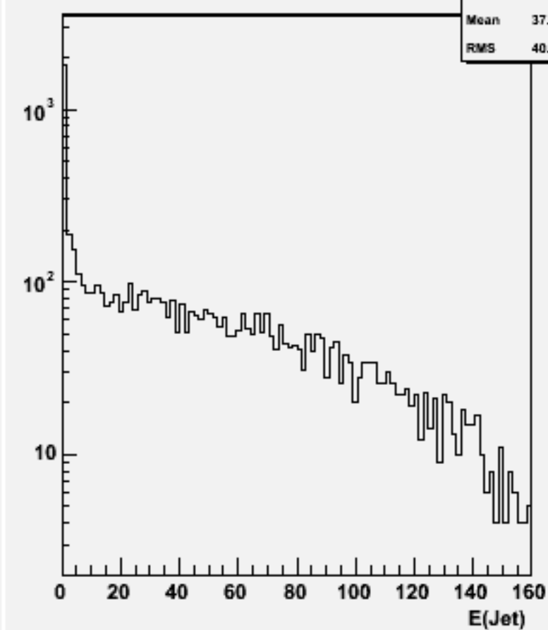
Jet energies(All jets)w100405 n2e2e3n3_o
