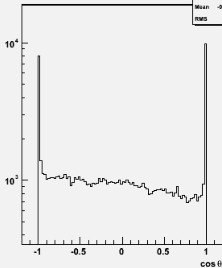
Particle cos \theta : w100405 n2e2e3n3_o
