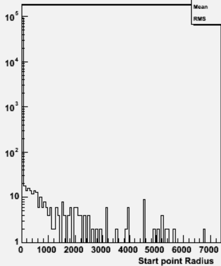
Start point R : w100405 n2e2e3n3_o
