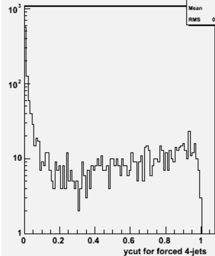
Ycut for 4-jets :w100405 n2e2e3n3_o
