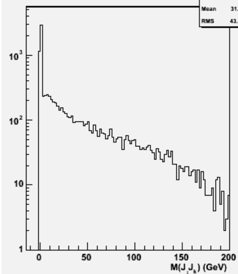
2jets mass(All comb)w100405 n2e2e3n3_o
