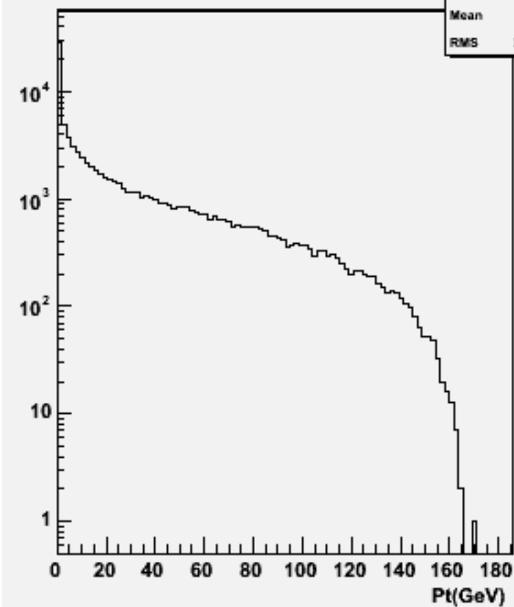
Particle Pt : w100405 n2e2e3n3_o
