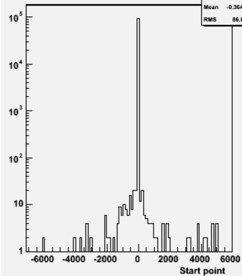
Start point Z : w100405 n2e2e3n3_o
