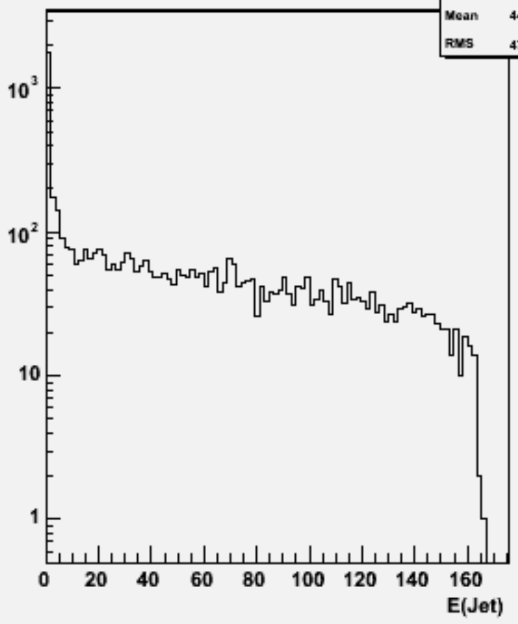
Jet energies(All jets)w100401 n2e2e2n2_o
