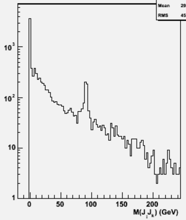
2jets mass(All comb)w100401 n2e2e2n2_o
