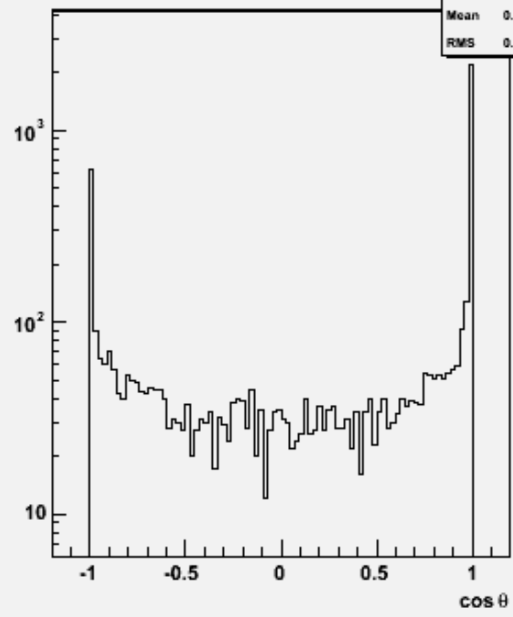
Jet cosθ (All jets)w100401 n2e2e2n2_o
