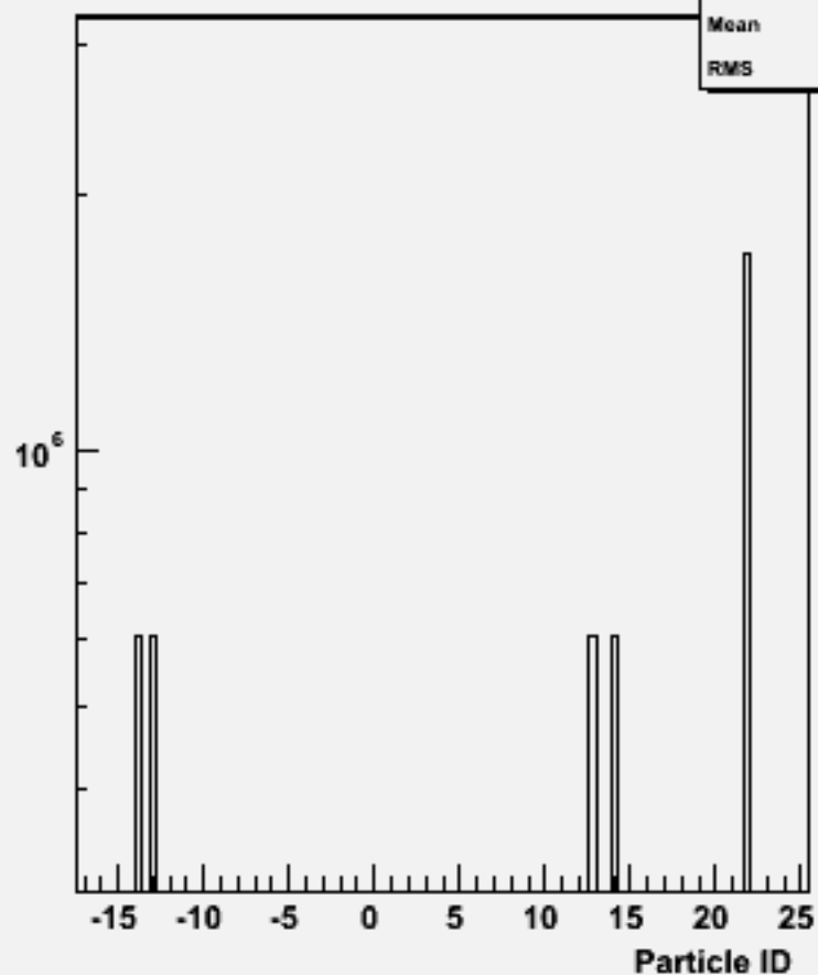
Particle ID : w100400 n2e2e2n2_o
