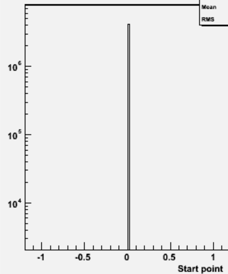
Start point Z : w100400 n2e2e2n2_o
