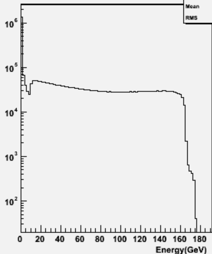
Particle Energy : w100400 n2e2e2n2_o
