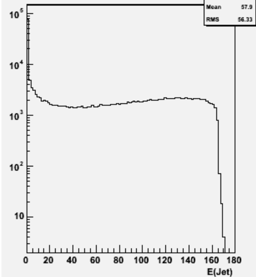
Jet energies(All jets)w100400 n2e2e2n2_o
