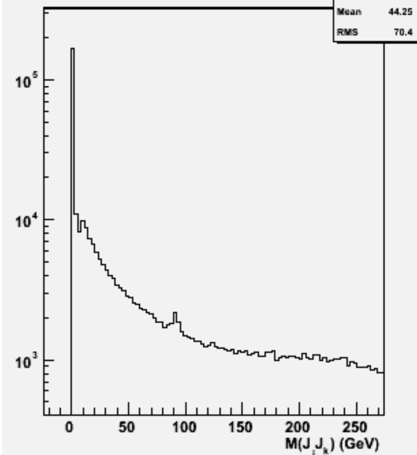
2jets mass(All comb)w100400 n2e2e2n2_o
