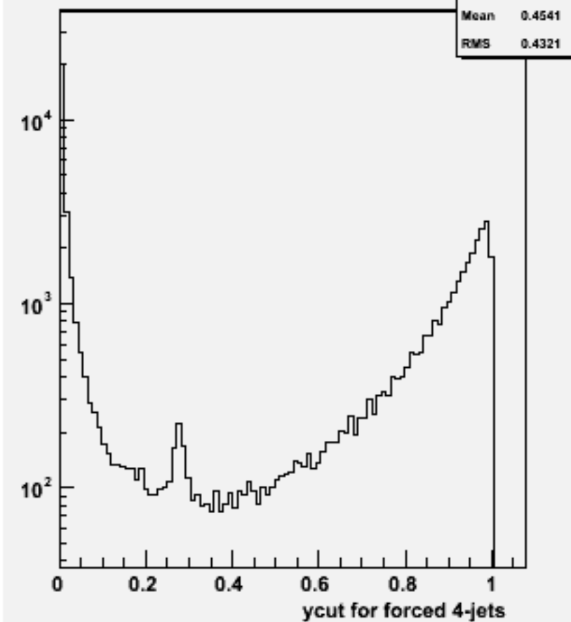
Ycut for 4-jets :w100400 n2e2e2n2_o
