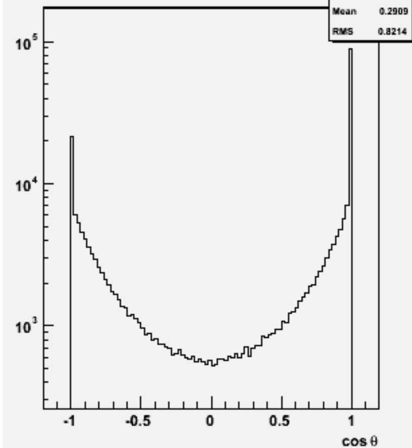
Jet cosθ (All jets)w100400 n2e2e2n2_o
