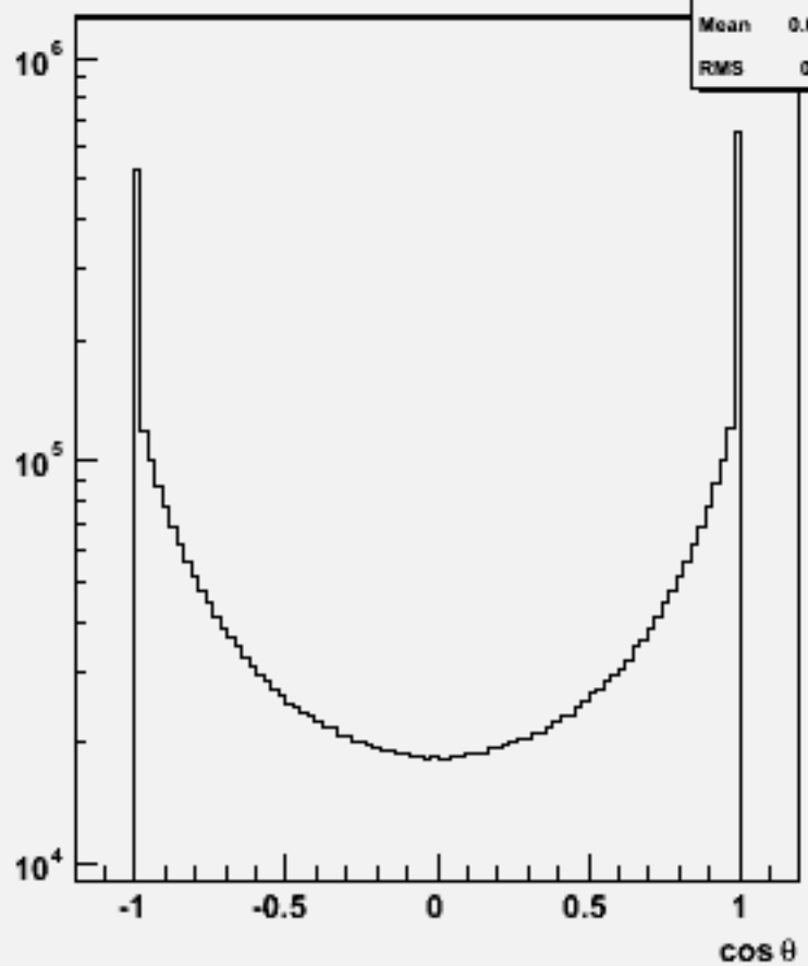
Particle cos \theta : w100400 n2e2e2n2_o
