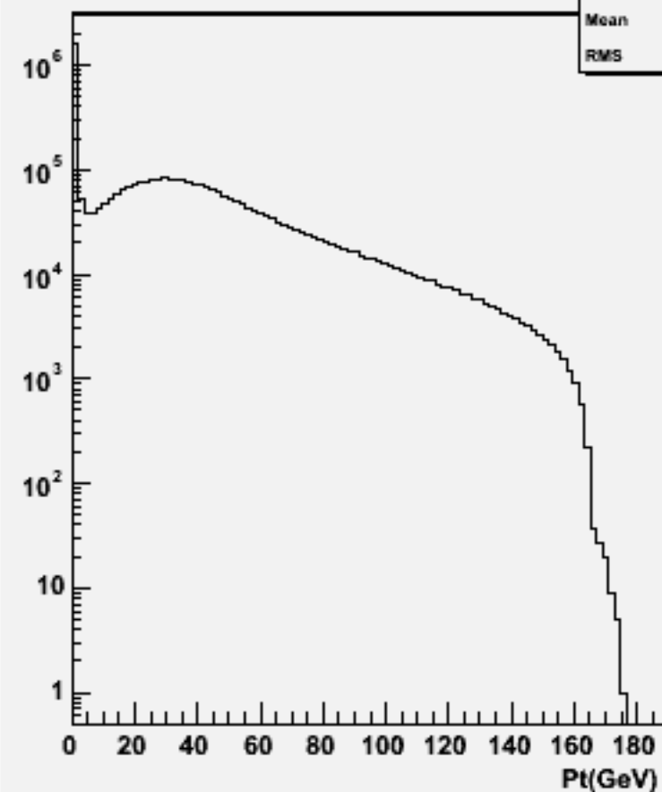
Particle Pt : w100400 n2e2e2n2_o
