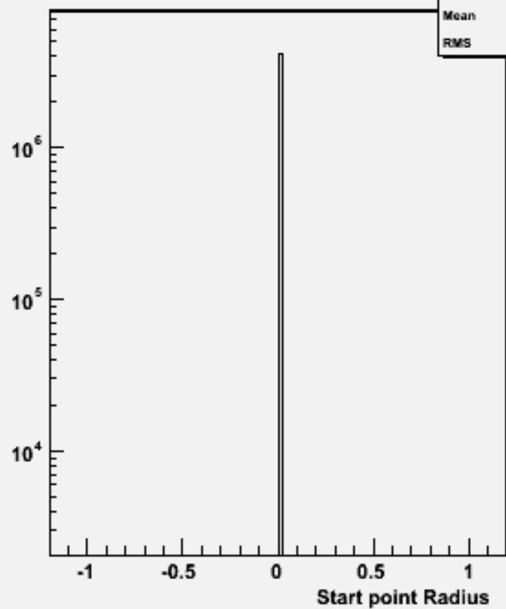
Start point R : w100400 n2e2e2n2_o
