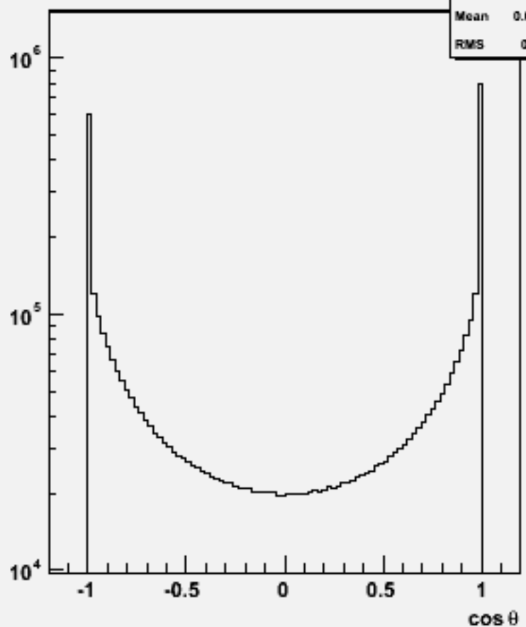
Particle cos \theta : w100396 n2e2e1n1_o
