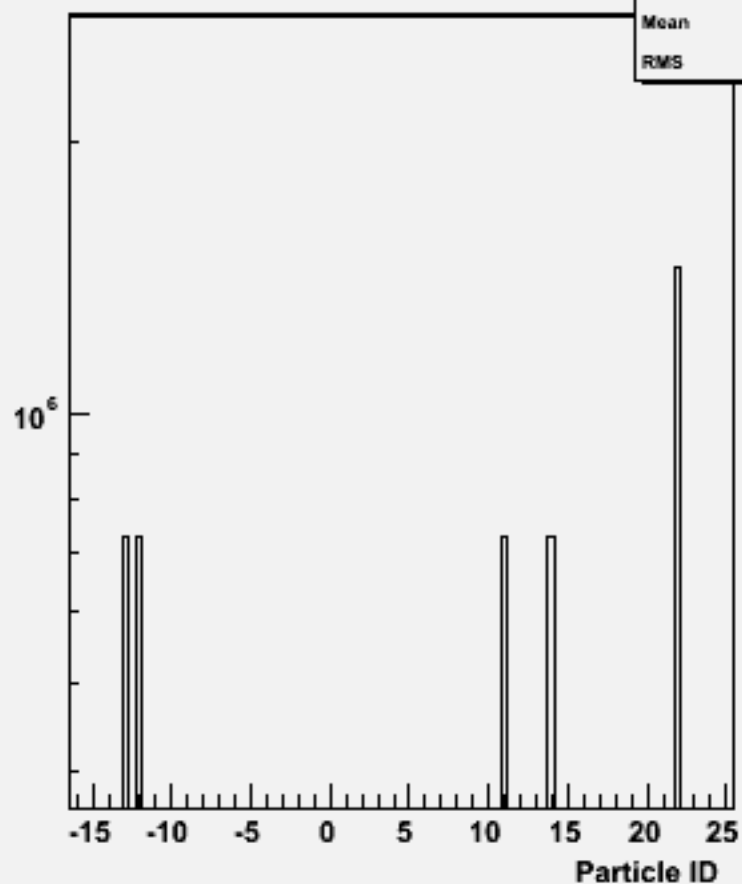
Particle ID : w100396 n2e2e1n1_o
