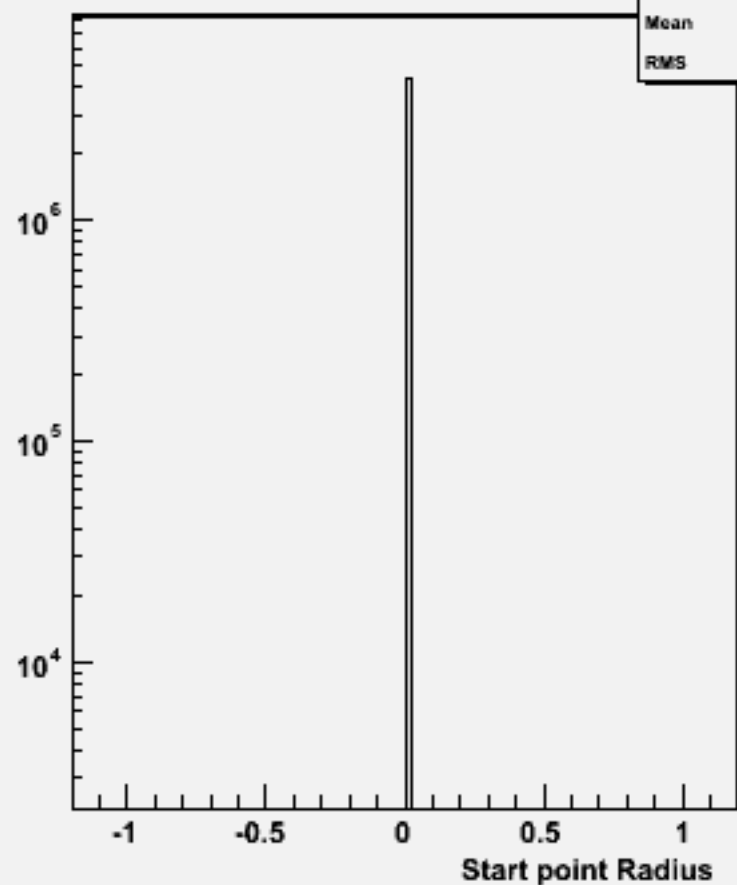
Start point R : w100396 n2e2e1n1_o
