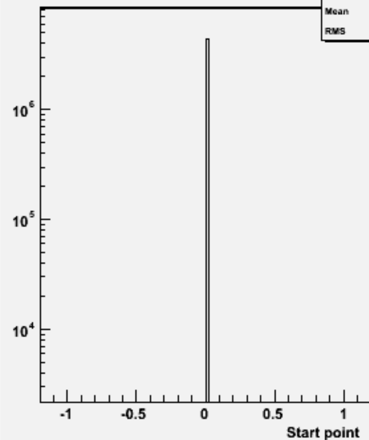
Start point Z : w100396 n2e2e1n1_o
