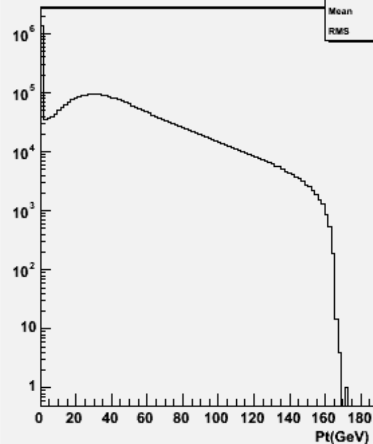
Particle Pt : w100396 n2e2e1n1_o
