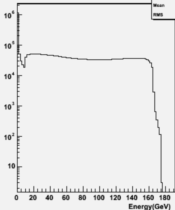
Particle Energy : w100396 n2e2e1n1_o
