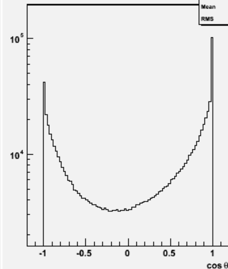
Jet cos \theta (All jets)w100392 n1e1sc_o
