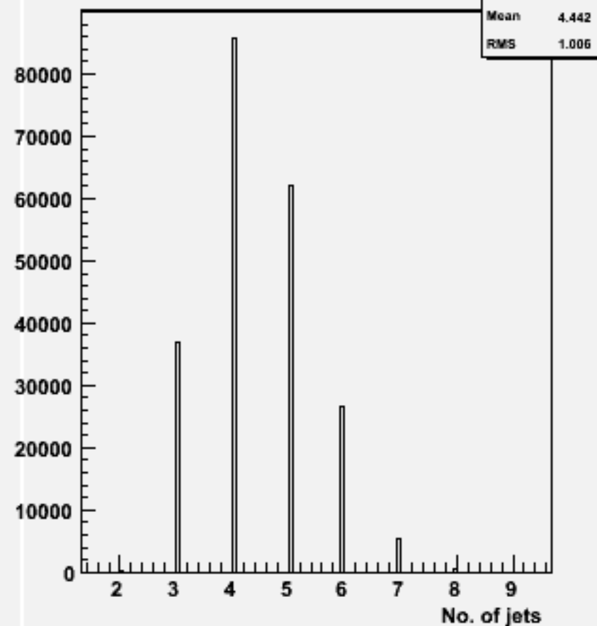
No. jets (ycut=0.001) : w100392 n1e1sc_o
