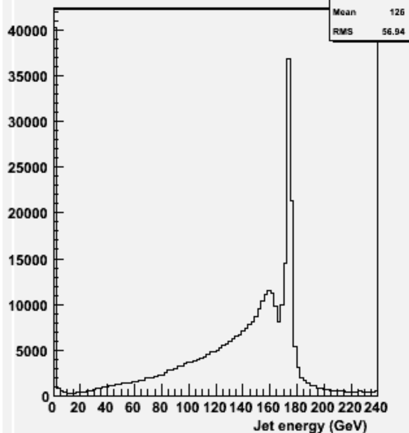
energy for 2-jets :w100392 n1e1sc_o
