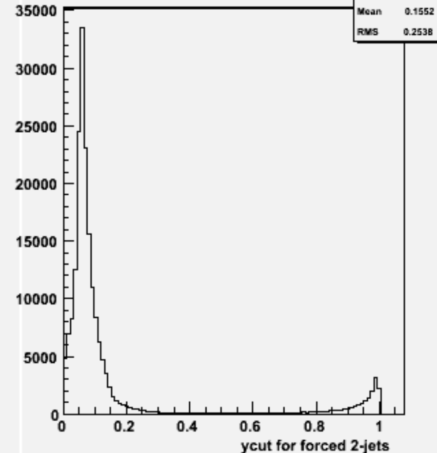
Ycut for 2-jets :w100392 n1e1sc_o
