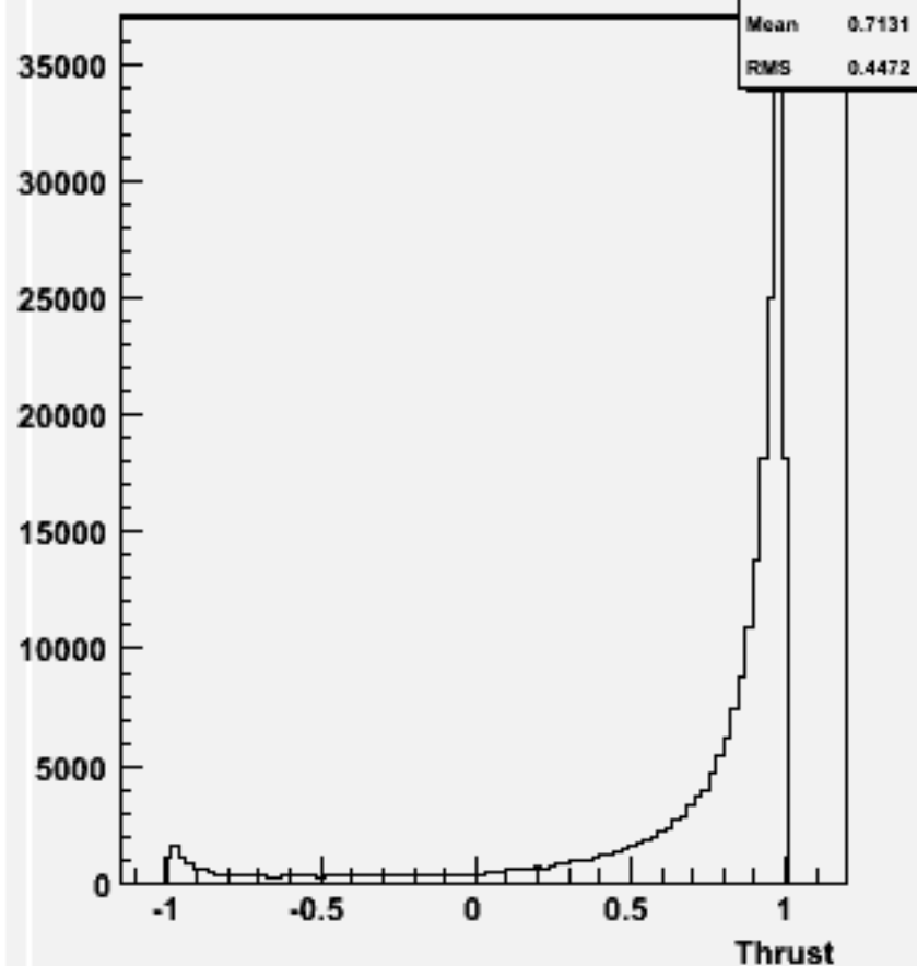
cos \Theta (thrust) w100392 n1e1sc_o
