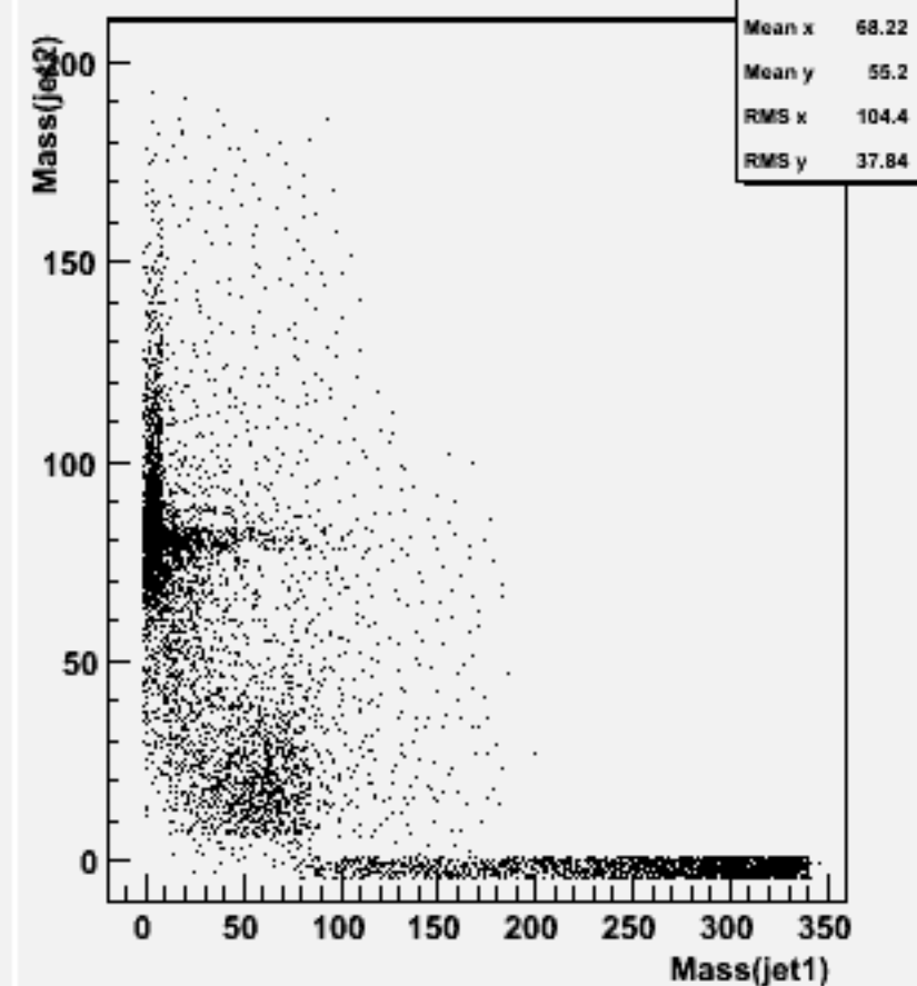
Jet mass for forced 2-jets : w100392 n1e1sc_o
