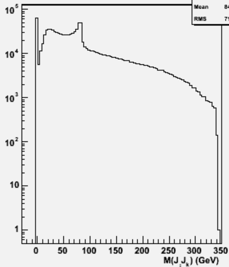
2jets mass(All comb)w100392 n1e1sc_o
