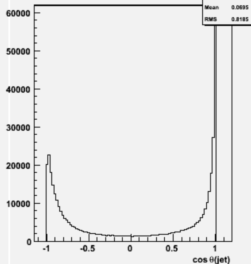
cos \theta for 2-jets :w100392 n1e1sc_o
