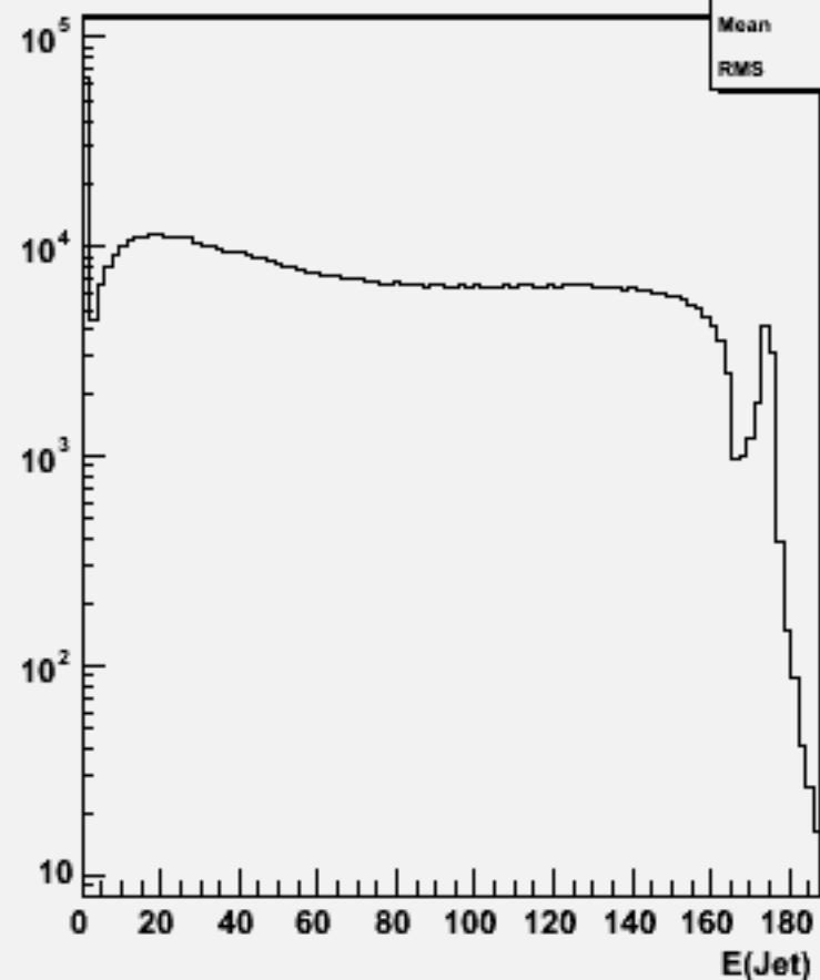
Jet energies(All jets)w100392 n1e1sc_o
