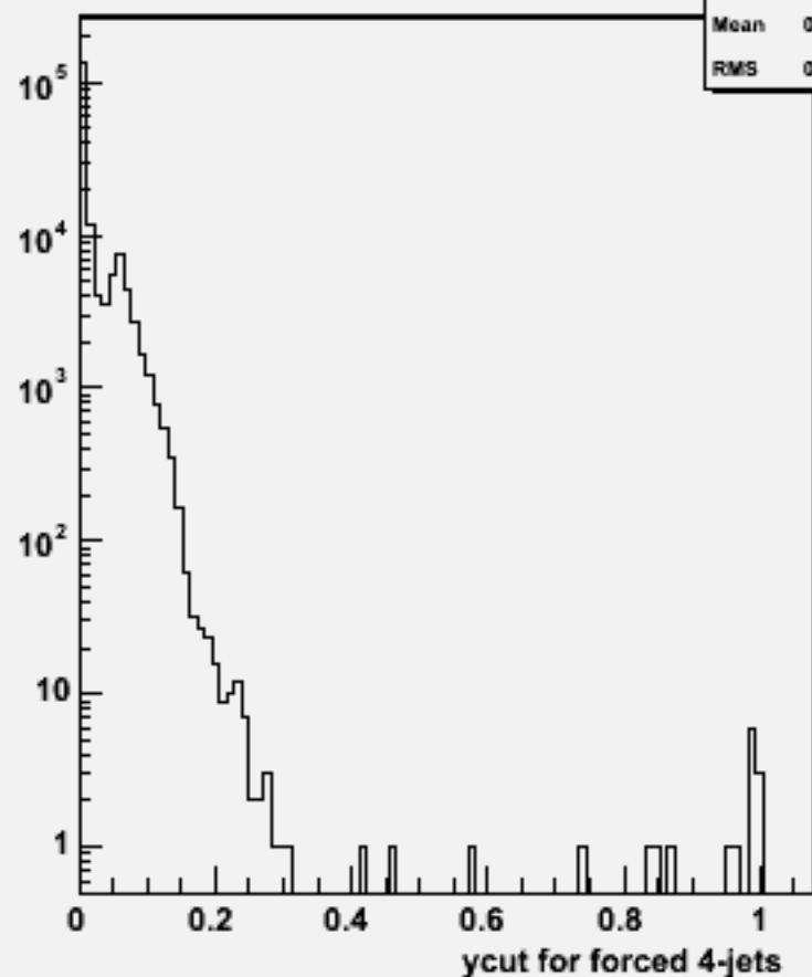
Ycut for 4-jets :w100392 n1e1sc_o
