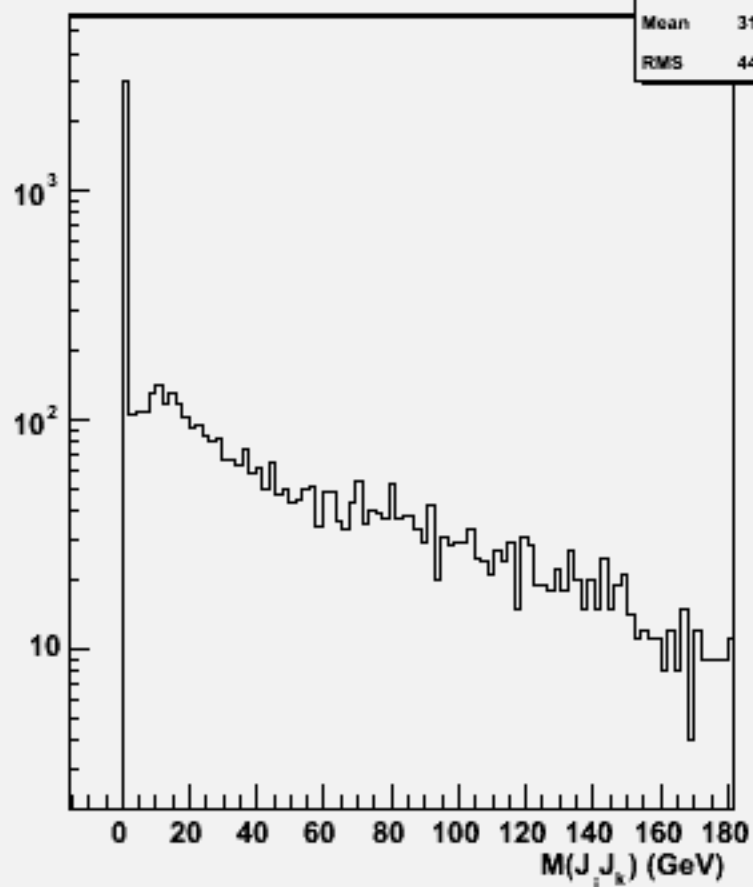
2jets mass(All comb)w100385 n1e1e3n3_o
