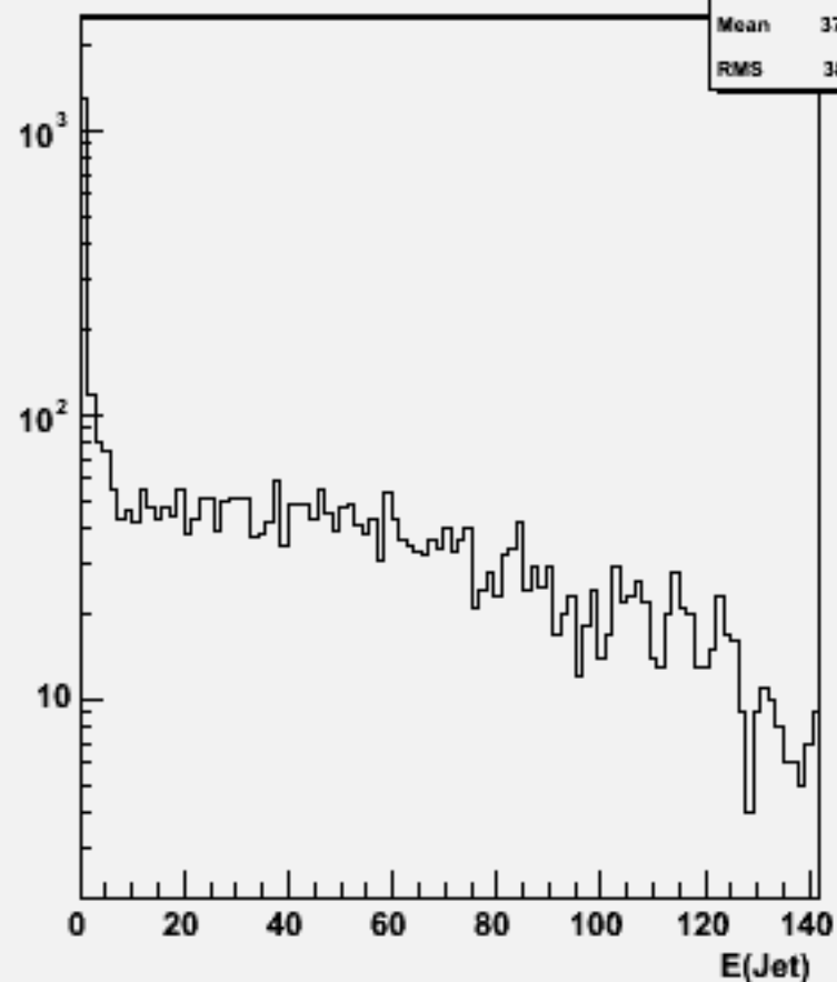
Jet energies(All jets)w100385 n1e1e3n3_o
