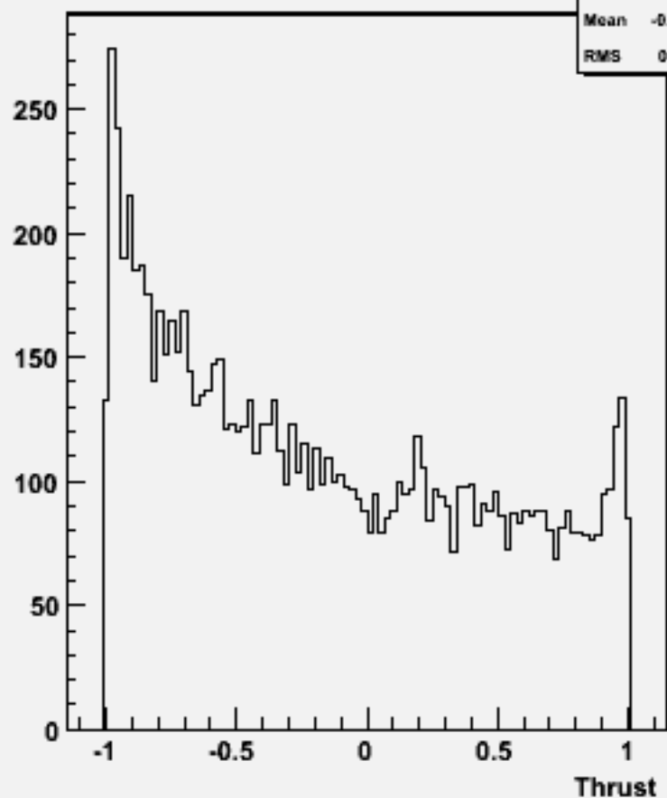
cos \Theta (thrust) w100385 n1e1e3n3_o
