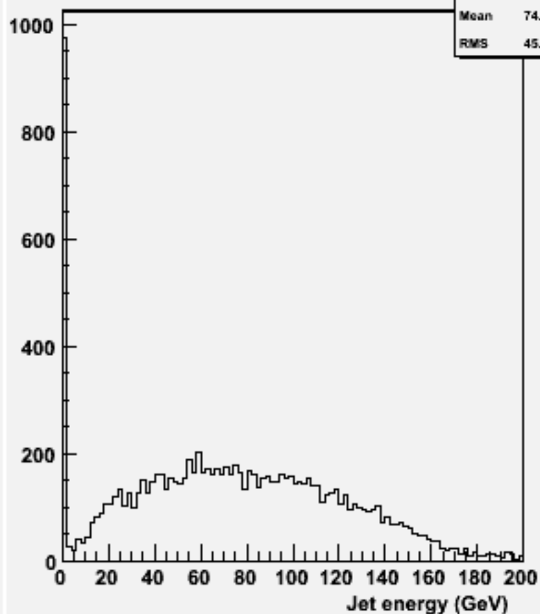
energy for 2-jets :w100385 n1e1e3n3_o
