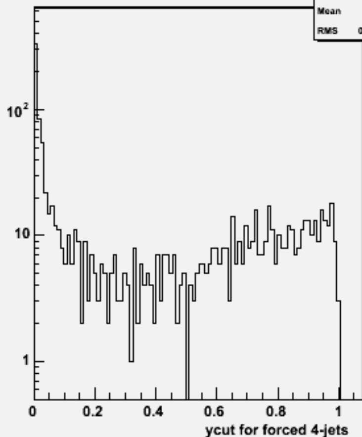
Ycut for 4-jets :w100385 n1e1e3n3_o
