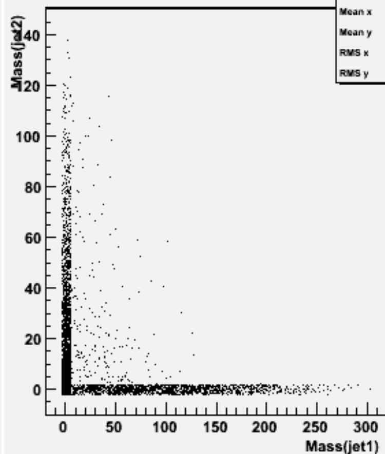
Jet mass for forced 2-jets : w100385 n1e1e3n3_o
