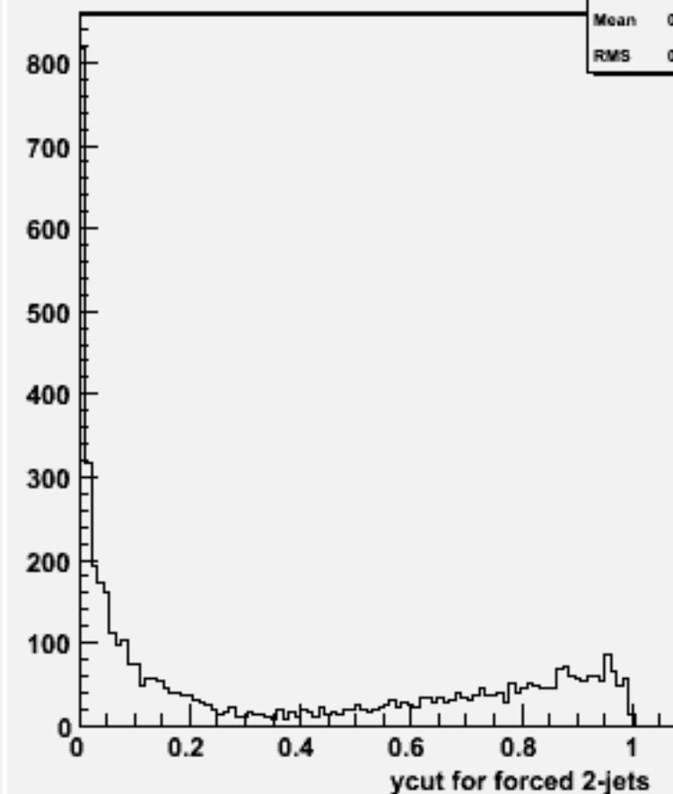
Ycut for 2-jets :w100385 n1e1e3n3_o
