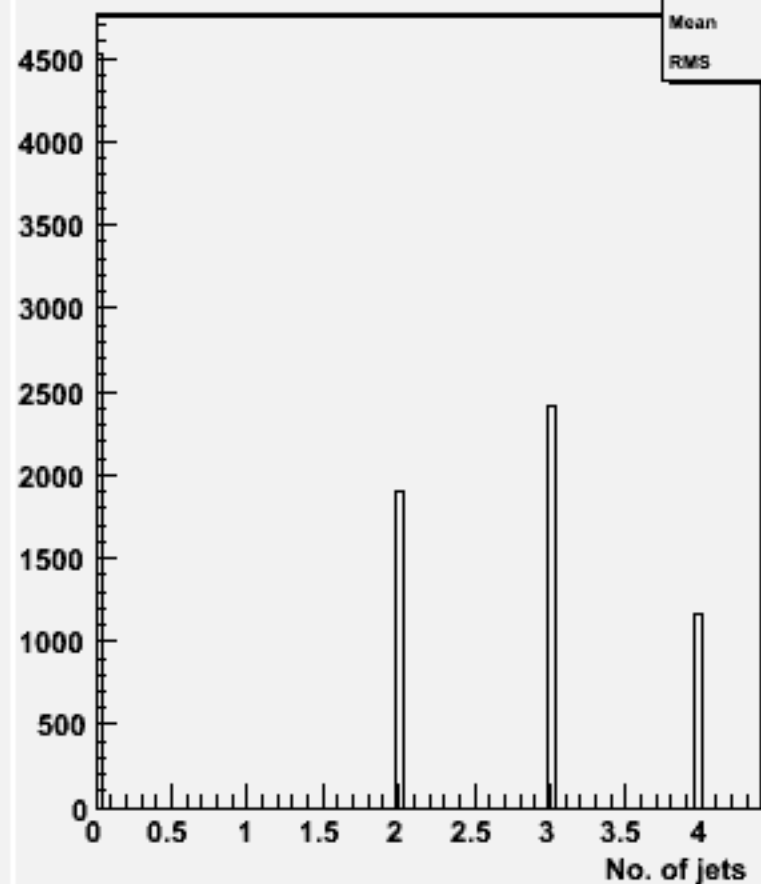
No. jets (ycut=0.001) : w100385 n1e1e3n3_o
