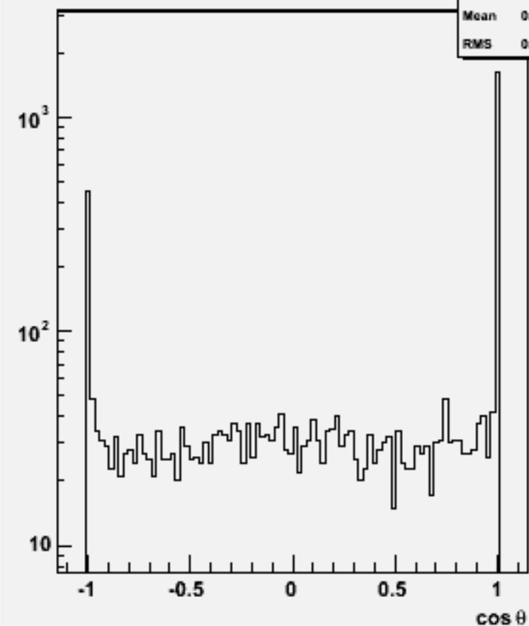
Jet cos \theta (All jets)w100385 n1e1e3n3_o
