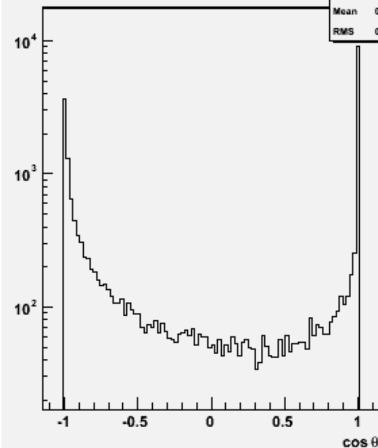
Jet cosθ (All jets)w100383 n1e1e3n3_o
