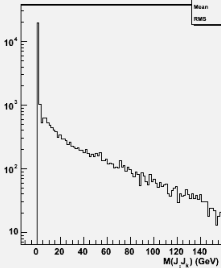
2jets mass(All comb)w100383 n1e1e3n3_o
