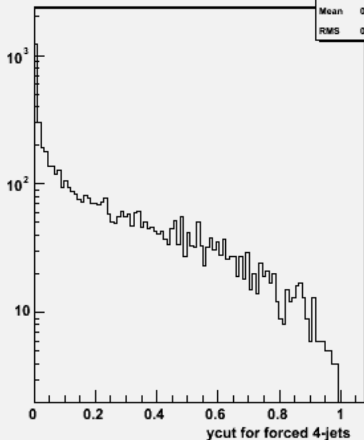
Ycut for 4-jets :w100383 n1e1e3n3_o
