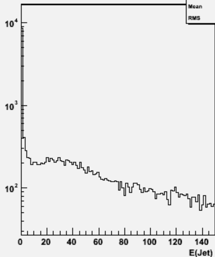
Jet energies(All jets)w100383 n1e1e3n3_o
