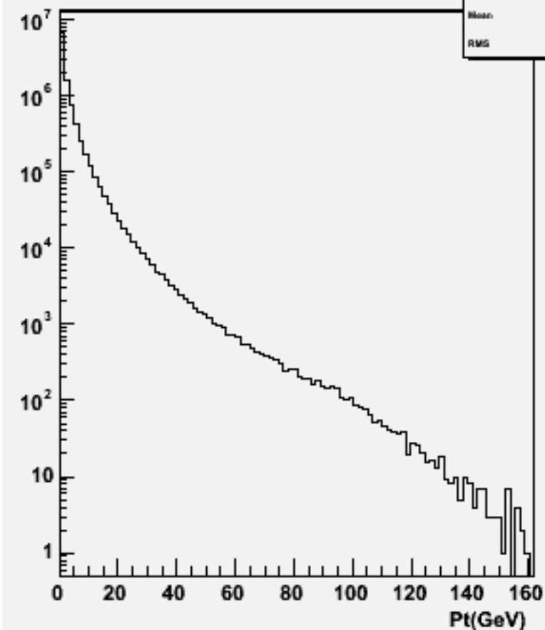
Particle Pt : w100372 bbh_o
