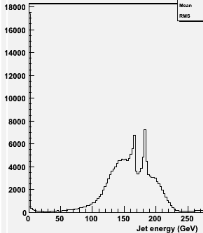
energy for 2-jets :w100372 bbh_o
