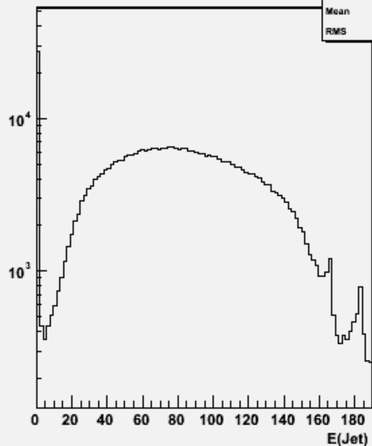
Jet energies(All jets)w100372 bbh_o
