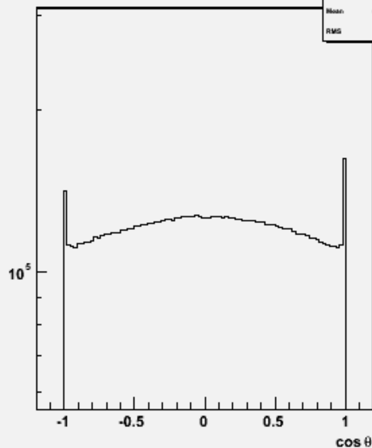
Particle cosθ : w100372 bbh_o
