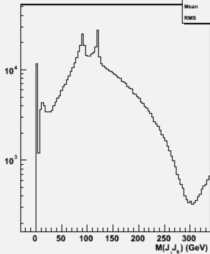
2jets mass(All comb)w100372 bbh_o
