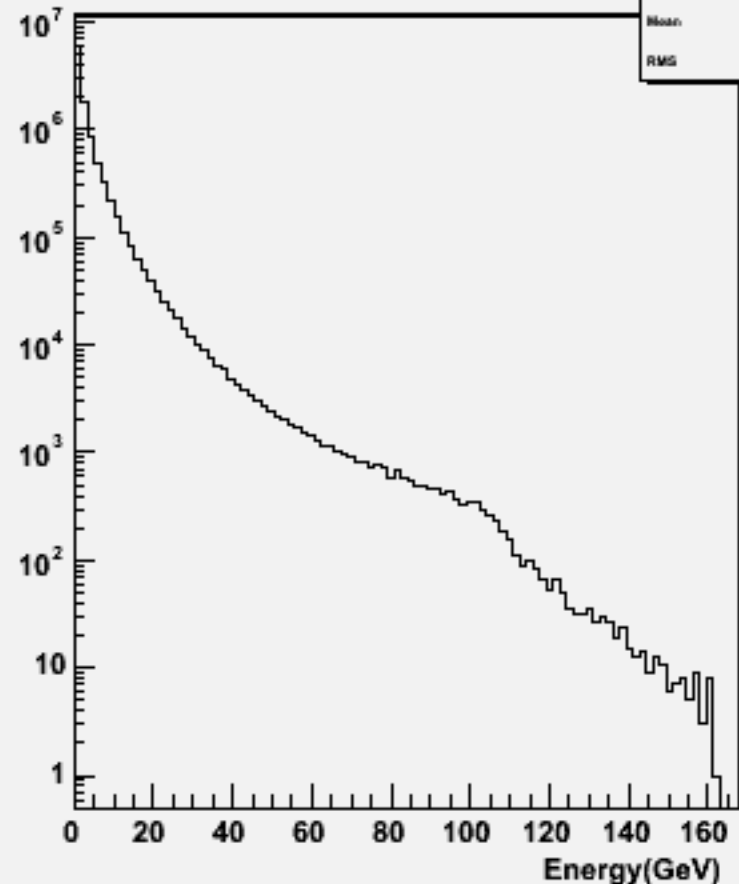
Particle Energy : w100372 bbh_o
