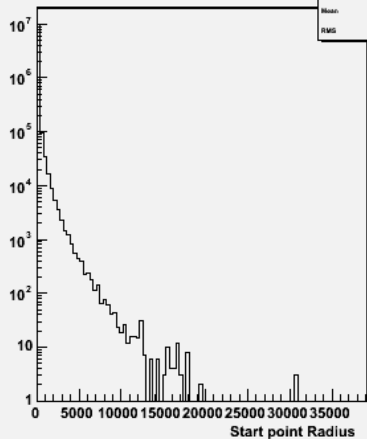
Start point R : w100372 bbh_o
