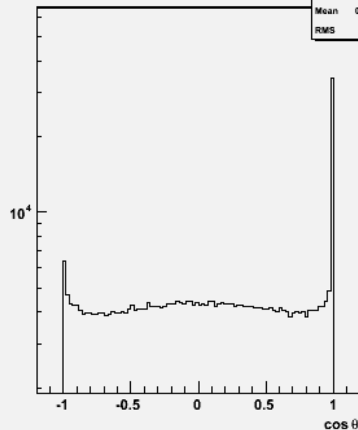
Jet cos \theta (All jets)w100372 bbh_o
