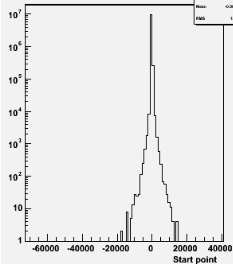
Start point Z : w100372 bbh_o
