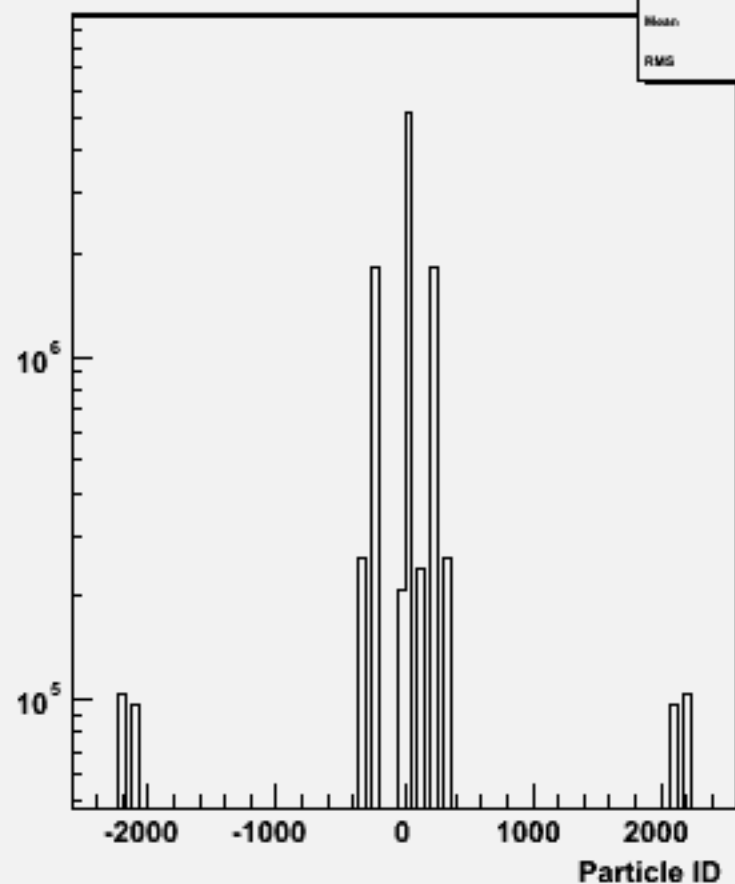
Particle ID : w100372 bbh_o
