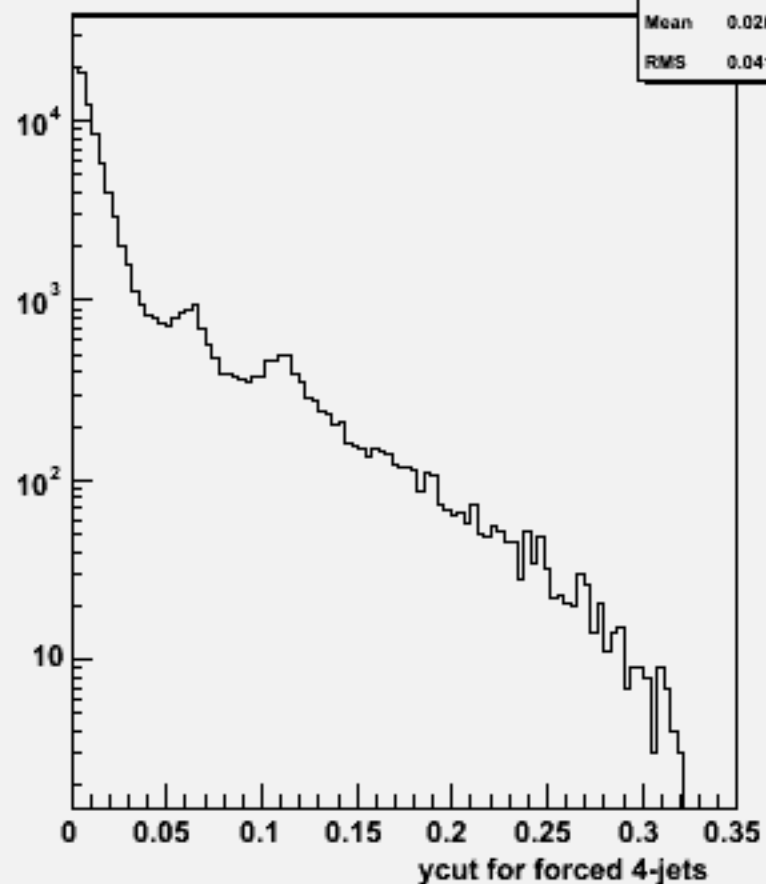
Ycut for 4-jets :w100372 bbh_o
