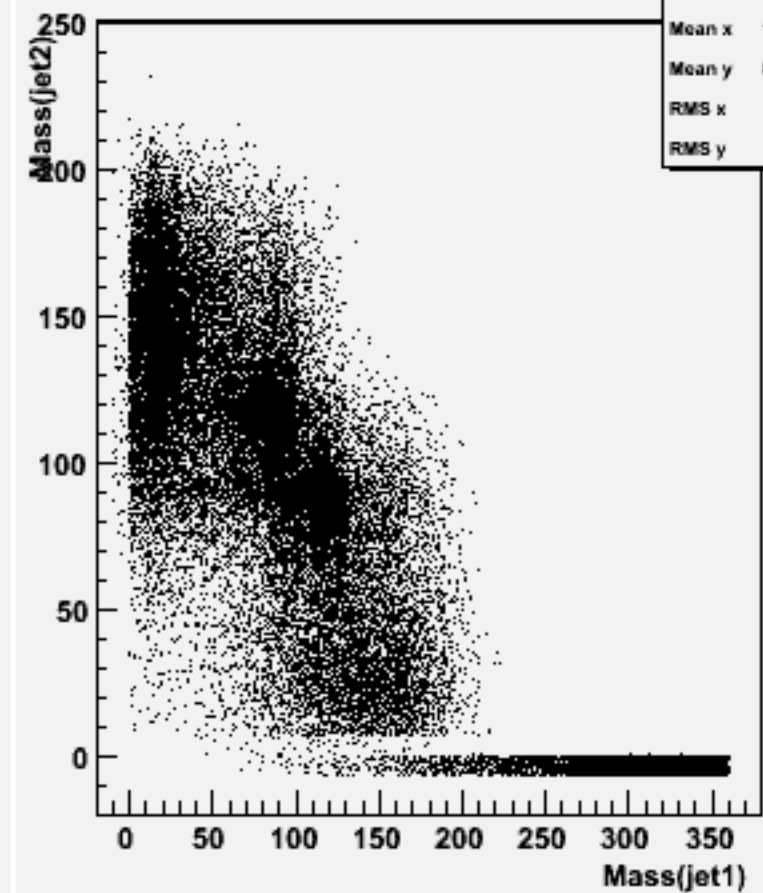
Jet mass for forced 2-jets : w100372 bbh_o
