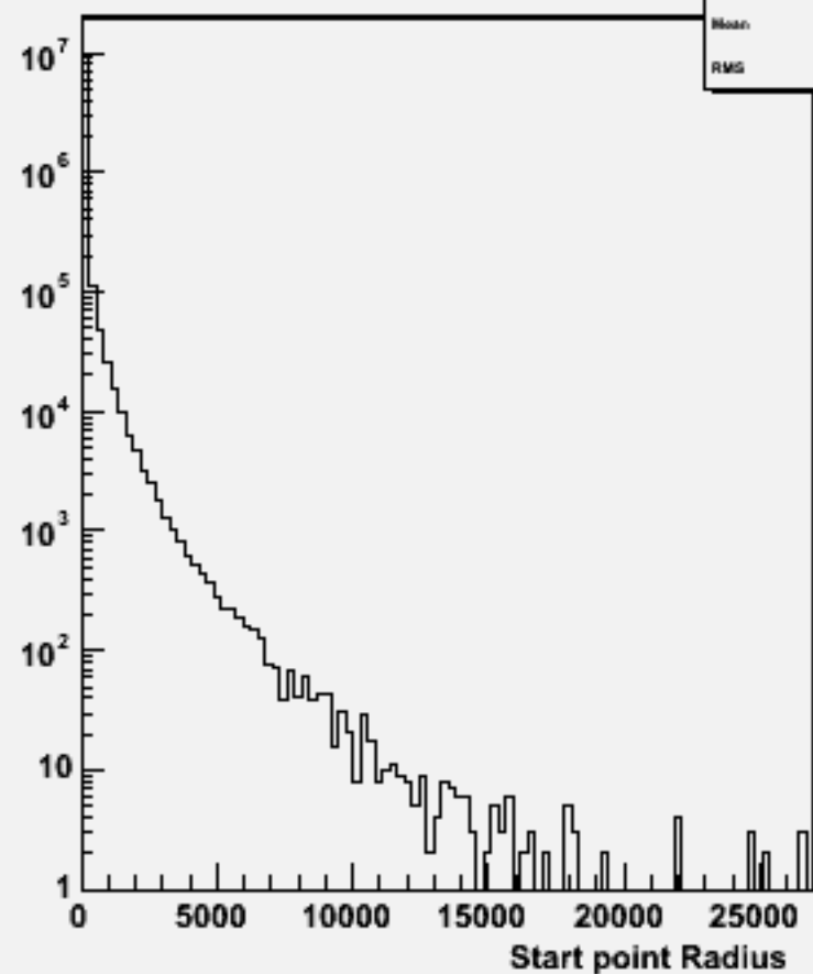
Start point R : w100371 bbh_o
