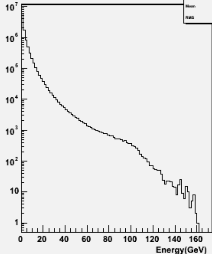
Particle Energy : w100371 bbh_o
