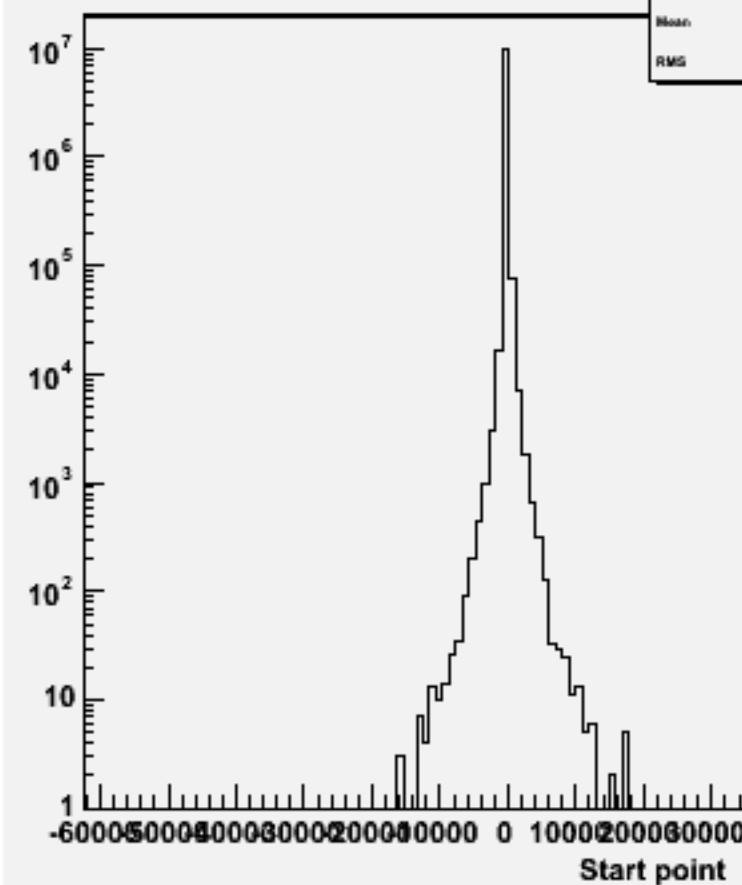
Start point Z : w100371 bbh_o
