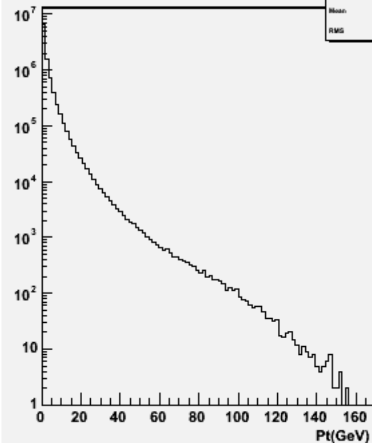
Particle Pt : w100371 bbh_o
