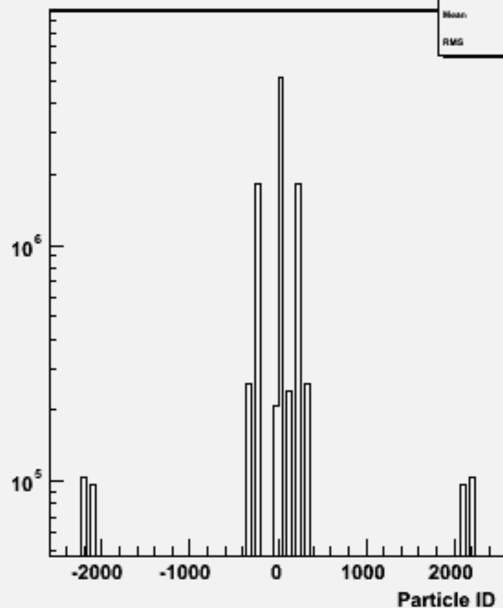
Particle ID : w100371 bbh_o
