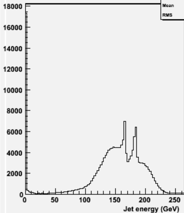
energy for 2-jets :w100371 bbh_o
