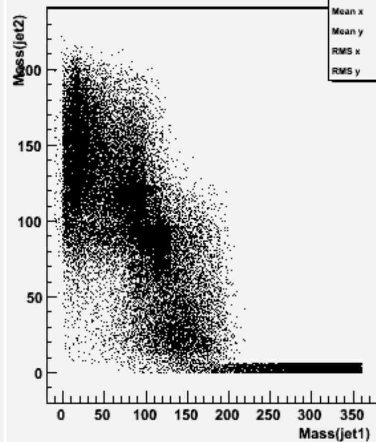
Jet mass for forced 2-jets : w100371 bbh_o
