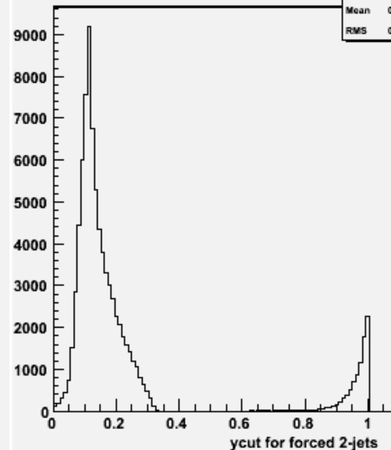
Ycut for 2-jets :w100371 bbh_o
