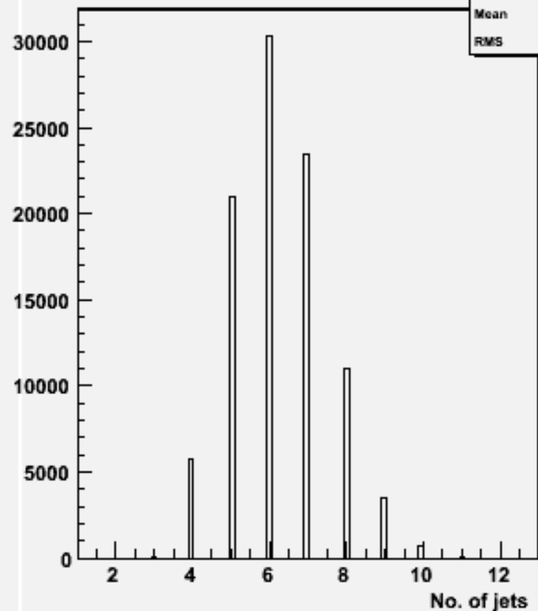
No. jets (ycut=0.001) : w100371 bbh_o
