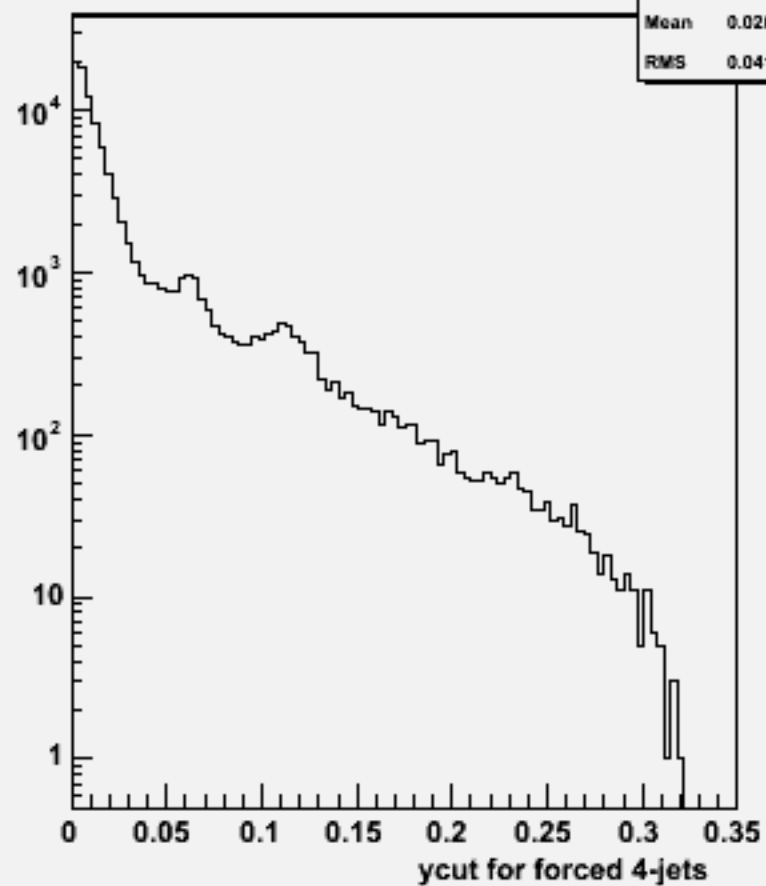
Ycut for 4-jets :w100371 bbh_o
