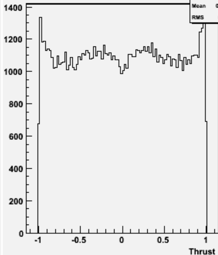
cos \Theta (thrust) w100371 bbh_o
