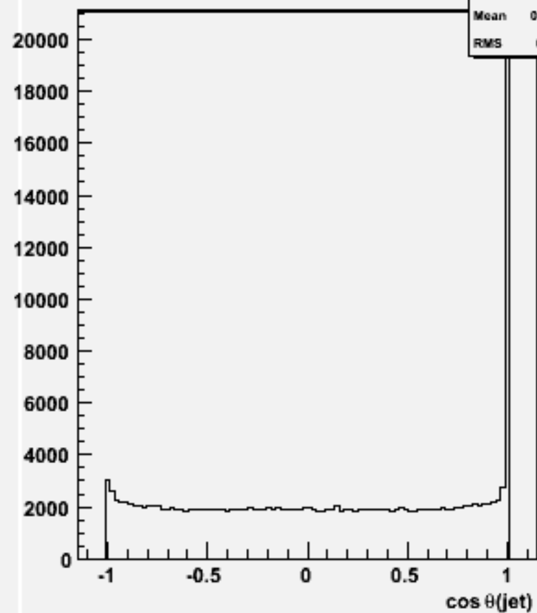
cos \theta for 2-jets :w100371 bbh_o
