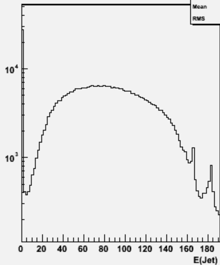
Jet energies(All jets)w100371 bbh_o
