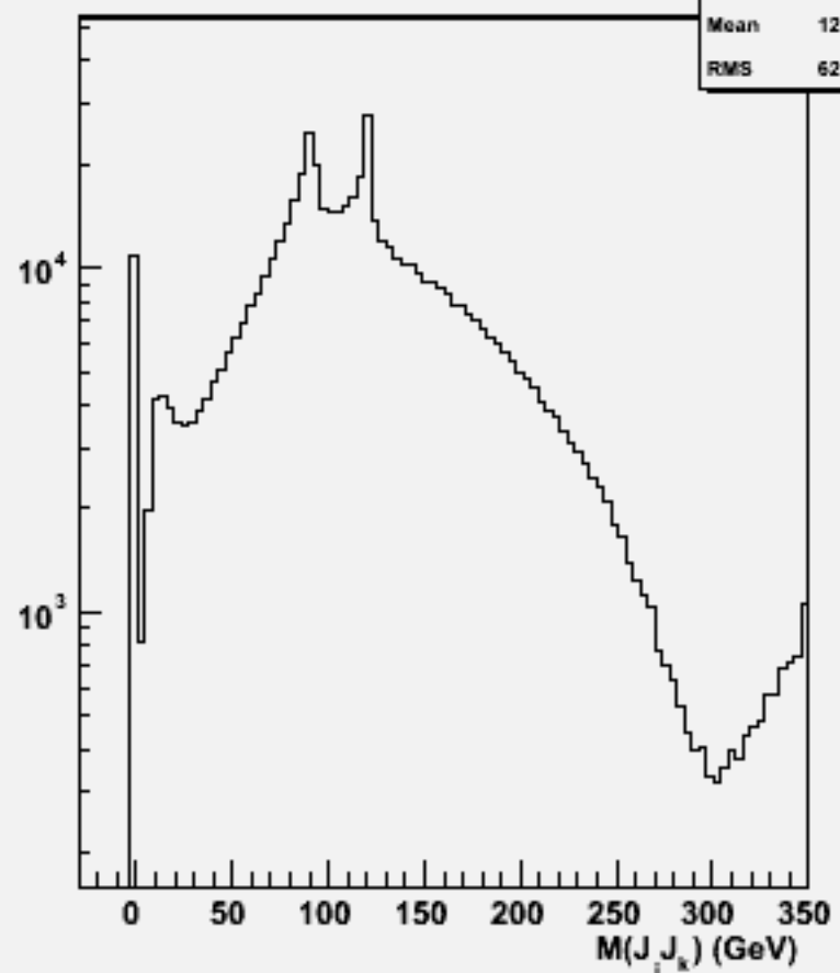
2jets mass(All comb)w100371 bbh_o
