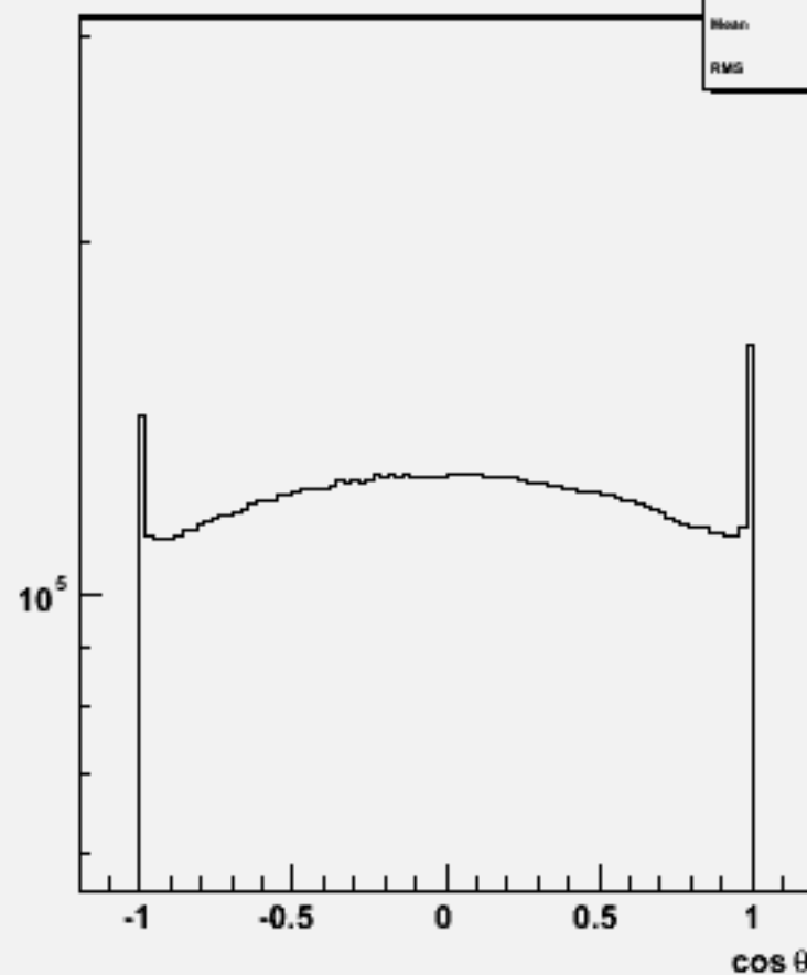
Particle cosθ : w100371 bbh_o
