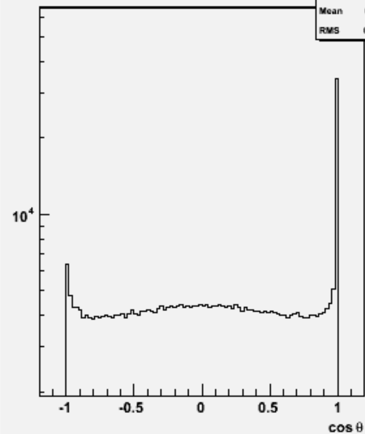
Jet cos \theta (All jets)w100371 bbh_o
