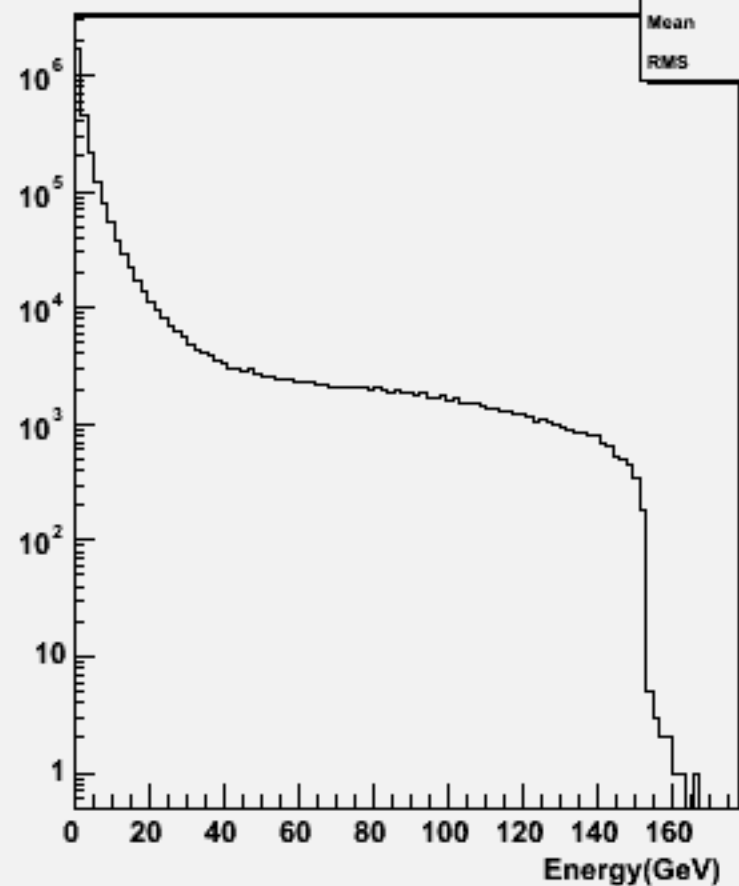
Particle Energy : w100356 e2e2h_o
