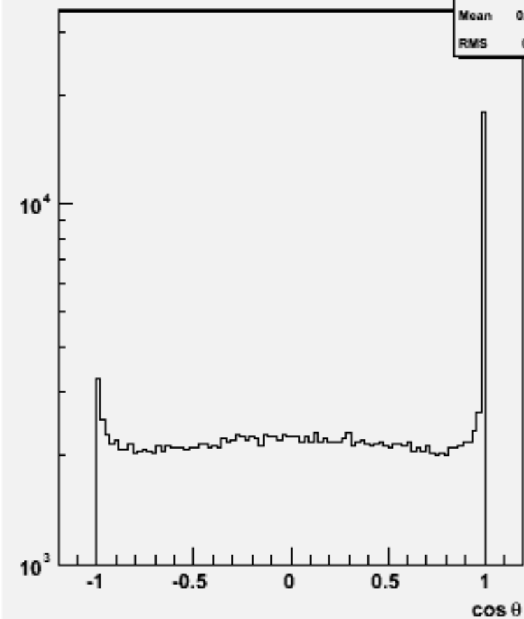
Jet cos \theta (All jets)w100356 e2e2h_o
