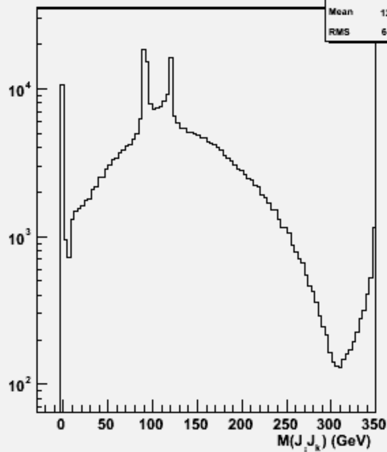
2jets mass(All comb)w100356 e2e2h_o
