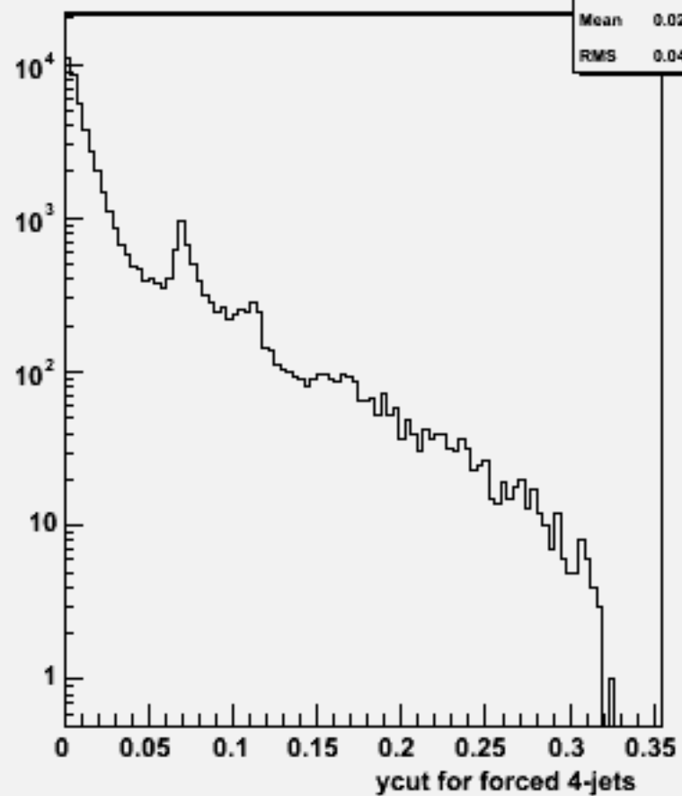
Ycut for 4-jets :w100356 e2e2h_o
