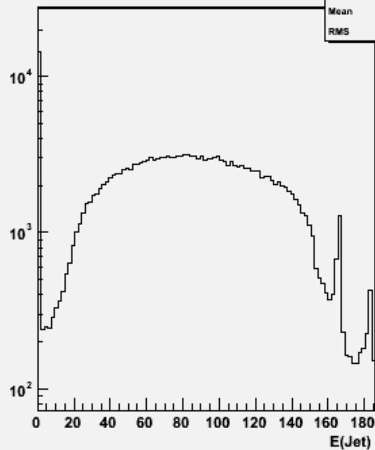
Jet energies(All jets)w100356 e2e2h_o
