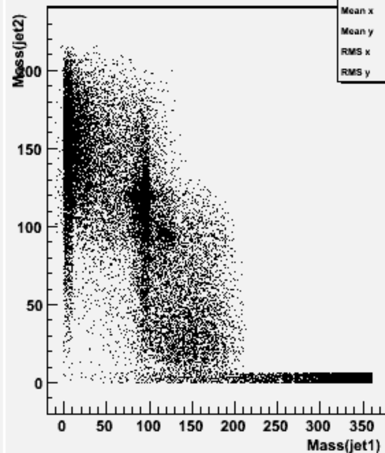
Jet mass for forced 2-jets : w100356 e2e2h_o
