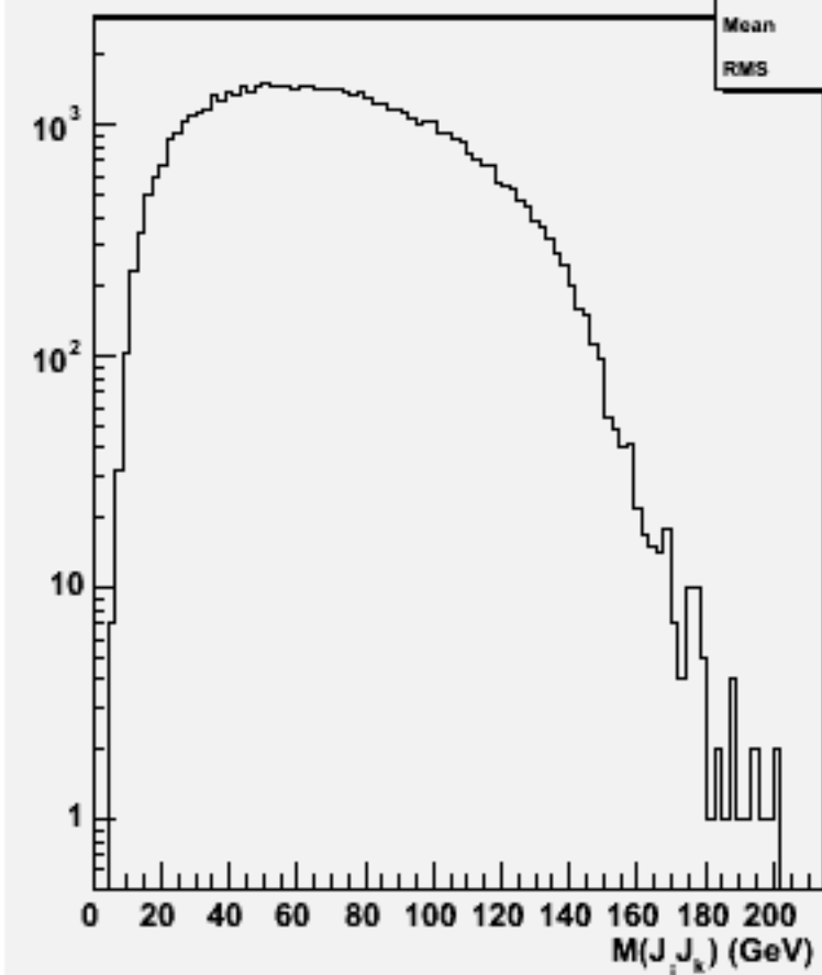
2jets mass(All comb)p105013 bbe1n1e3n3_p
