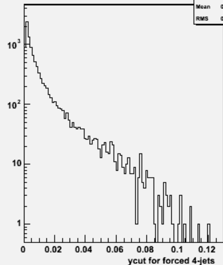
Ycut for 4-jets :p105013 bbe1n1e3n3_p
