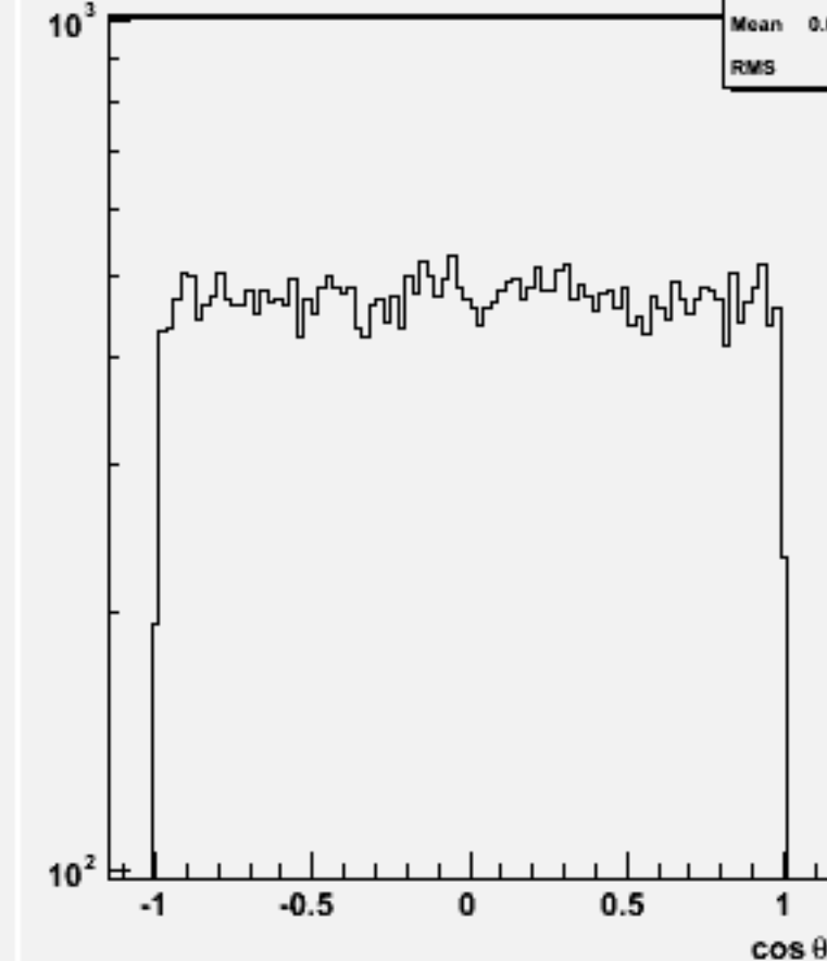
Jet cos \theta (All jets)p105013 bbe1n1e3n3_p
