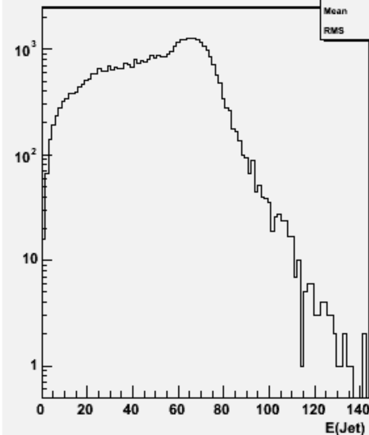
Jet energies(All jets)p105013 bbe1n1e3n3_p
