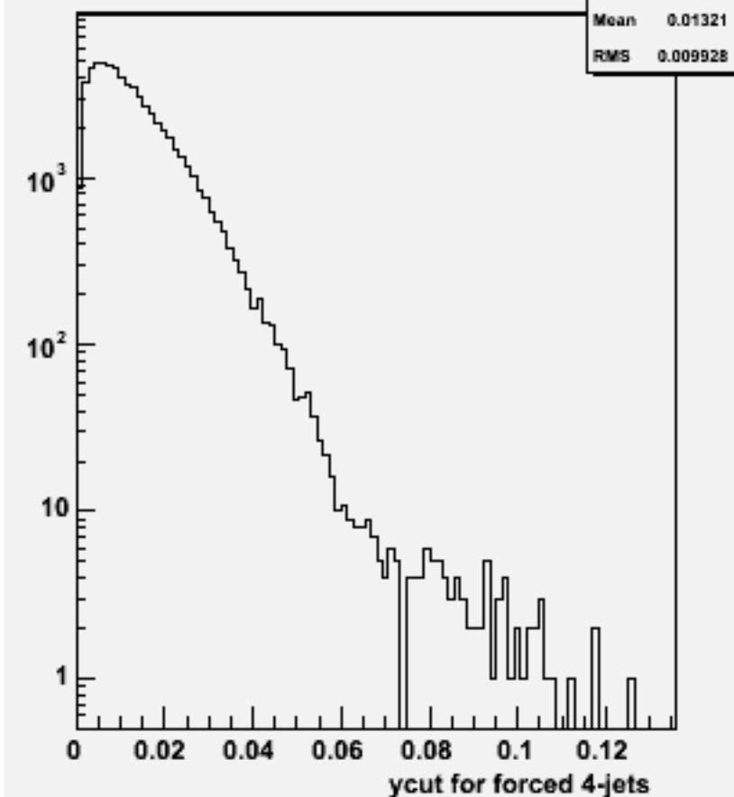
Ycut for 4-jets :p105007 bbe3n3qq_p
