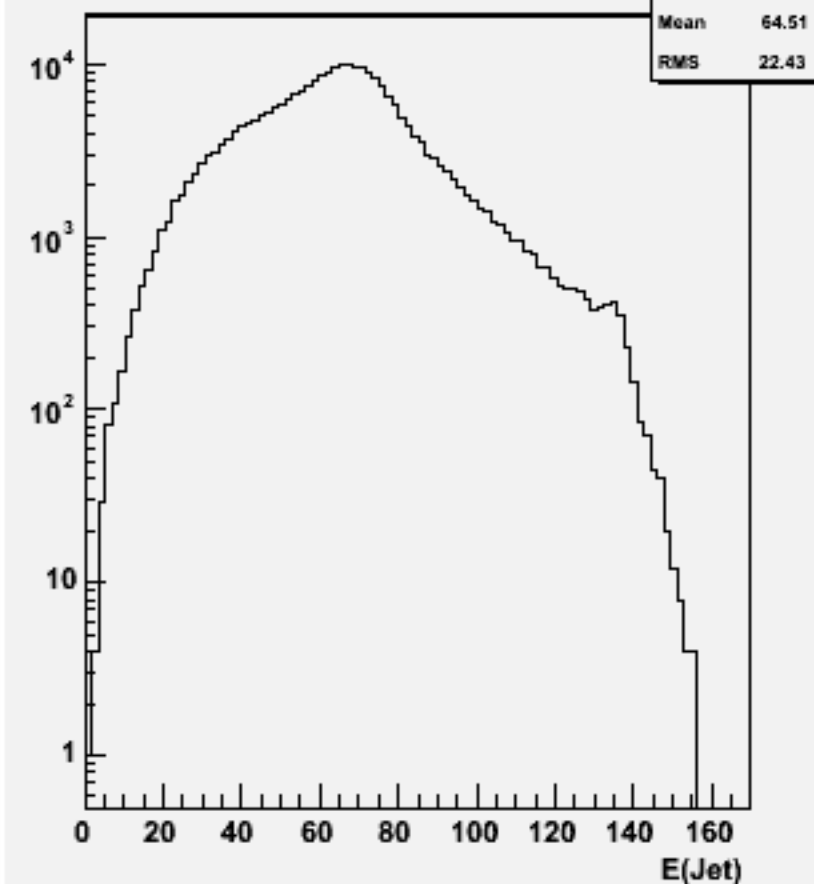
Jet energies(All jets)p105007 bbe3n3qq_p
