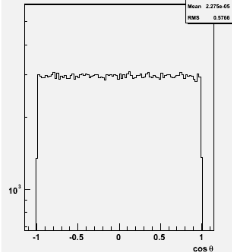
Jet cos \theta (All jets)p105007 bbe3n3qq_p
