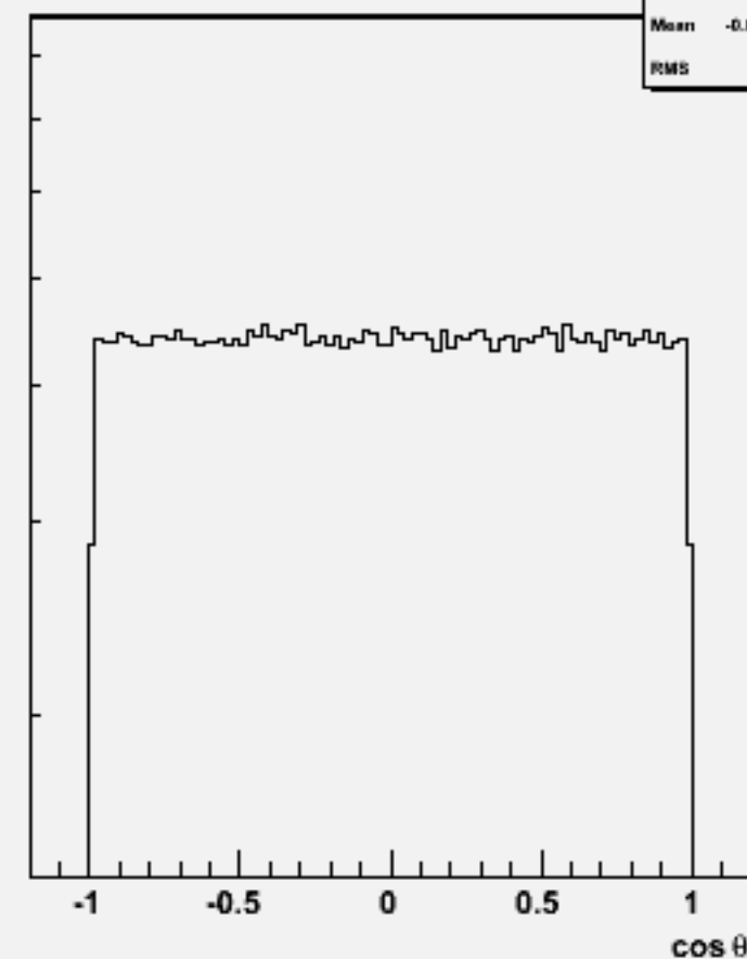
Jet cosθ (All jets)p105006 bbe3n3qq_p
