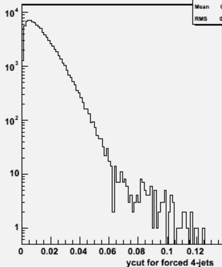
Ycut for 4-jets :p105006 bbe3n3qq_p
