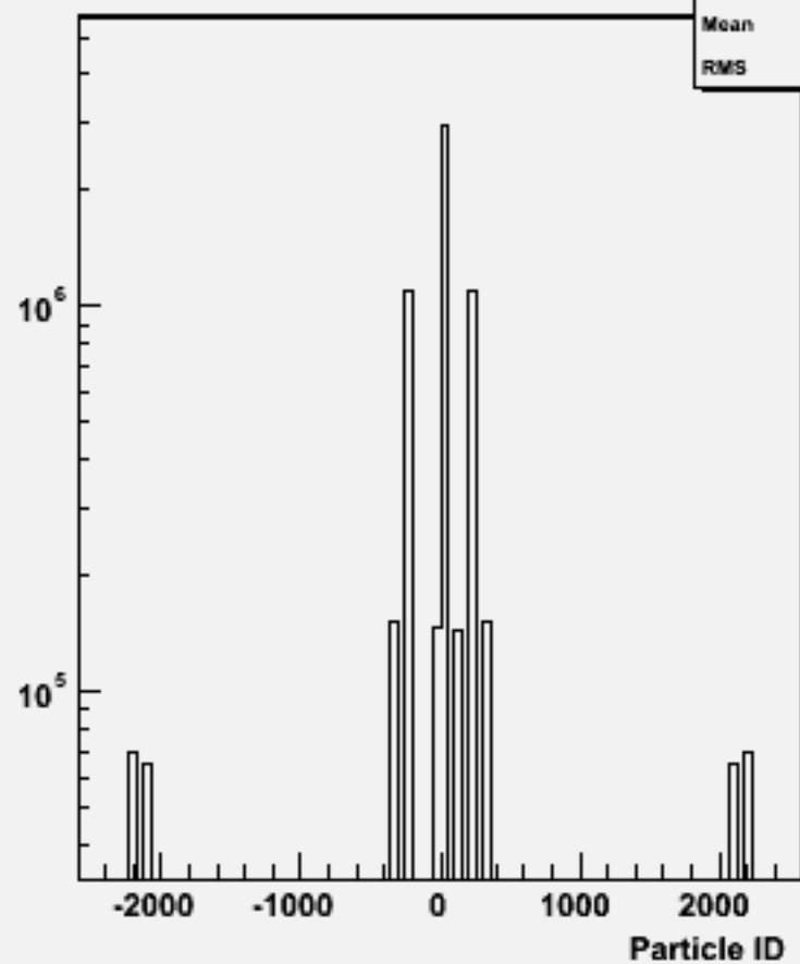
Particle ID : p105005 bbe2n2qq_p
