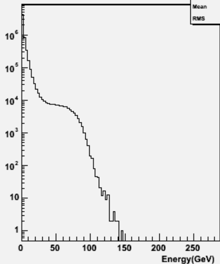
Particle Energy : p105005 bbe2n2qq_p
