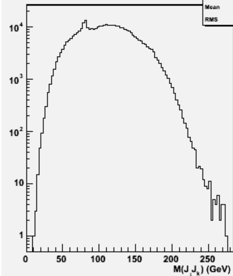
2jets mass(All comb)p105005 bbe2n2qq_p
