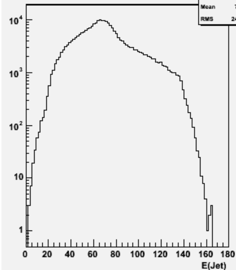
Jet energies(All jets)p105005 bbe2n2qq_p
