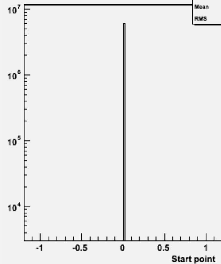
Start point Z : p105005 bbe2n2qq_p
