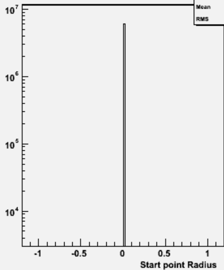
Start point R : p105005 bbe2n2qq_p
