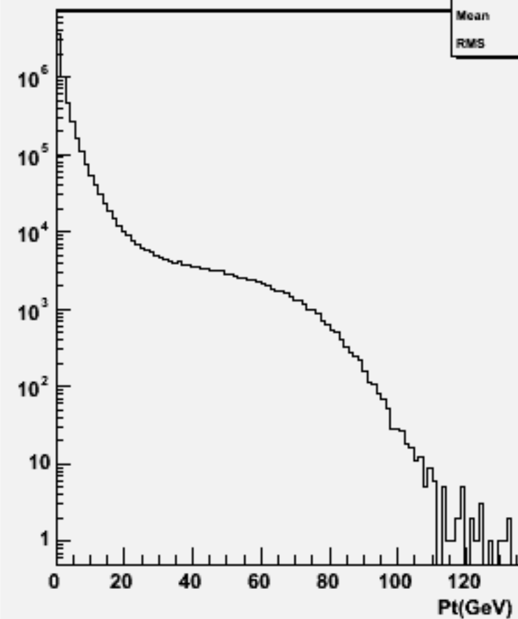
Particle Pt : p105005 bbe2n2qq_p
