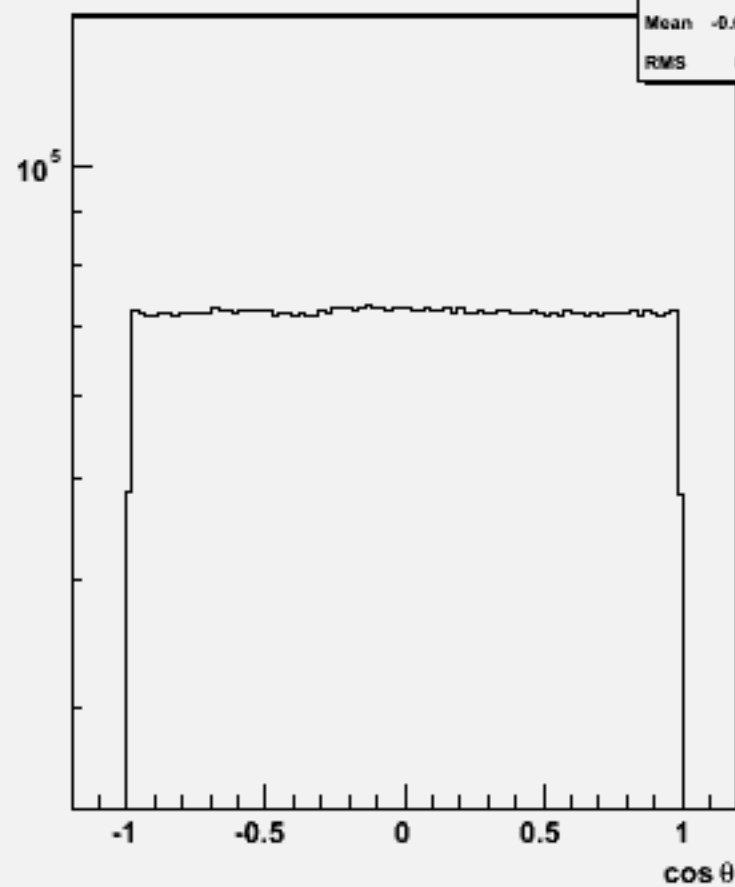
Particle cos \theta : p105005 bbe2n2qq_p
