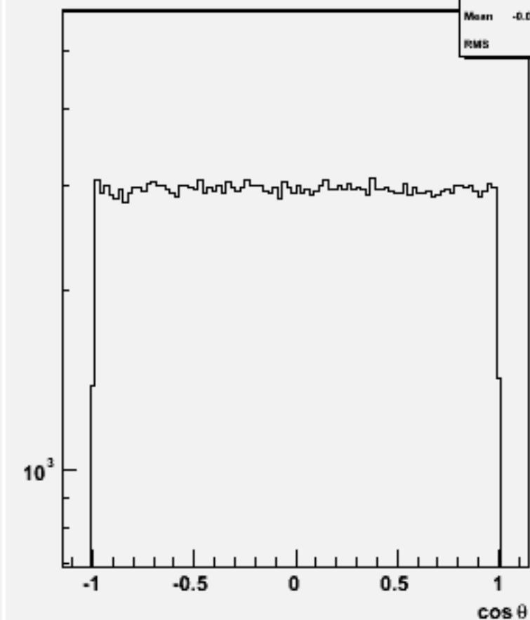
Jet cosθ (All jets)p105005 bbe2n2qq_p
