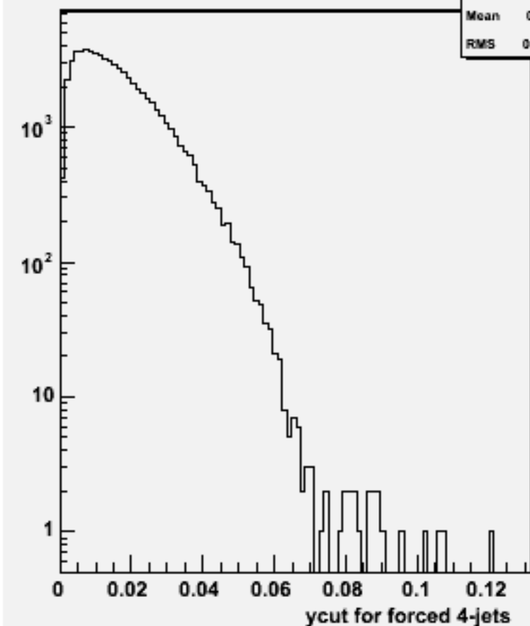
Ycut for 4-jets :p105005 bbe2n2qq_p
