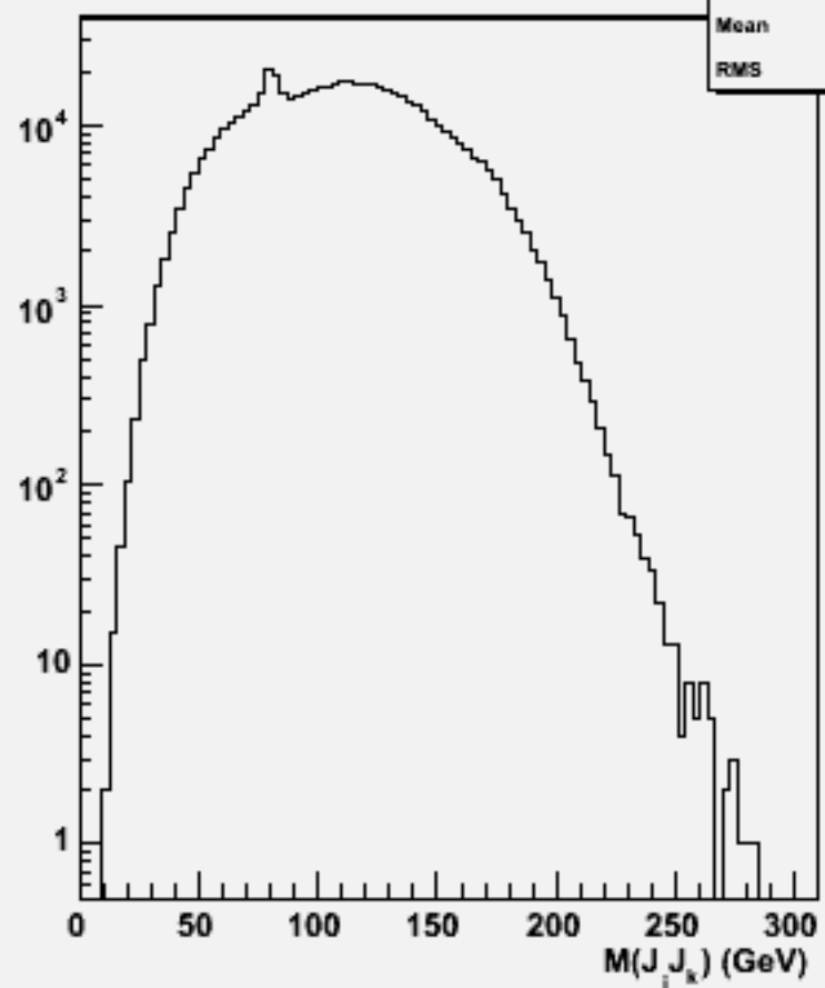
2jets mass(All comb)p105002 bbe1n1qq_p
