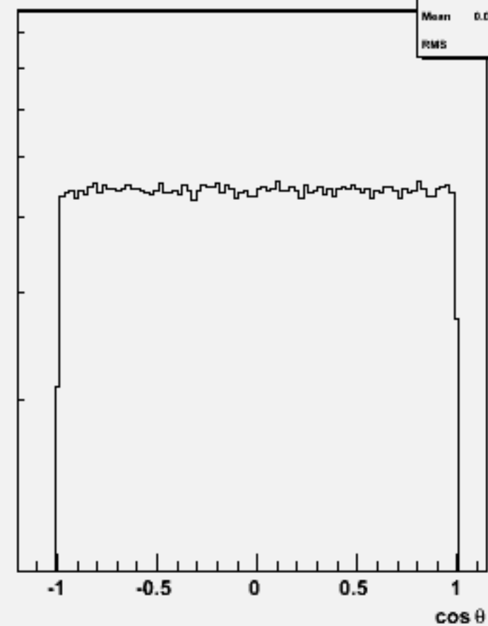
Jet cosθ (All jets)p105002 bbe1n1qq_p
