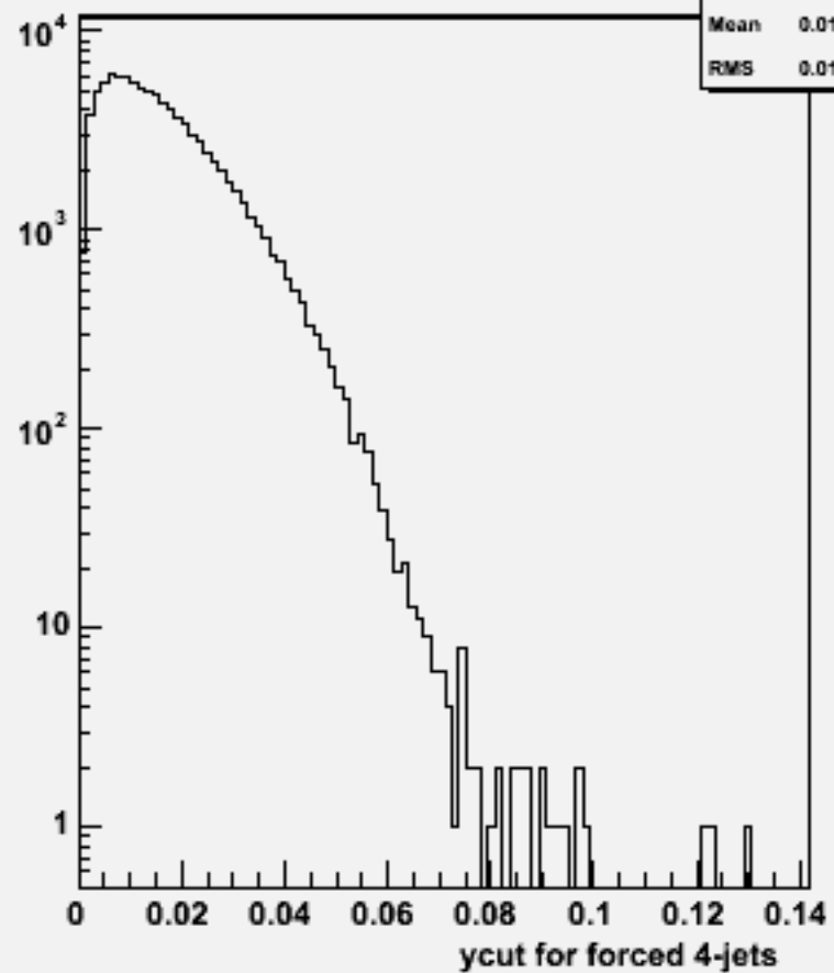
Ycut for 4-jets :p105002 bbe1n1qq_p
