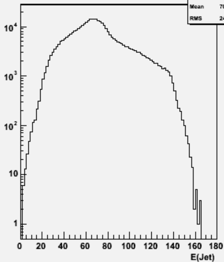
Jet energies(All jets)p105002 bbe1n1qq_p
