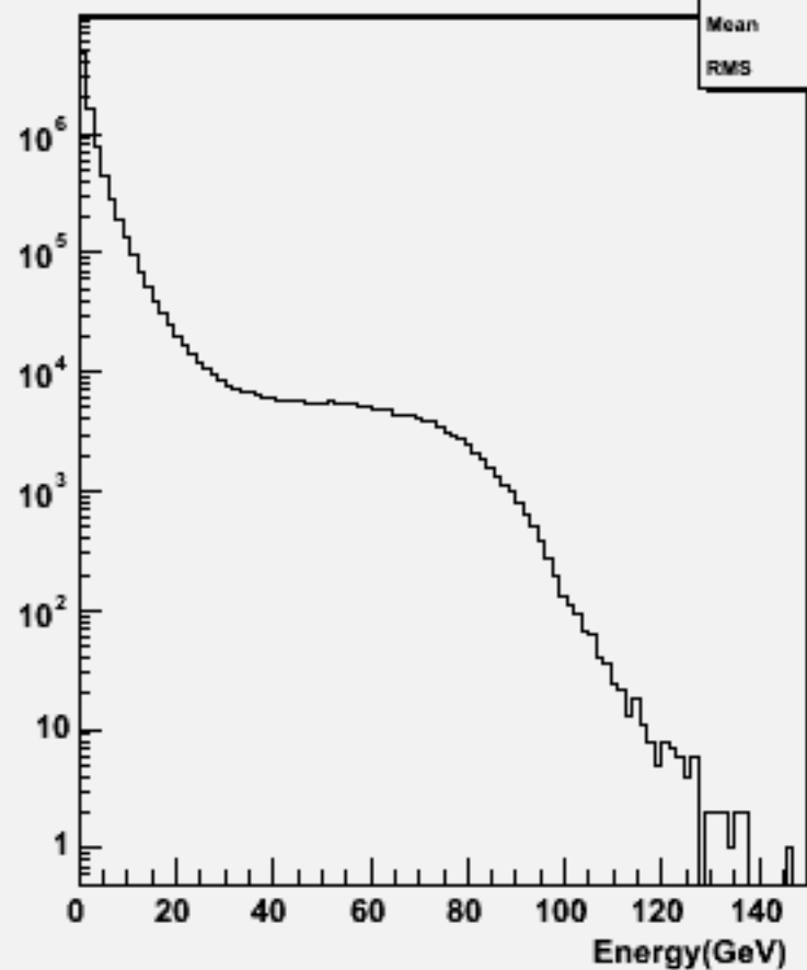
Particle Energy : p105002 bbe1n1qq_p
