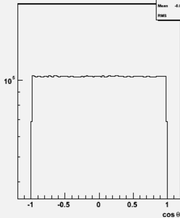
Particle cos \theta : p105000 bbqqqq_p
