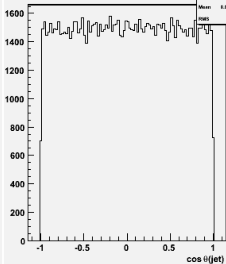
cos \theta for 2-jets : p105000 bbqqqq_p
