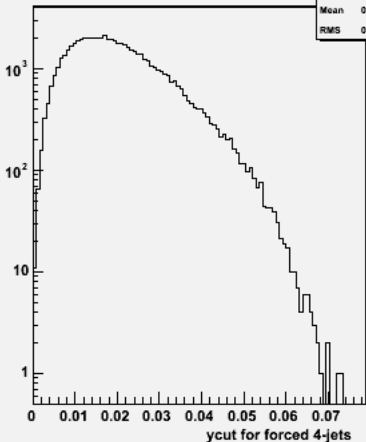
Ycut for 4-jets :p105000 bbqqqq_p
