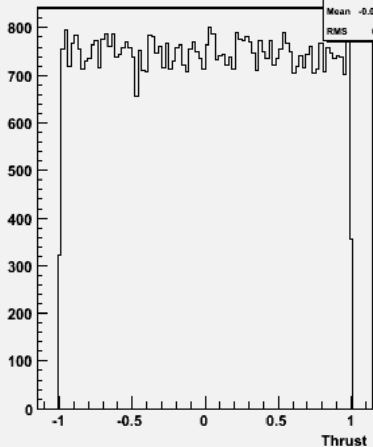
cos \Theta (thrust) p105000 bbqqqq_p
