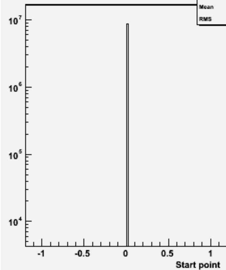
Start point Z : p105000 bbqqqq_p
