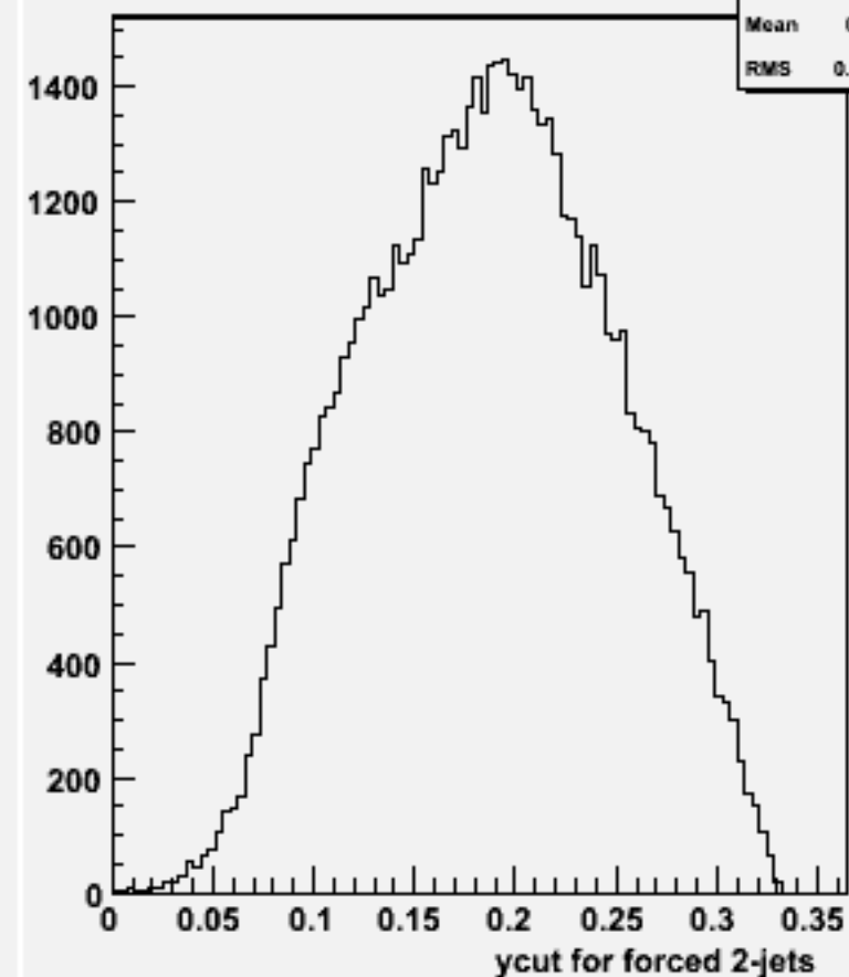
Ycut for 2-jets : p105000 bbqqqq_p
