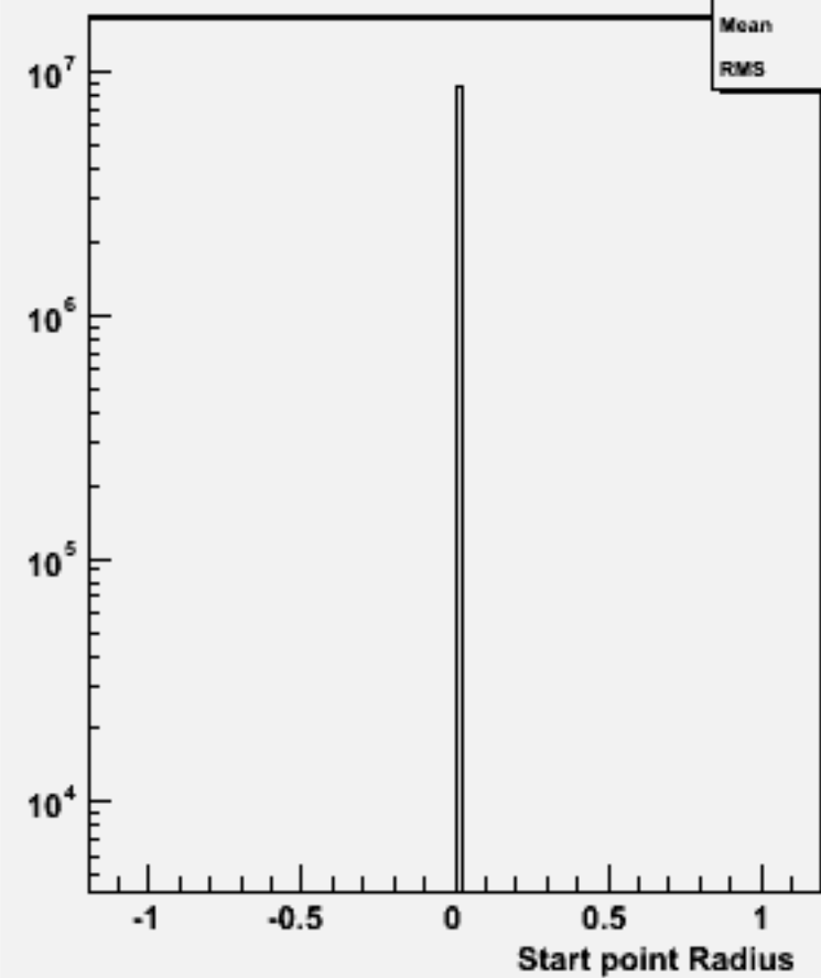
Start point R : p105000 bbqqqq_p
