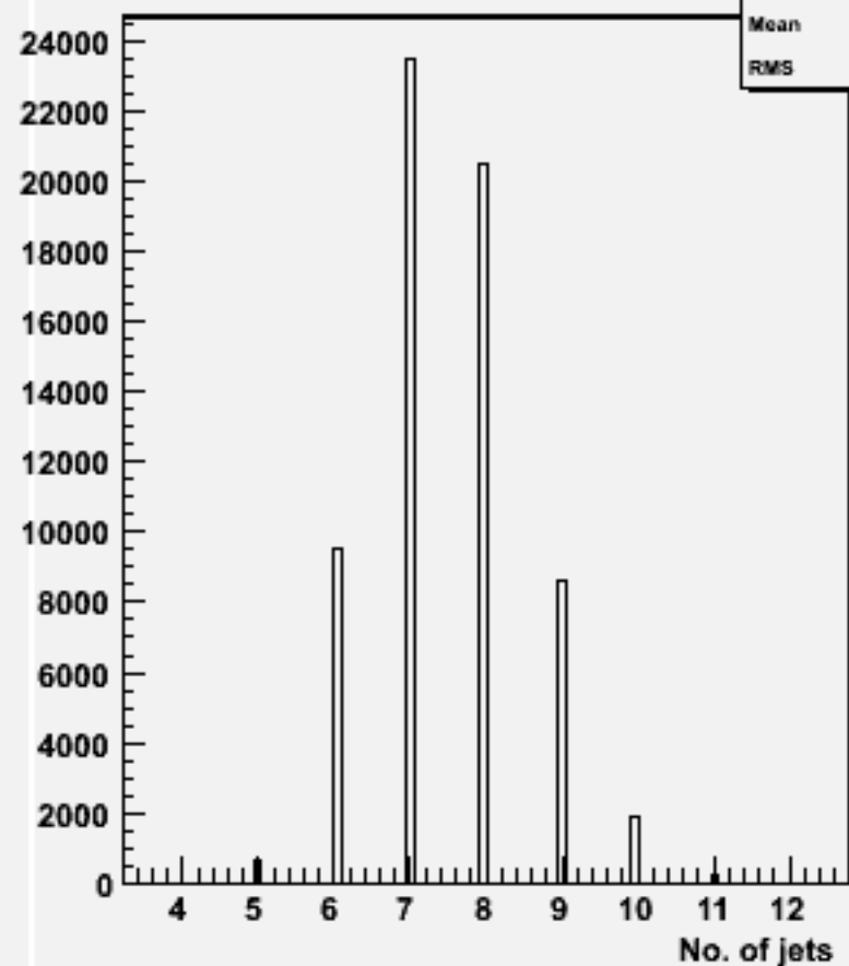
No. jets (ycut=0.001) : p105000 bbqqqq_p
