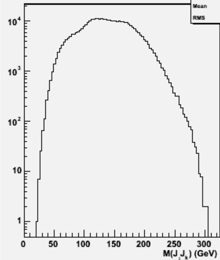
2jets mass(All comb)p105000 bbqqqq_p
