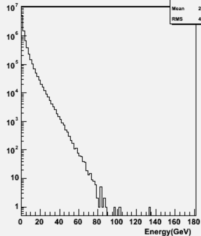
Particle Energy : p105000 bbqqqq_p
