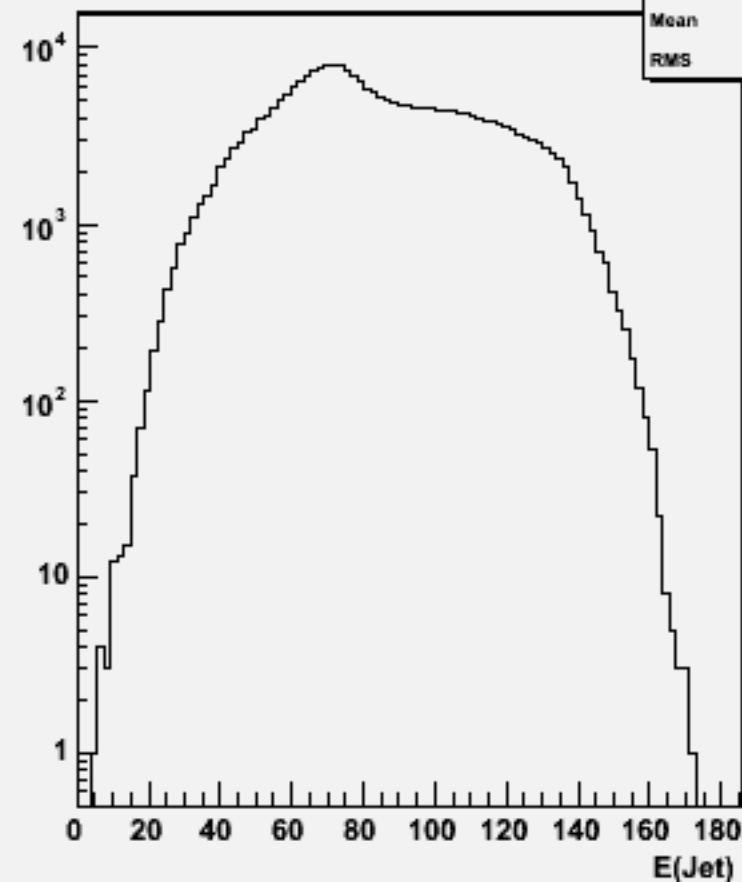
Jet energies(All jets)p105000 bbqqqq_p
