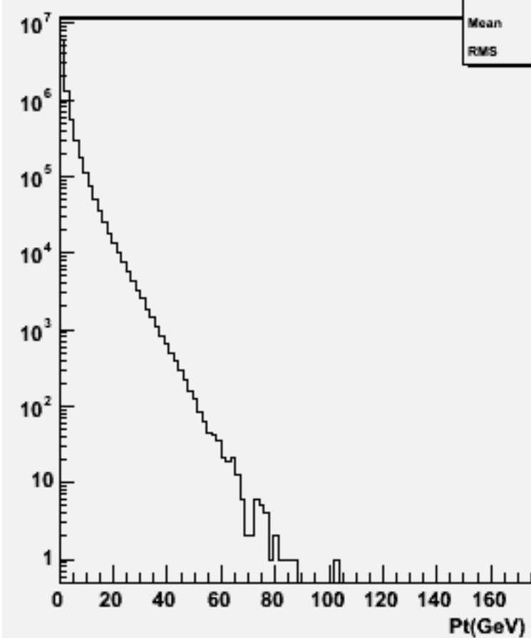
Particle Pt : p105000 bbqqqq_p
