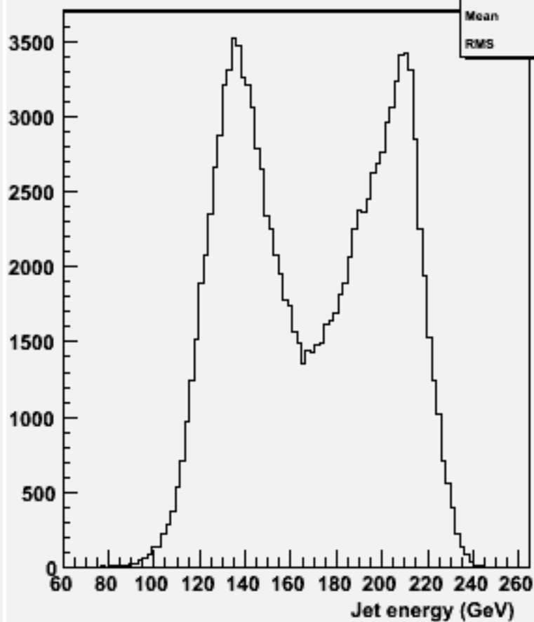
energy for 2-jets : p105000 bbqqqq_p
