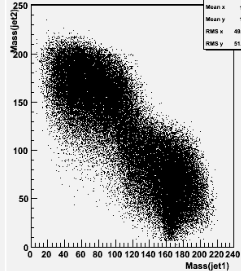
Jet mass for forced 2-jets : p105000 bbqqqq_p
