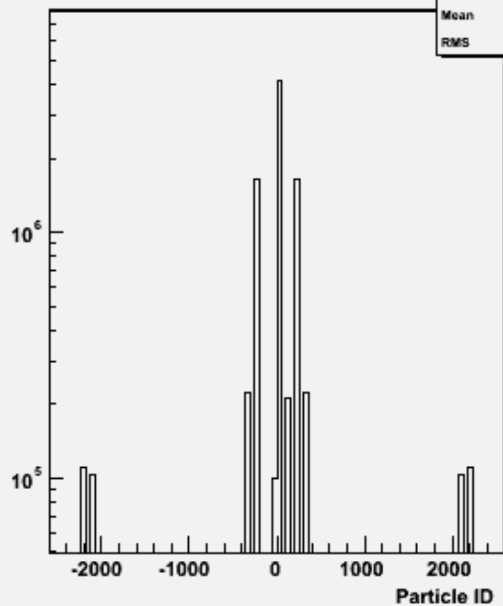
Particle ID : p105000 bbqqqq_p
