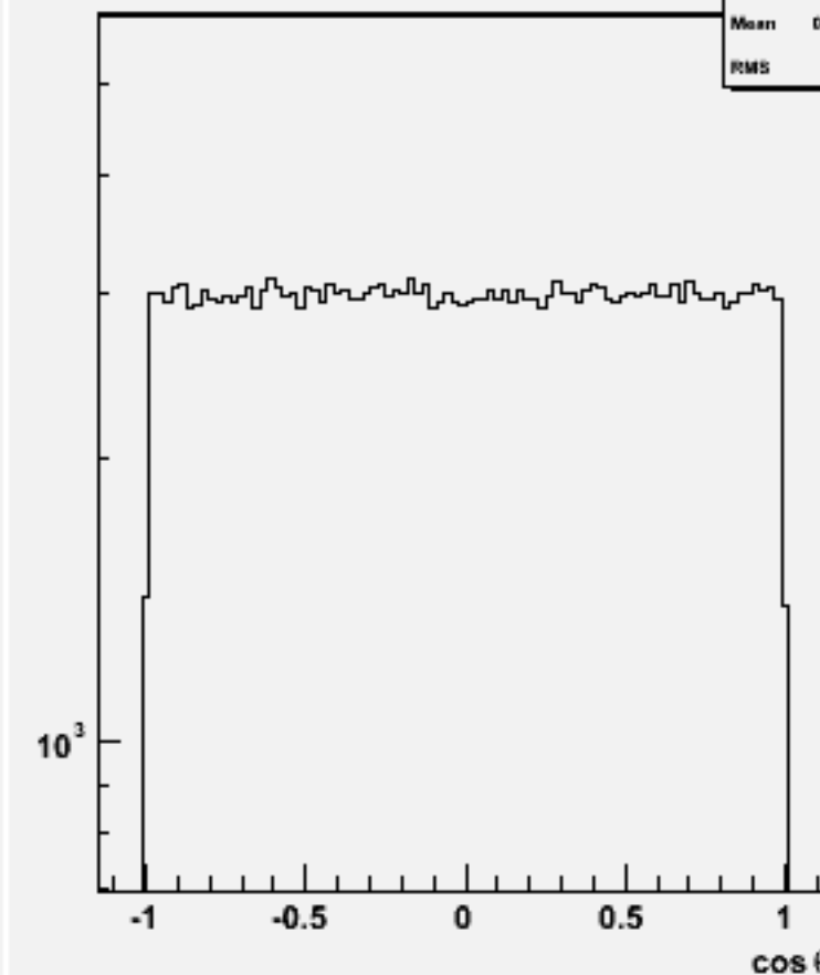
Jet cos \theta (All jets)p105000 bbqqqq_p
