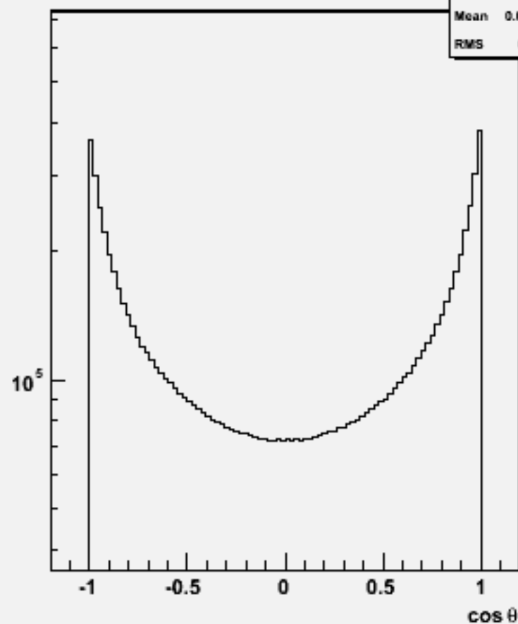
Particle cosθ : w104767 bb_o
