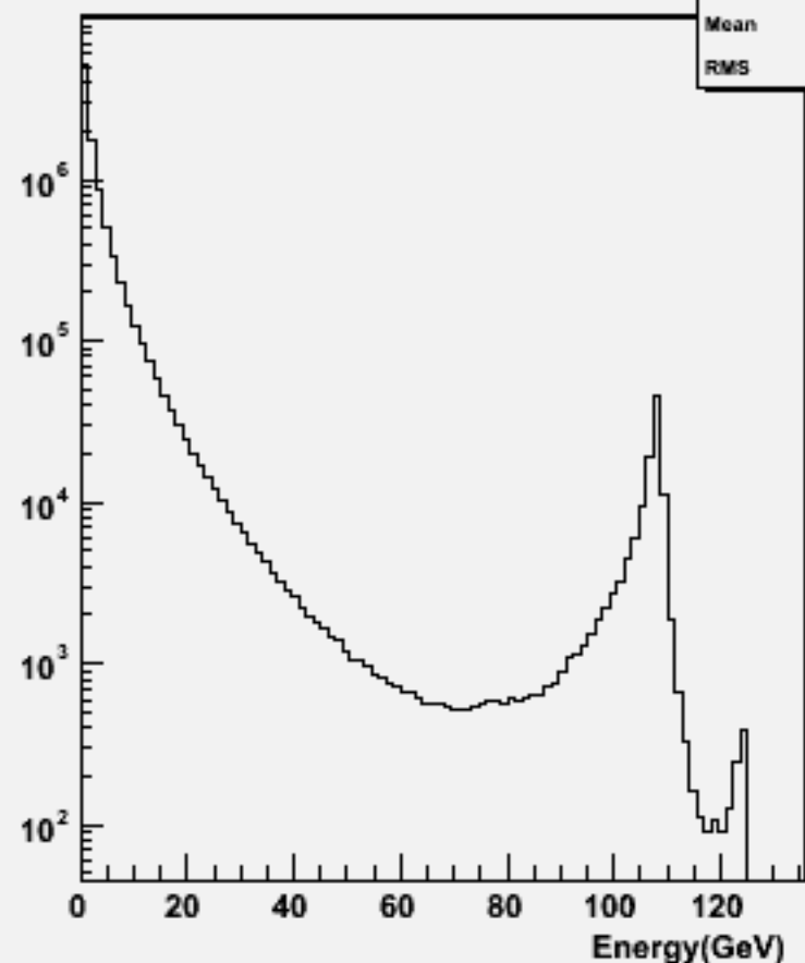
Particle Energy : w104767 bb_o
