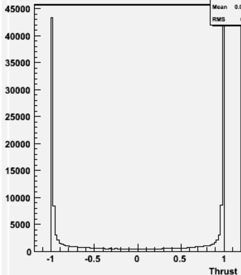
cos \Theta (thrust) w104767 bb_o
