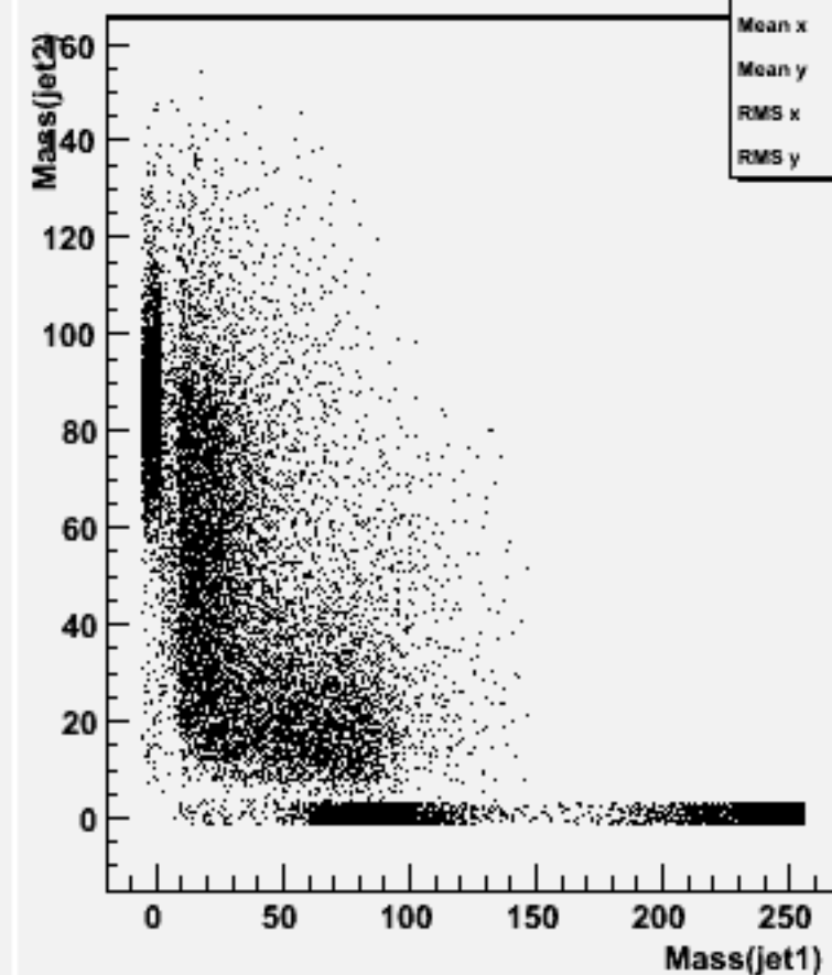
Jet mass for forced 2-jets : w104767 bb_o
