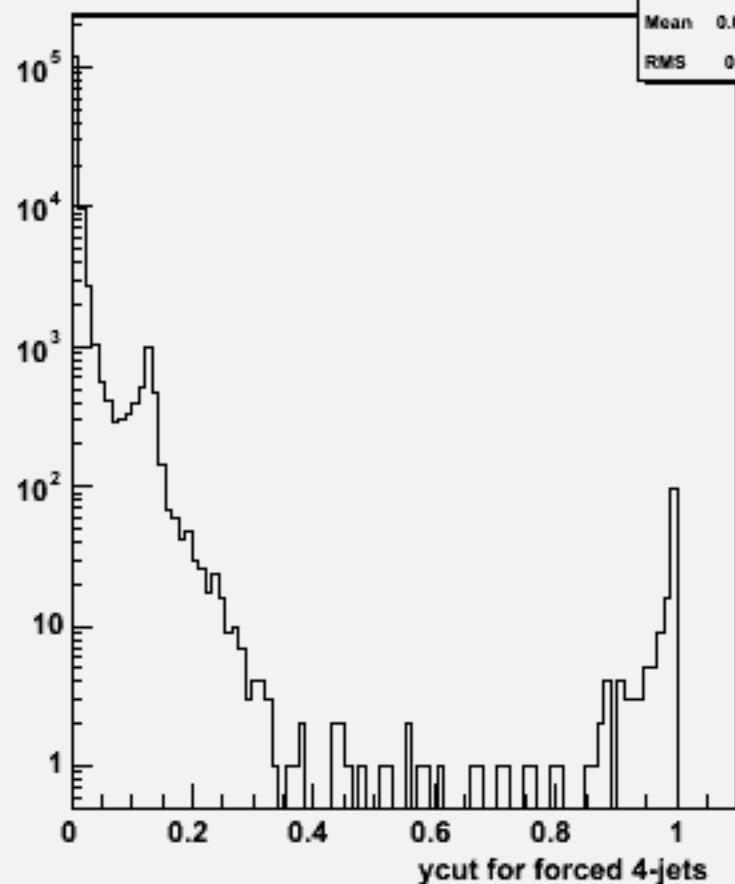
Ycut for 4-jets :w104767 bb_o
