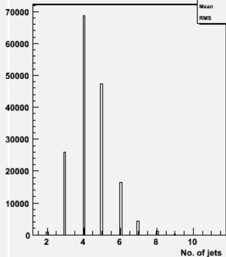
No. jets (ycut=0.001) : w104767 bb_o
