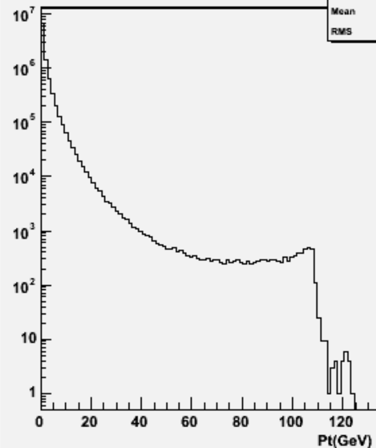
Particle Pt : w104767 bb_o
