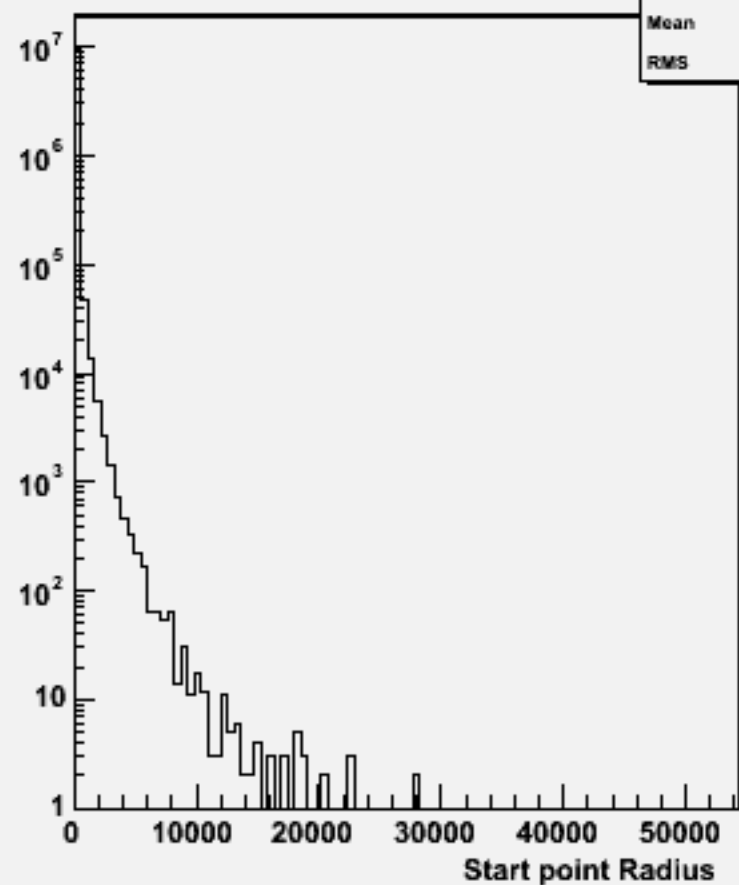
Start point R : w104767 bb_o
