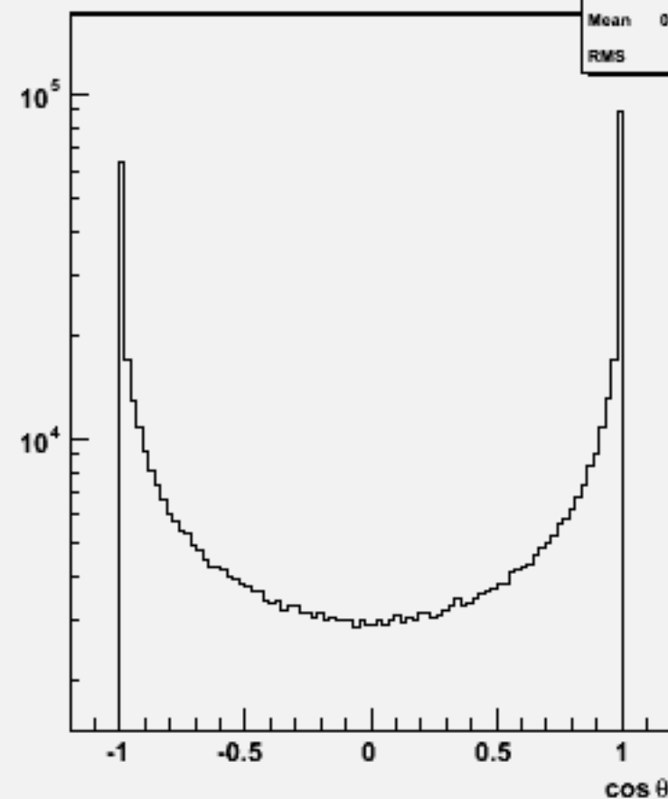
Jet cos \theta (All jets)w104767 bb_o
