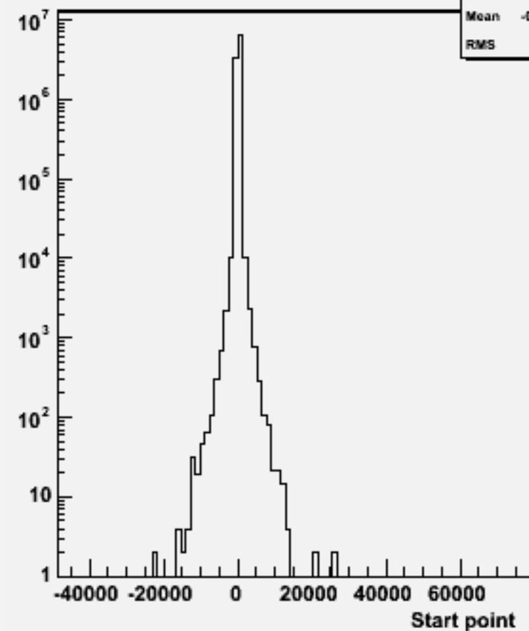
Start point Z : w104767 bb_o
