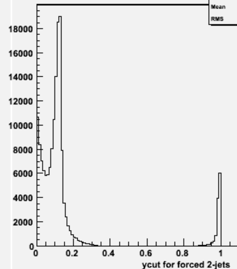
Ycut for 2-jets :w104767 bb_o
