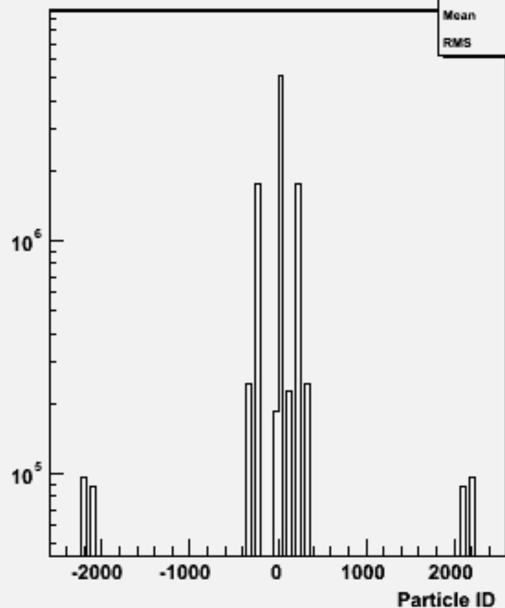
Particle ID : w104767 bb_o
