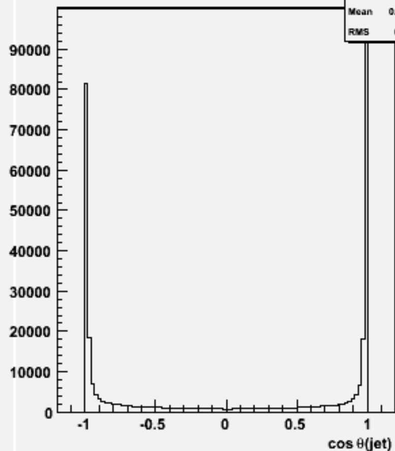
cos \Theta for 2-jets :w104767 bb_o
