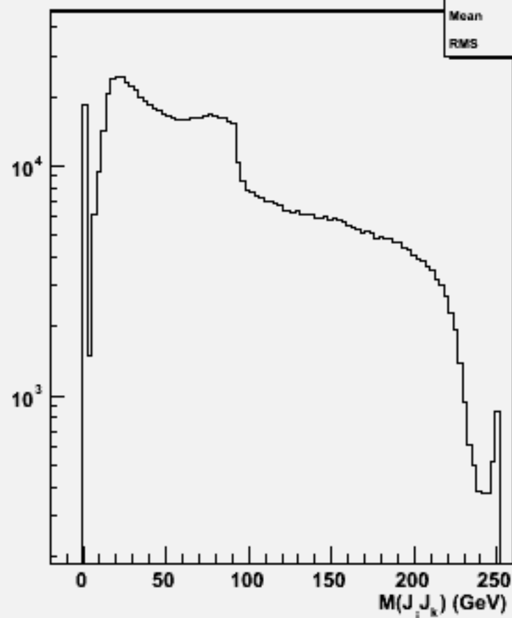
2jets mass(All comb)w104767 bb_o
