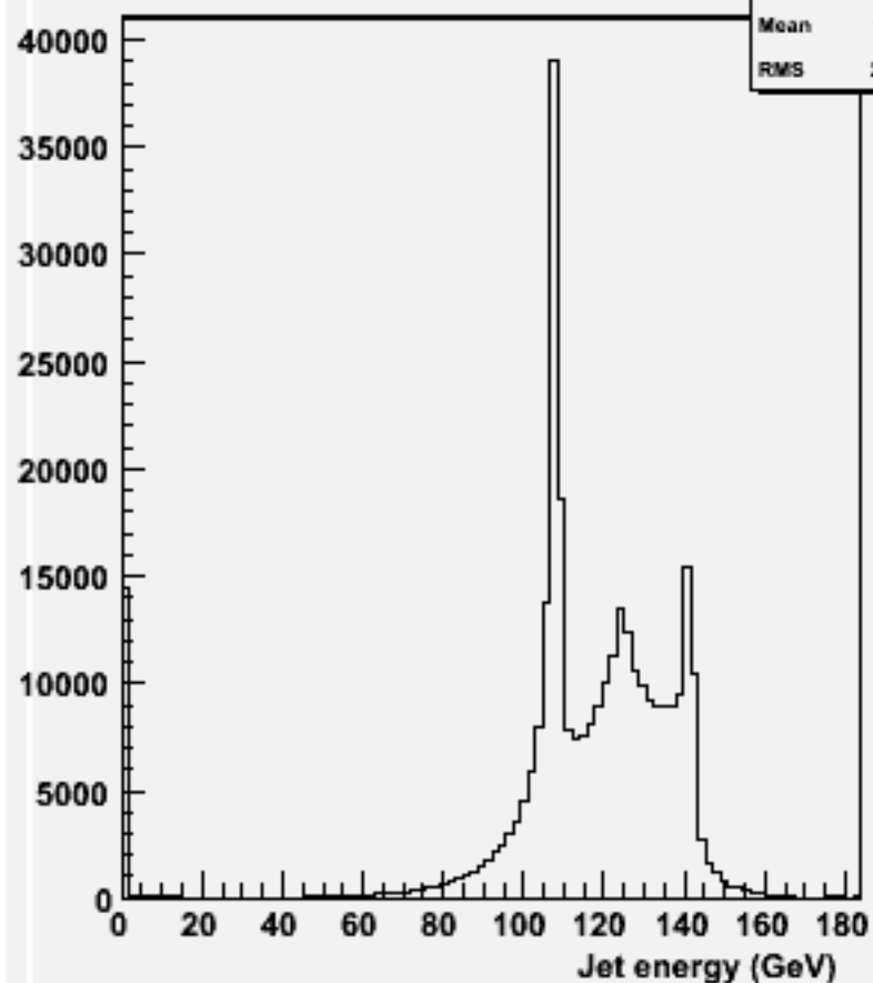
energy for 2-jets :w104767 bb_o
