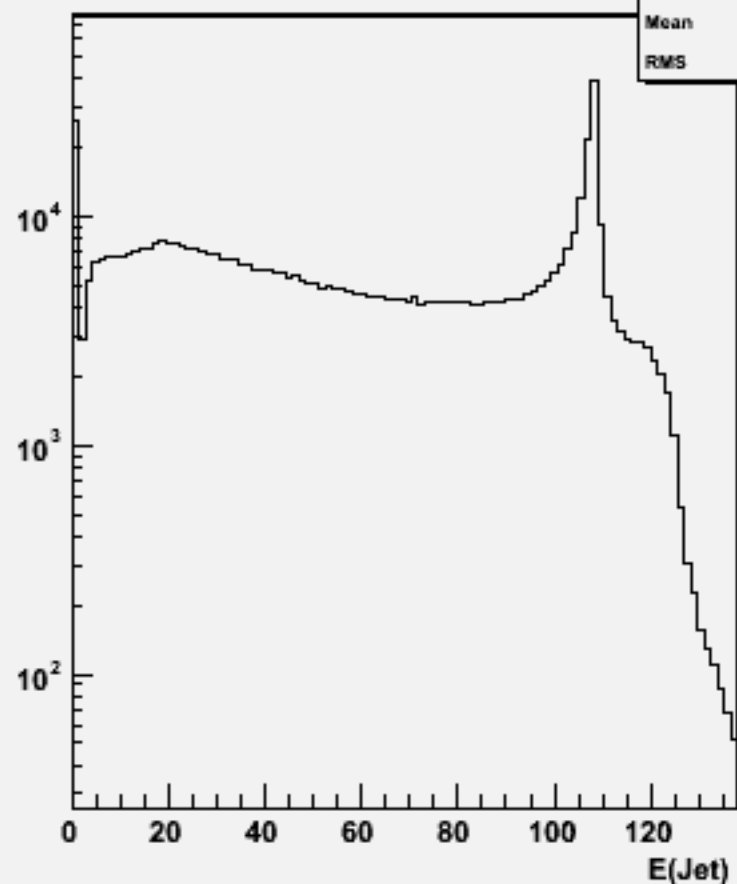
Jet energies(All jets)w104767 bb_o
