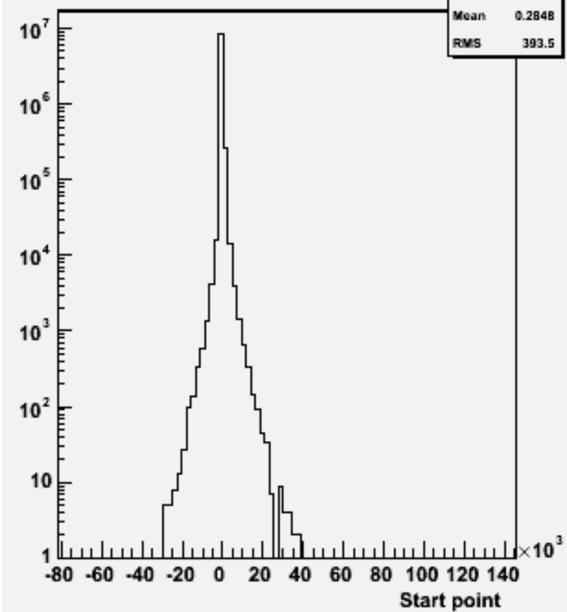
Start point Z : w104764 ss_o
