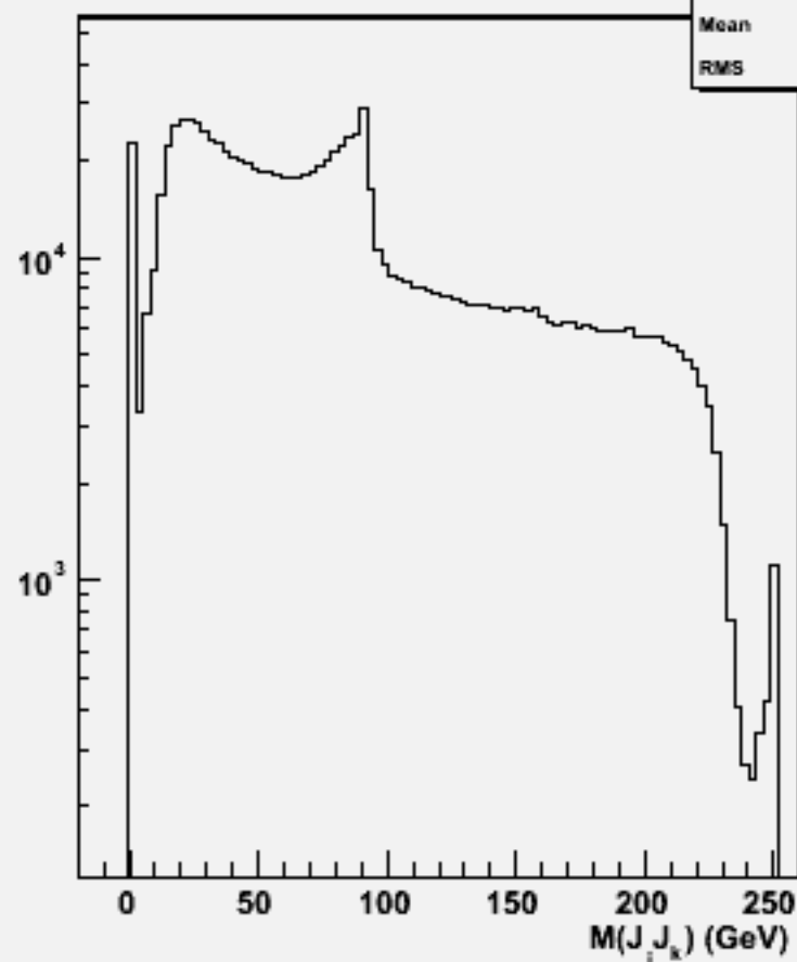
2jets mass(All comb)w104764 ss_o
