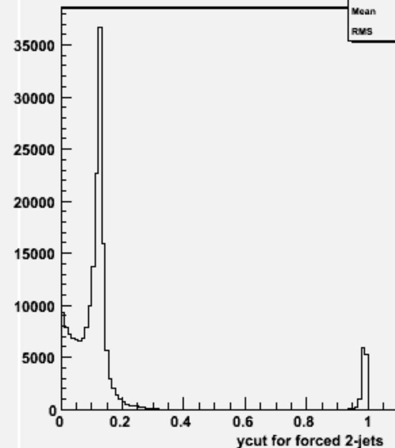
Ycut for 2-jets :w104764 ss_o
