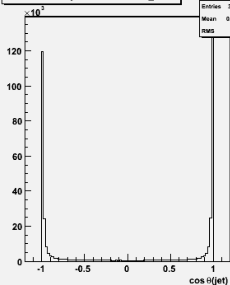
cos \theta for 2-jets :w104764 ss_o
