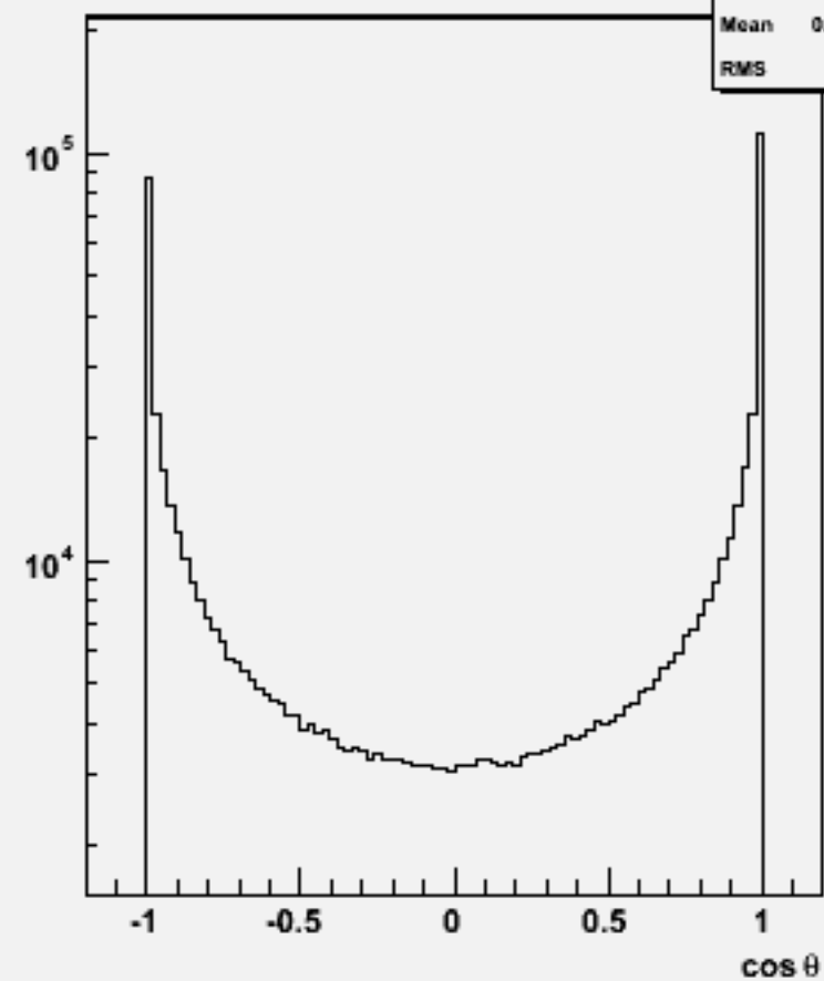
Jet cos \theta (All jets)w104764 ss_o
