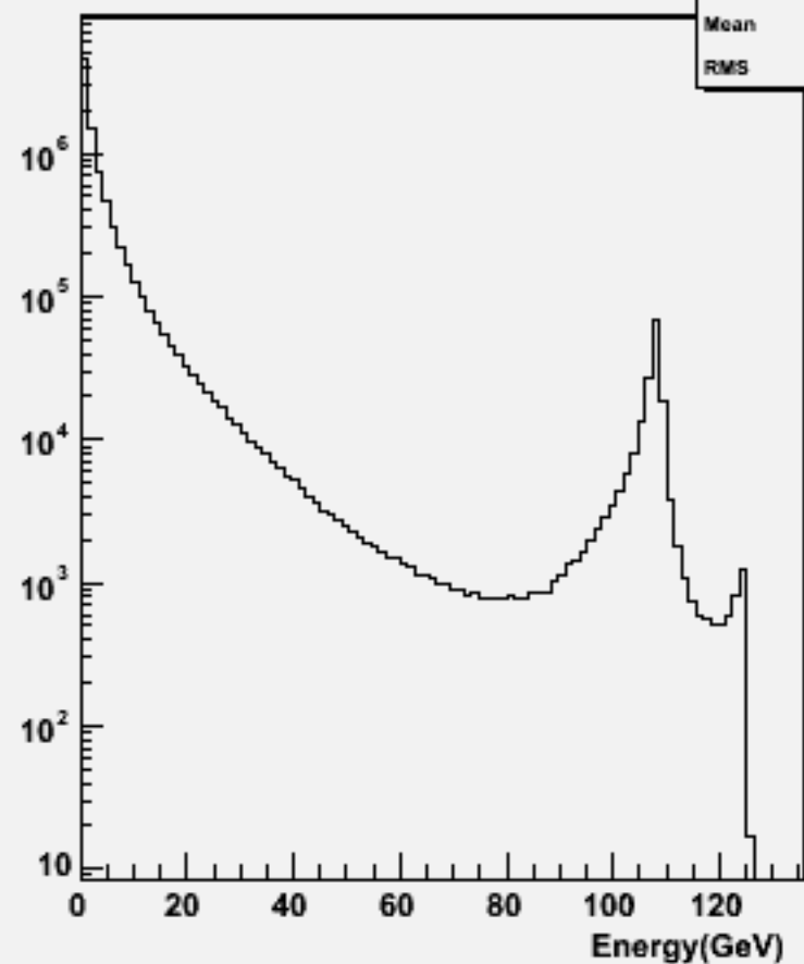
Particle Energy : w104764 ss_o
