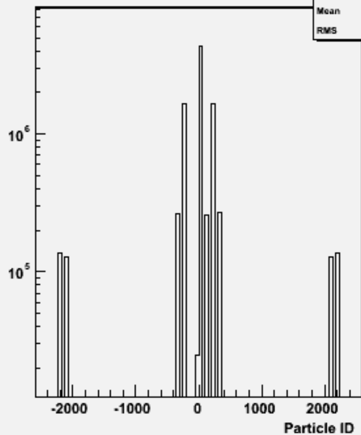
Particle ID : w104764 ss_o
