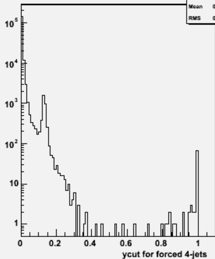
Ycut for 4-jets :w104764 ss_o
