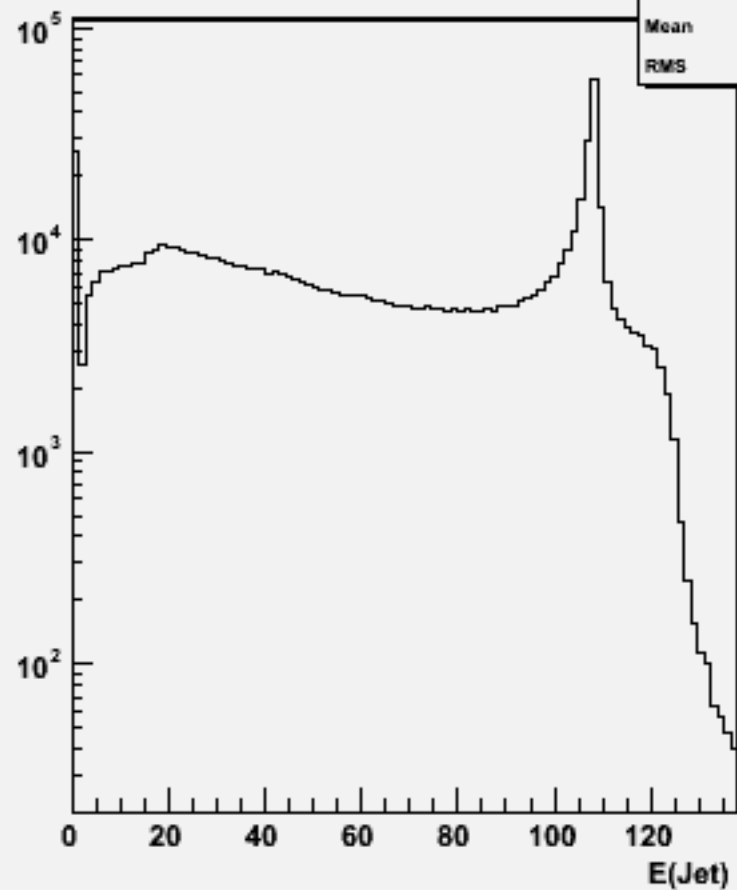
Jet energies(All jets)w104764 ss_o
