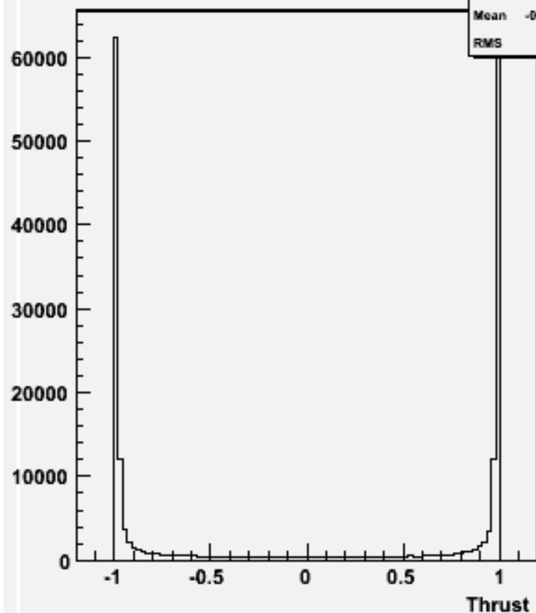
cos \Theta (thrust) w104764 ss_o
