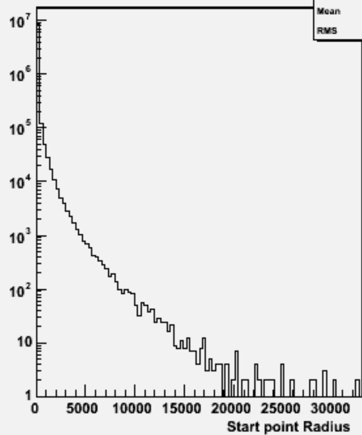
Start point R : w104764 ss_o
