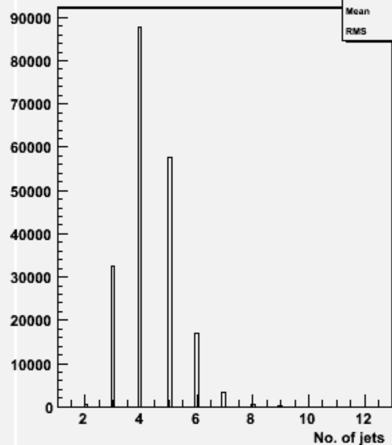
No. jets (ycut=0.001) : w104764 ss_o
