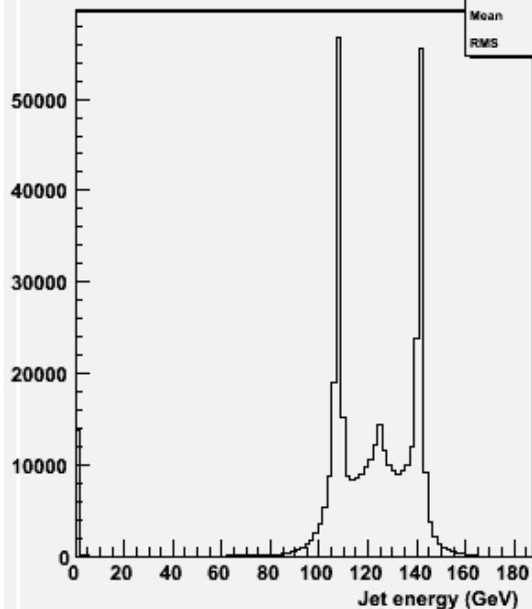
energy for 2-jets :w104764 ss_o
