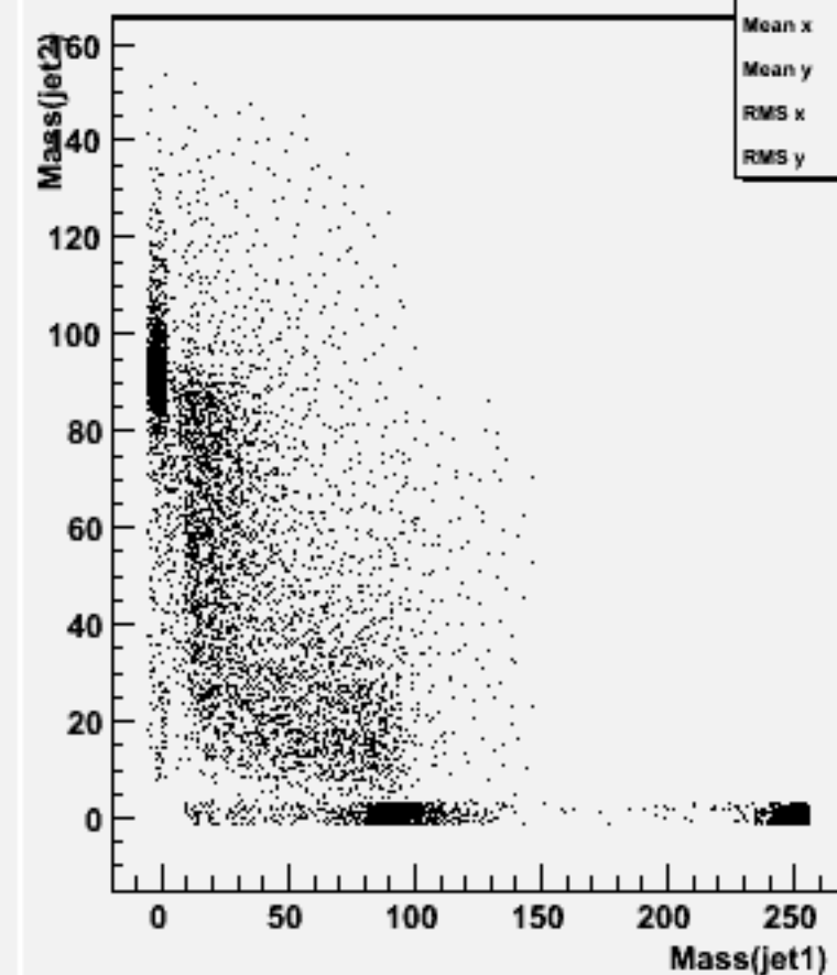
Jet mass for forced 2-jets : w104764 ss_o
