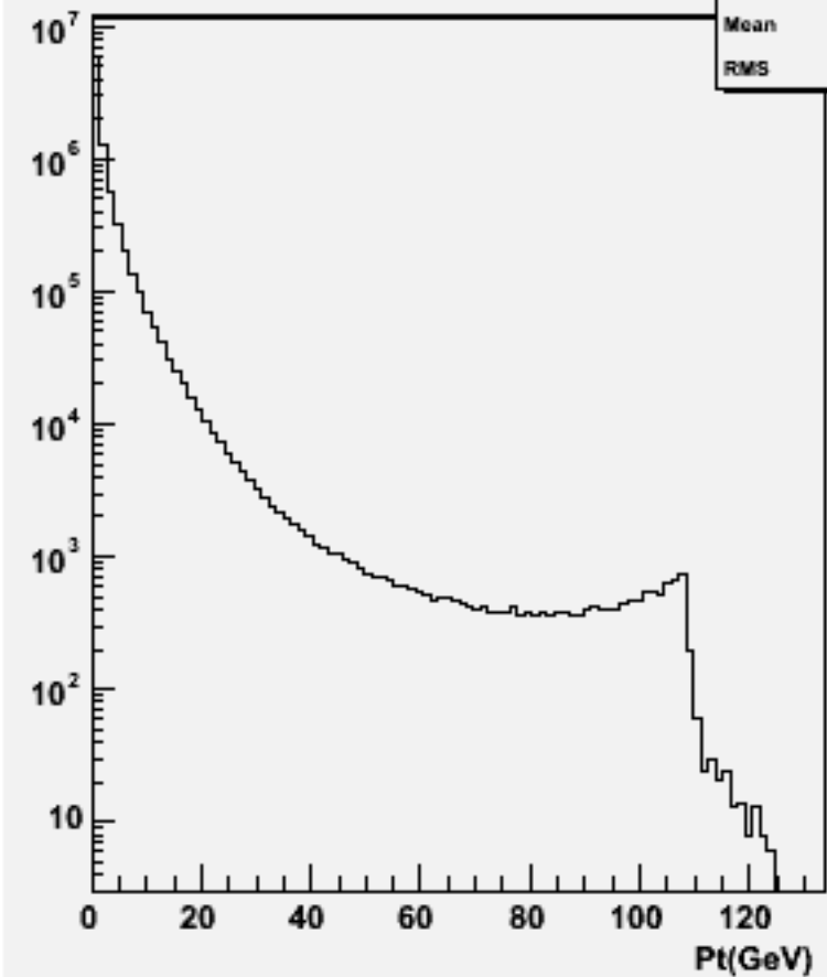
Particle Pt : w104764 ss_o
