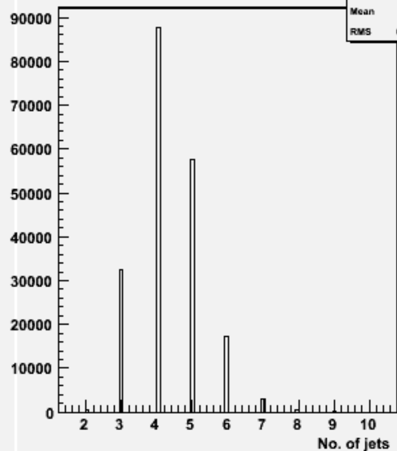
No. jets (ycut=0.001) : w104760 dd_o
