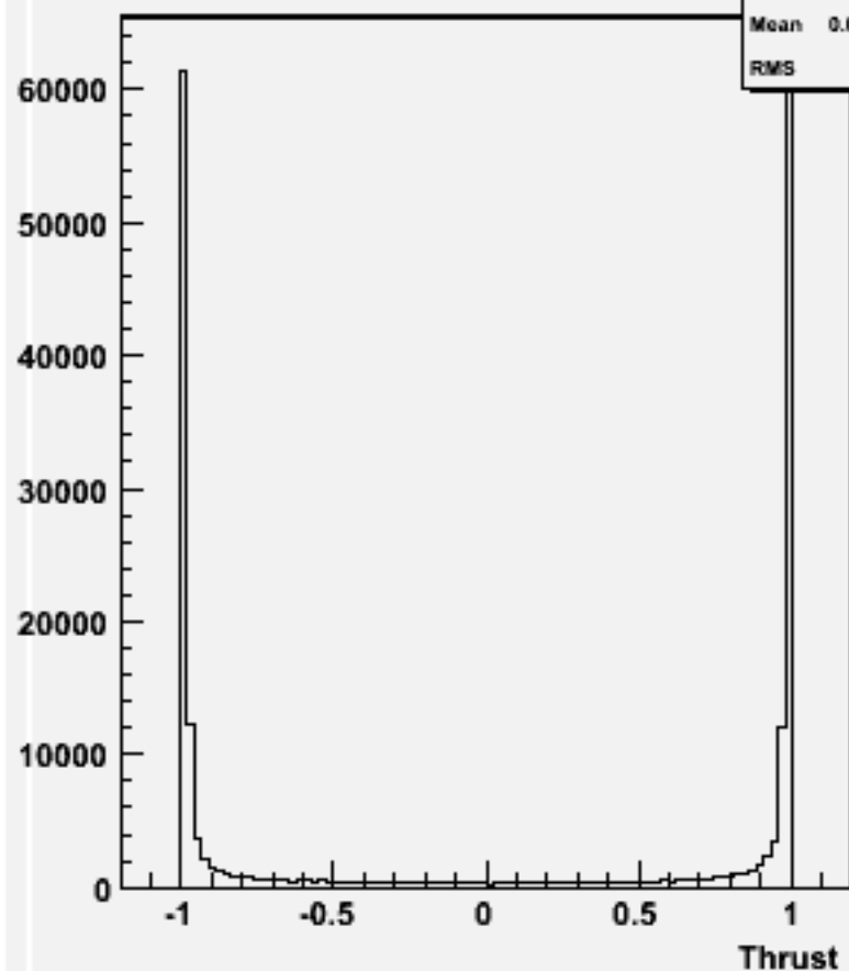
cos \Theta (thrust) w104760 dd_o
