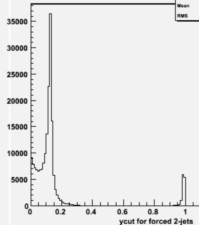
Ycut for 2-jets :w104760 dd_o
