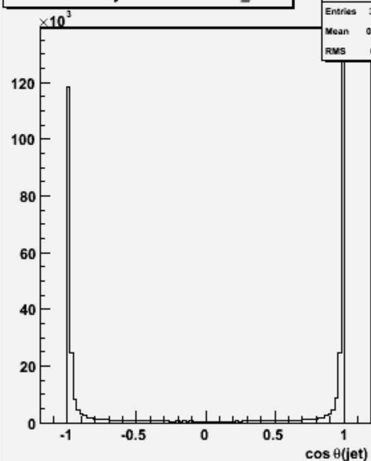
cos \theta for 2-jets :w104760 dd_o
