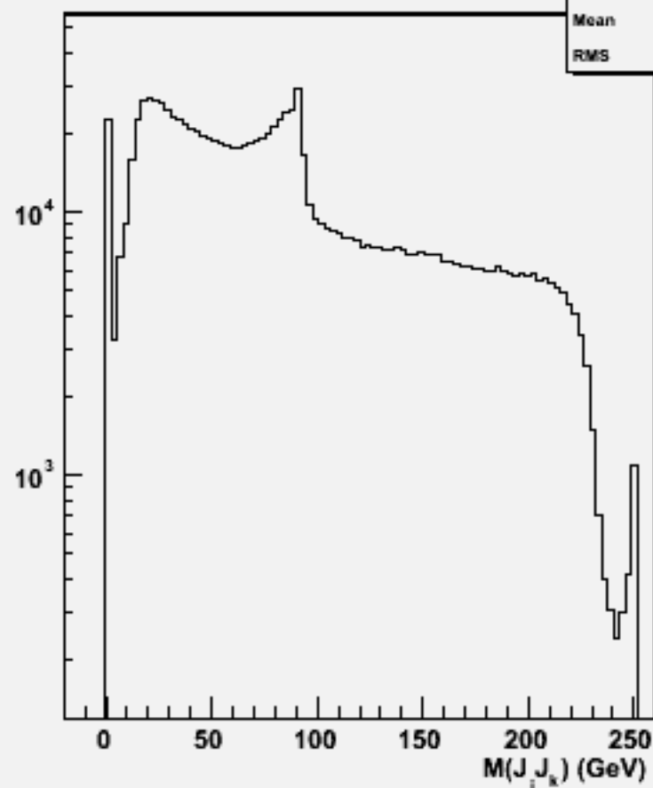
2jets mass(All comb)w104760 dd_o
