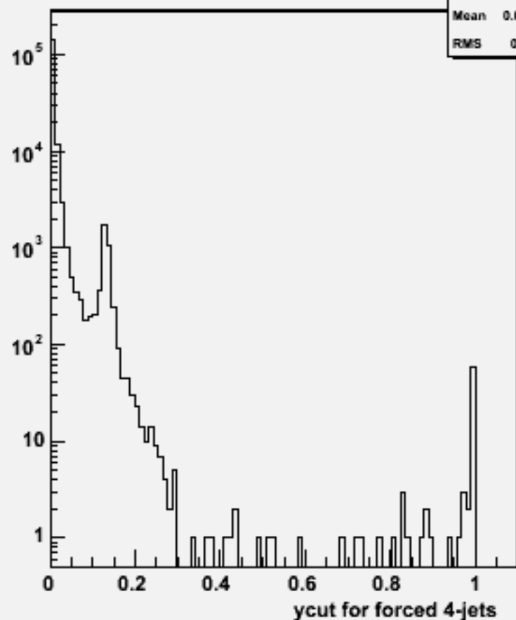
Ycut for 4-jets :w104760 dd_o
