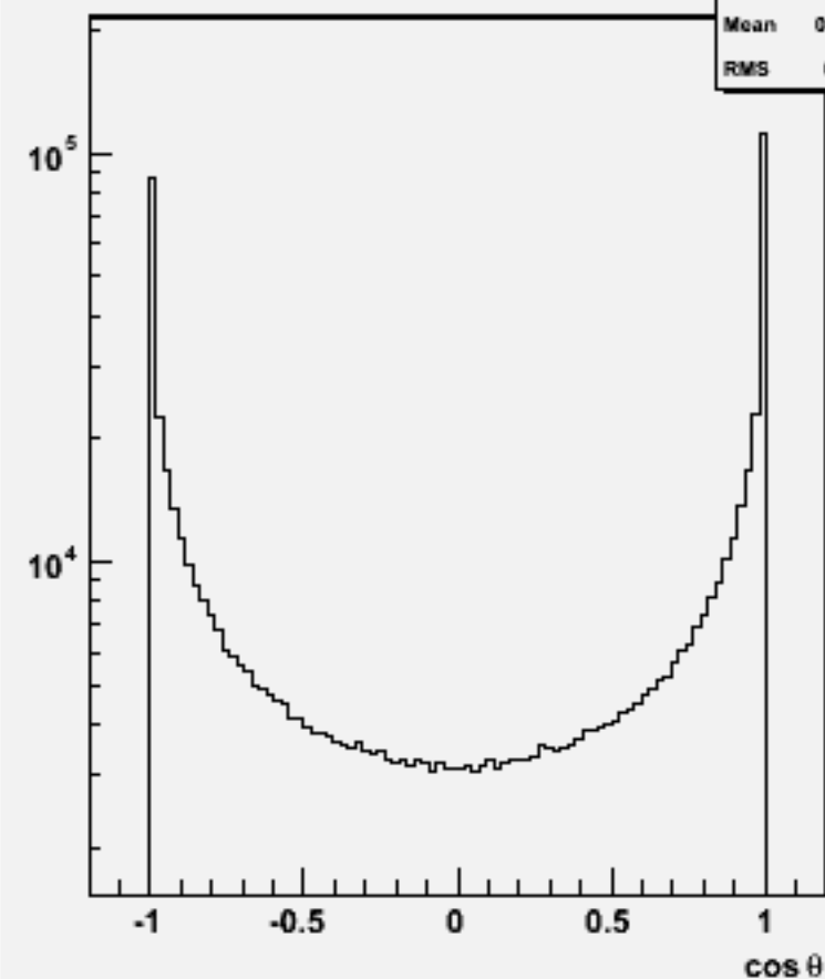
Jet cos \theta (All jets)w104760 dd_o
