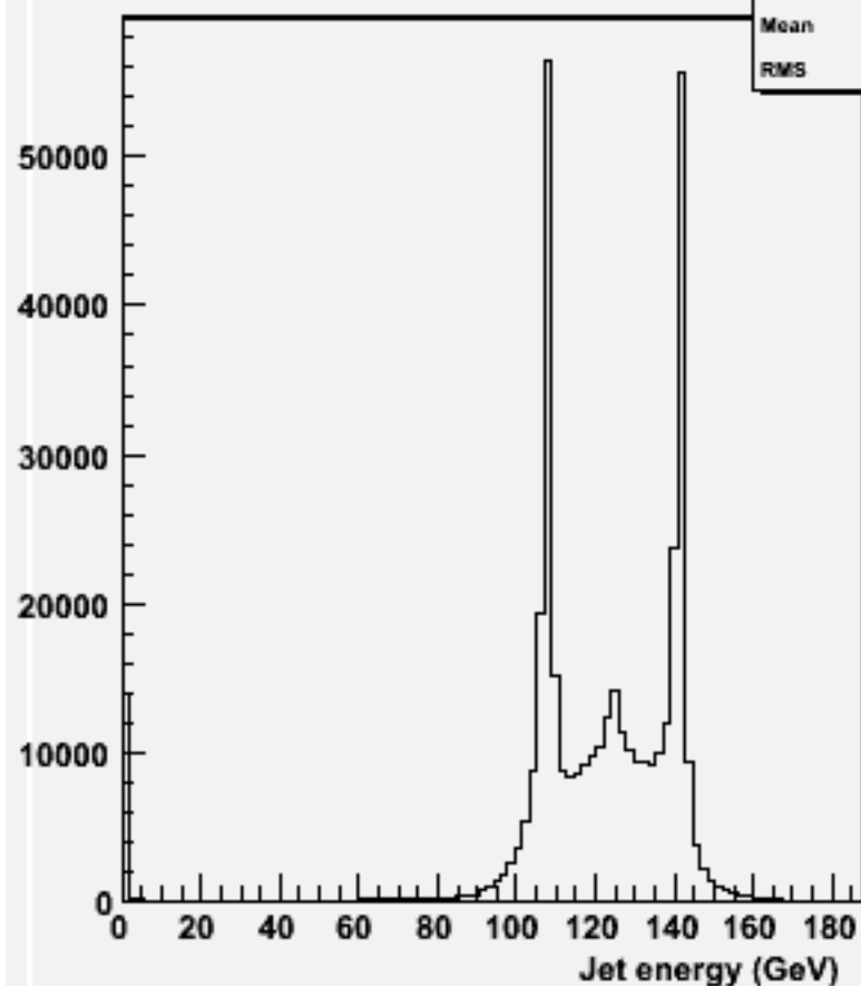
energy for 2-jets :w104760 dd_o
