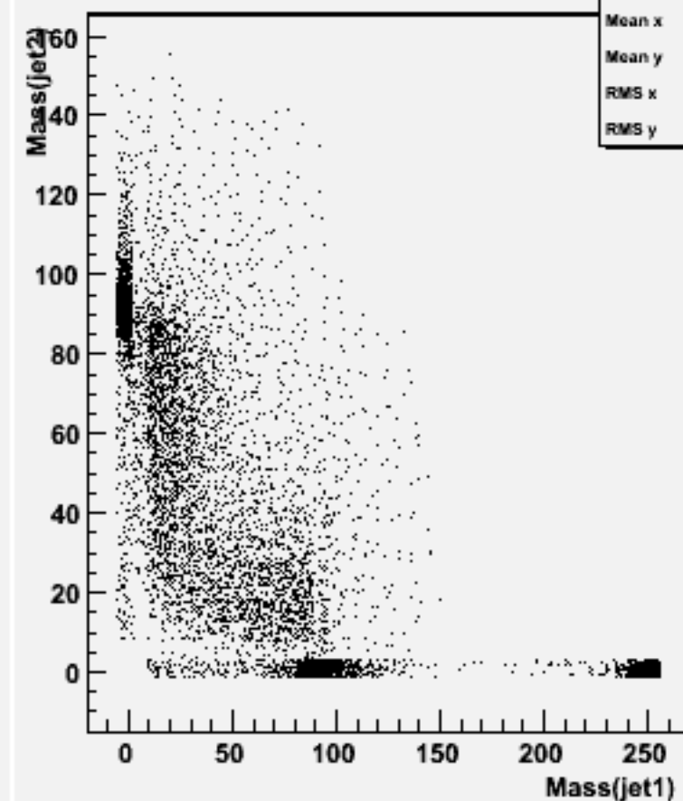
Jet mass for forced 2-jets : w104760 dd_o
