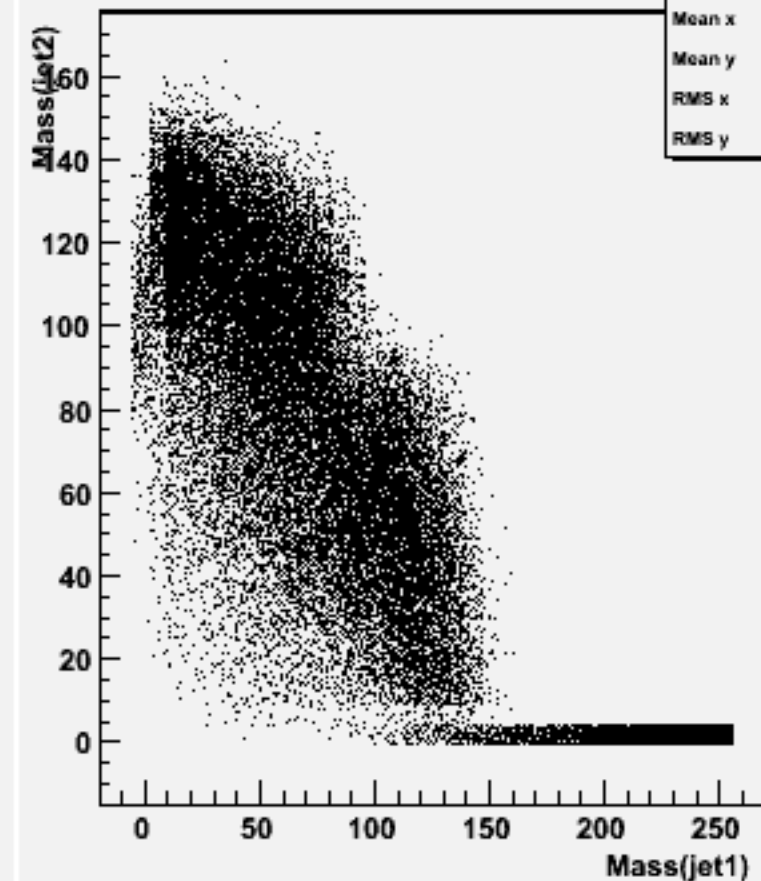
Jet mass for forced 2-jets : w104742 bbh_o
