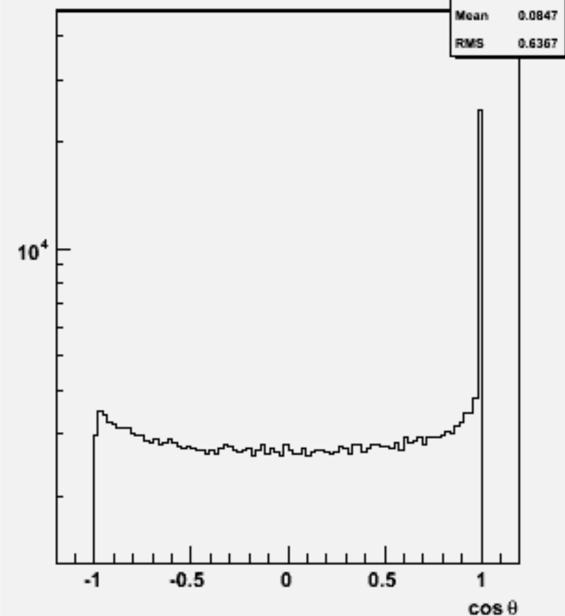
Jet cos \theta (All jets)w104742 bbh_o
