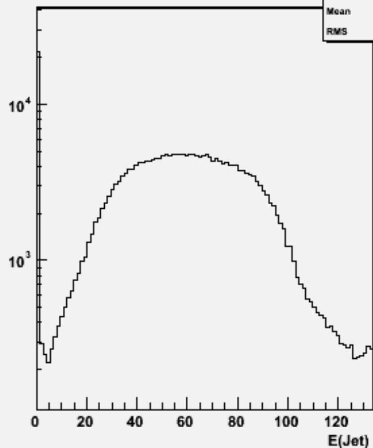
Jet energies(All jets)w104742 bbh_o
