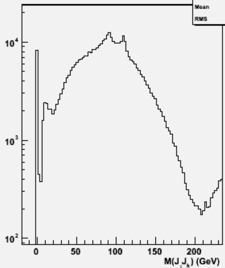
2jets mass(All comb)w104742 bbh_o
