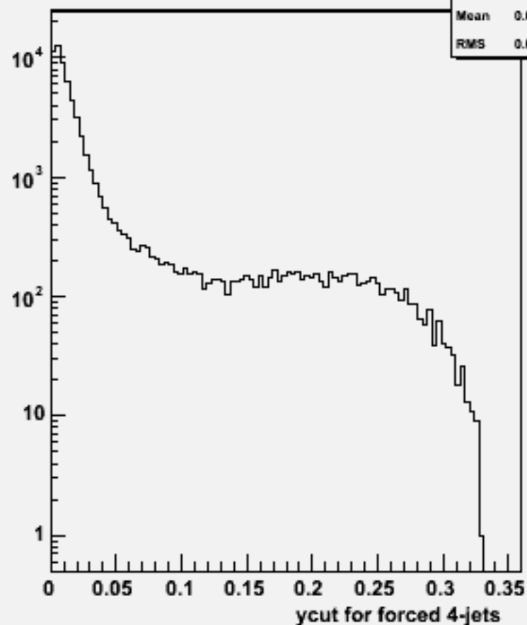
Ycut for 4-jets :w104742 bbh_o
