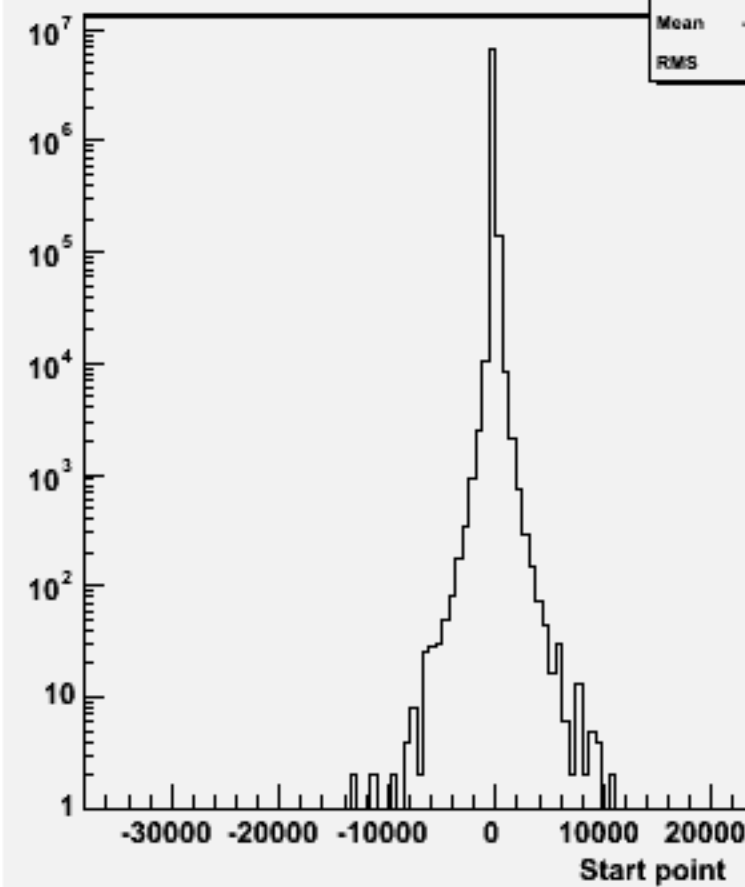
Start point Z : w104742 bbh_o
