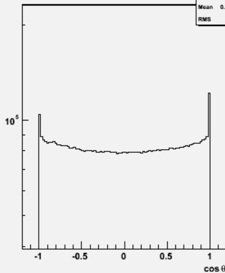
Particle cosθ : w104742 bbh_o
