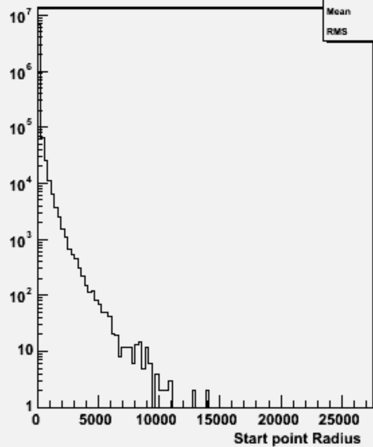
Start point R : w104742 bbh_o
