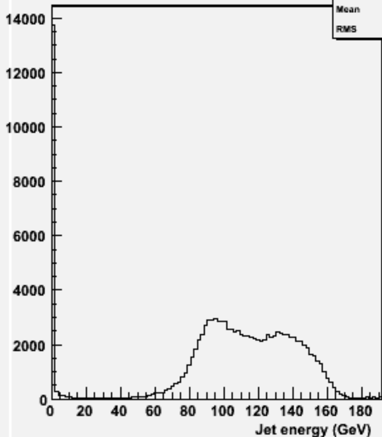
energy for 2-jets :w104742 bbh_o
